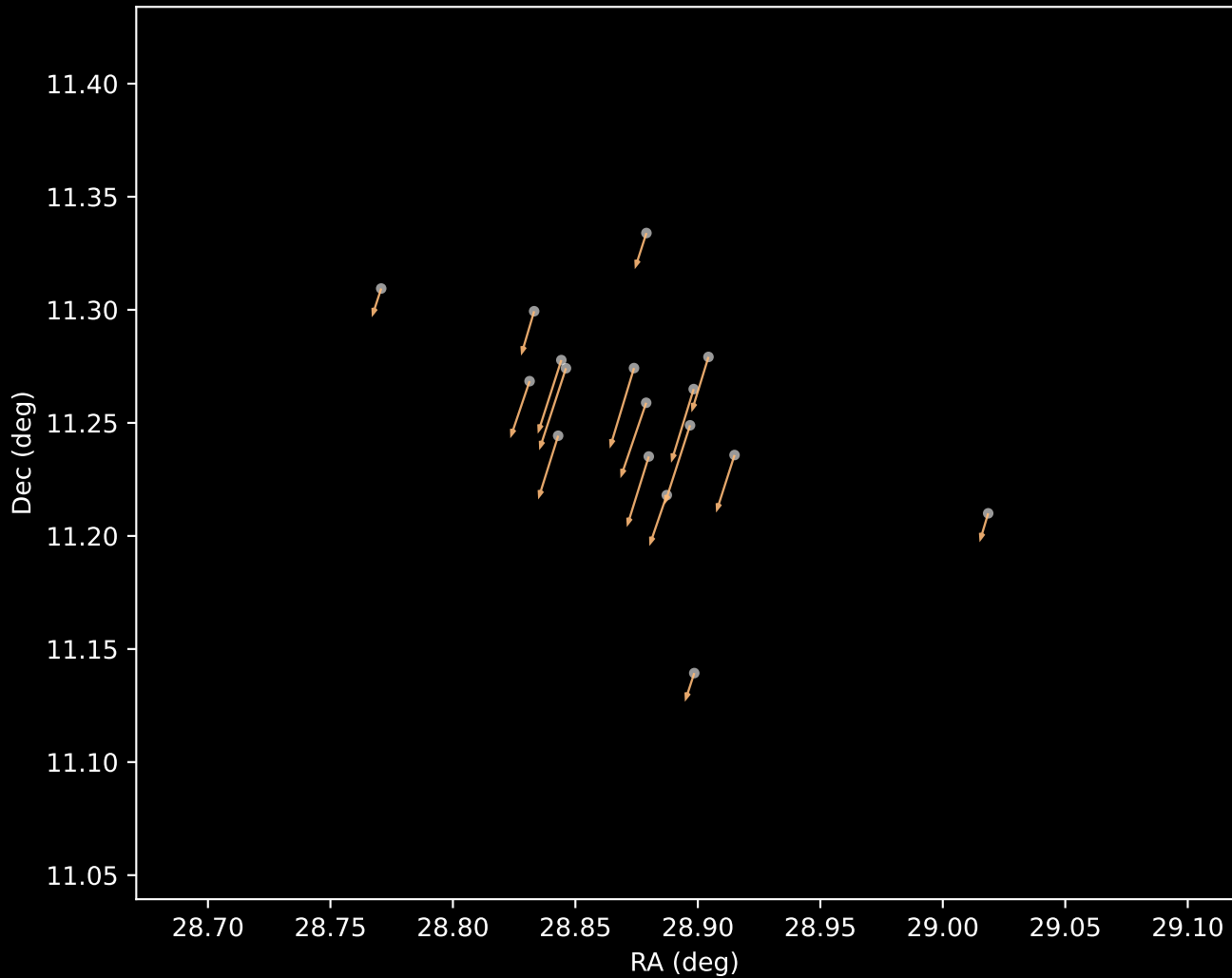
Gaia DR3 Cluster 3 Proper Motion Vectors (n=17)
