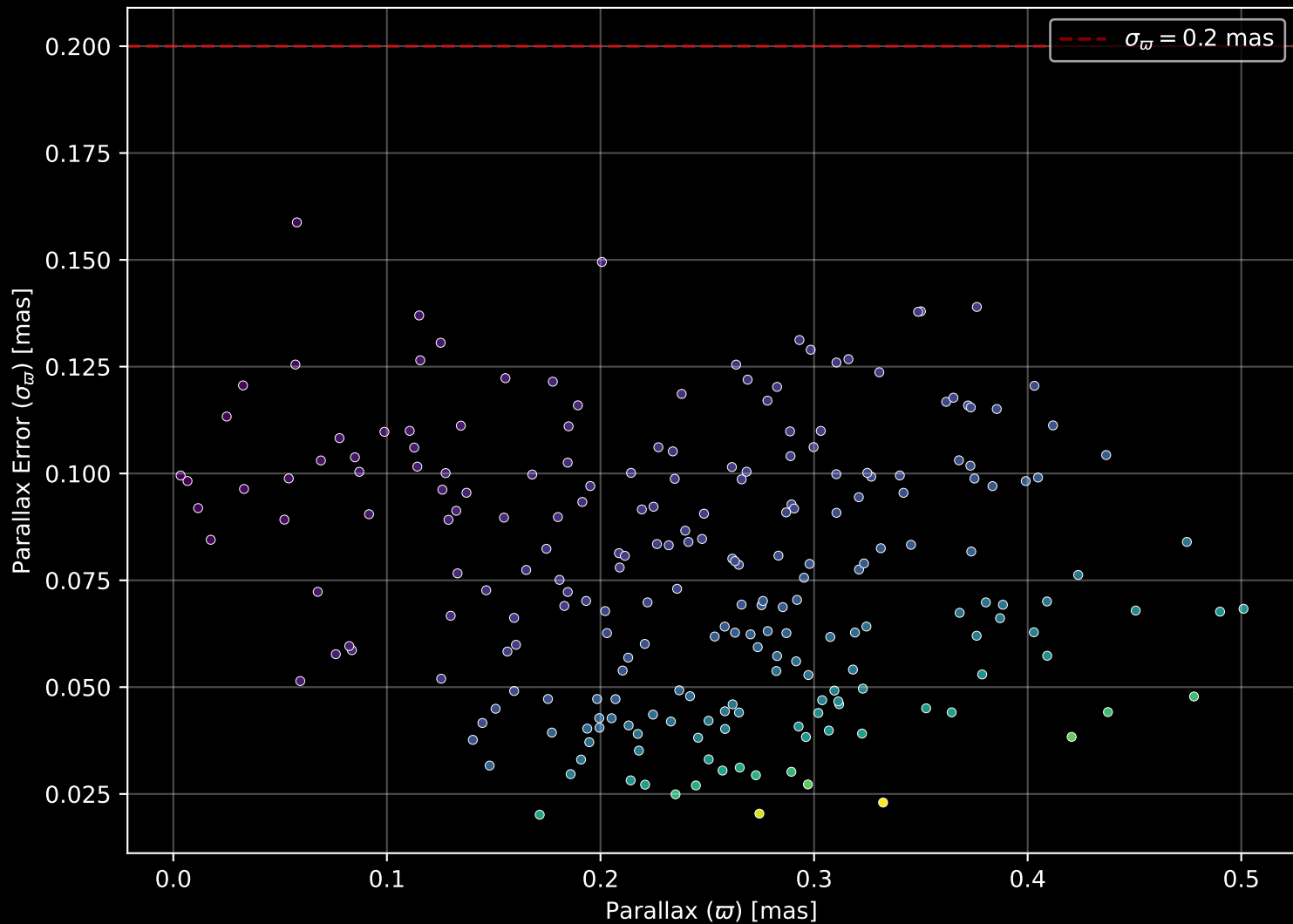
Gaia Cluster: [Berkeley_43] Parallax Quality (n= 226)
