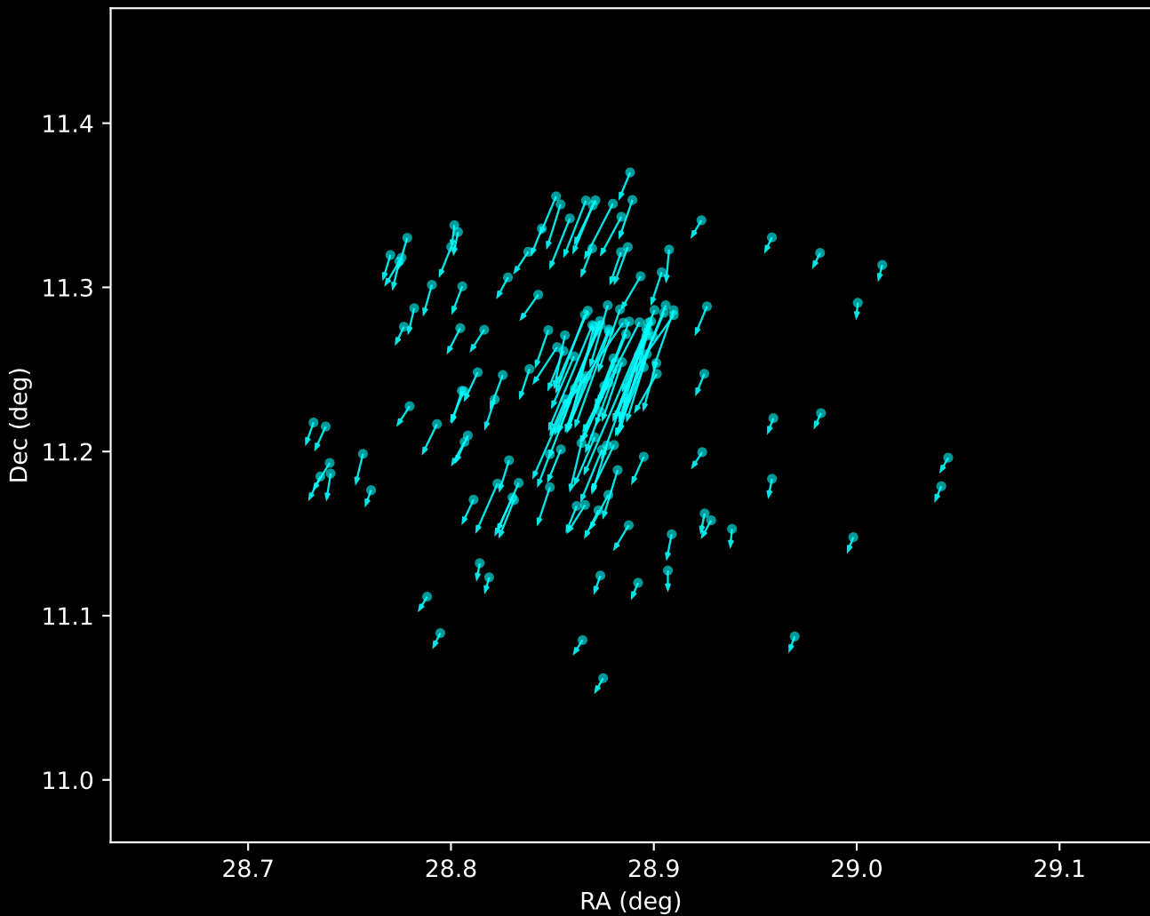
Gaia DR3 Noise Stream Proper Motion Vectors (n=146)
