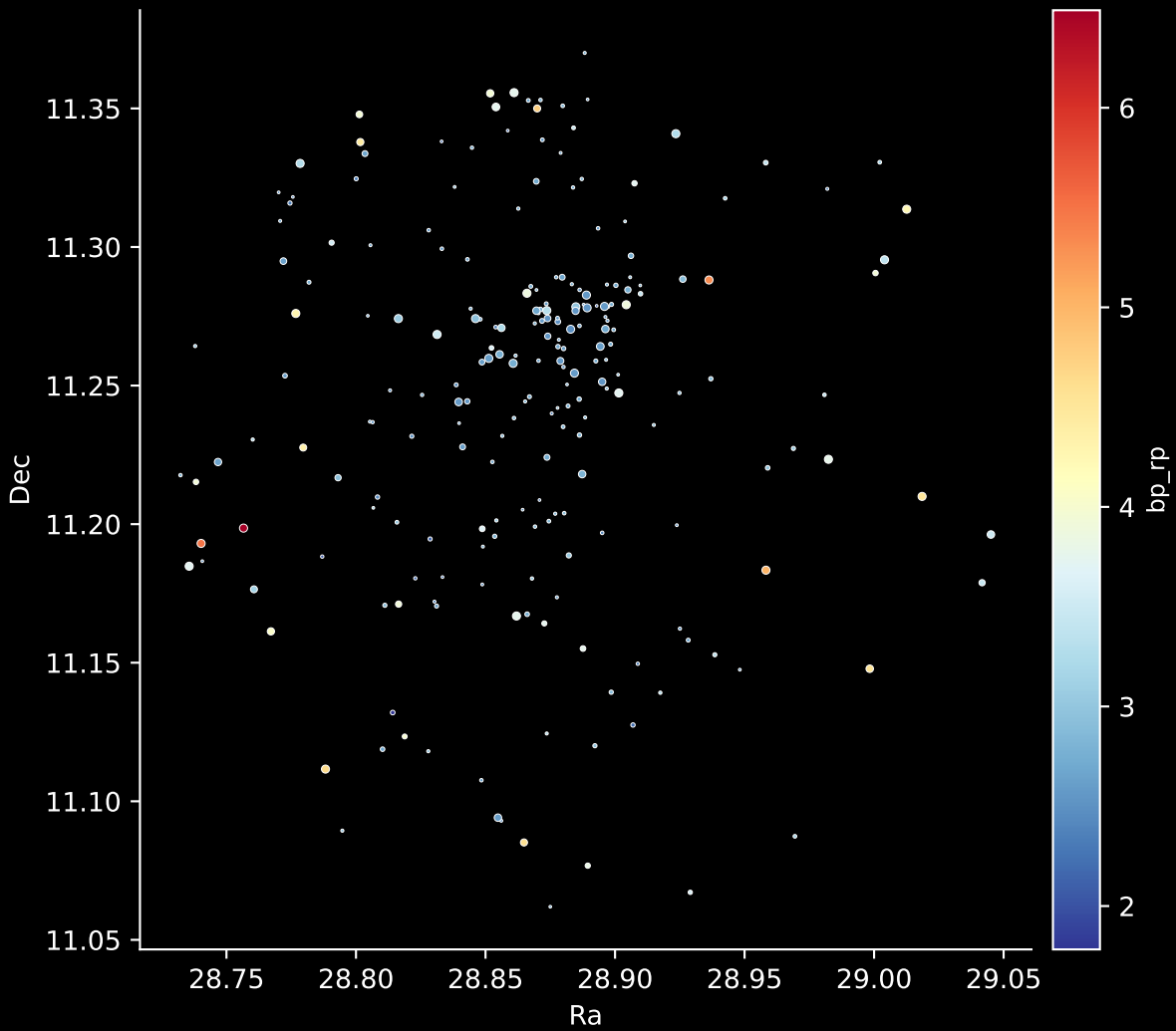
Gaia Cluster: [Berkeley_43] Stars: 226
