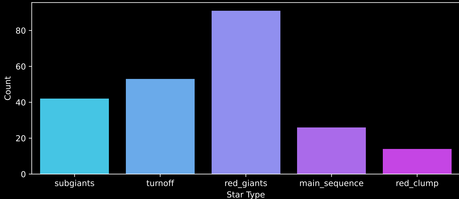
Gaia Cluster: [Berkeley_43] Count plot of Star Type
