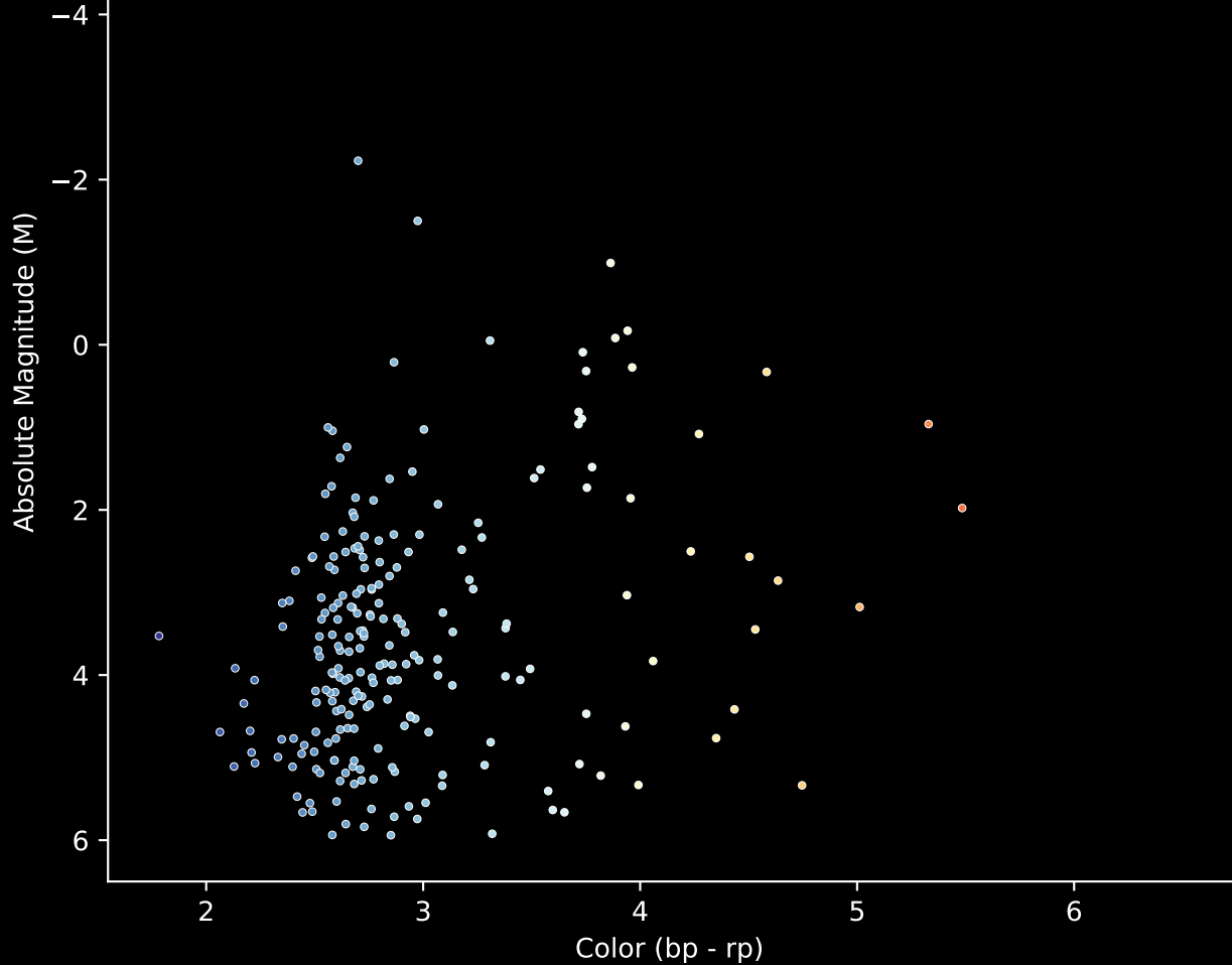
Gaia Cluster: [Berkeley_43] Stars (n= 226) Hertzprung-Russel Diagram
