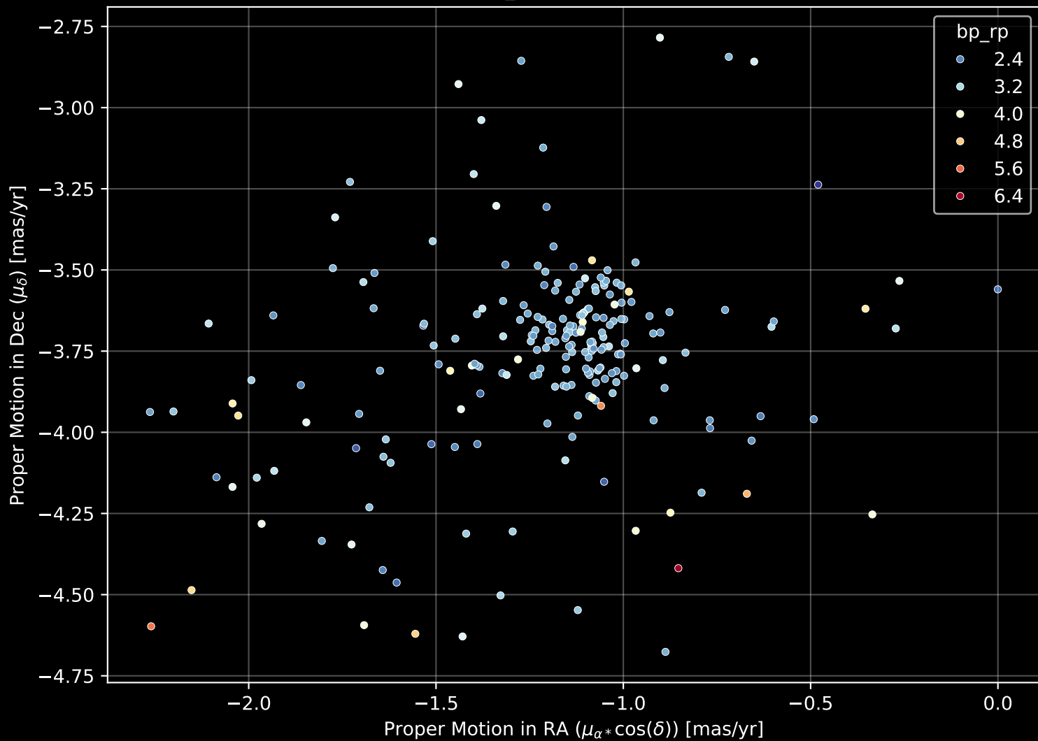
Gaia Cluster: [Berkeley_43] Proper Motion Diagram (n= 226)
