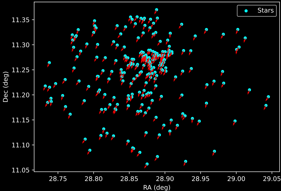
Gaia Cluster: [Berkeley_43] Proper Motion Vectors for Gaia Star Field (n= 226)
