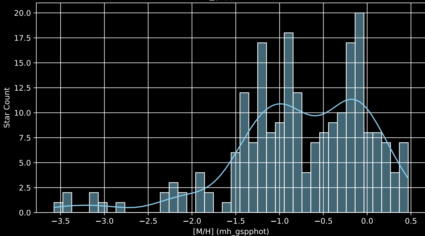
Gaia Cluster: [Berkeley_43 [M/H] (mh_gspphot) (n= 219)
