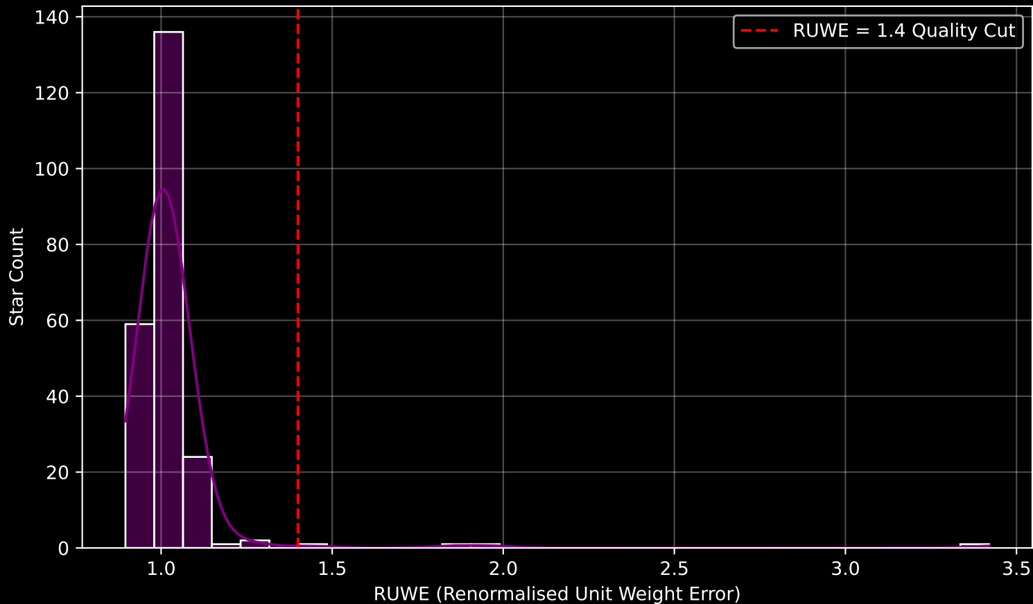
Gaia Cluster: [Berkeley_43] RUWE Distribution (n= 226)
