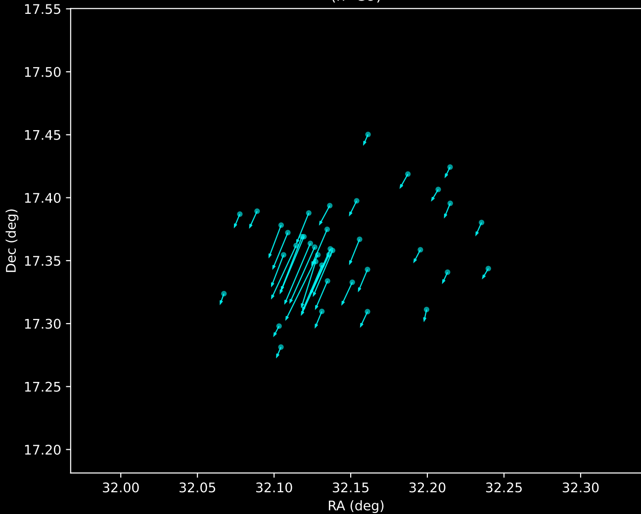
Gaia DR3 Noise Stream Proper Motion Vectors (n=39)
