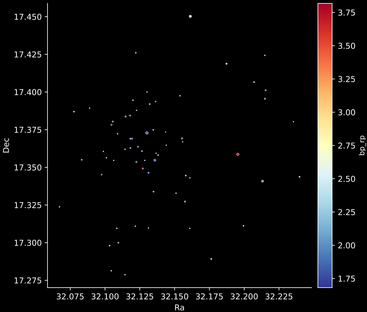
Gaia Cluster: [Berkeley_47] Stars: 64
