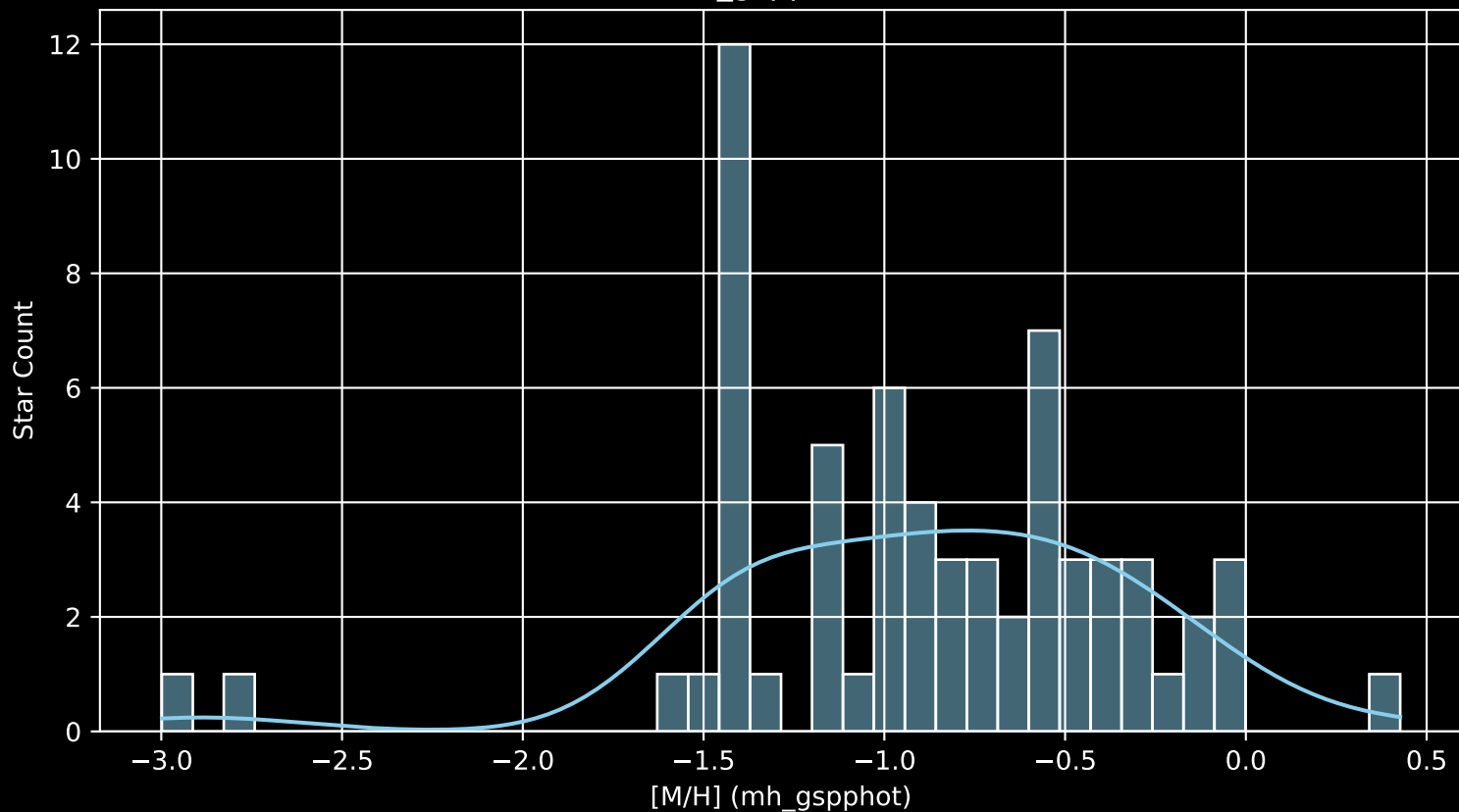
Gaia Cluster: [Berkeley_47 [M/H] (mh_gspphot) (n= 64)
