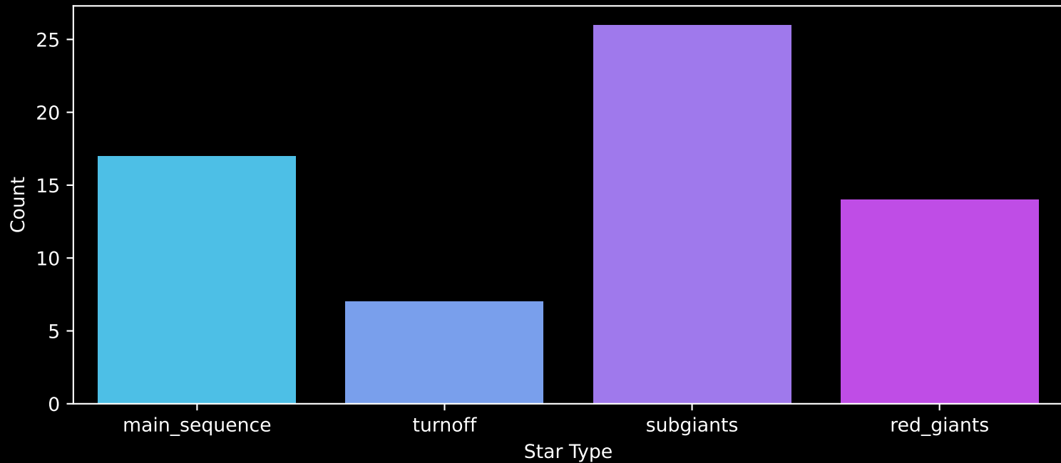
Gaia Cluster: [Berkeley_47] Count plot of Star Type
