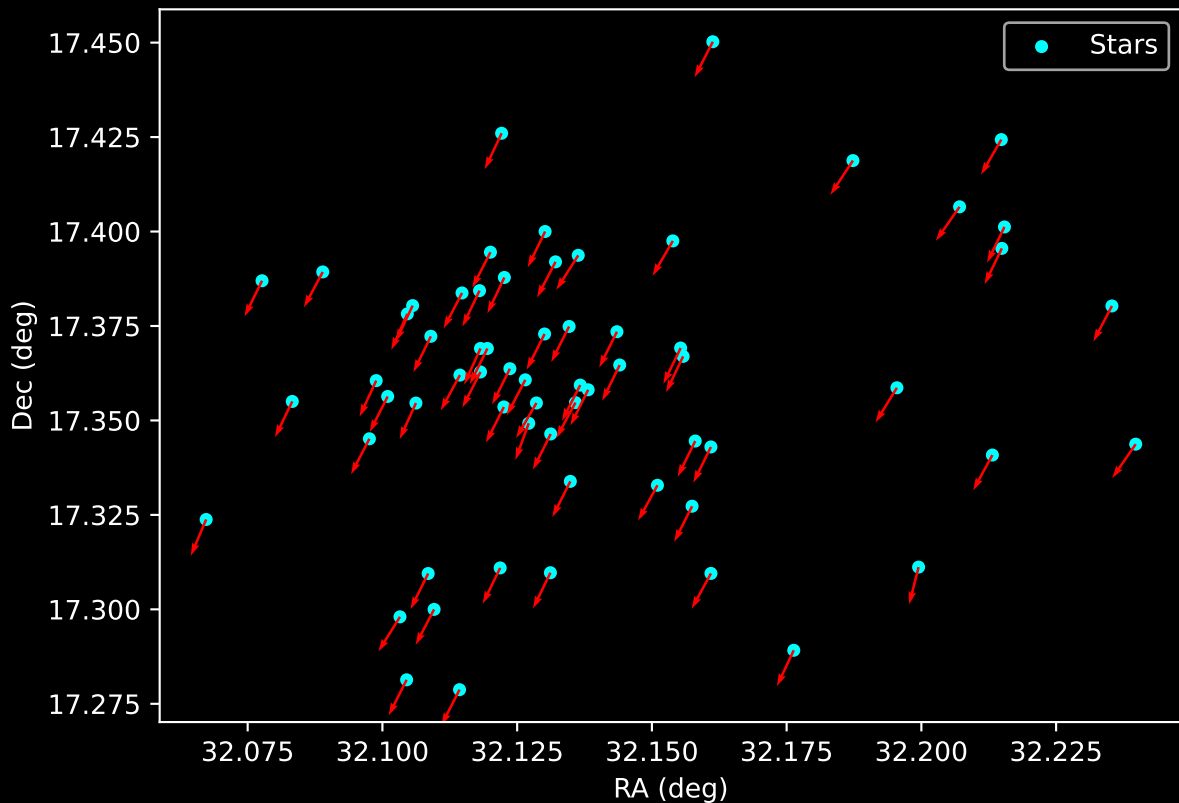
Gaia Cluster: [Berkeley_47] Proper Motion Vectors for Gaia Star Field (n= 64)
