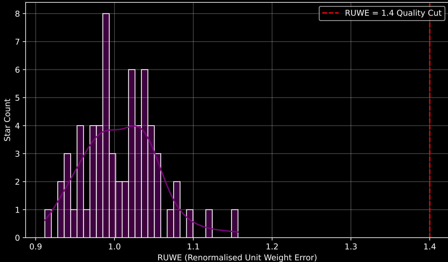
Gaia Cluster: [Berkeley_47] RUWE Distribution (n= 64)
