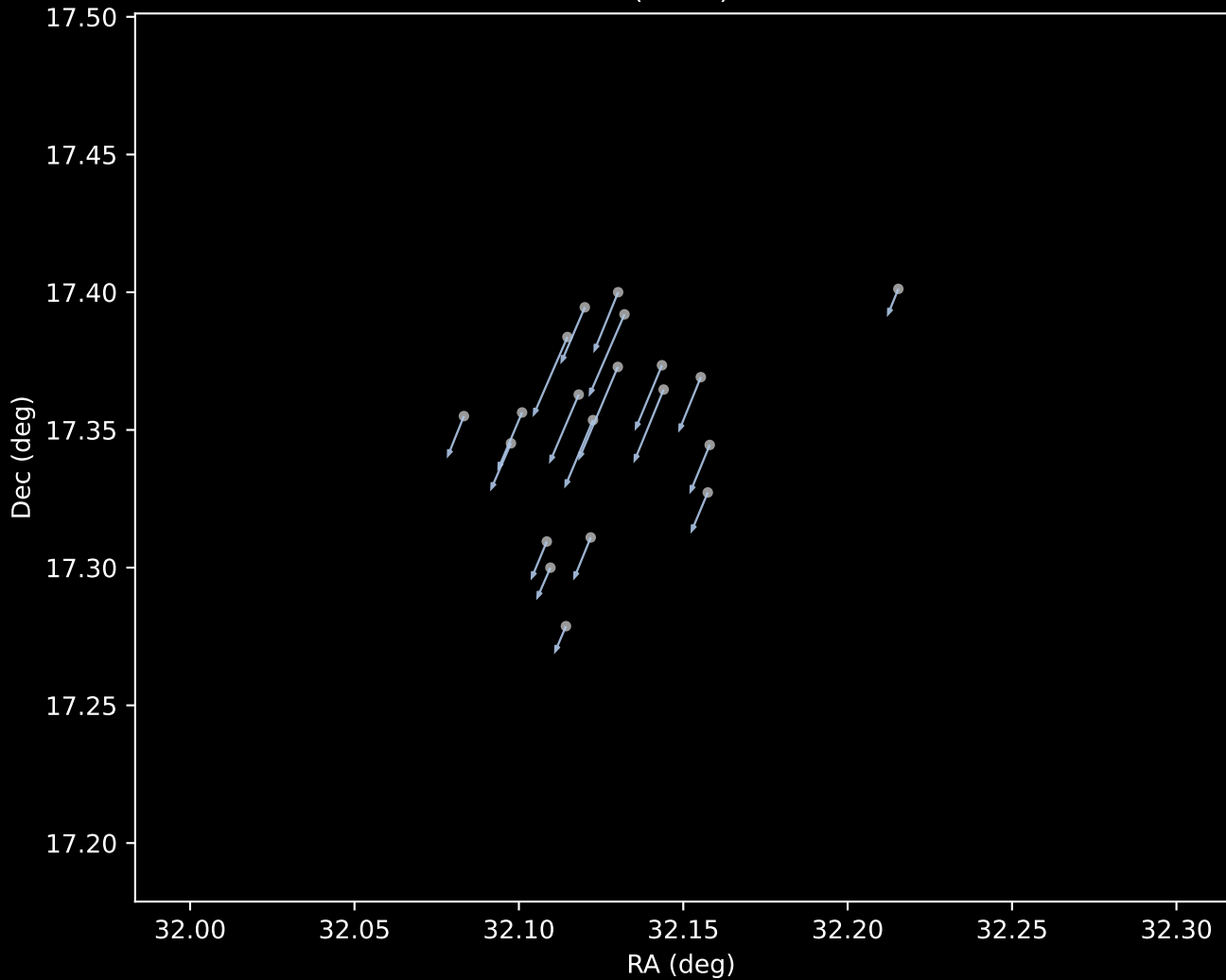
Gaia DR3 Cluster 1 Proper Motion Vectors (n=20)
