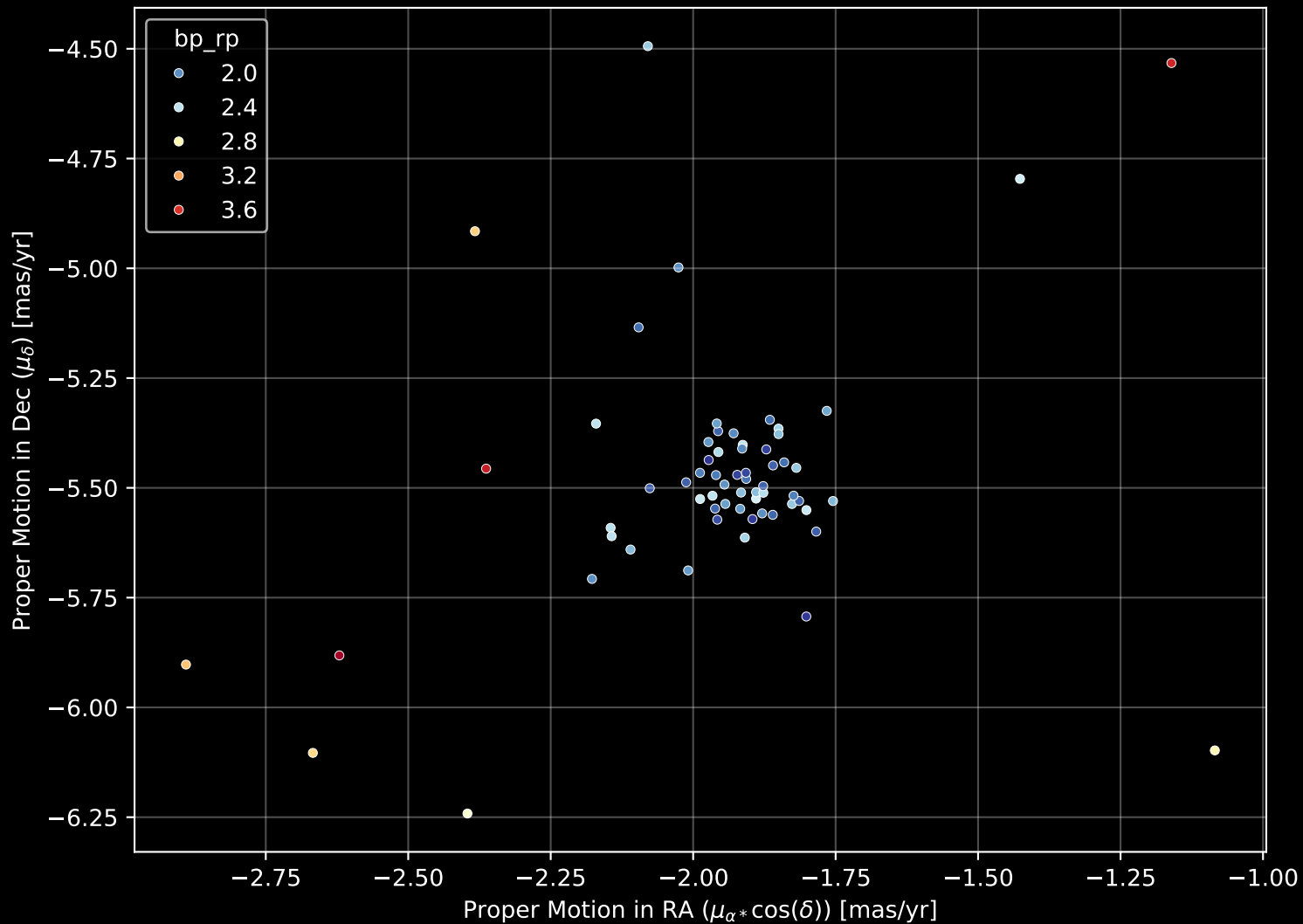
Gaia Cluster: [Berkeley_47] Proper Motion Diagram (n= 64)
