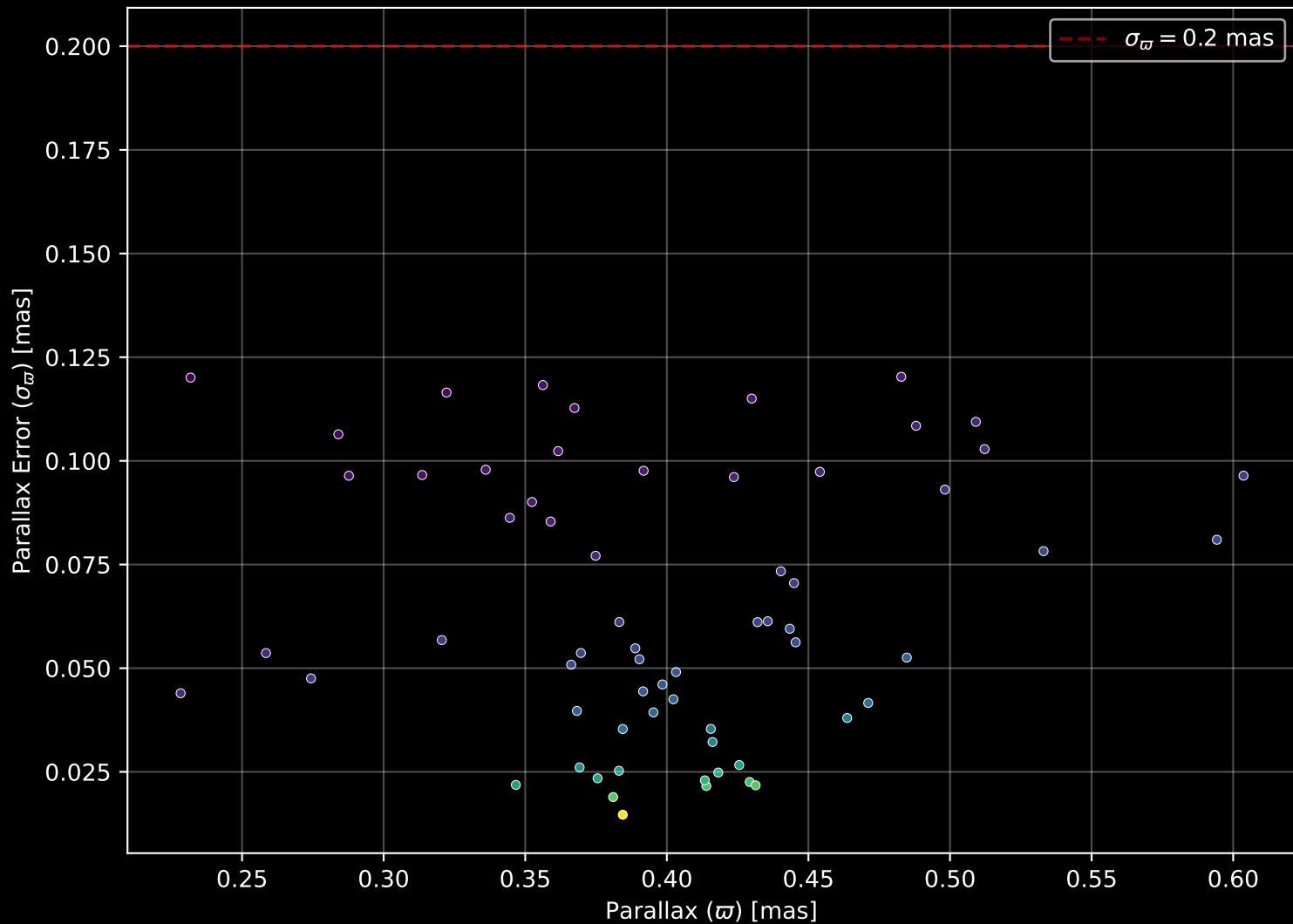
Gaia Cluster: [Berkeley_47] Parallax Quality (n= 64)
