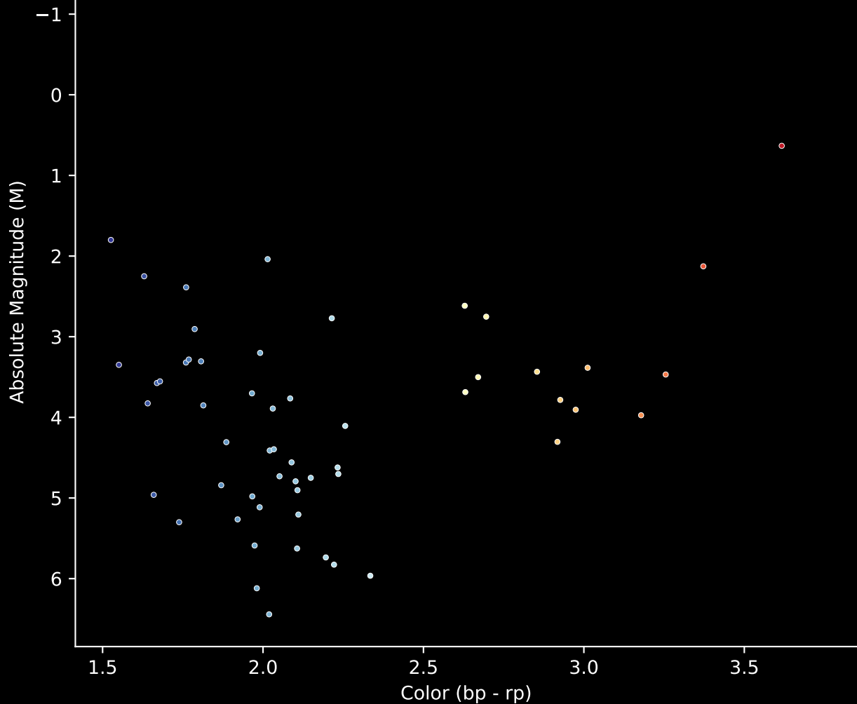
Gaia Cluster: [Berkeley_49] Stars (n= 57) Hertzsprung-Russel Diagram
