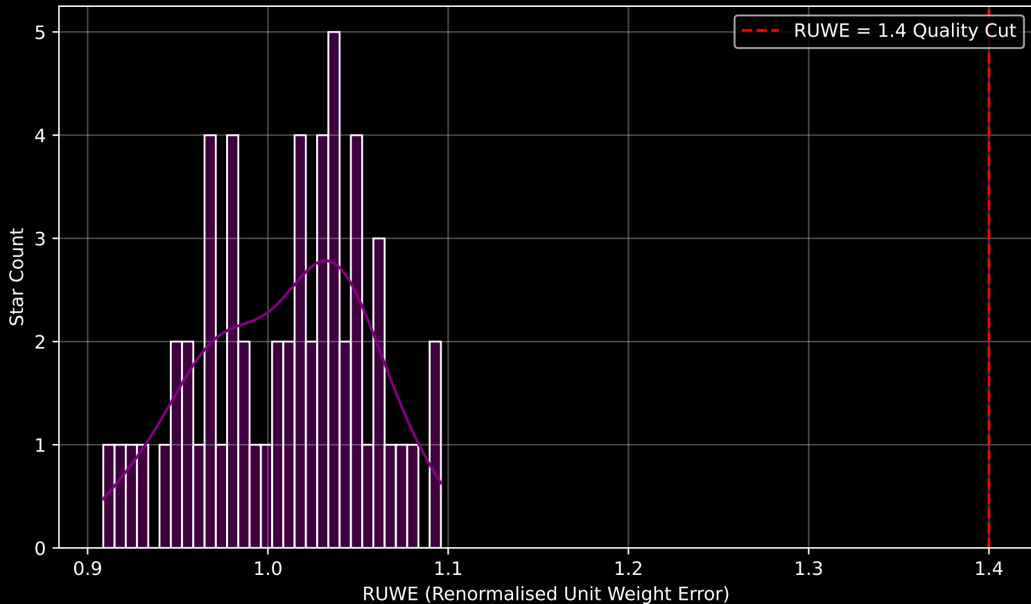
Gaia Cluster: [Berkeley_49] RUWE Distribution (n= 57)
