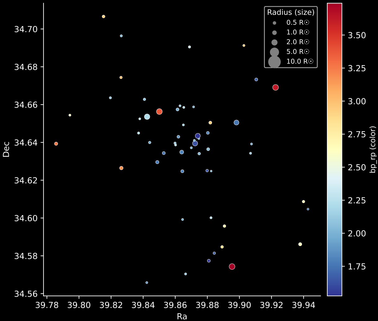
Gaia Cluster: [Berkeley_49] Stars: 57
