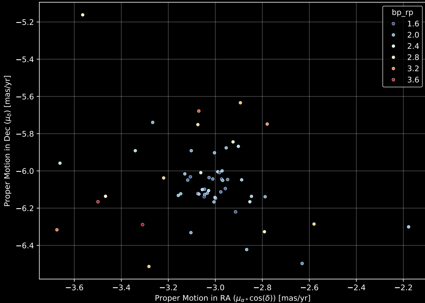
Gaia Cluster: [Berkeley_49] Proper Motion Diagram (n= 57)
