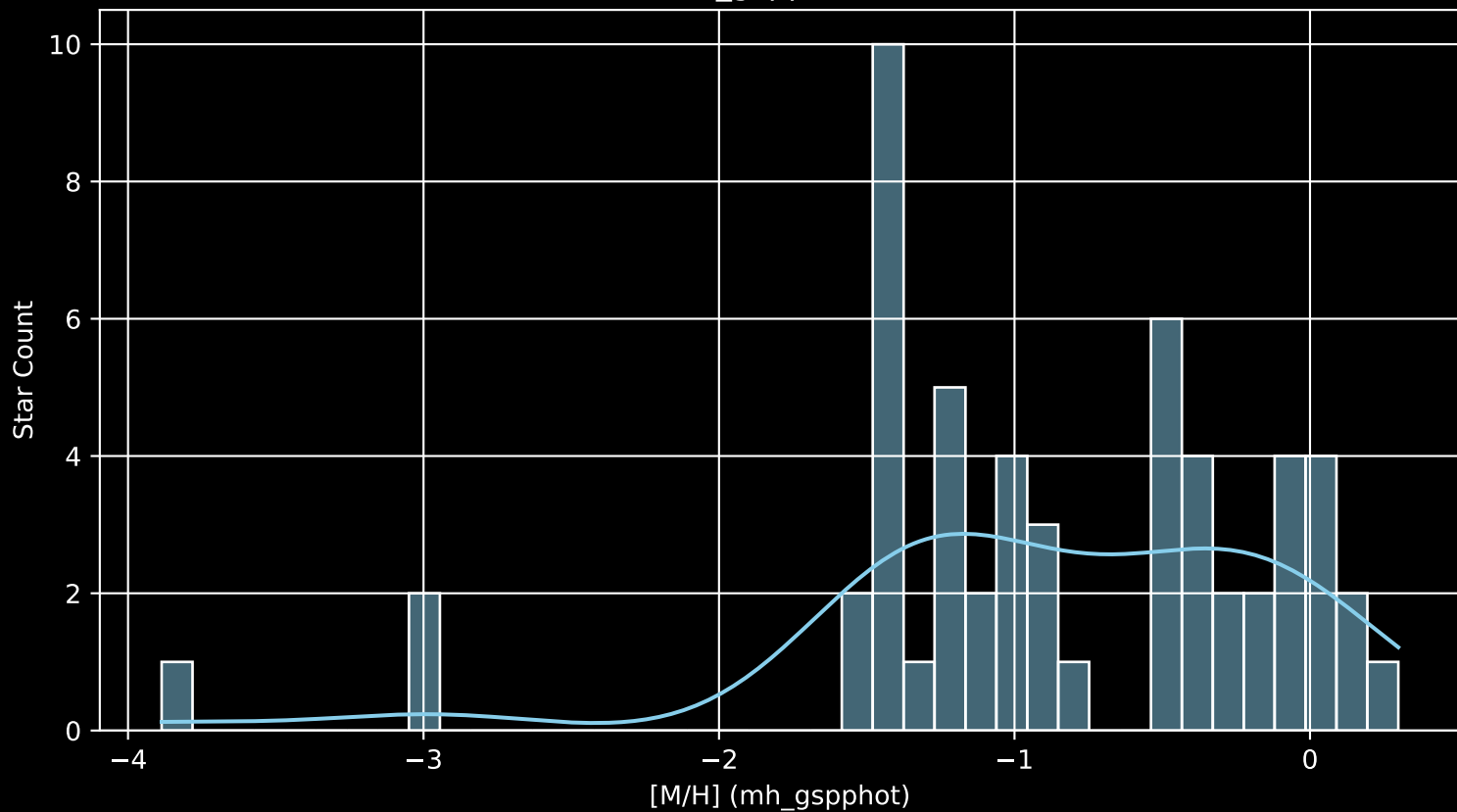
Gaia Cluster: [Berkeley_49 [M/H] (mh_gspphot) (n= 56)
