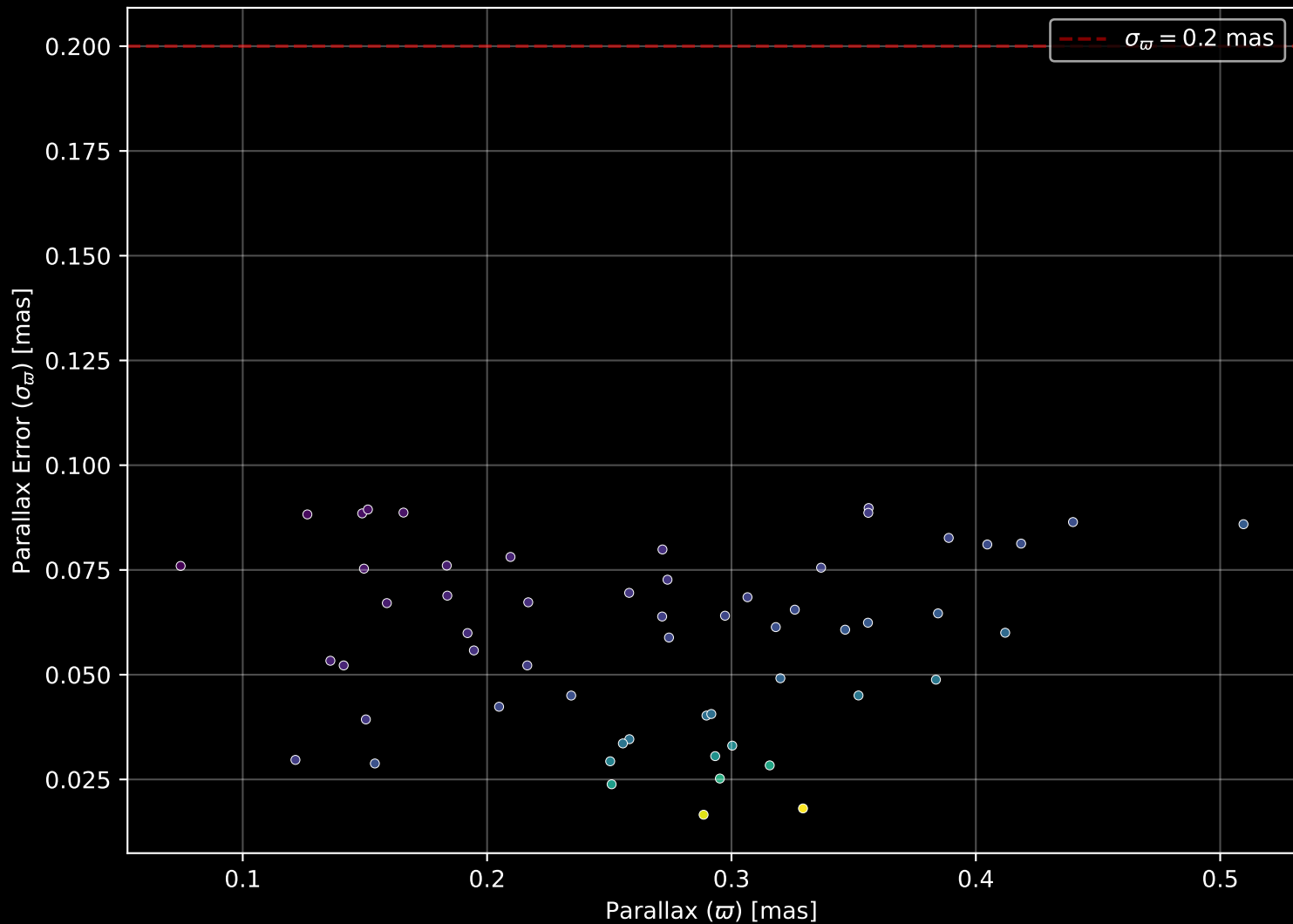
Gaia Cluster: [Berkeley_49] Parallax Quality (n= 57)
