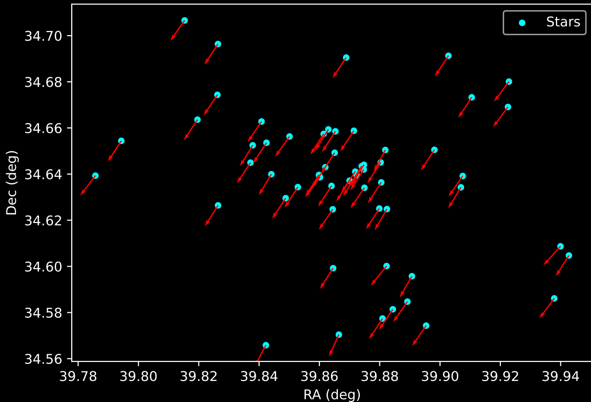
Gaia Cluster: [Berkeley_49] Proper Motion Vectors for Gaia Star Field (n= 57)
