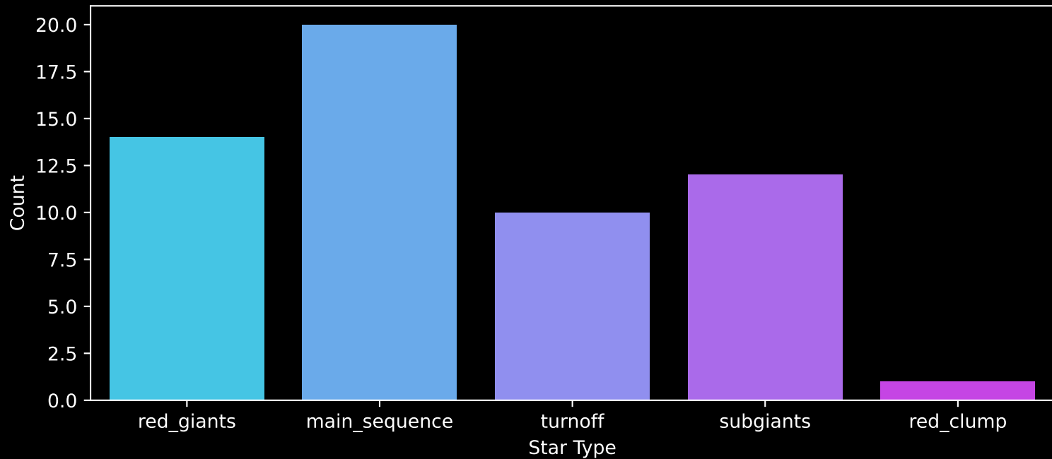
Gaia Cluster: [Berkeley_49] Count plot of Star Type
