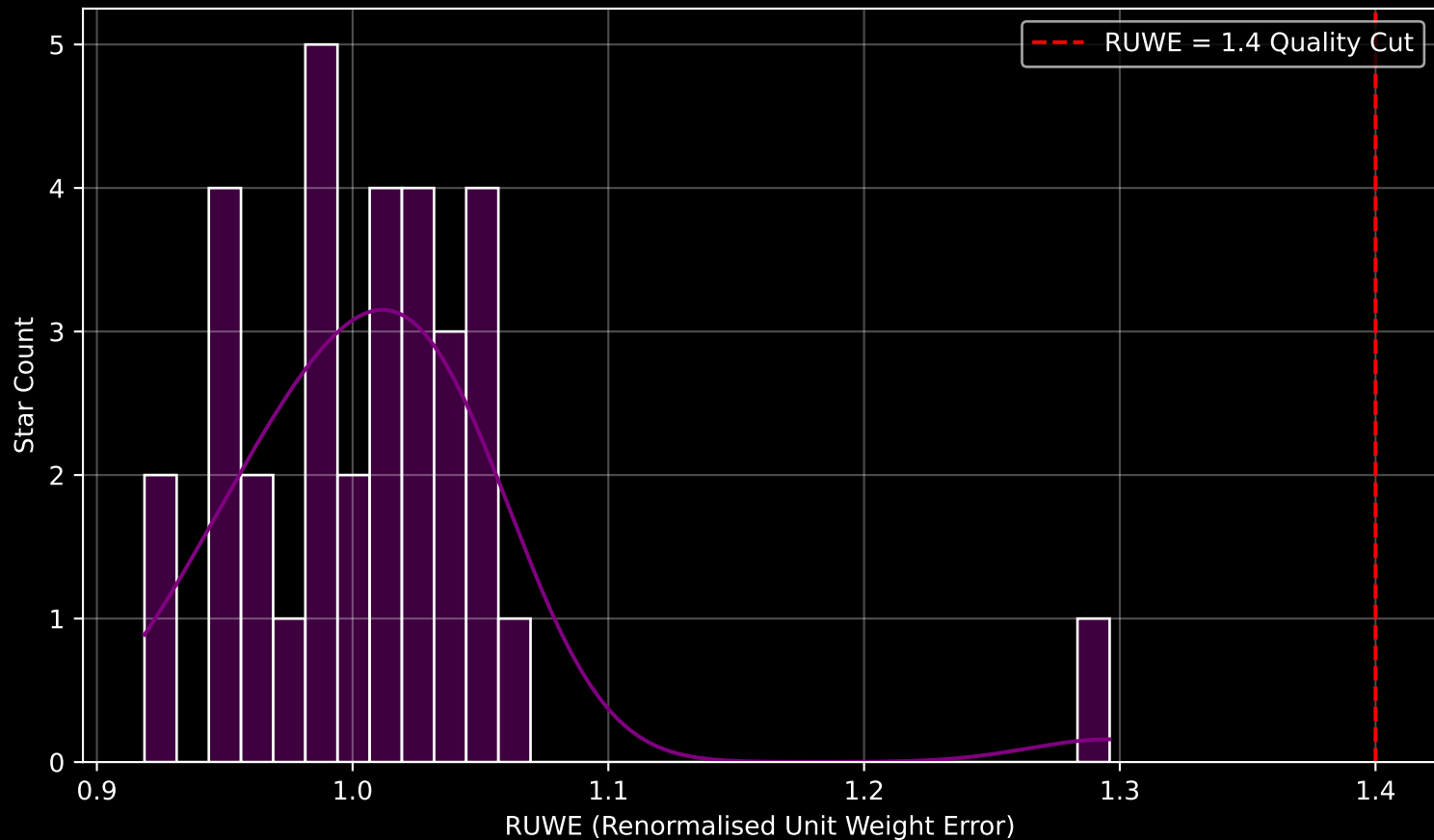
Gaia Cluster: [Berkeley_5] RUWE Distribution (n= 33)
