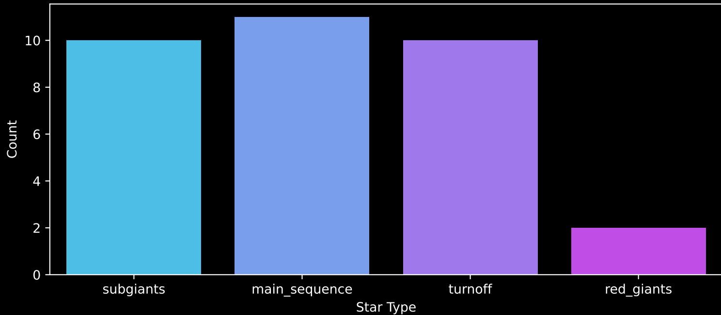
Gaia Cluster: [Berkeley_5] Count plot of Star Type
