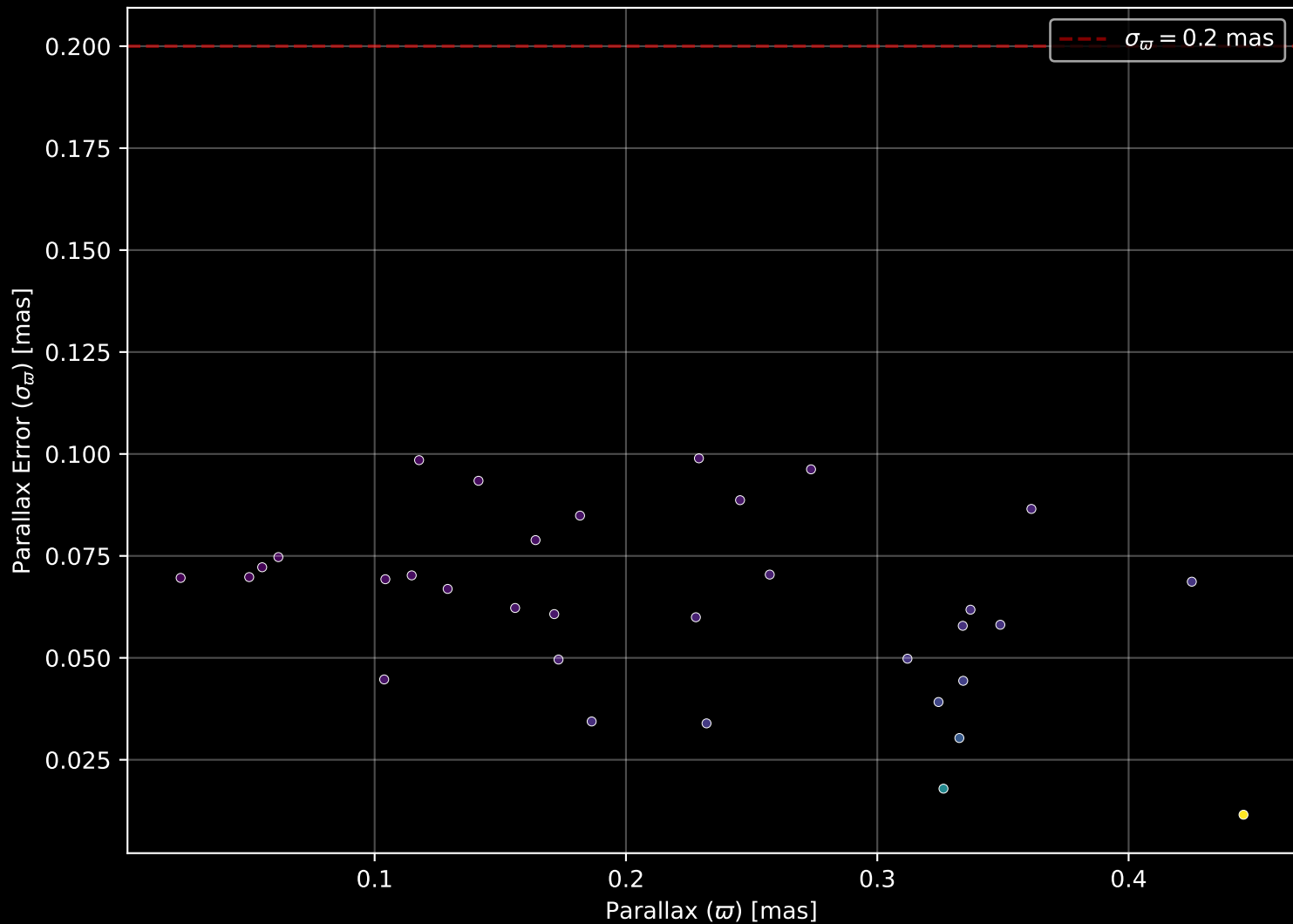
Gaia Cluster: [Berkeley_5] Parallax Quality (n= 33)
