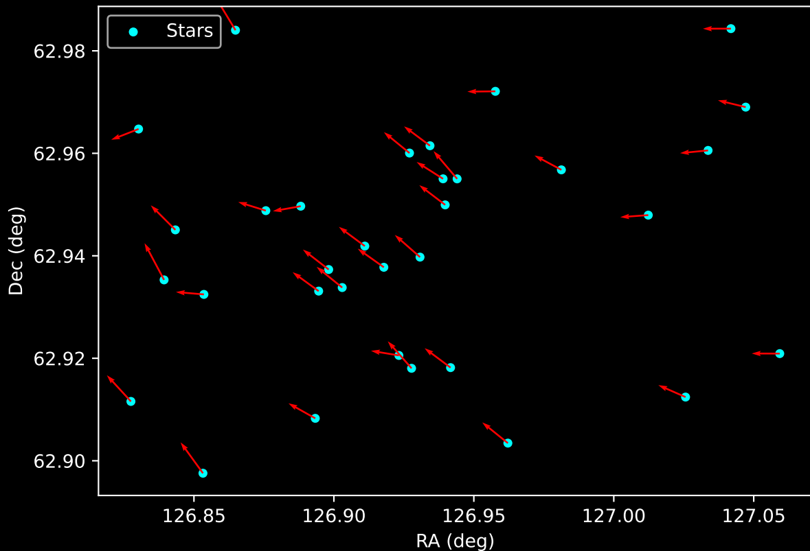
Gaia Cluster: [Berkeley_5] Proper Motion Vectors for Gaia Star Field (n= 33)
