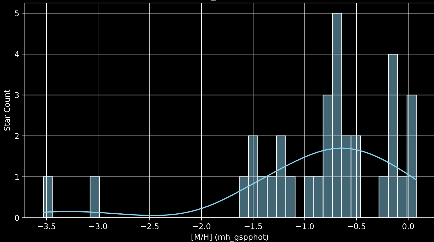
Gaia Cluster: [Berkeley_5 [M/H] (mh_gspphot) (n= 33)
