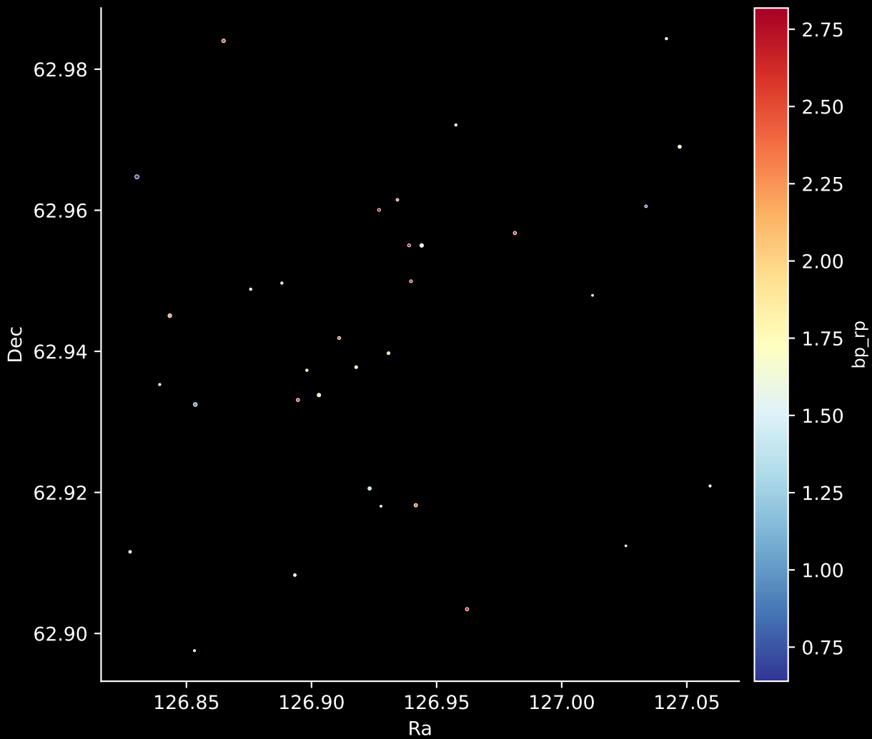
Gaia Cluster: [Berkeley_5] Stars: 33
