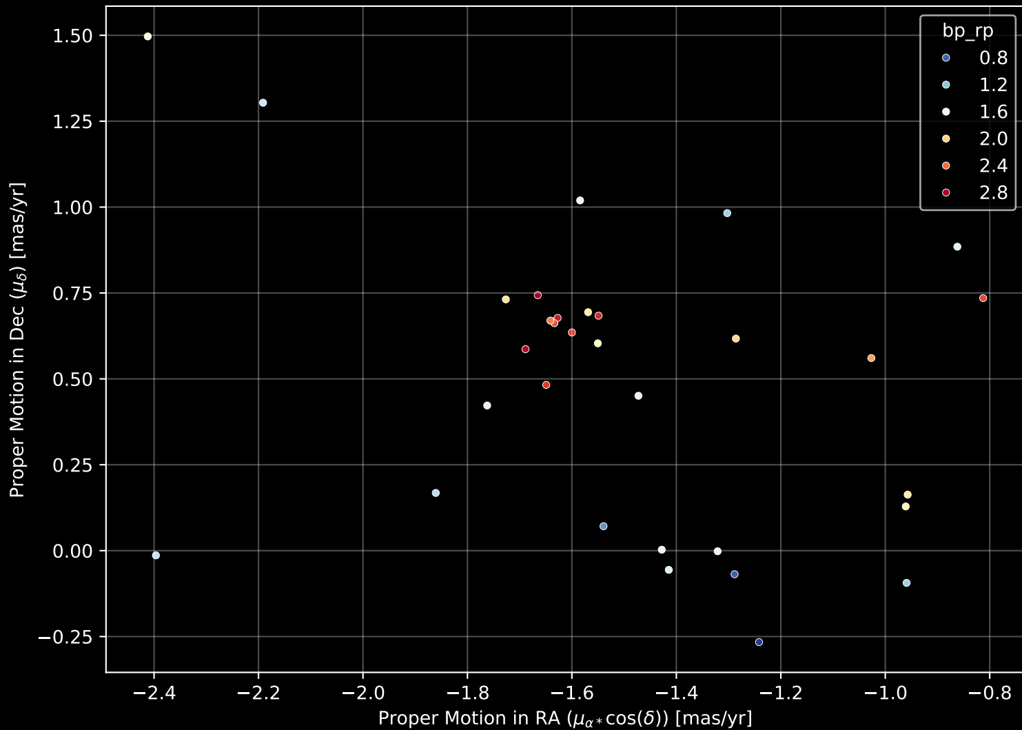
Gaia Cluster: [Berkeley_5] Proper Motion Diagram (n= 33)
