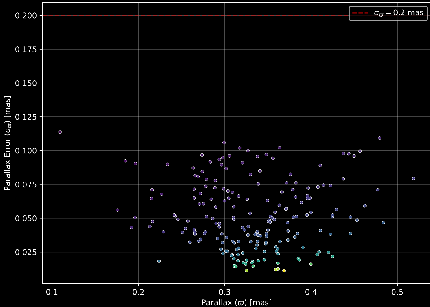
Gaia Cluster: [Berkeley_6] Parallax Quality (n= 198)
