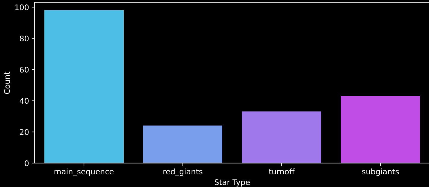
Gaia Cluster: [Berkeley_6] Count plot of Star Type
