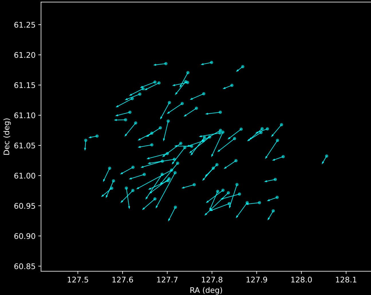
Gaia DR3 Noise Stream Proper Motion Vectors (n=77)
