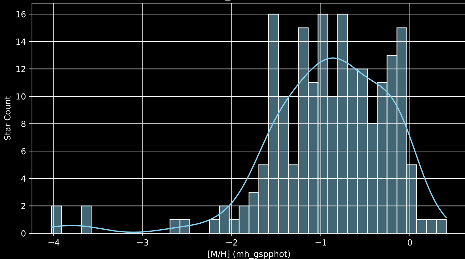
Gaia Cluster: [Berkeley_6 [M/H] (mh_gspphot) (n= 198)
