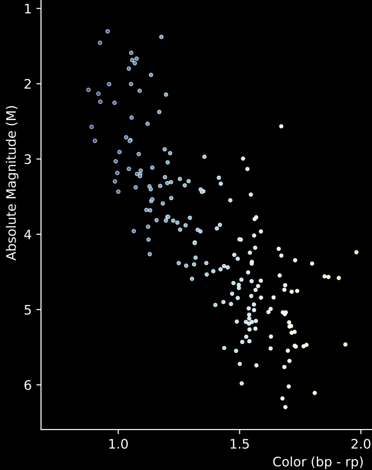
Gaia Cluster: [Berkeley_6] Stars (n= 198) Hertzsprung-Russel Diagram
