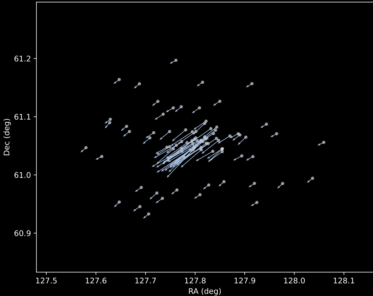
Gaia DR3 Cluster 1 Proper Motion Vectors (n=87)
