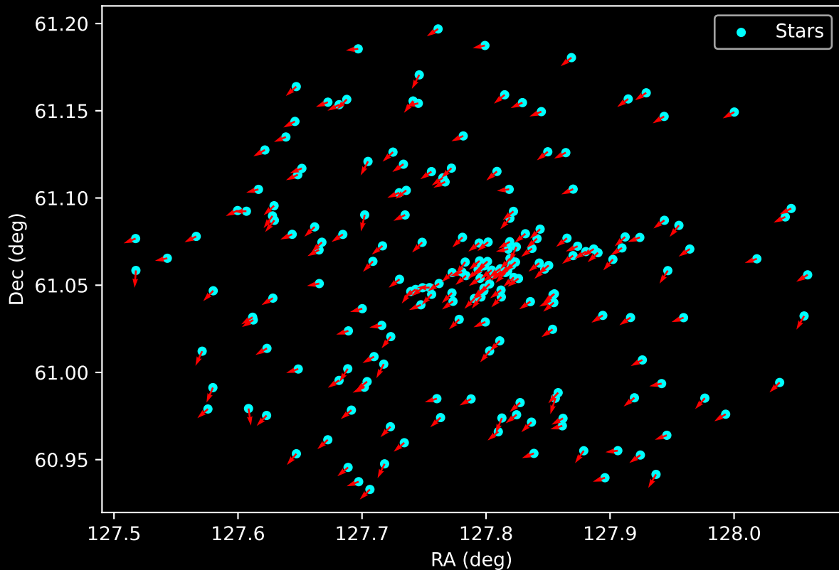
Gaia Cluster: [Berkeley_6] Proper Motion Vectors for Gaia Star Field (n= 198)
