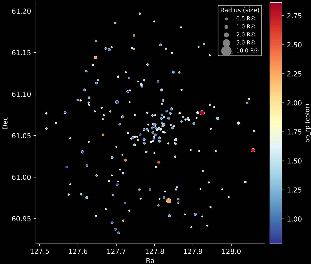
Gaia Cluster: [Berkeley_6] Stars: 198
