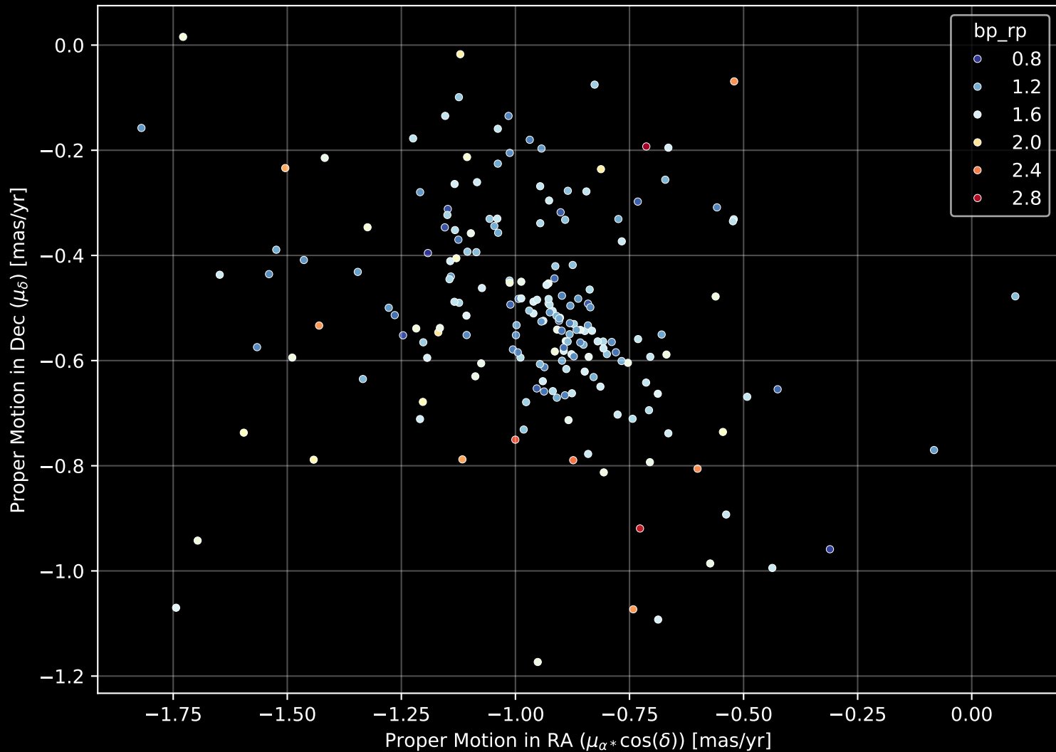
Gaia Cluster: [Berkeley_6] Proper Motion Diagram (n= 198)
