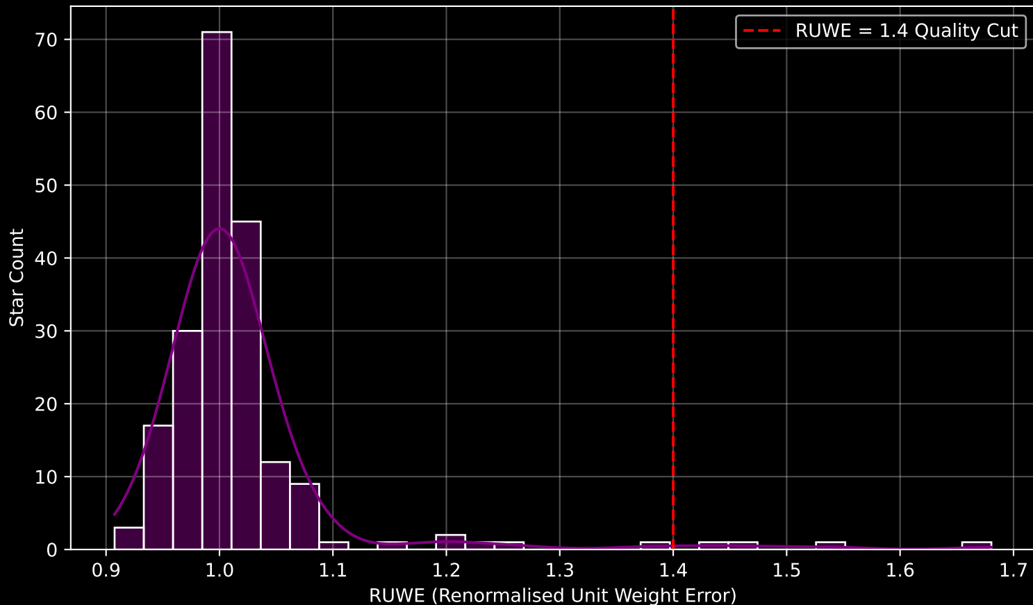
Gaia Cluster: [Berkeley_6] RUWE Distribution (n= 198)
