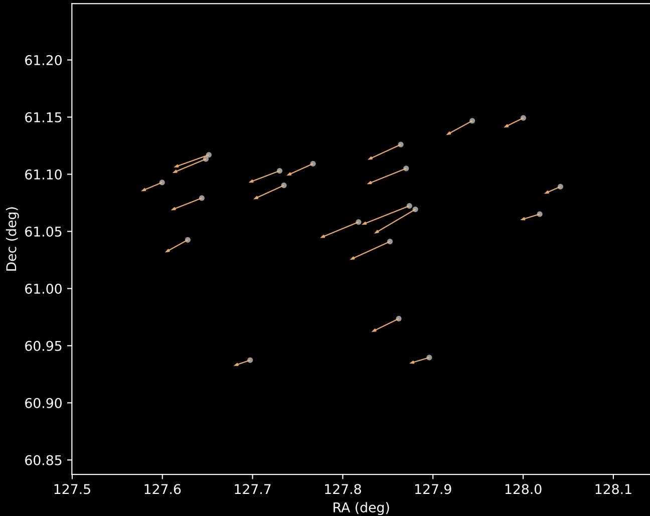
Gaia DR3 Cluster 3 Proper Motion Vectors (n=21)
