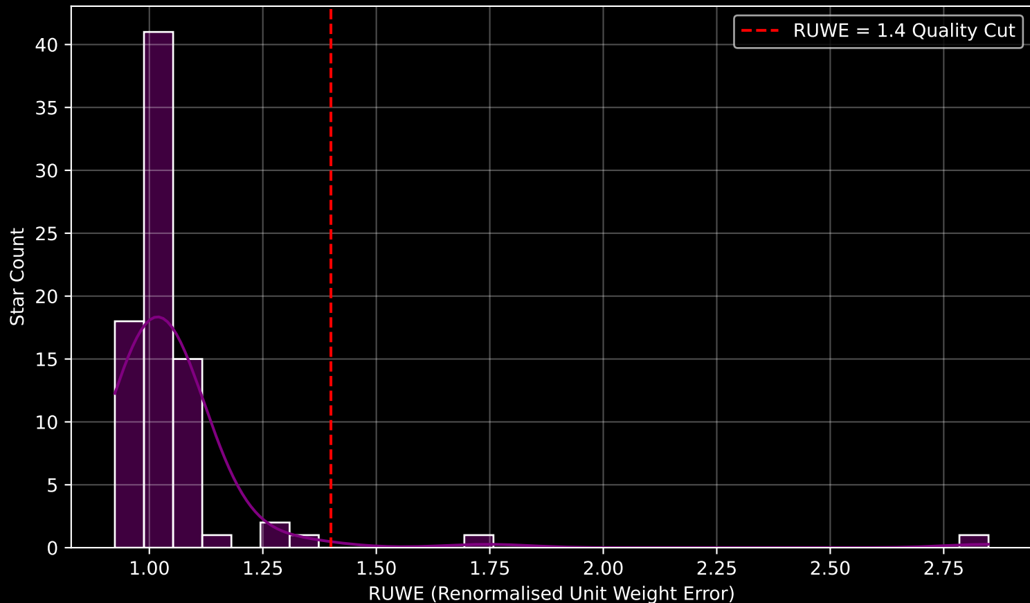
Gaia Cluster: [Berkeley_60] RUWE Distribution (n= 80)
