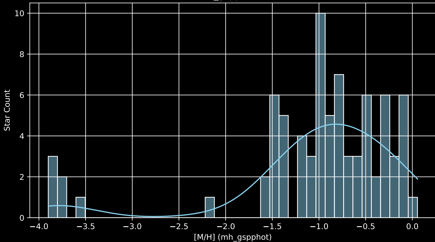
Gaia Cluster: [Berkeley_60 [M/H] (mh_gspphot) (n= 79)
