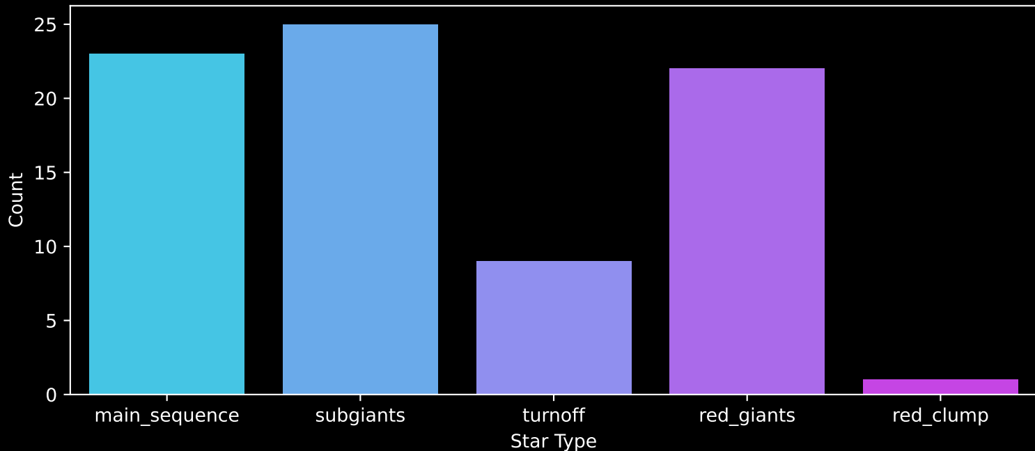
Gaia Cluster: [Berkeley_60] Count plot of Star Type
