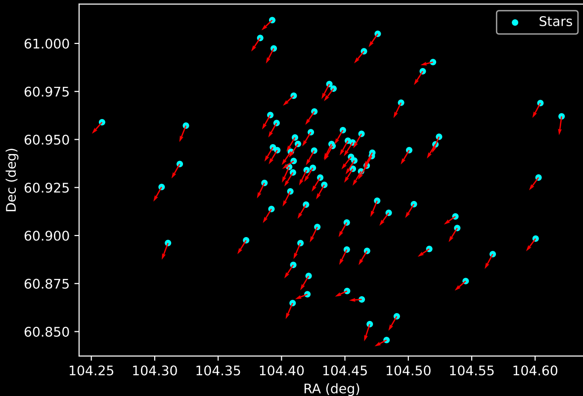
Gaia Cluster: [Berkeley_60] Proper Motion Vectors for Gaia Star Field (n= 80)
