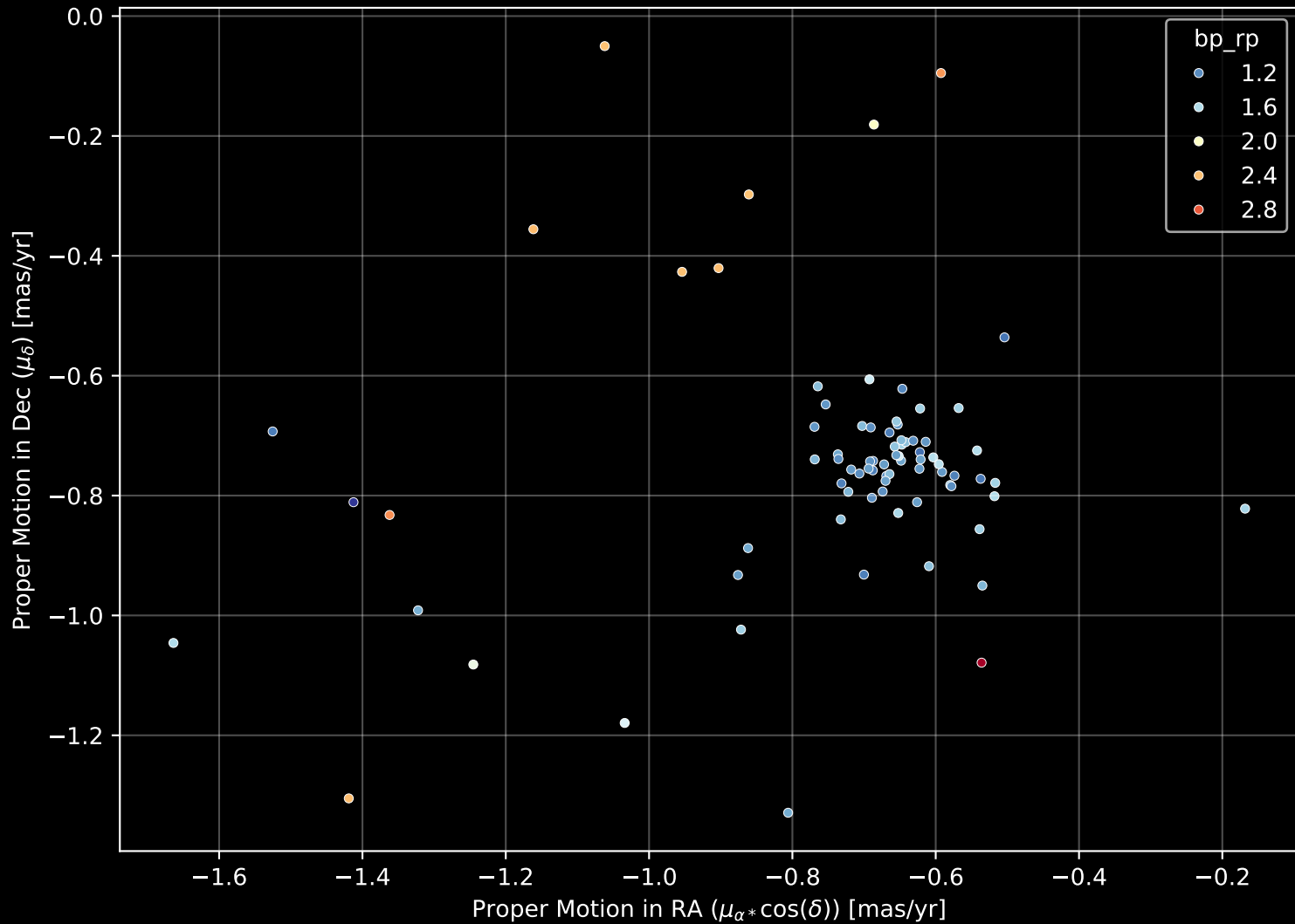
Gaia Cluster: [Berkeley_60] Proper Motion Diagram (n= 80)
