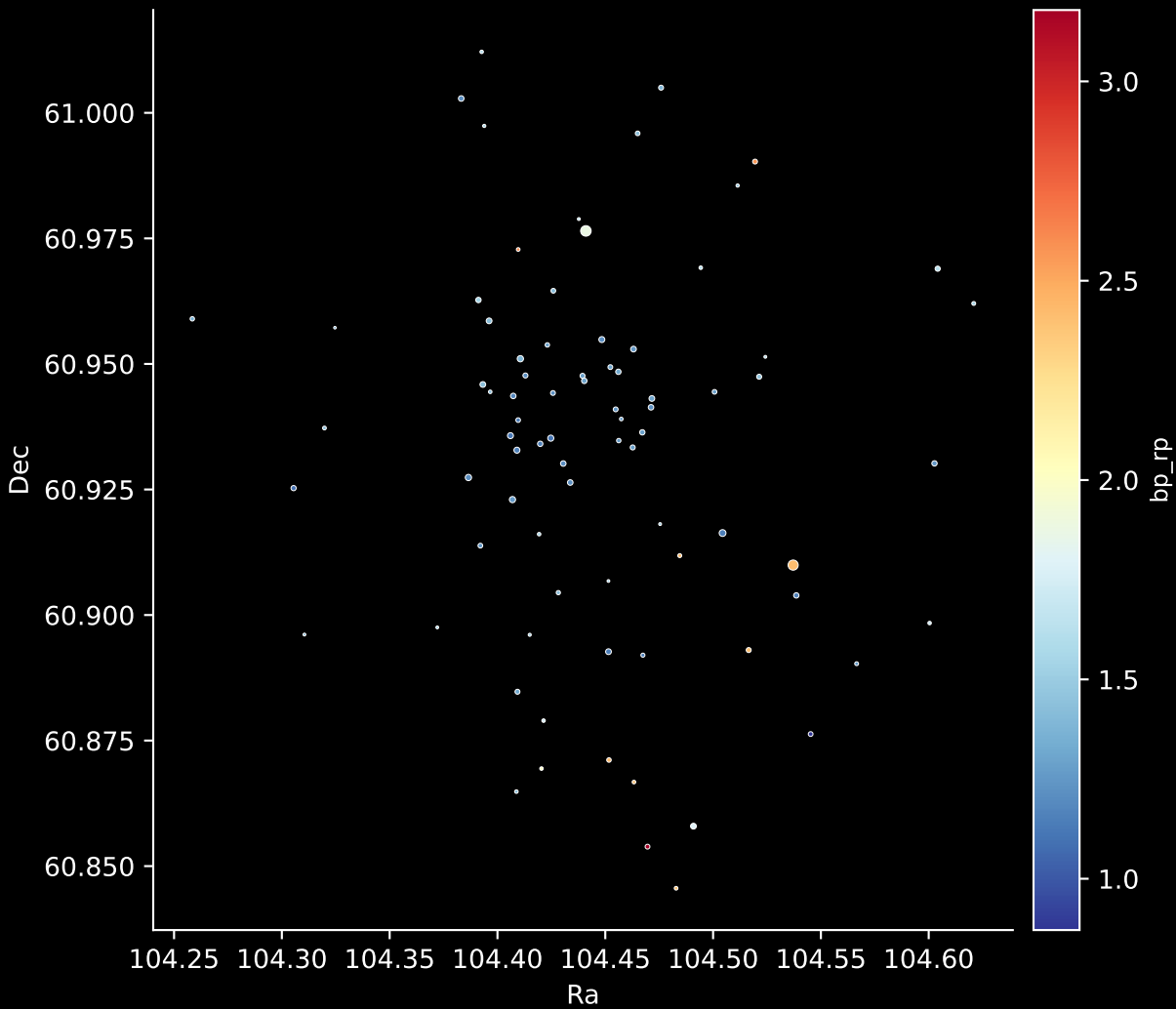
Gaia Cluster: [Berkeley_60] Stars: 80
