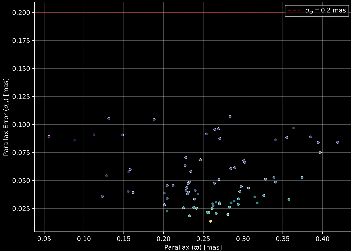
Gaia Cluster: [Berkeley_60] Parallax Quality (n= 80)
