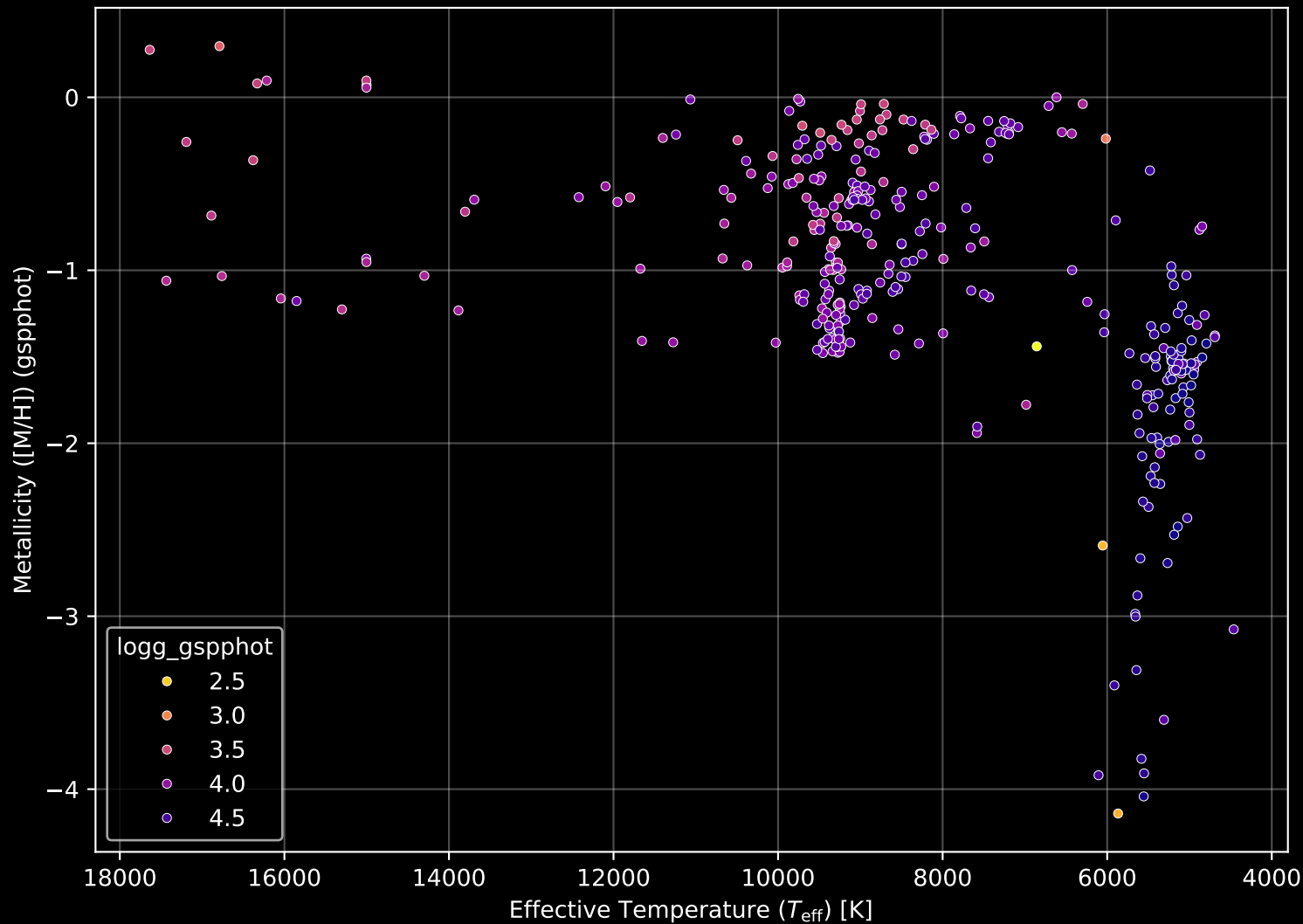
Gaia Cluster: [Berkeley_62] Stellar Population Parameters (n= 357)
