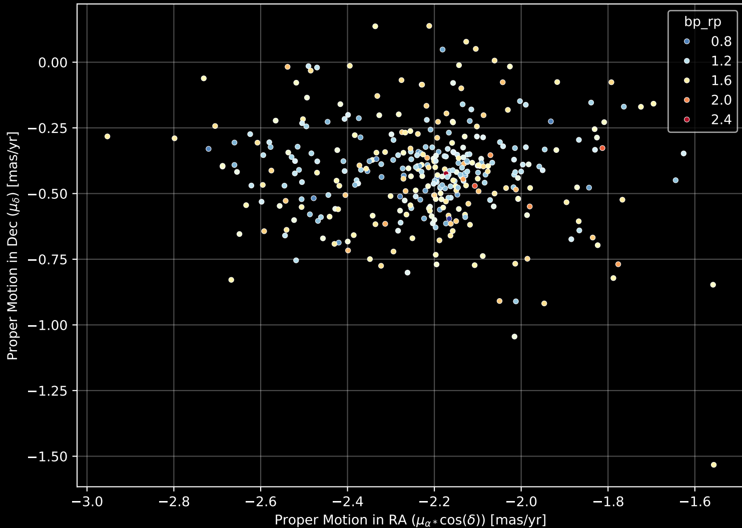
Gaia Cluster: [Berkeley_62] Proper Motion Diagram (n= 357)
