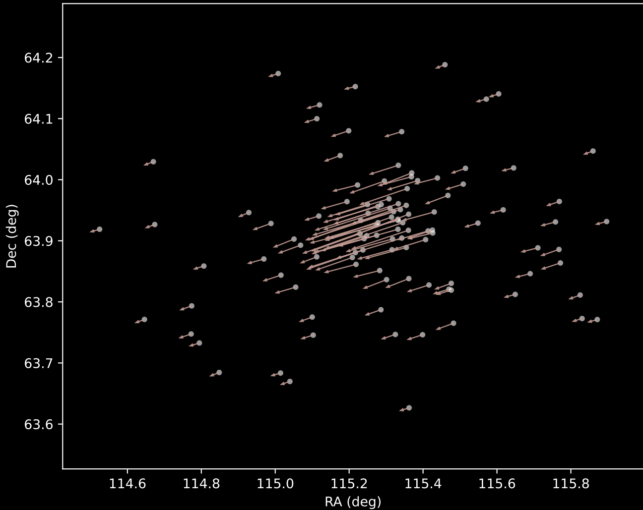
Gaia DR3 Cluster 11 Proper Motion Vectors (n=108)
