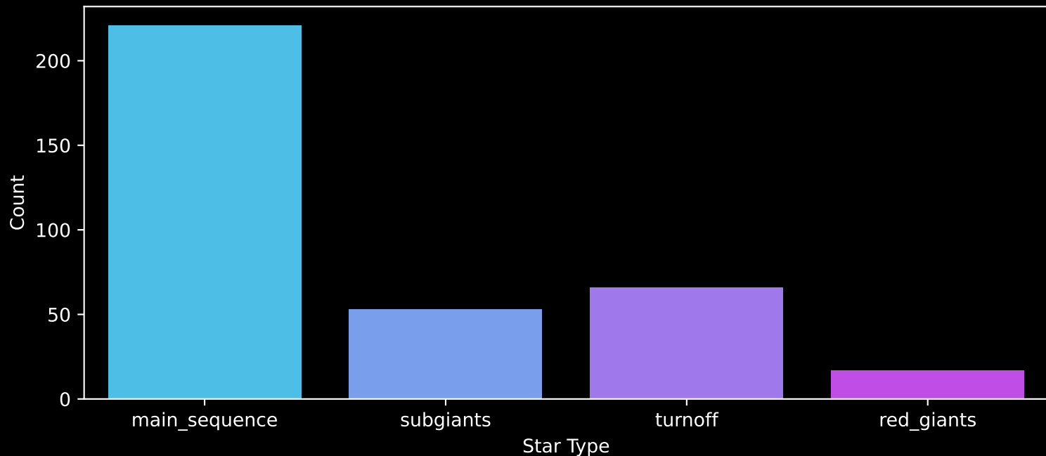
Gaia Cluster: [Berkeley_62] Count plot of Star Type
