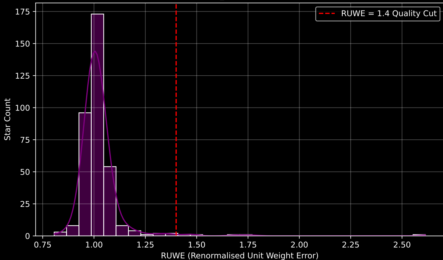
Gaia Cluster: [Berkeley_62] RUWE Distribution (n= 356)
