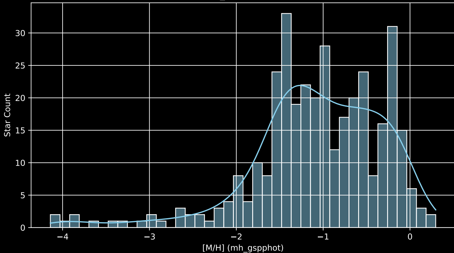
Gaia Cluster: [Berkeley_62 [M/H] (mh_gspphot) (n= 357)
