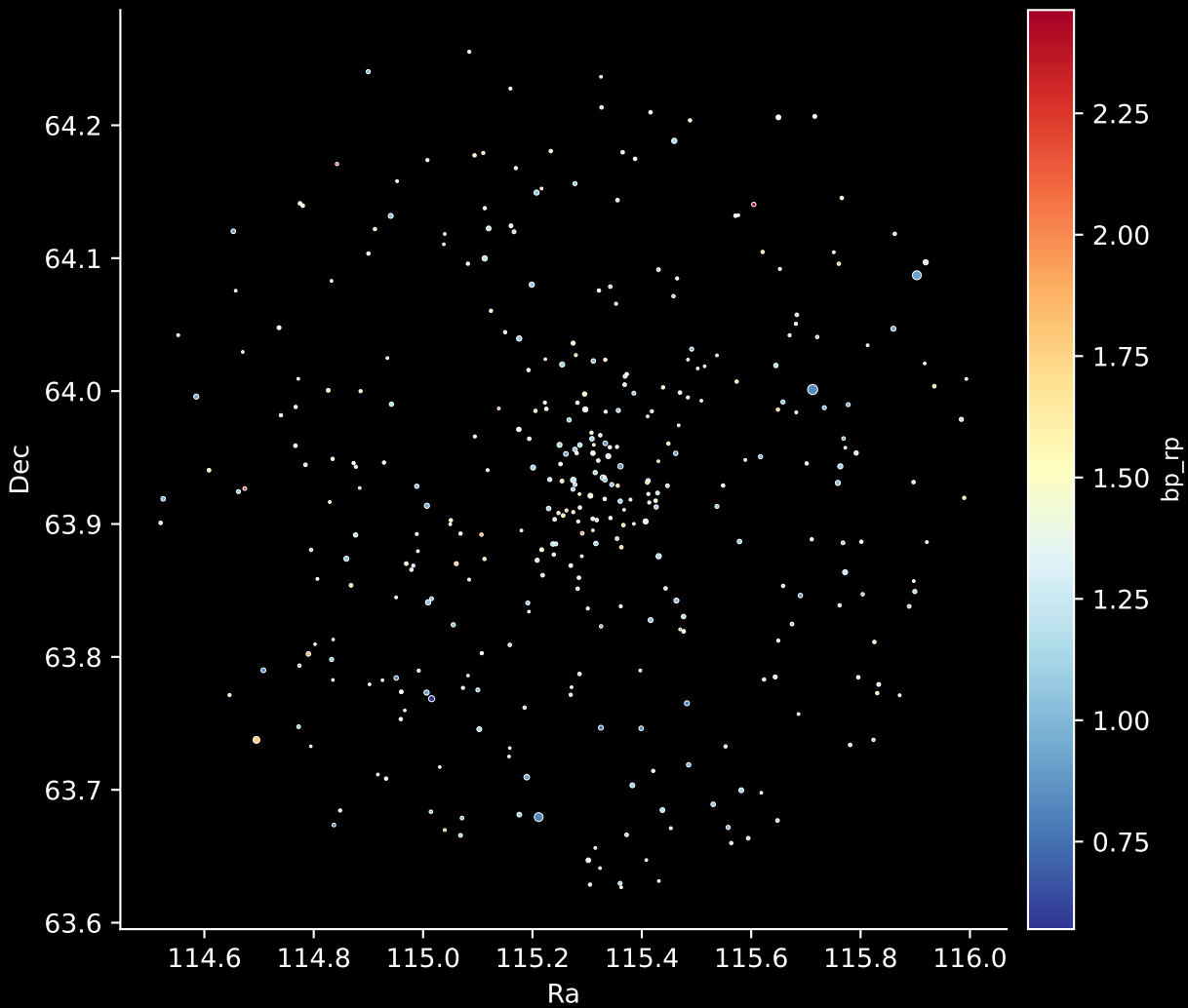
Gaia Cluster: [Berkeley_62] Stars: 357
