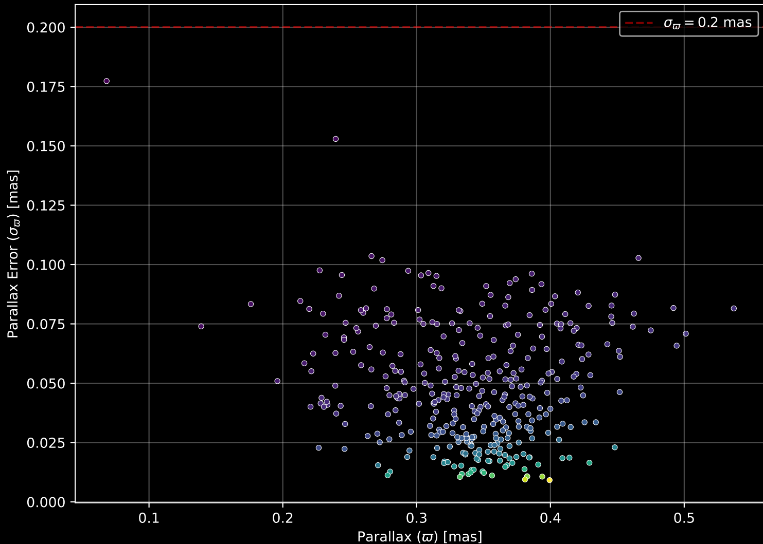
Gaia Cluster: [Berkeley_62] Parallax Quality (n= 357)
