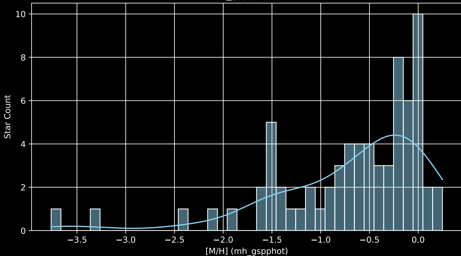
Gaia Cluster: [Berkeley_66 [M/H] (mh_gspphot) (n= 70)
