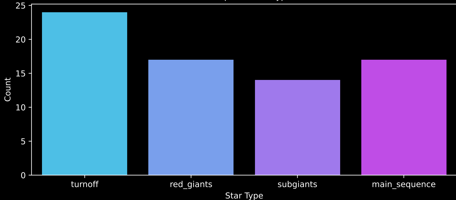
Gaia Cluster: [Berkeley_66] Count plot of Star Type
