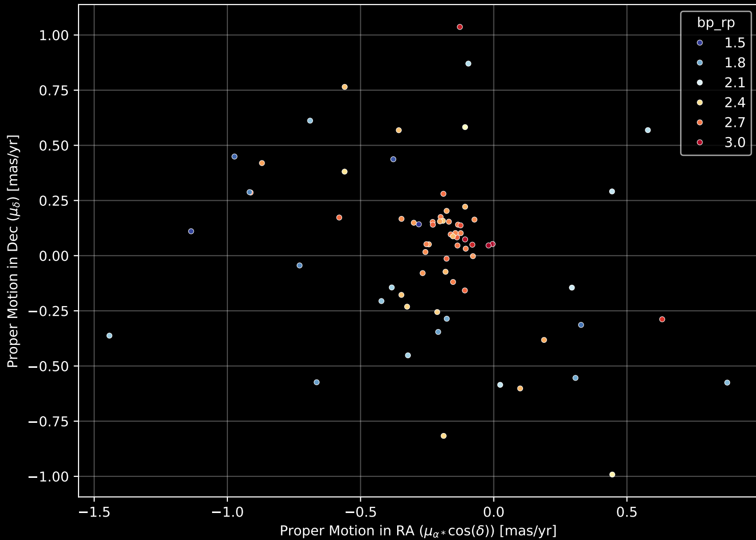
Gaia Cluster: [Berkeley_66] Proper Motion Diagram (n= 72)
