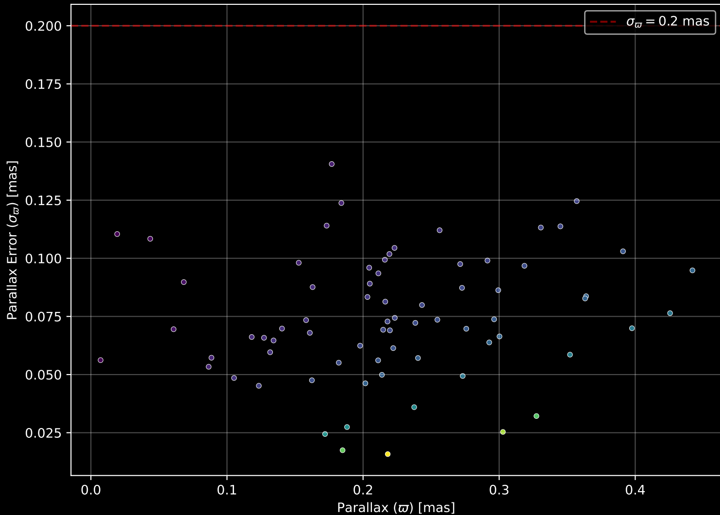
Gaia Cluster: [Berkeley_66] Parallax Quality (n= 72)
