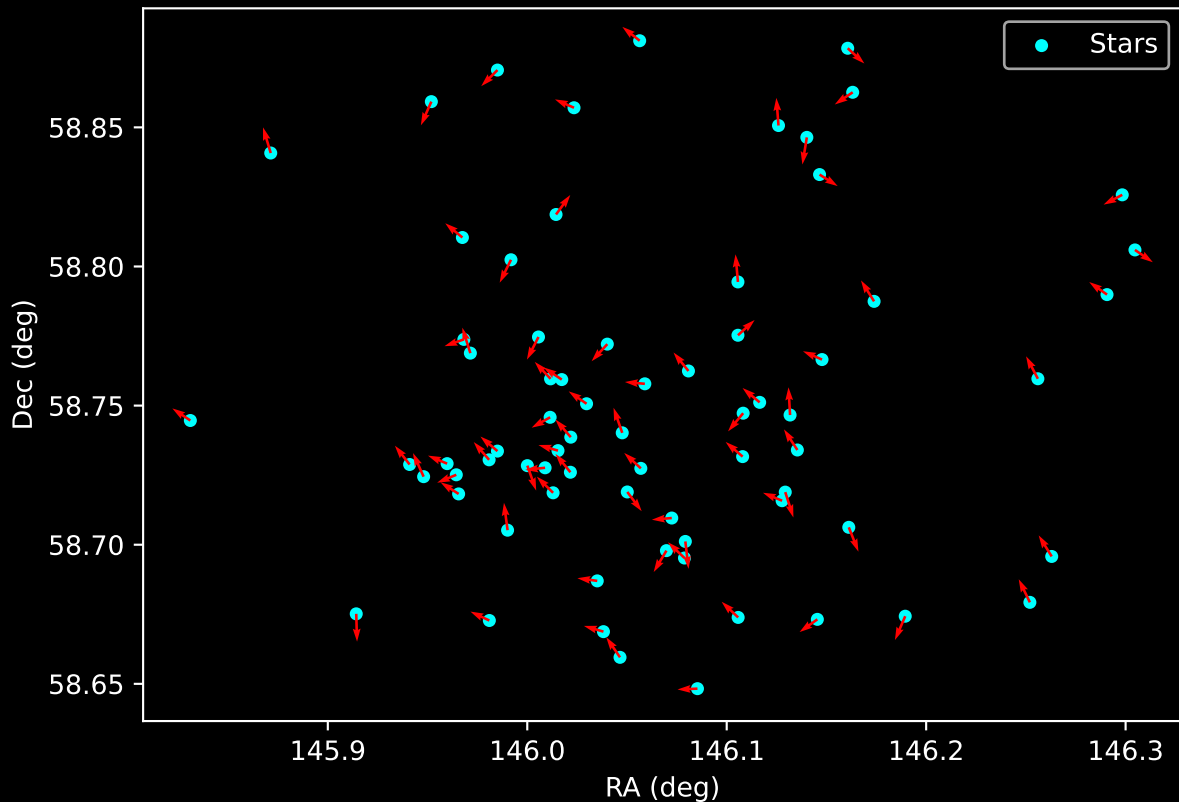
Gaia Cluster: [Berkeley_66] Proper Motion Vectors for Gaia Star Field (n= 72)
