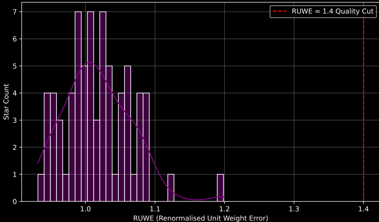
Gaia Cluster: [Berkeley_66] RUWE Distribution (n= 72)
