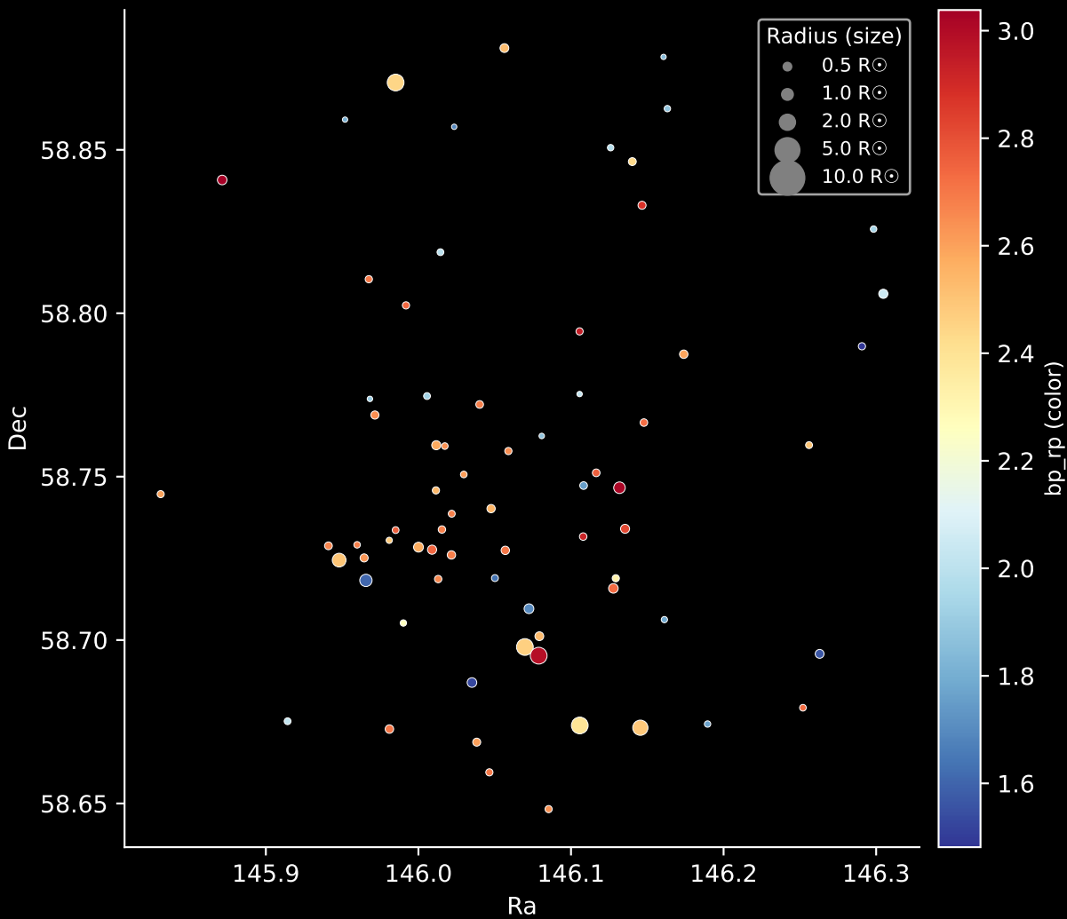
Gaia Cluster: [Berkeley_66] Stars: 72
