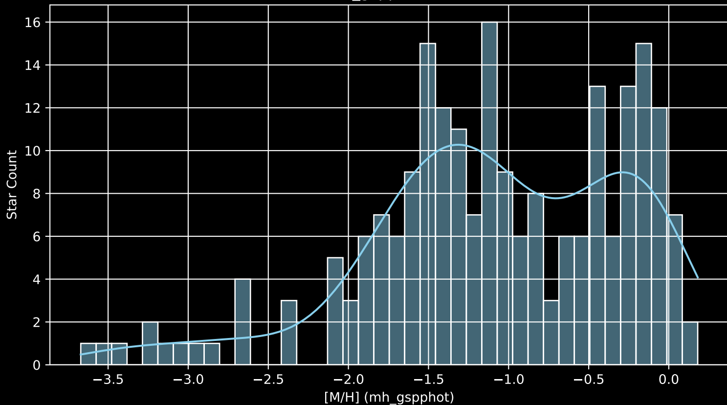
Gaia Cluster: [Berkeley_67 [M/H] (mh_gspphot) (n= 219)
