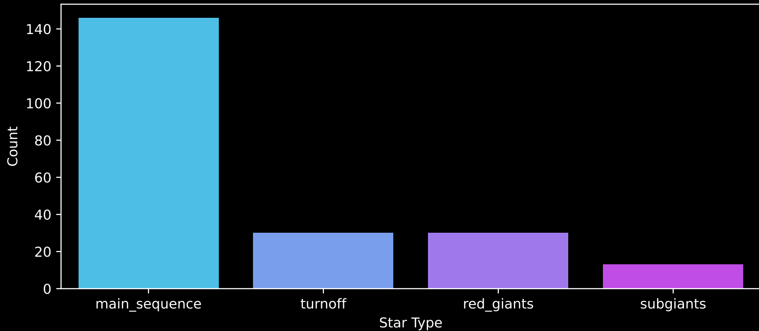
Gaia Cluster: [Berkeley_67] Count plot of Star Type
