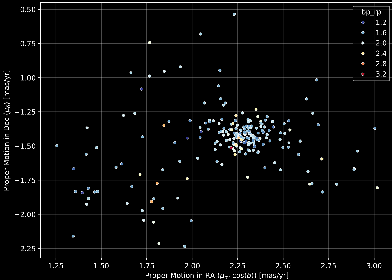
Gaia Cluster: [Berkeley_67] Proper Motion Diagram (n= 219)
