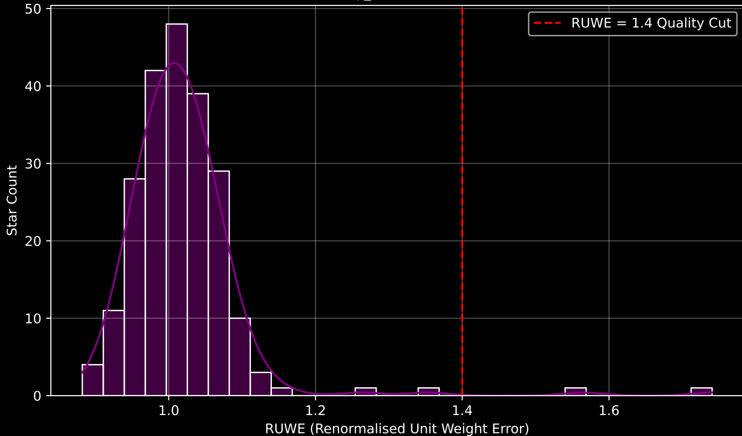
Gaia Cluster: [Berkeley_67] RUWE Distribution (n= 219)
