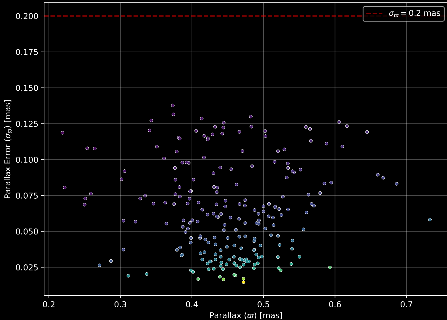
Gaia Cluster: [Berkeley_67] Parallax Quality (n= 219)
