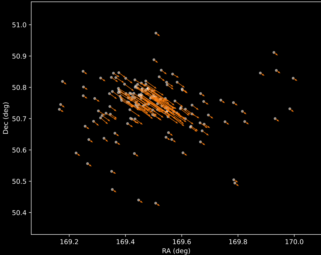
Gaia DR3 Cluster 2 Proper Motion Vectors (n=155)
