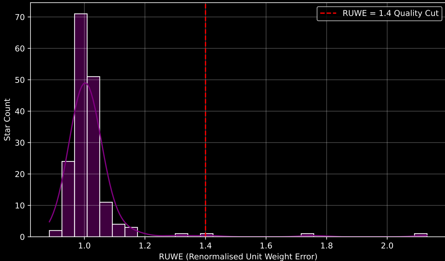
Gaia Cluster: [Berkeley_7] RUWE Distribution (n= 170)
