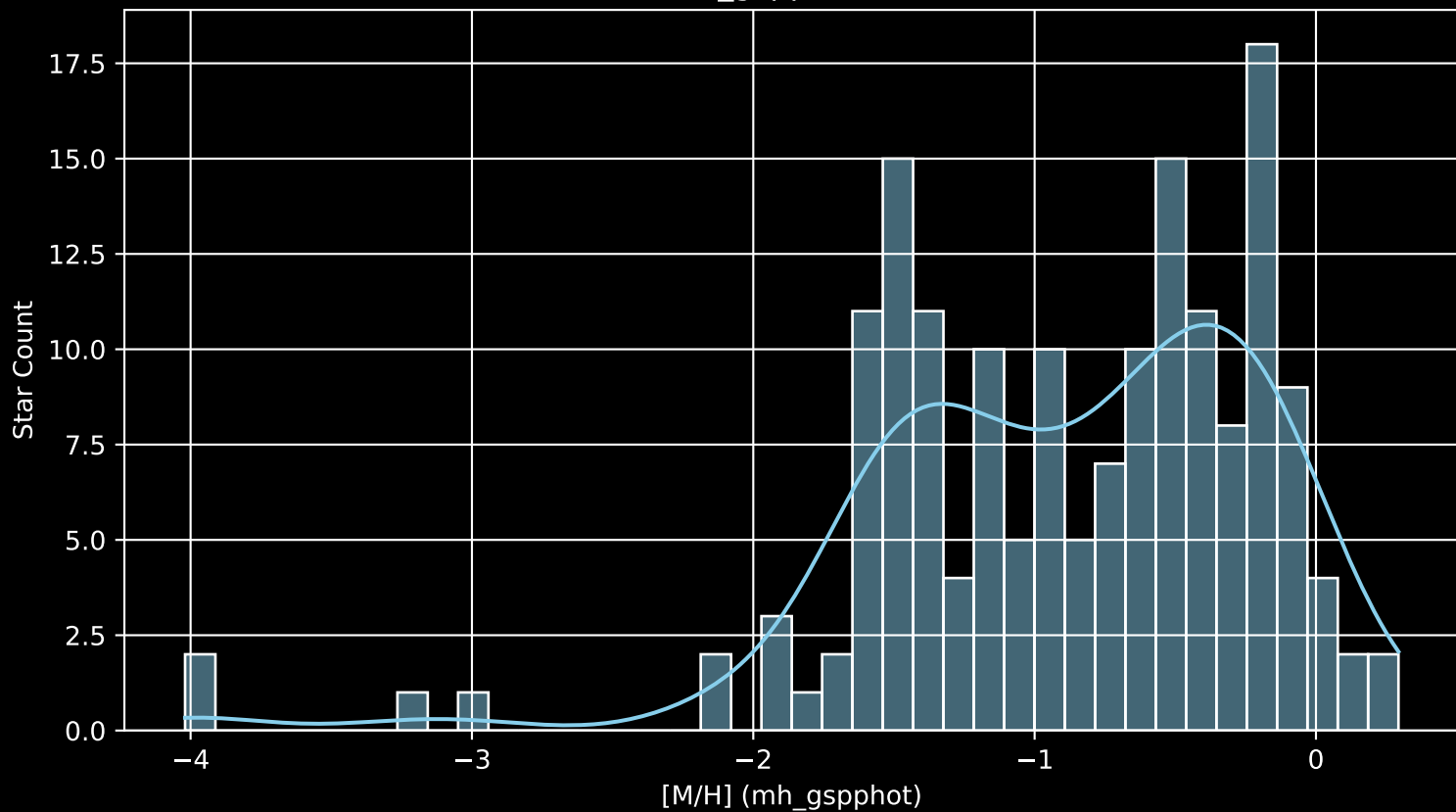
Gaia Cluster: [Berkeley_7 [M/H] (mh_gspphot) (n= 169)
