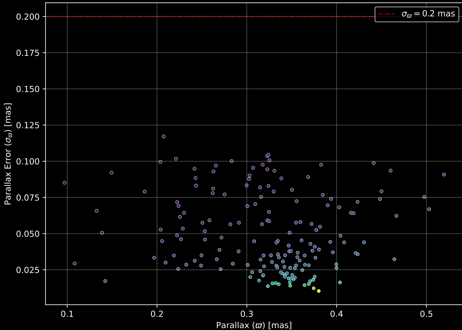
Gaia Cluster: [Berkeley_7] Parallax Quality (n= 170)
