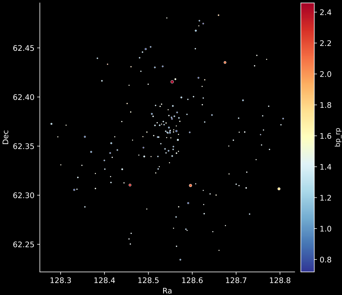
Gaia Cluster: [Berkeley_7] Stars: 170
