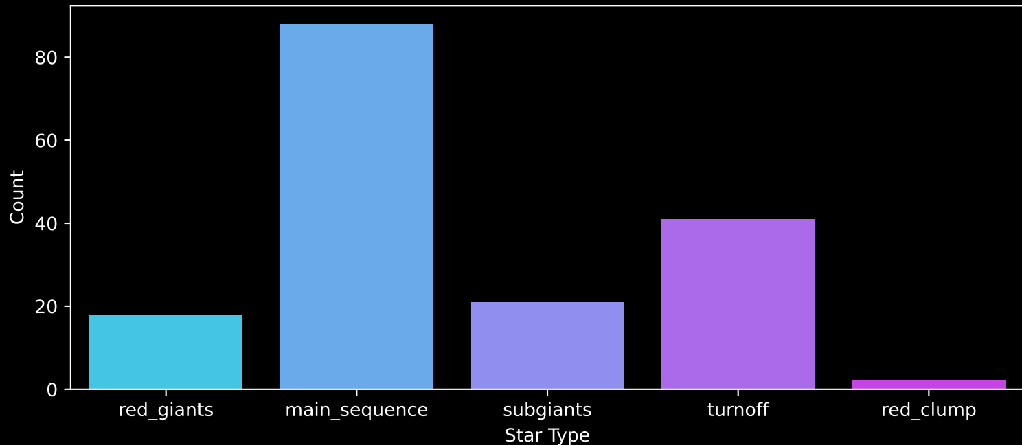
Gaia Cluster: [Berkeley_7] Count plot of Star Type
