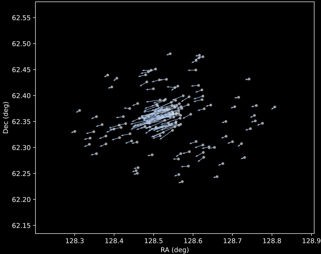
Gaia DR3 Cluster 1 Proper Motion Vectors (n=141)
