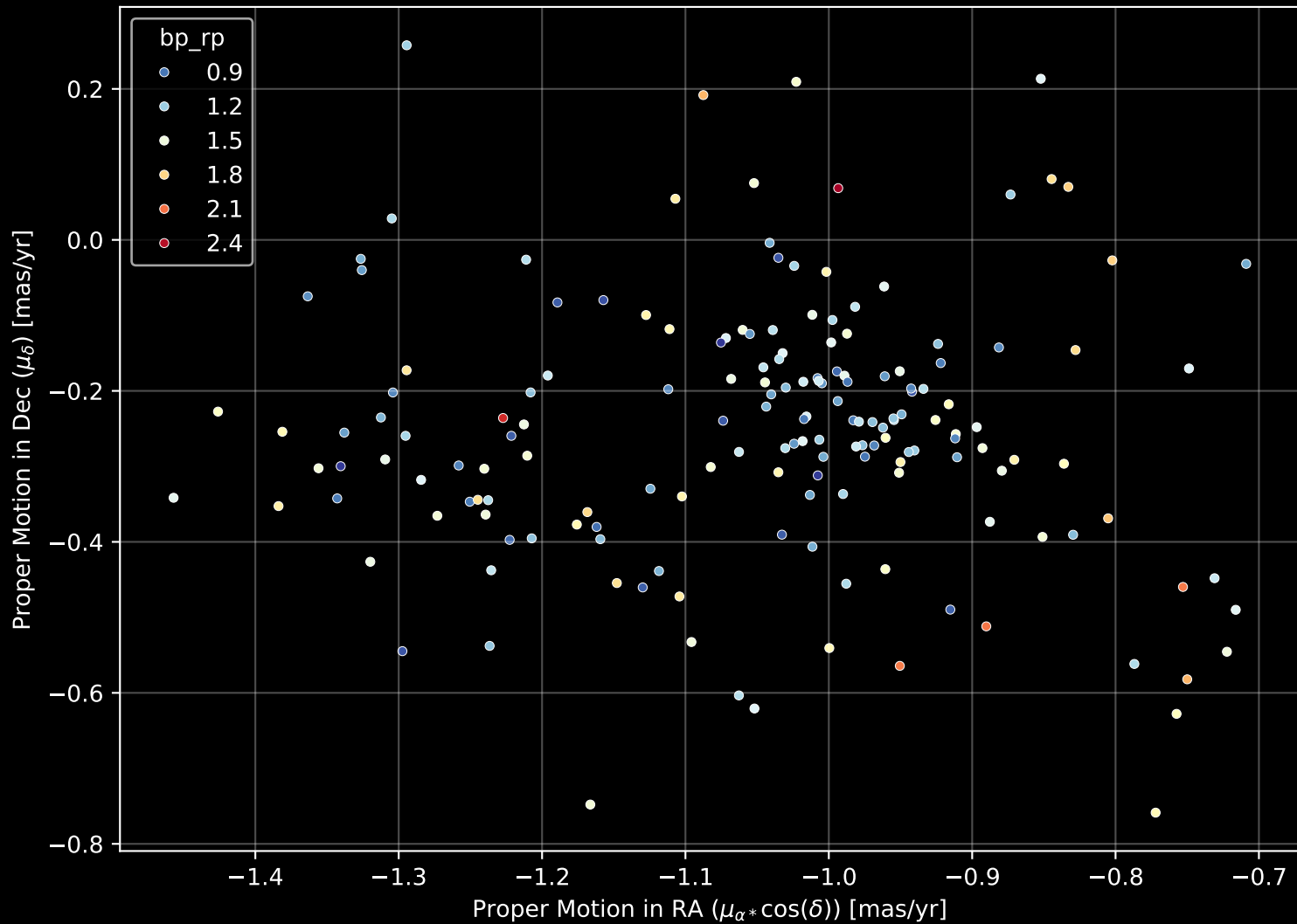
Gaia Cluster: [Berkeley_7] Proper Motion Diagram (n= 170)
