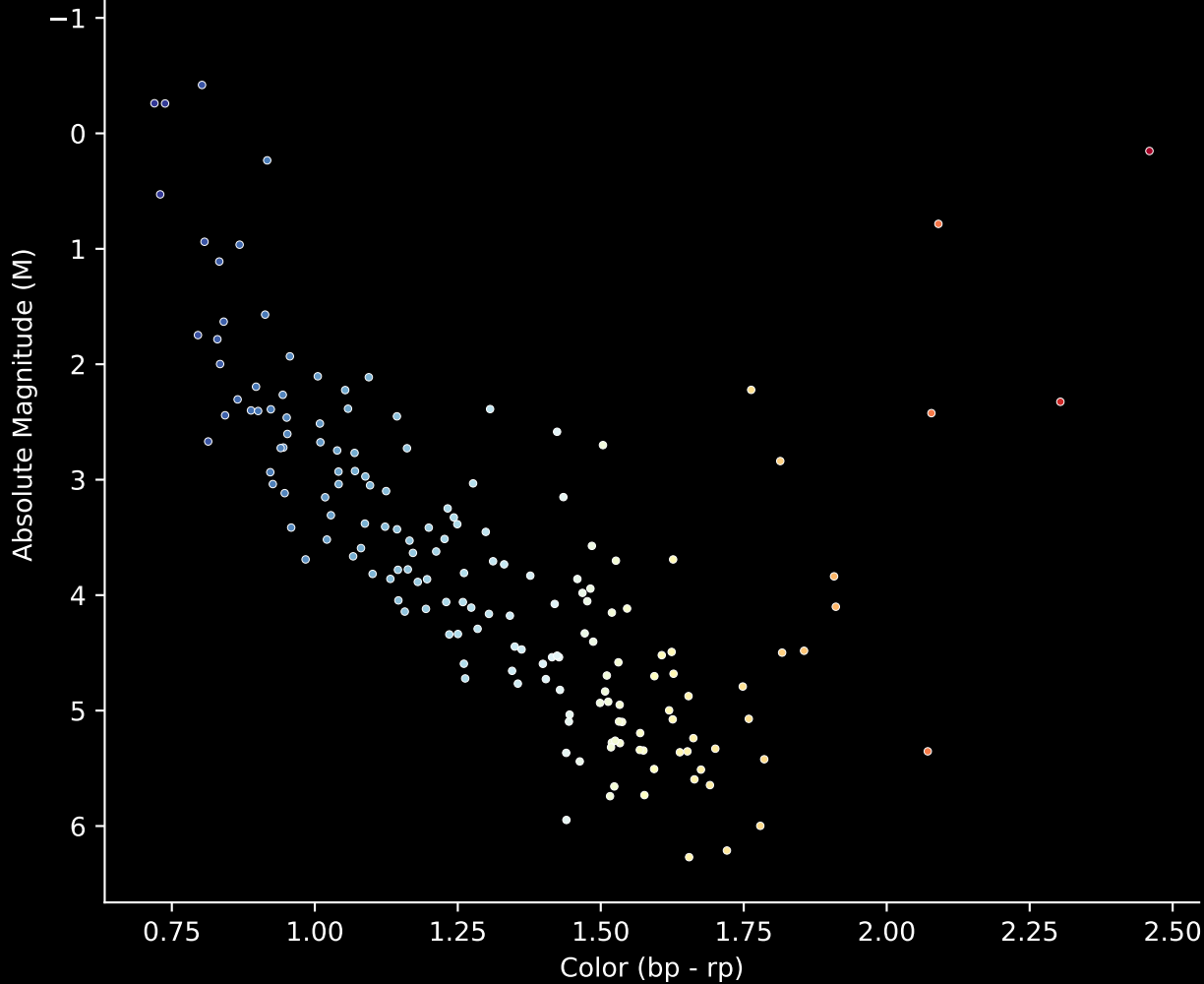
Gaia Cluster: [Berkeley_7] Stars (n= 170) Hertzsprung-Russel Diagram
