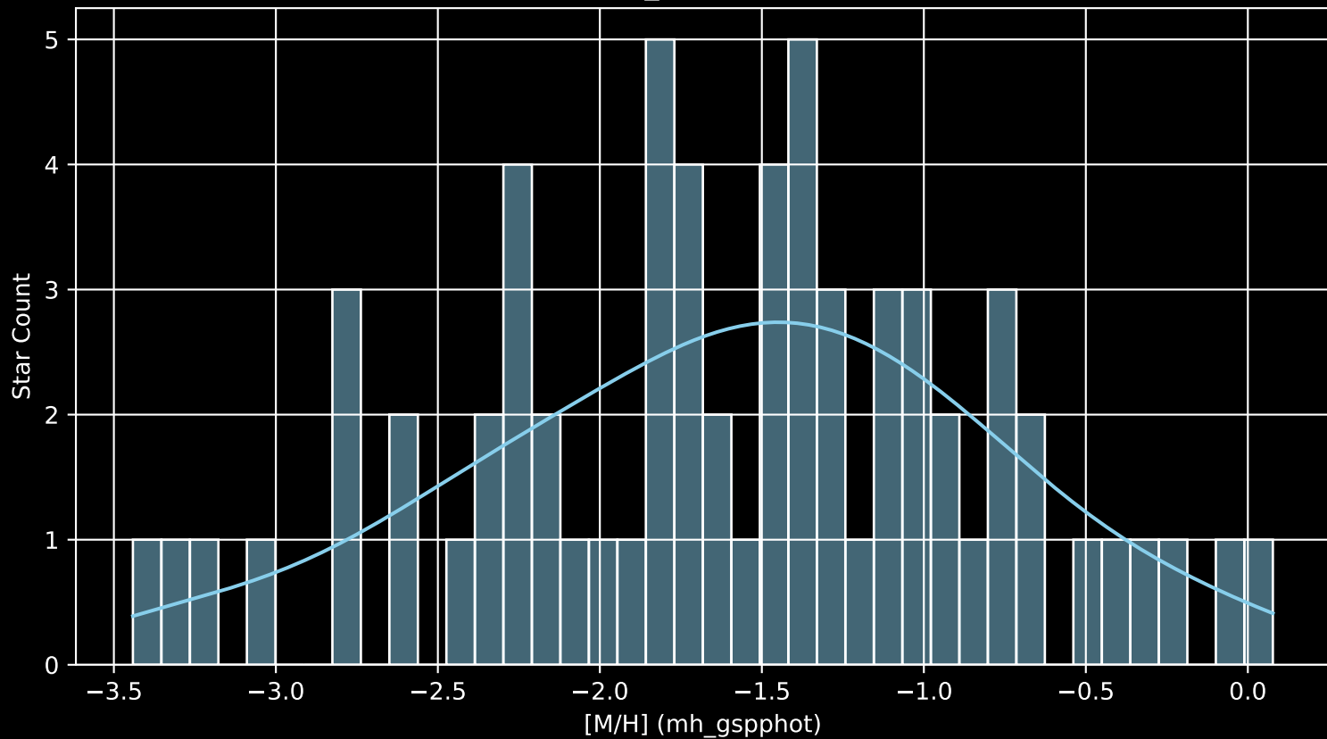
Gaia Cluster: [Berkeley_73 [M/H] (mh_gspphot) (n= 66)
