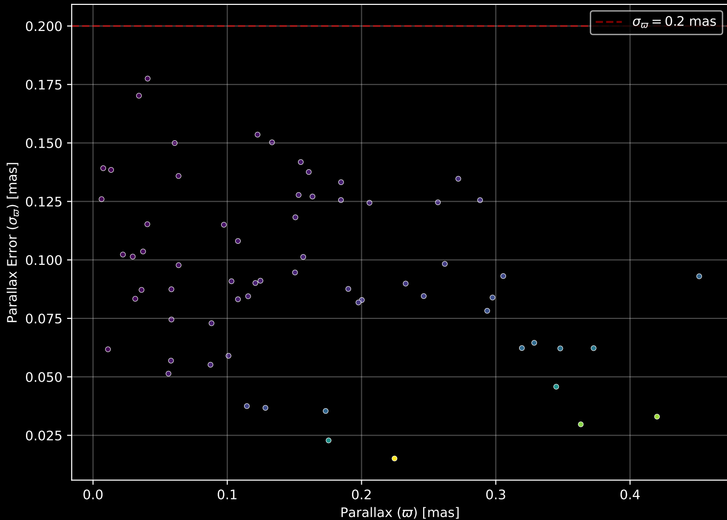
Gaia Cluster: [Berkeley_73] Parallax Quality (n= 66)
