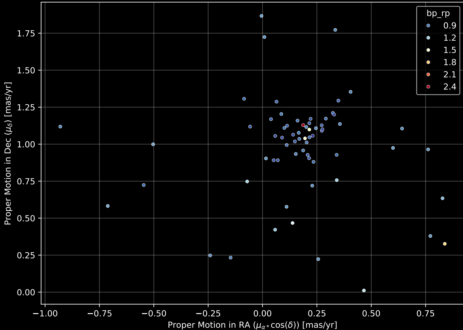
Gaia Cluster: [Berkeley_73] Proper Motion Diagram (n= 66)
