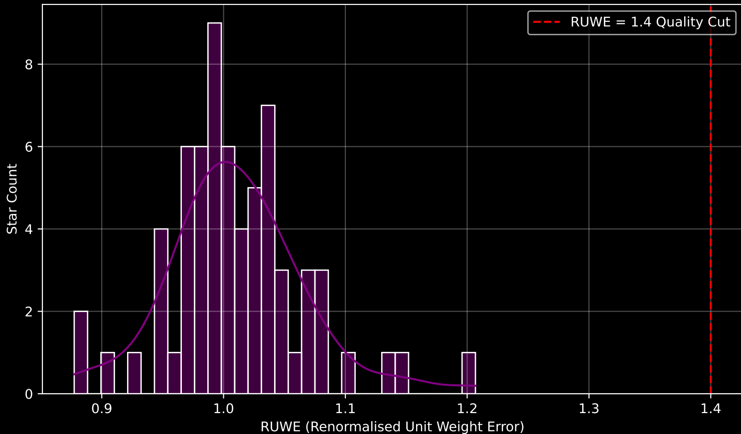
Gaia Cluster: [Berkeley_73] RUWE Distribution (n= 66)
