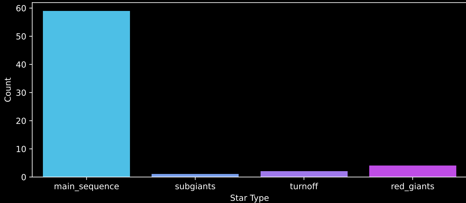
Gaia Cluster: [Berkeley_73] Count plot of Star Type
