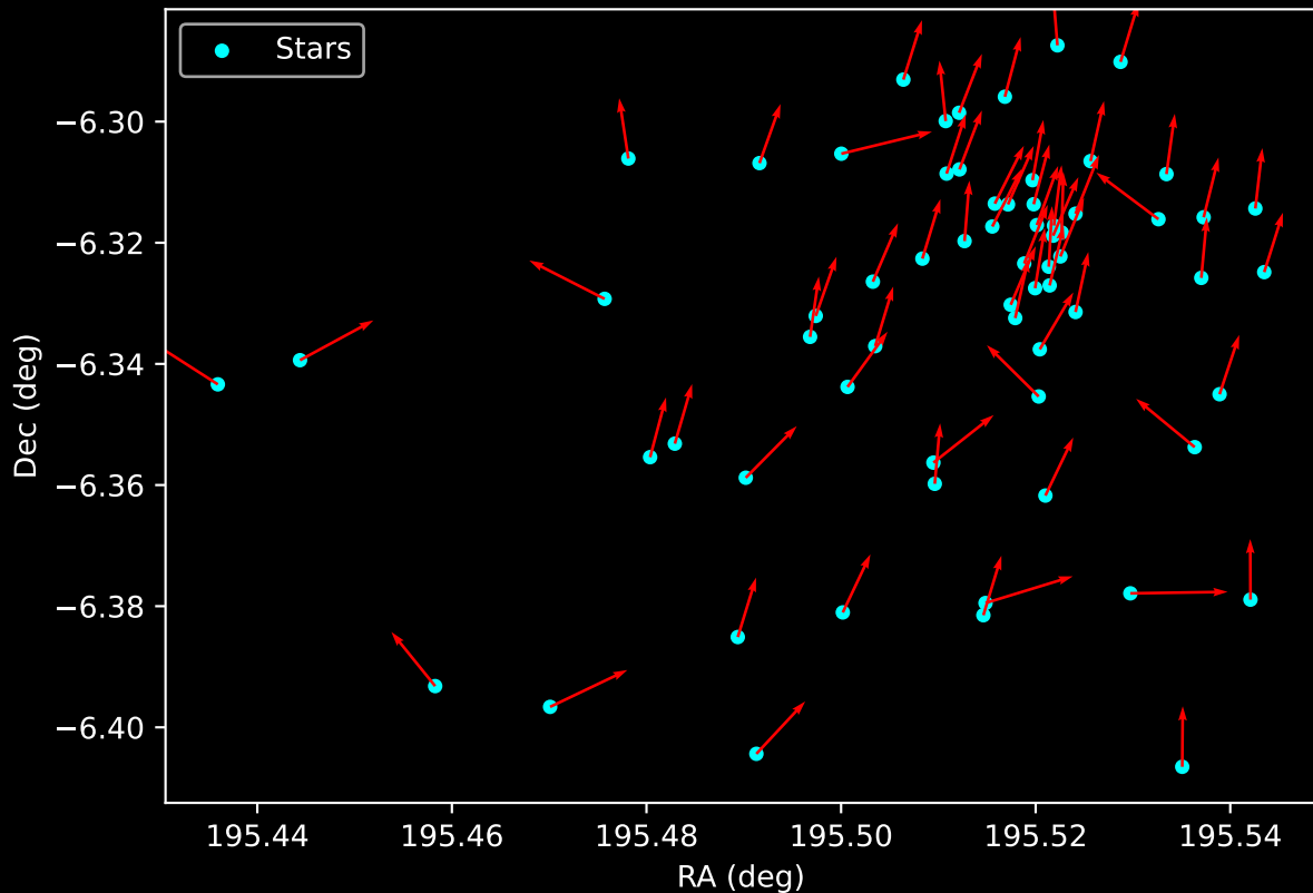
Gaia Cluster: [Berkeley_73] Proper Motion Vectors for Gaia Star Field (n= 66)
