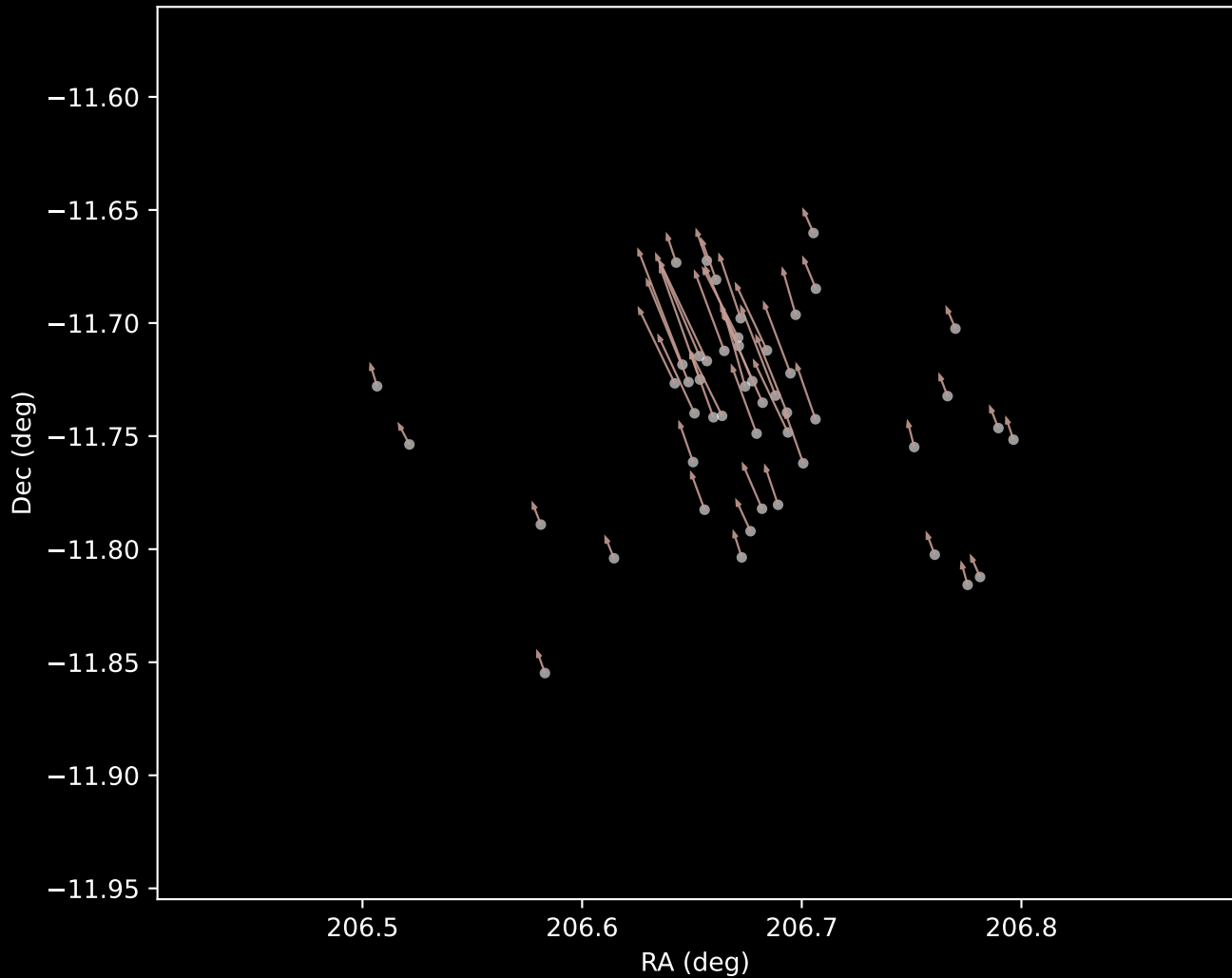
Gaia DR3 Cluster 11 Proper Motion Vectors (n=49)
