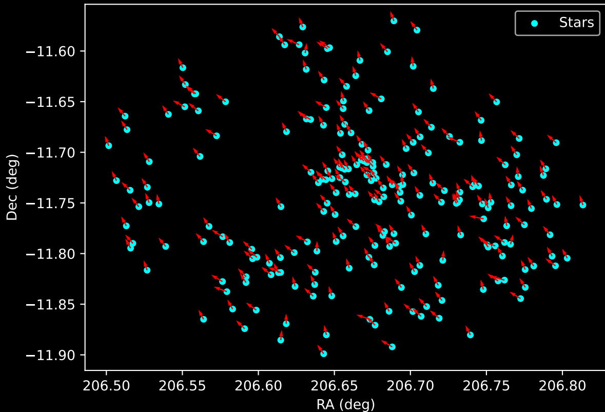
Gaia Cluster: [Berkeley_76] Proper Motion Vectors for Gaia Star Field (n= 220)
