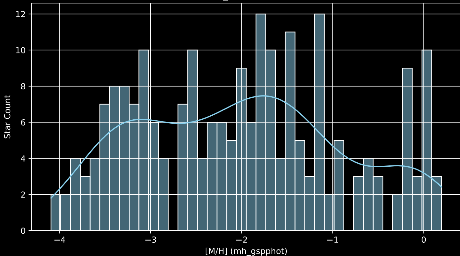
Gaia Cluster: [Berkeley_76 [M/H] (mh_gspphot) (n= 219)
