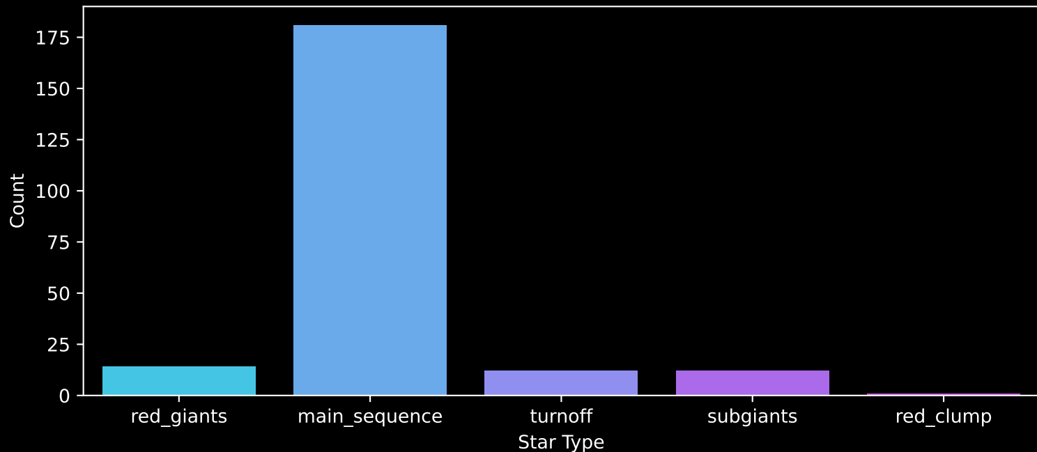
Gaia Cluster: [Berkeley_76] Count plot of Star Type
