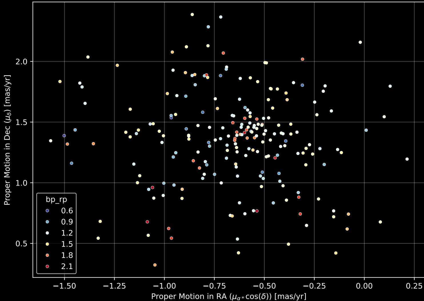
Gaia Cluster: [Berkeley_76] Proper Motion Diagram (n= 220)
