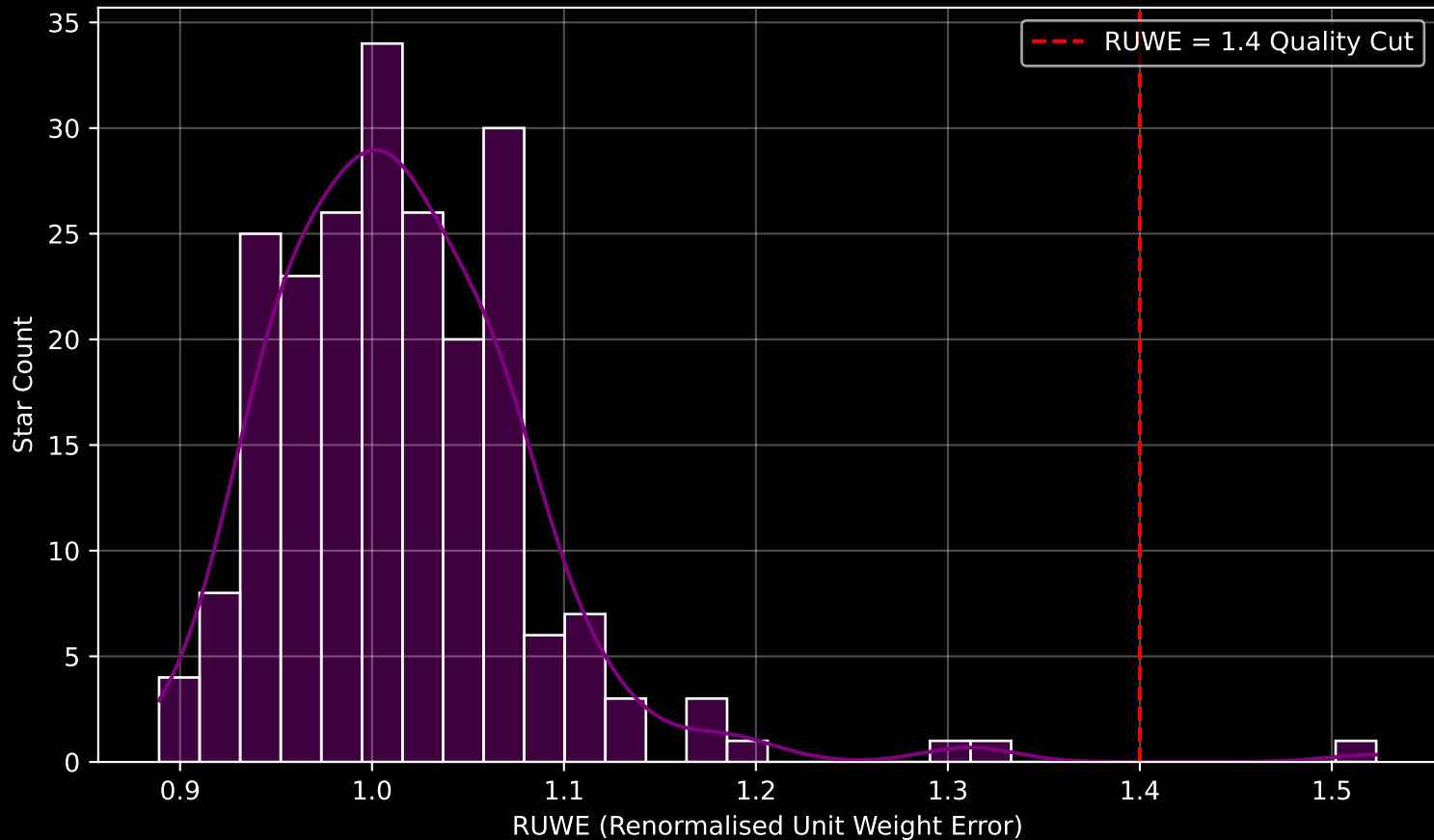
Gaia Cluster: [Berkeley_76] RUWE Distribution (n= 219)
