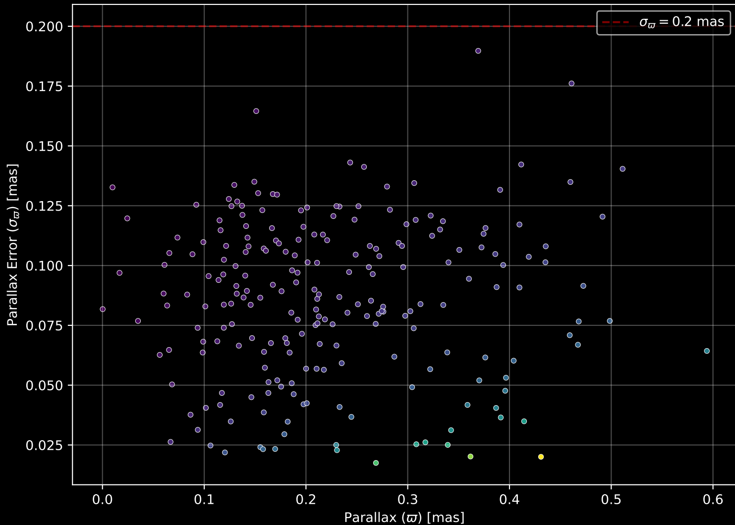
Gaia Cluster: [Berkeley_76] Parallax Quality (n= 220)
