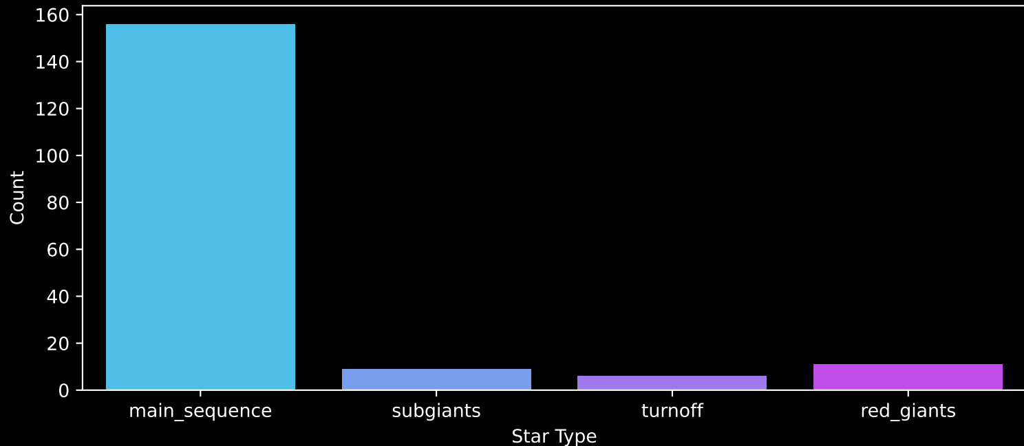
Gaia Cluster: [Berkeley_78] Count plot of Star Type
