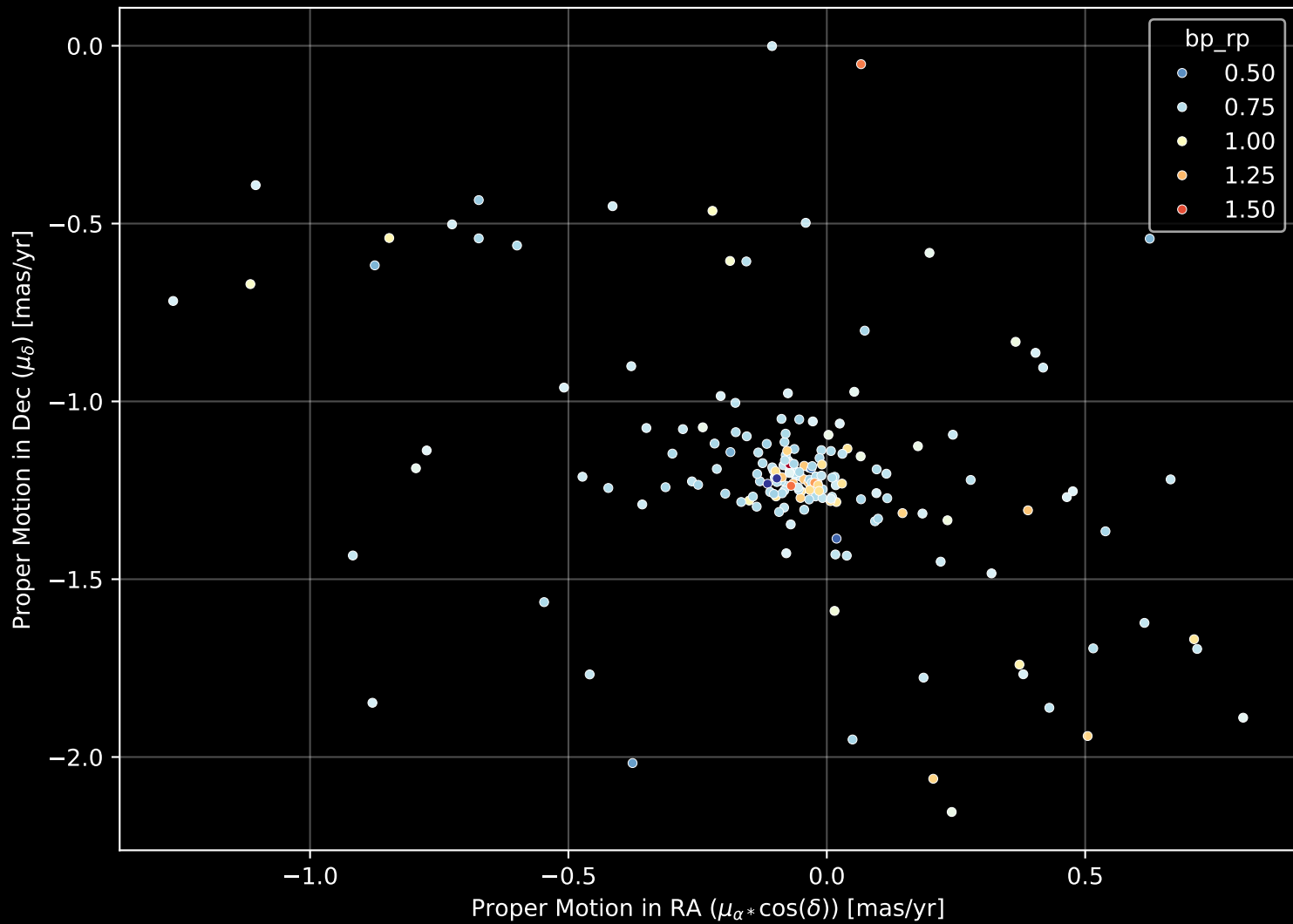
Gaia Cluster: [Berkeley_78] Proper Motion Diagram (n= 182)
