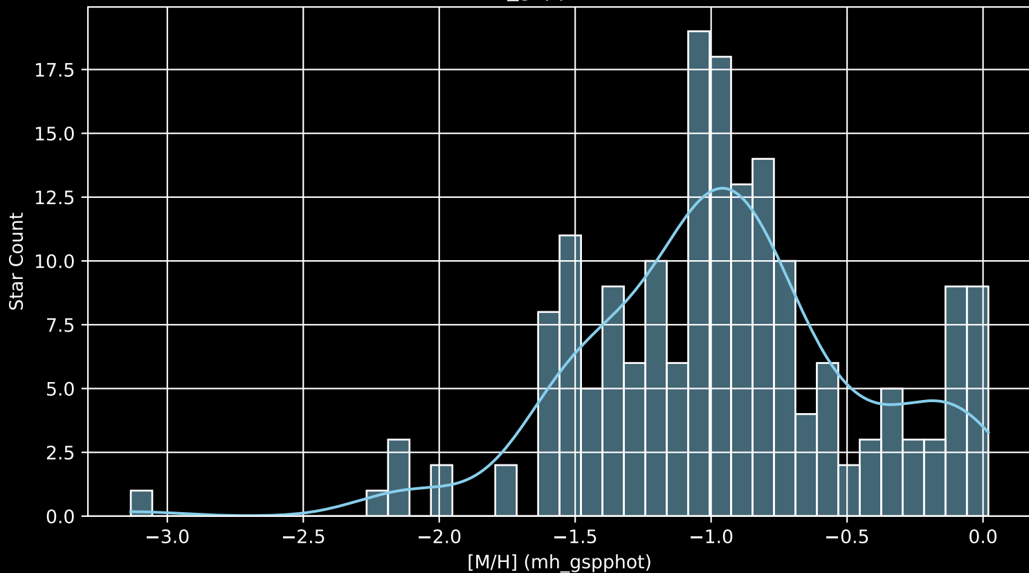
Gaia Cluster: [Berkeley_78 [M/H] (mh_gspphot) (n=182)
