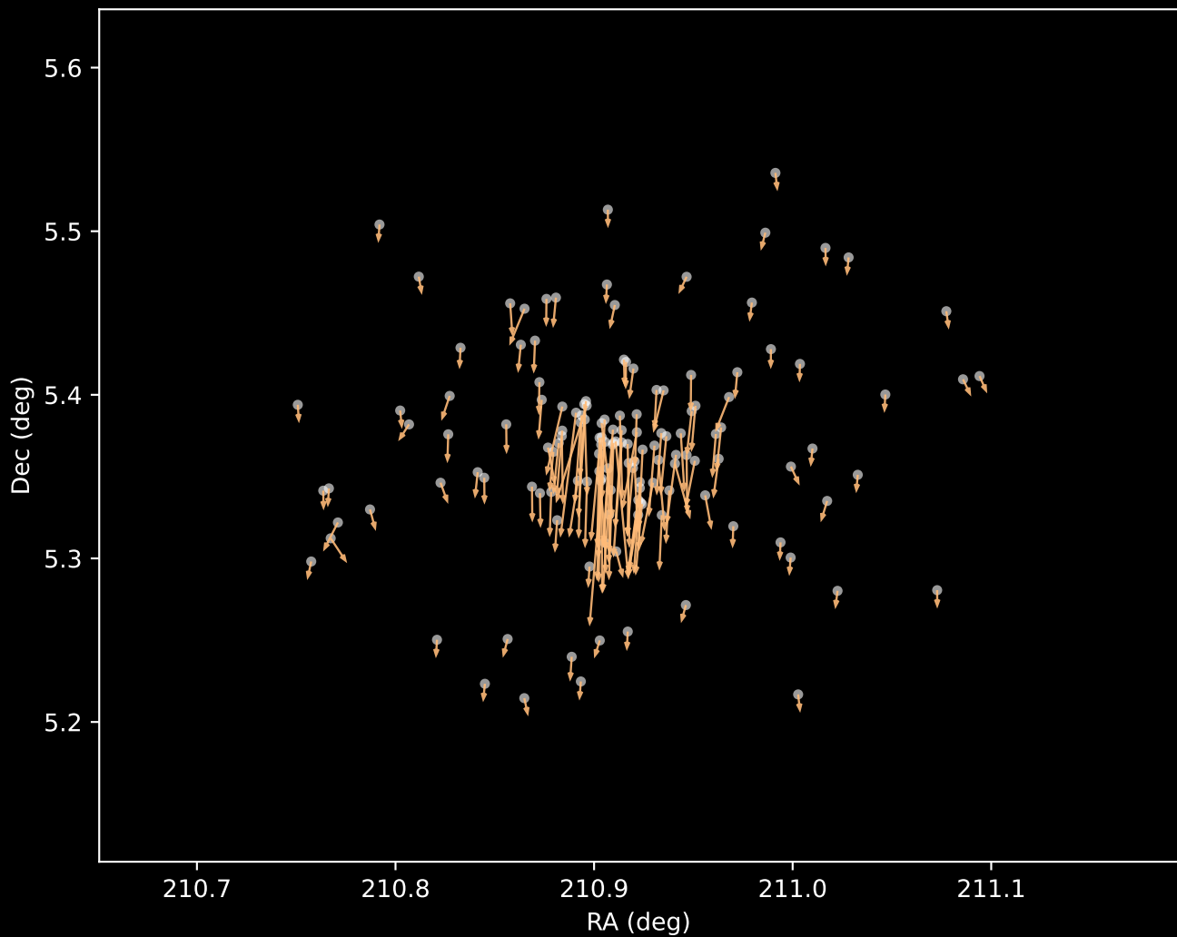
Gaia DR3 Cluster 3 Proper Motion Vectors (n=141)
