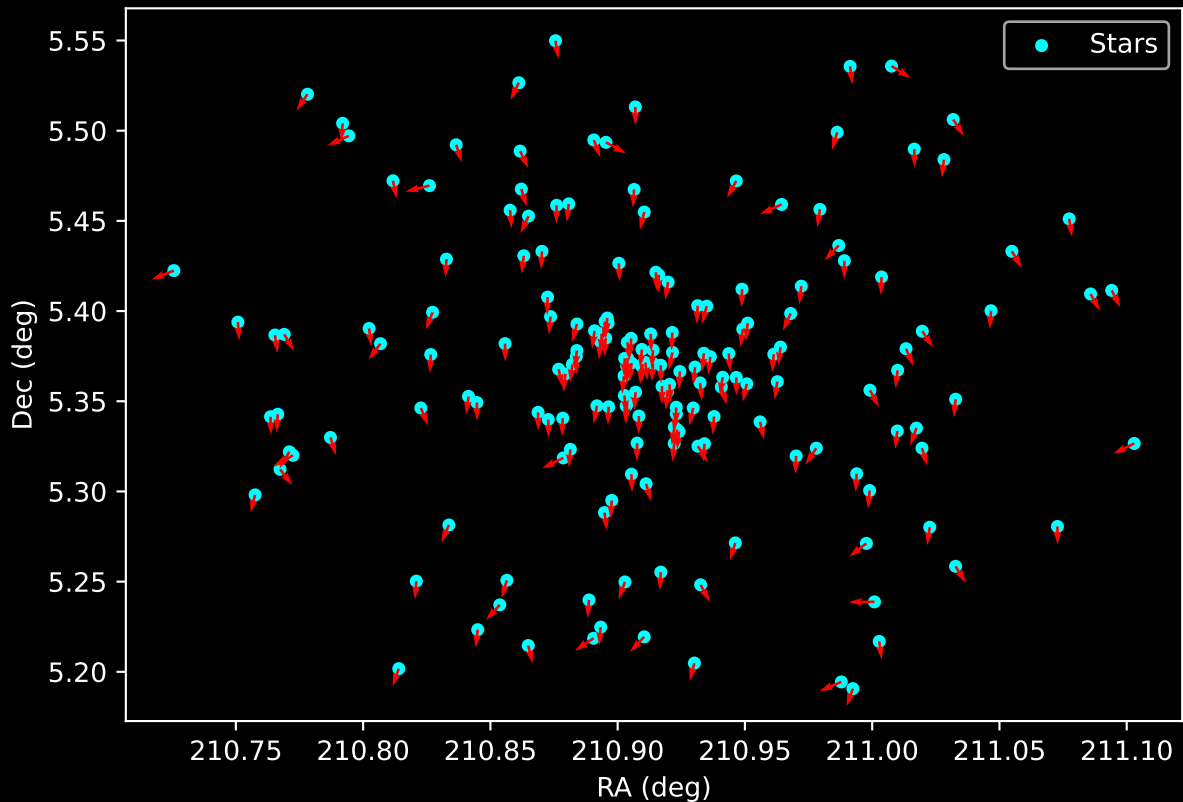
Gaia Cluster: [Berkeley_78] Proper Motion Vectors for Gaia Star Field (n= 182)
