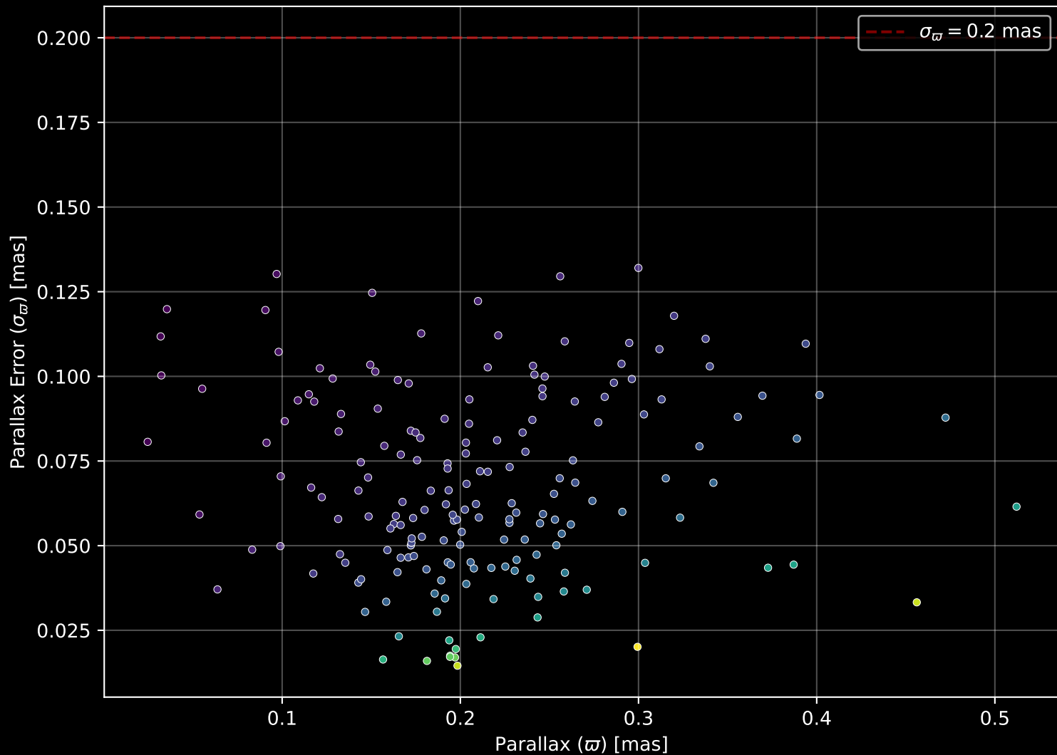
Gaia Cluster: [Berkeley_78] Parallax Quality (n= 182)
