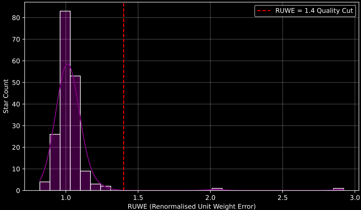
Gaia Cluster: [Berkeley_78] RUWE Distribution (n= 182)
