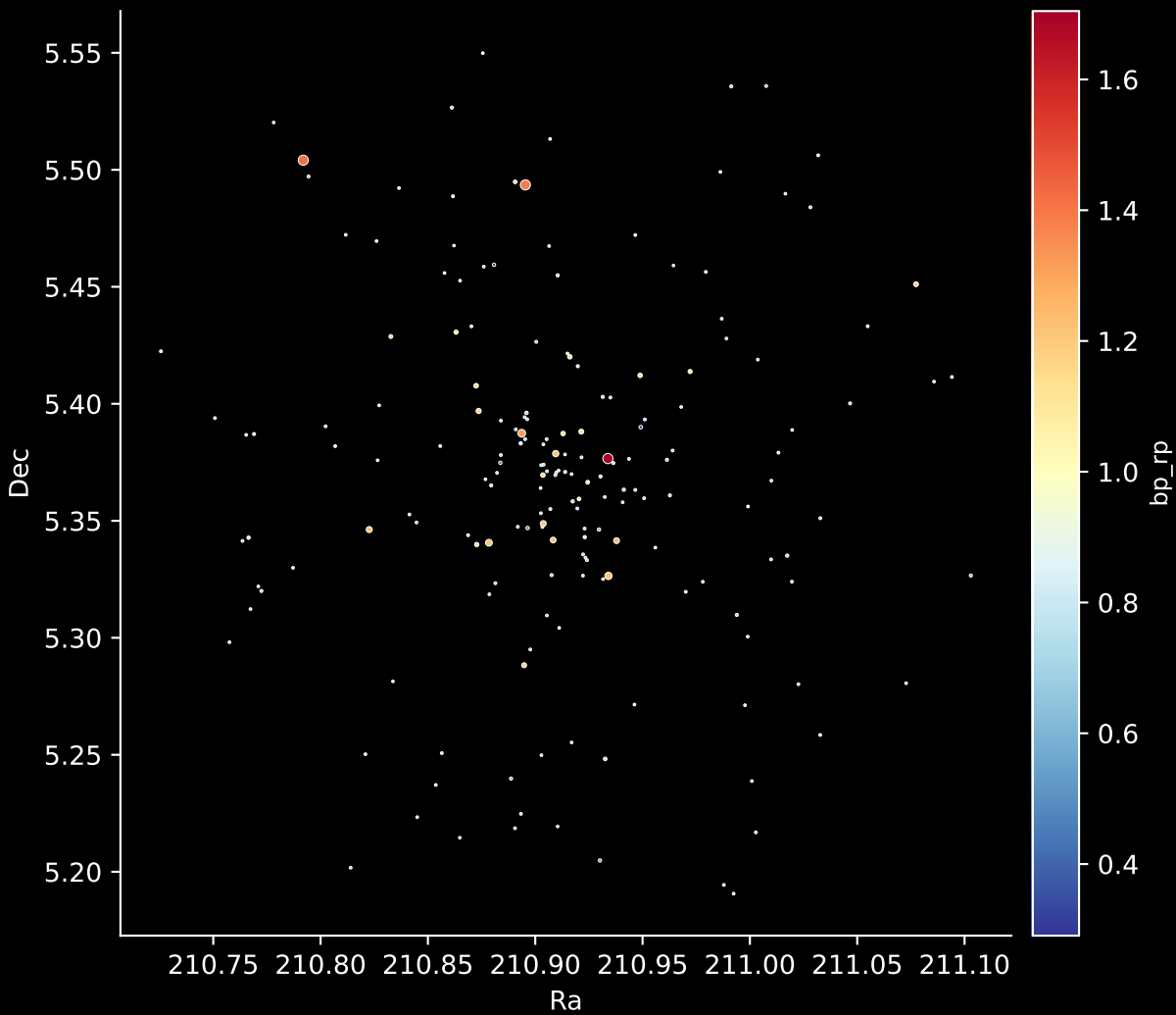
Gaia Cluster: [Berkeley_78] Stars: 182
