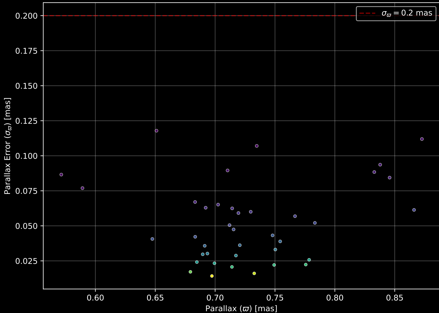
Gaia Cluster: [Berkeley_82] Parallax Quality (n= 39)
