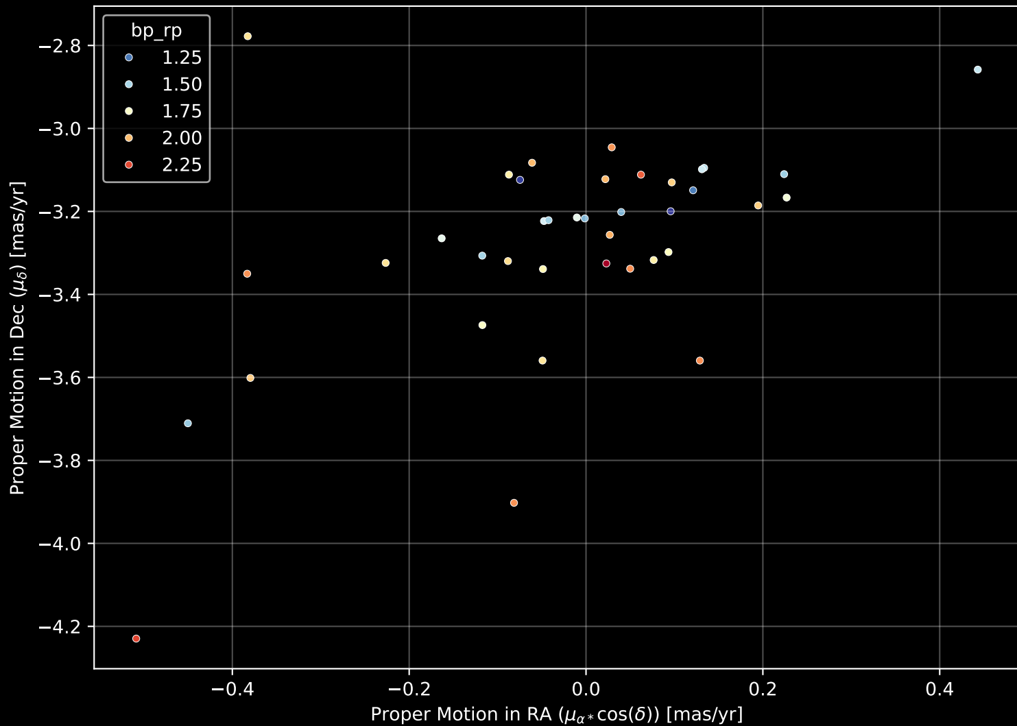
Gaia Cluster: [Berkeley_82] Proper Motion Diagram (n= 39)
