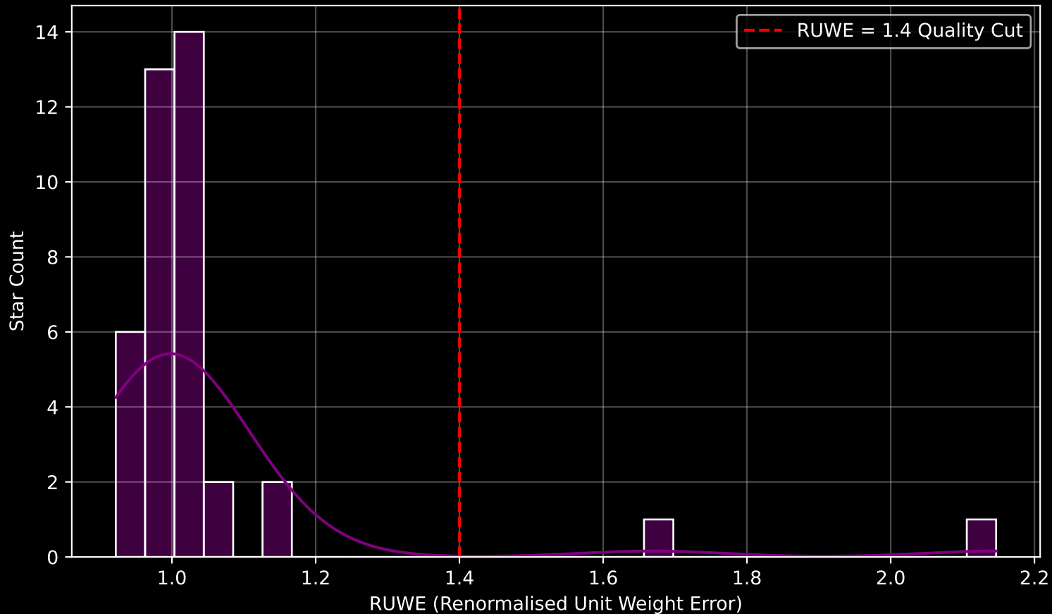
Gaia Cluster: [Berkeley_82] RUWE Distribution (n= 39)
