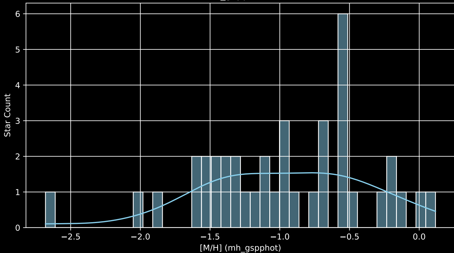
Gaia Cluster: [Berkeley_82 [M/H] (mh_gspphot) (n= 39)
