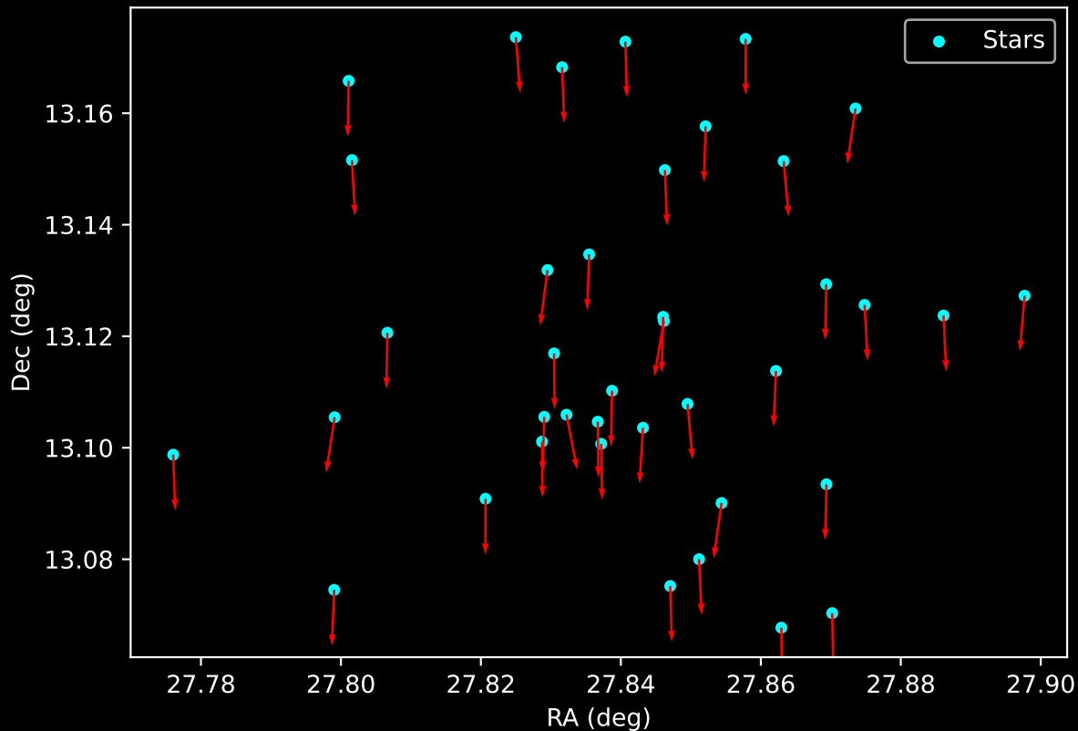
Gaia Cluster: [Berkeley_82] Proper Motion Vectors for Gaia Star Field (n= 39)
