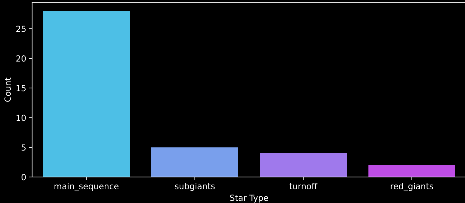
Gaia Cluster: [Berkeley_82] Count plot of Star Type
