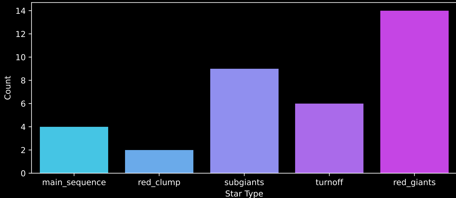
Gaia Cluster: [Berkeley_83] Count plot of Star Type
