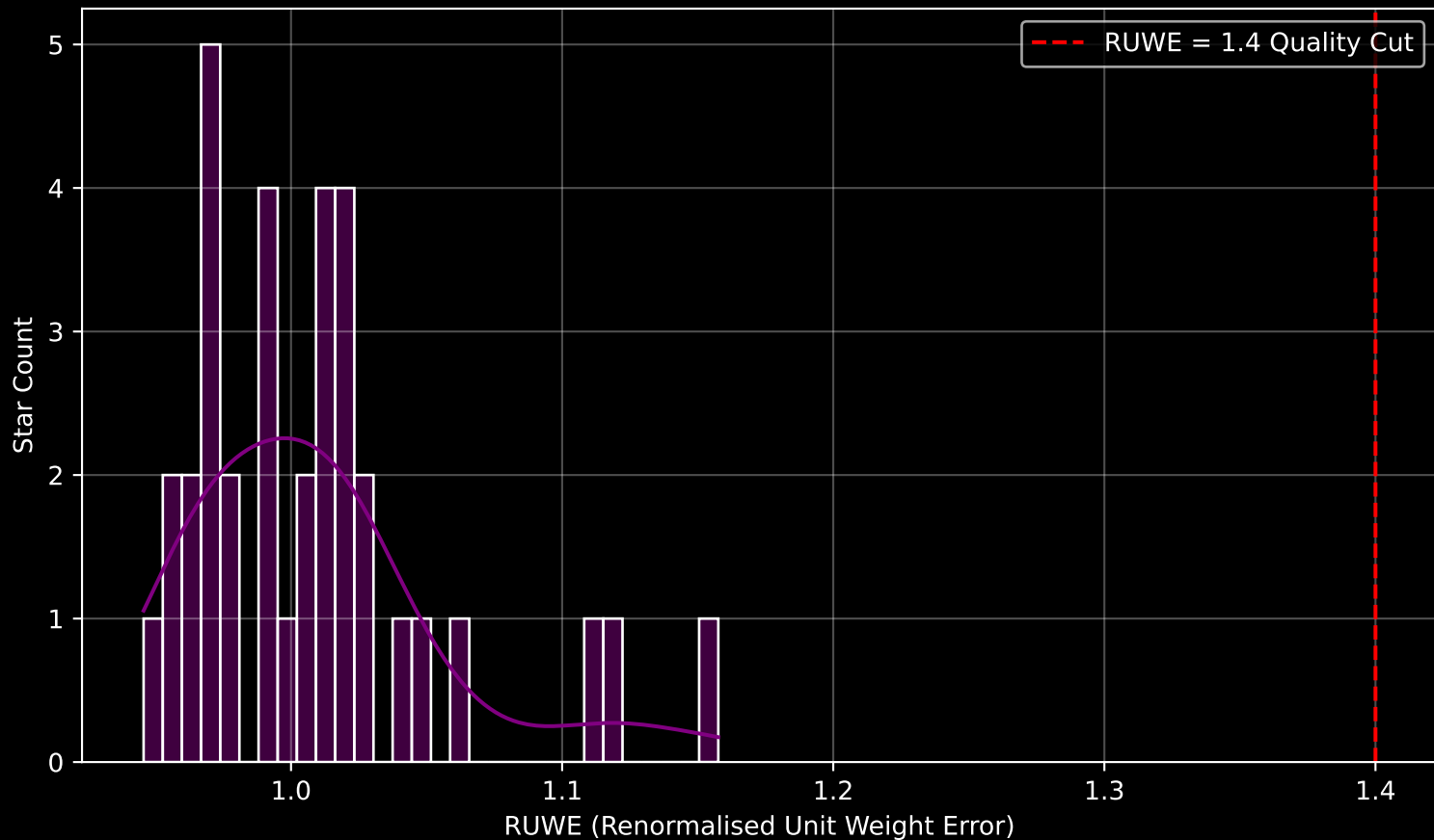
Gaia Cluster: [Berkeley_83] RUWE Distribution (n= 35)
