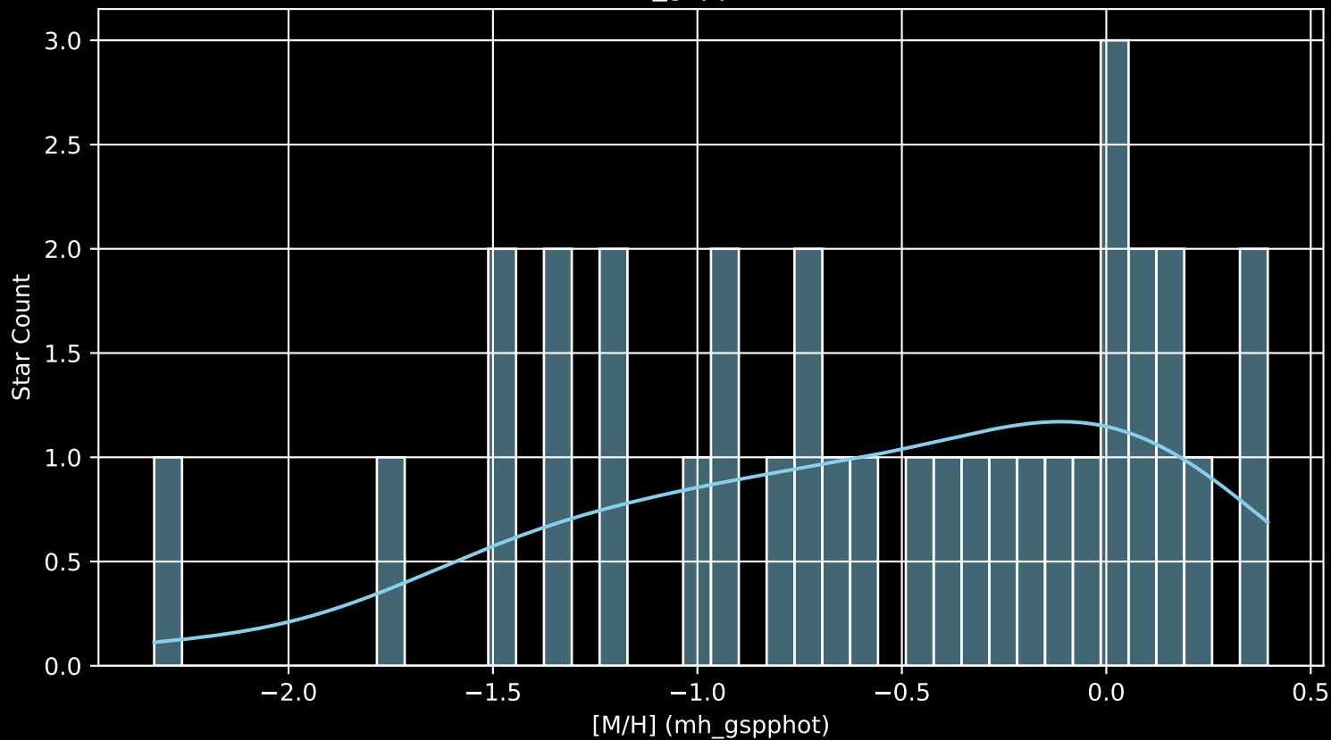
Gaia Cluster: [Berkeley_83 [M/H] (mh_gspphot) (n= 33)
