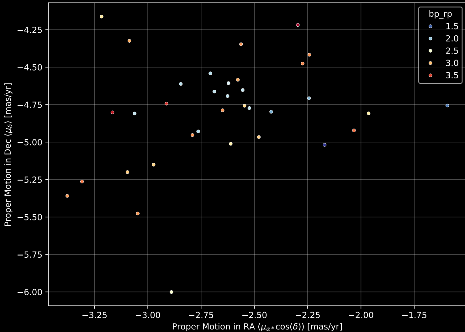
Gaia Cluster: [Berkeley_83] Proper Motion Diagram (n= 35)
