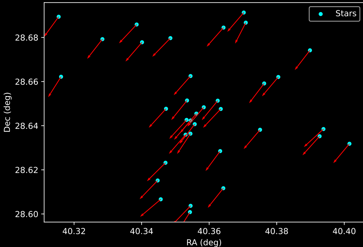
Gaia Cluster: [Berkeley_83] Proper Motion Vectors for Gaia Star Field (n= 35)
