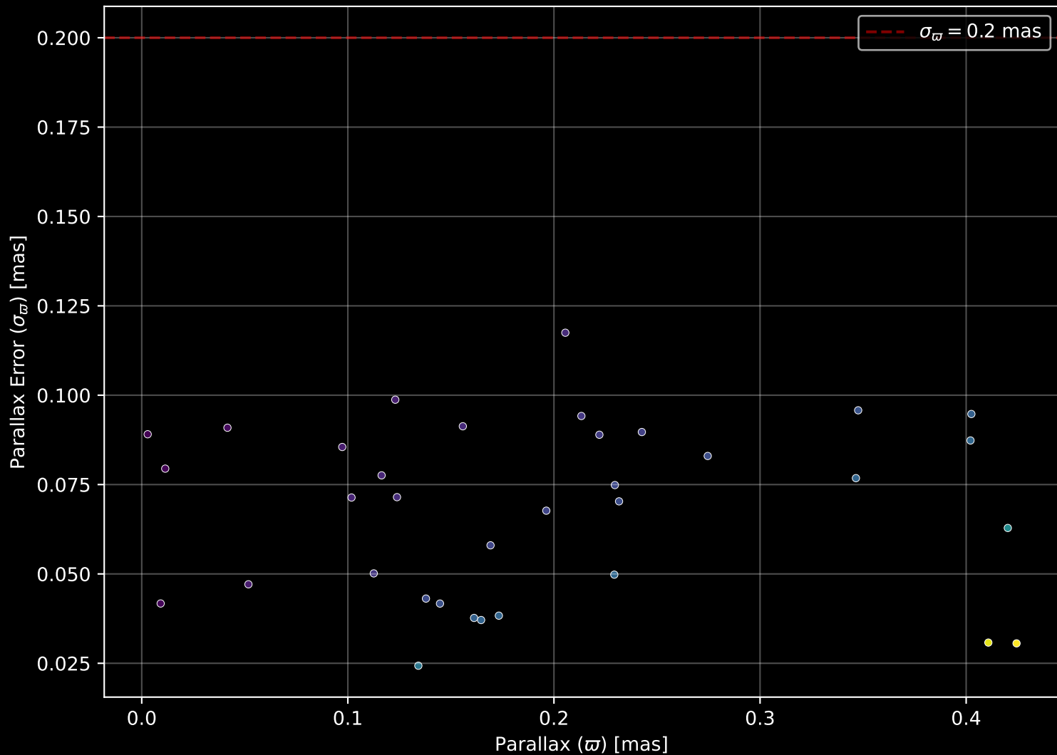
Gaia Cluster: [Berkeley_83] Parallax Quality (n= 35)
