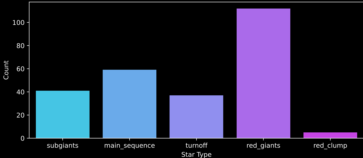
Gaia Cluster: [Berkeley_85] Count plot of Star Type
