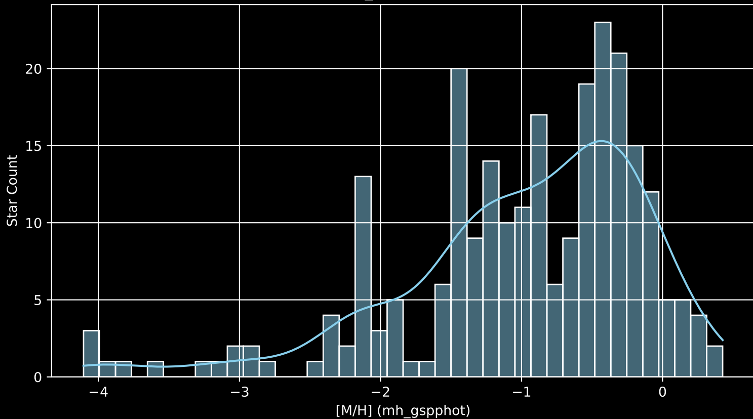
Gaia Cluster: [Berkeley_85 [M/H] (mh_gspphot) (n= 251)
