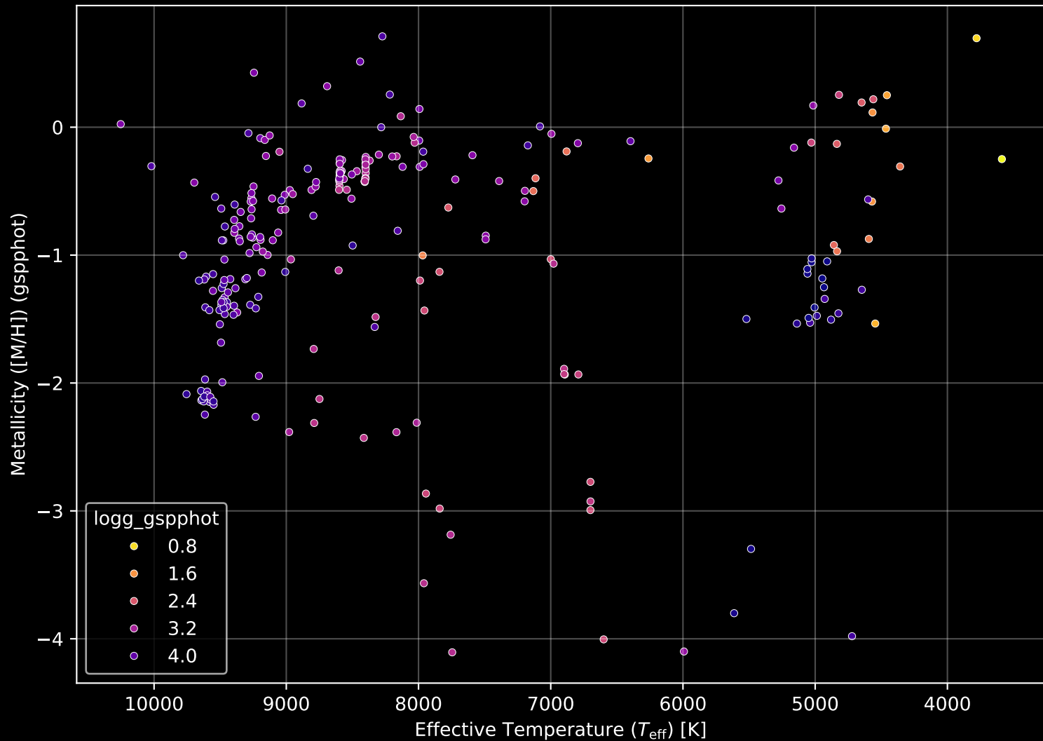
Gaia Cluster: [Berkeley_85] Stellar Population Parameters (n= 254)
