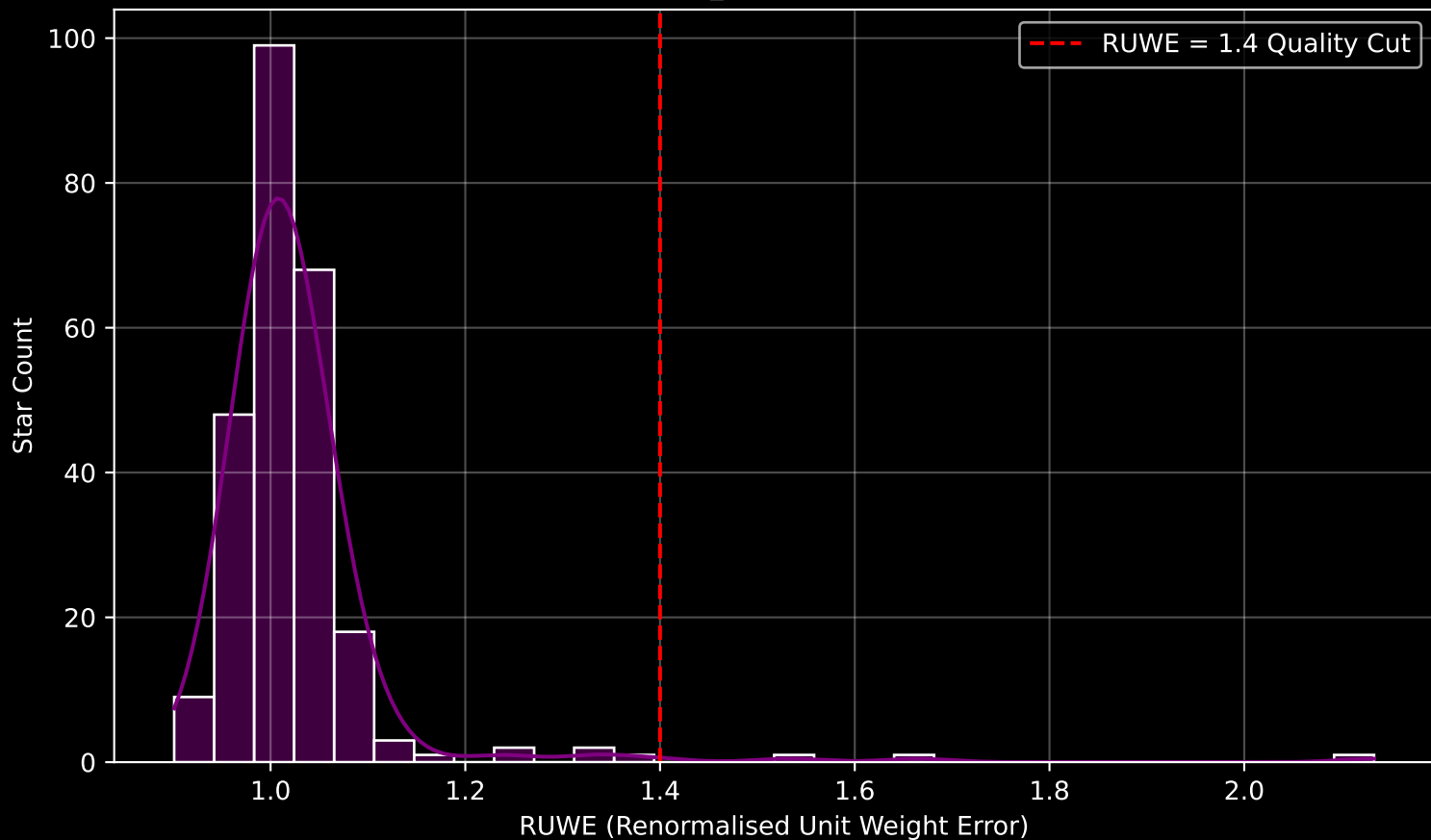
Gaia Cluster: [Berkeley_85] RUWE Distribution (n= 254)
