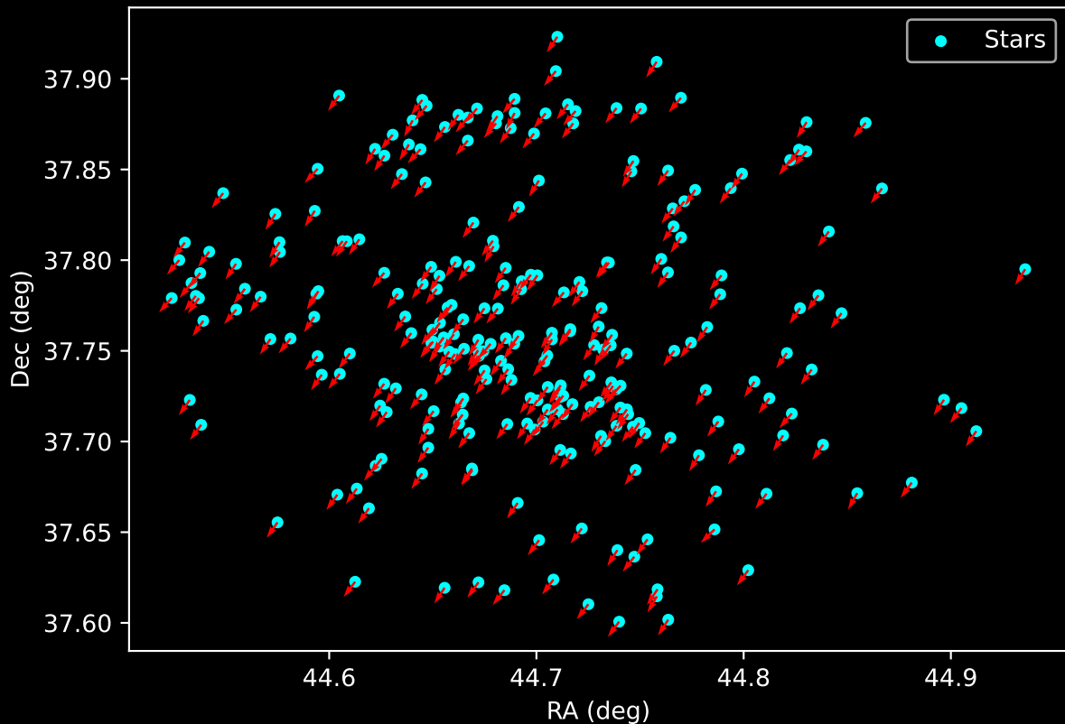
Gaia Cluster: [Berkeley_85] Proper Motion Vectors for Gaia Star Field (n= 254)
