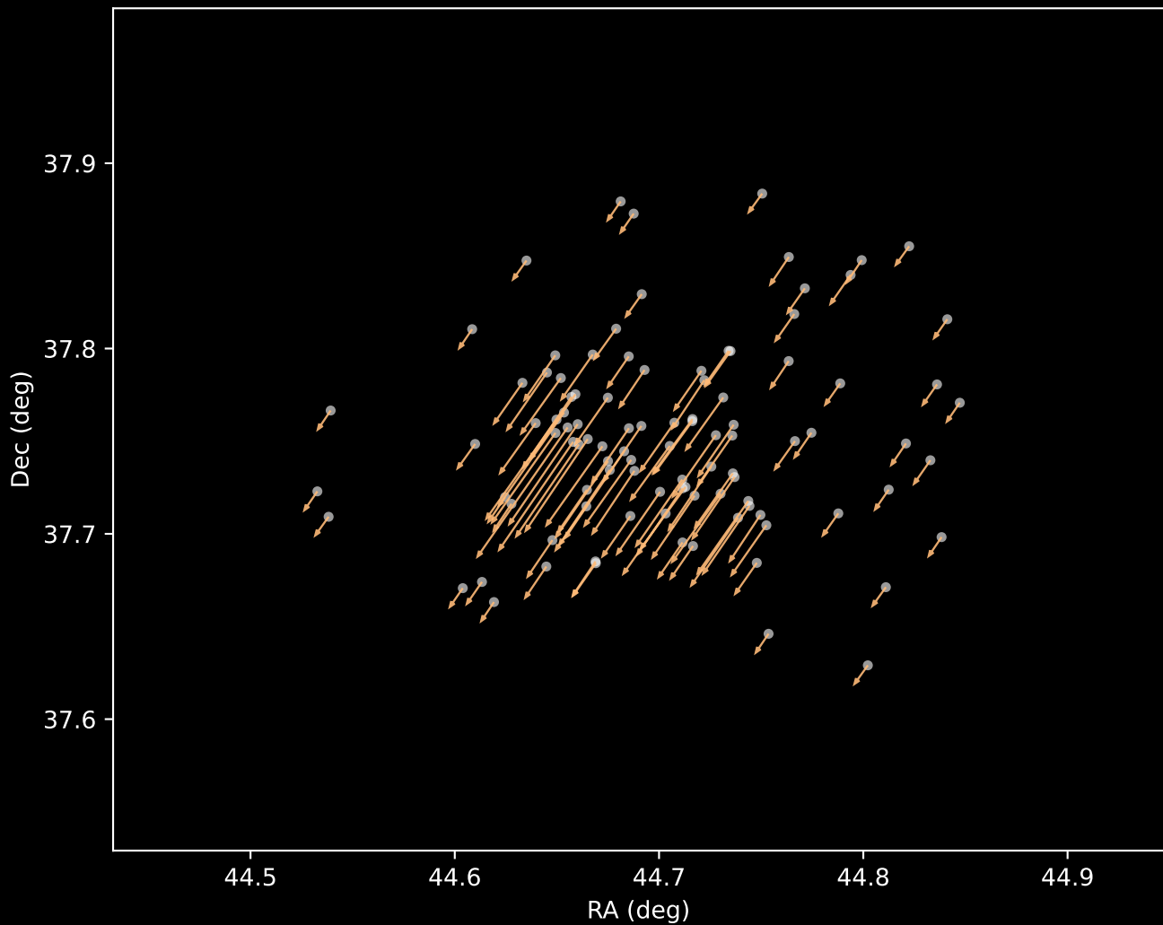
Gaia DR3 Cluster 3 Proper Motion Vectors (n=101)
