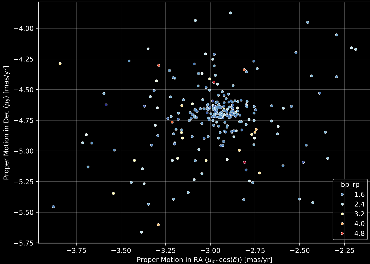
Gaia Cluster: [Berkeley_85] Proper Motion Diagram (n= 254)
