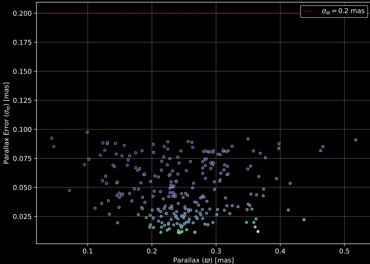
Gaia Cluster: [Berkeley_85] Parallax Quality (n= 254)
