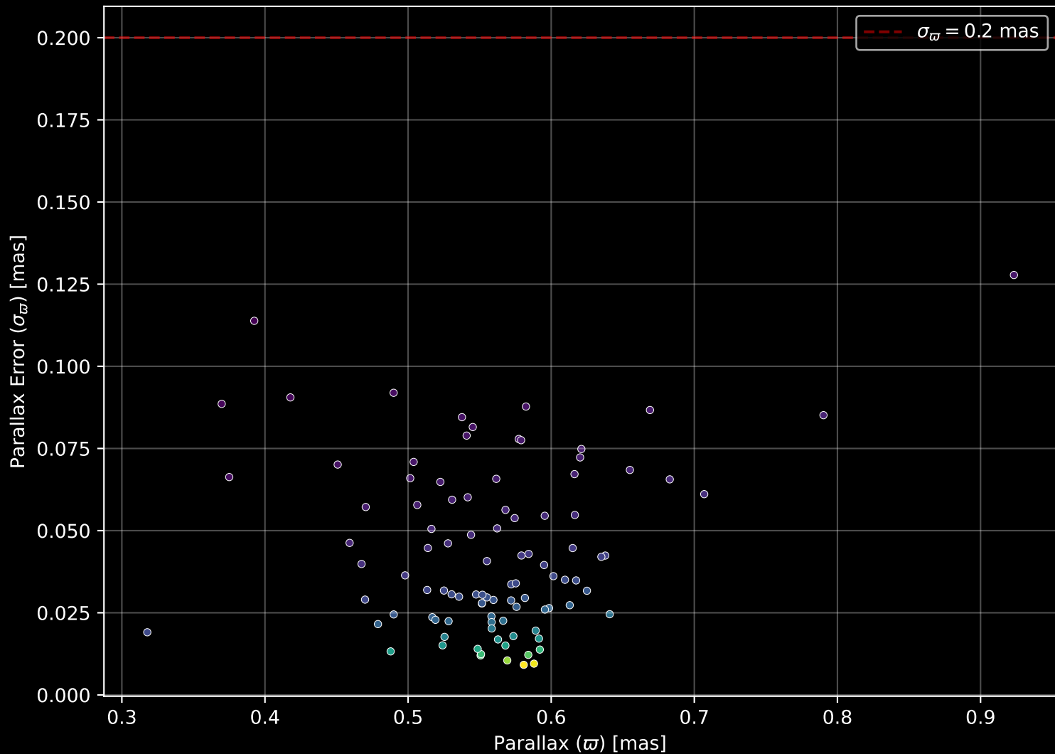
Gaia Cluster: [Berkeley_86] Parallax Quality (n= 98)
