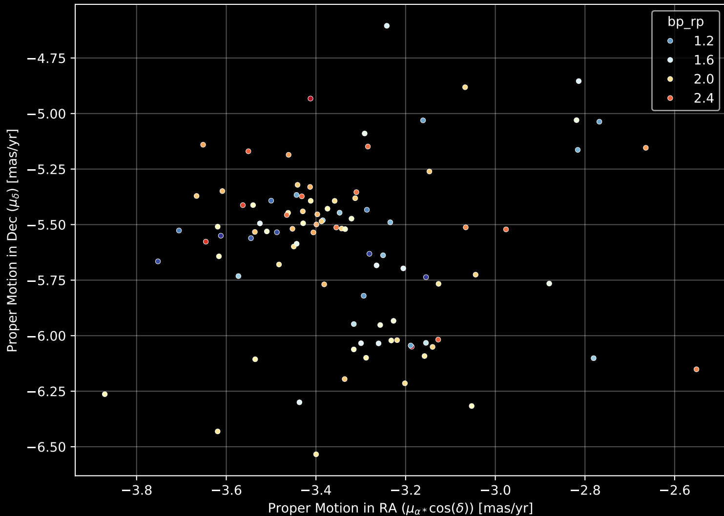
Gaia Cluster: [Berkeley_86] Proper Motion Diagram (n= 98)
