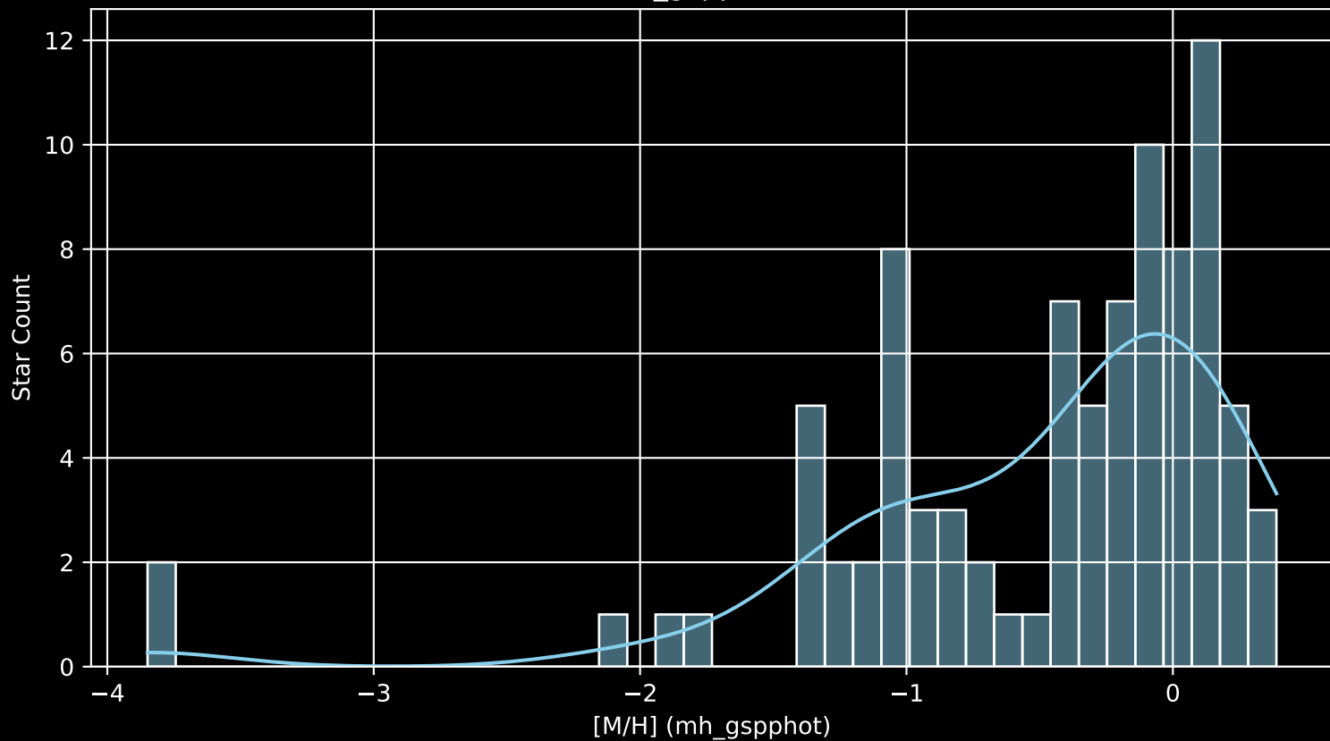
Gaia Cluster: [Berkeley_86 [M/H] (mh_gspphot) (n= 89)
