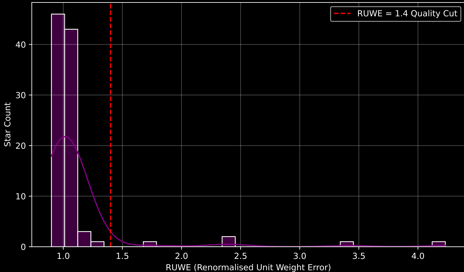
Gaia Cluster: [Berkeley_86] RUWE Distribution (n= 98)
