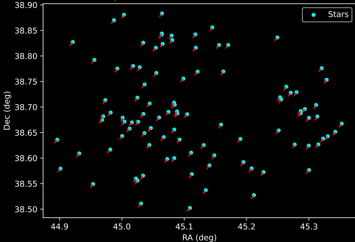
Gaia Cluster: [Berkeley_86] Proper Motion Vectors for Gaia Star Field (n= 98)
