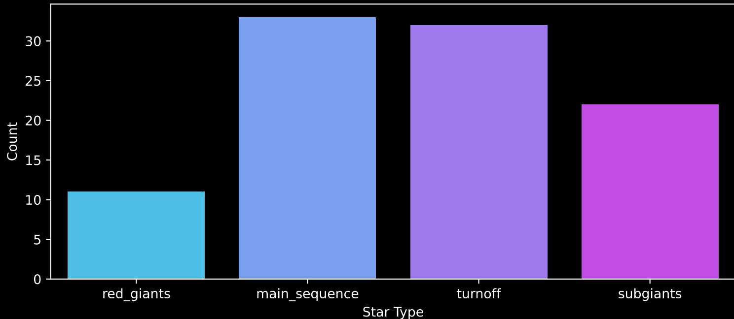
Gaia Cluster: [Berkeley_86] Count plot of Star Type
