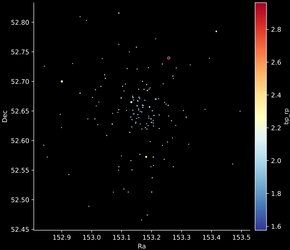
Gaia Cluster: [Berkeley_9] Stars: 141
