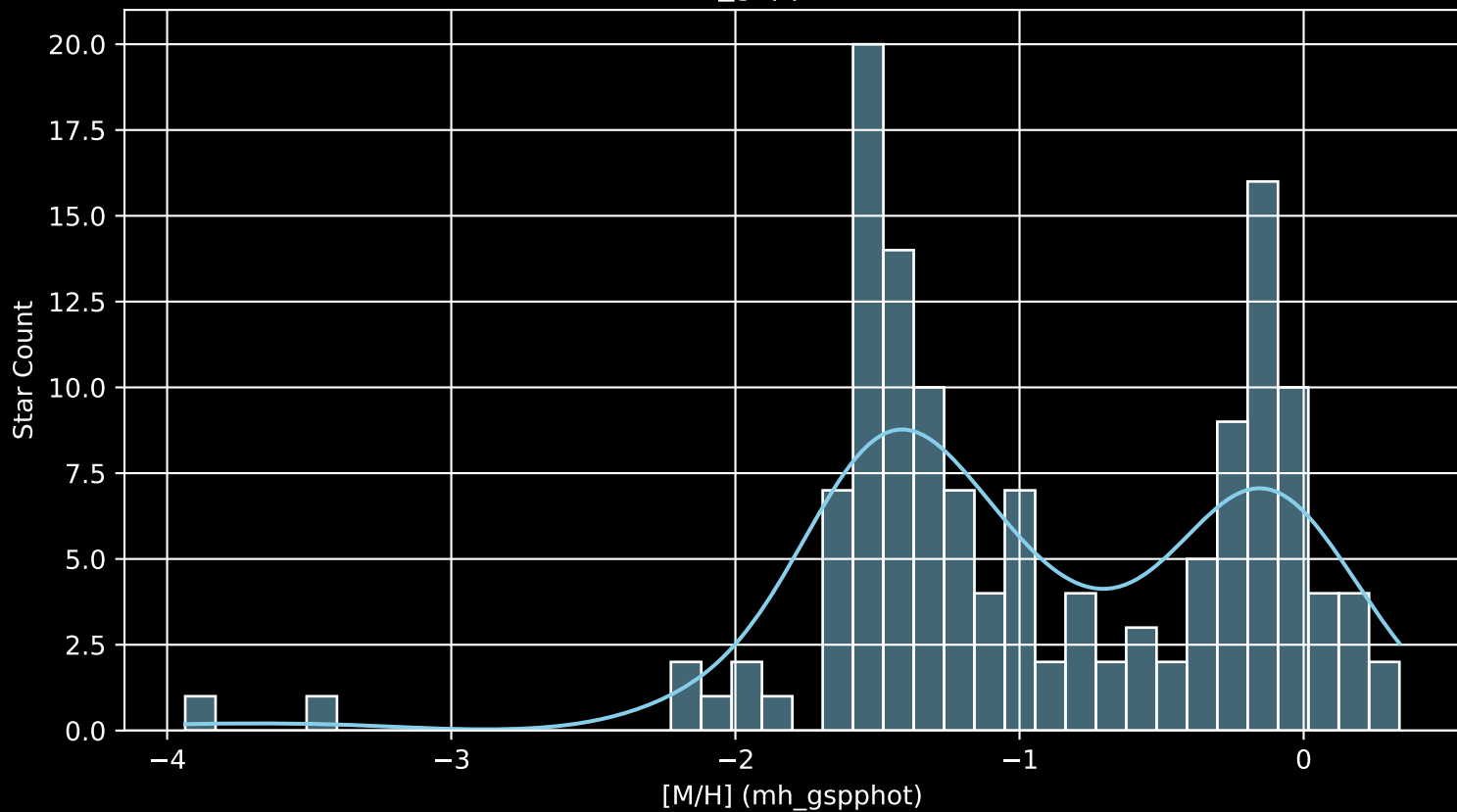
Gaia Cluster: [Berkeley_9 [M/H] (mh_gspphot) (n= 140)
