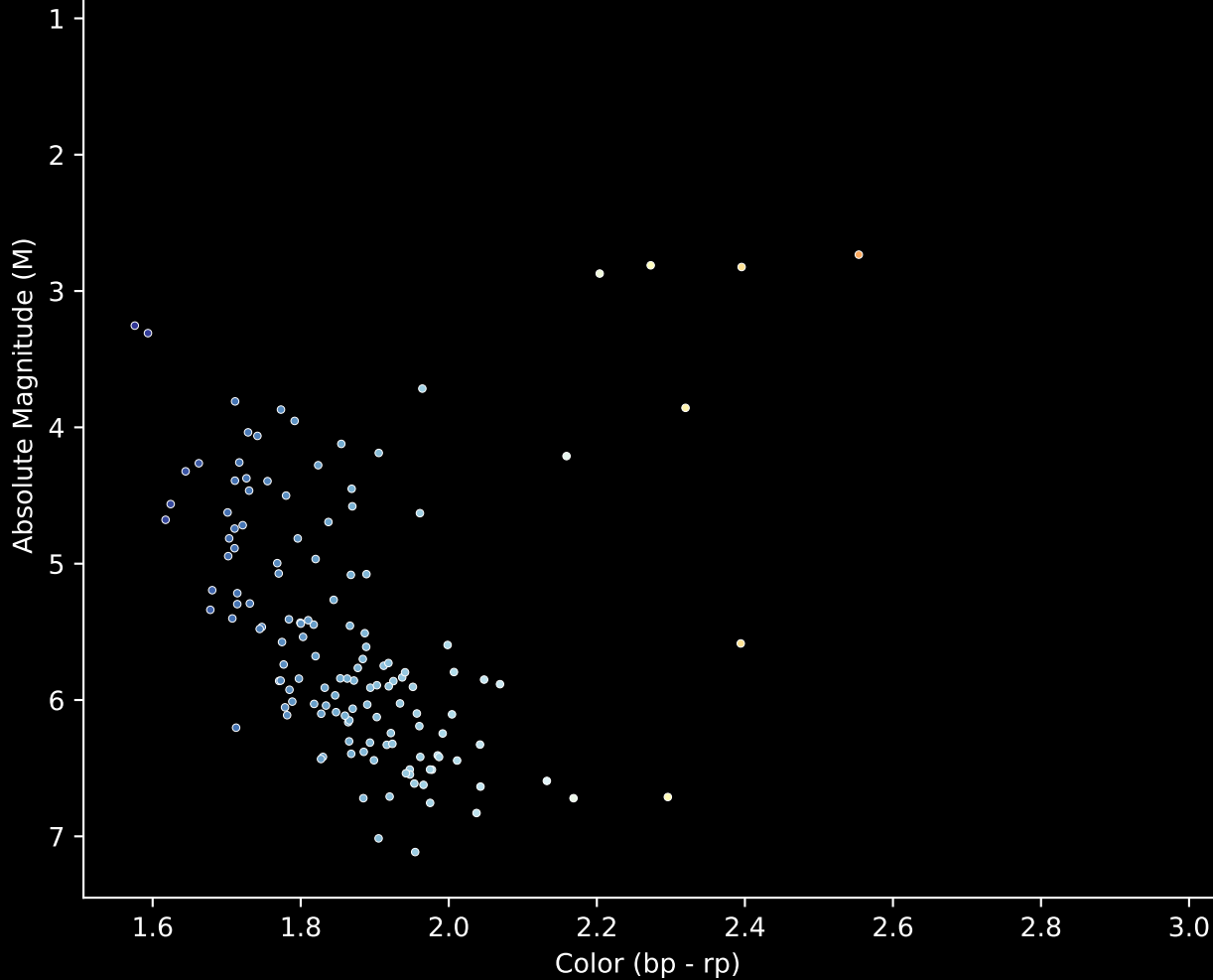
Gaia Cluster: [Berkeley_9] Stars (n= 141) Hertzsprung-Russel Diagram
