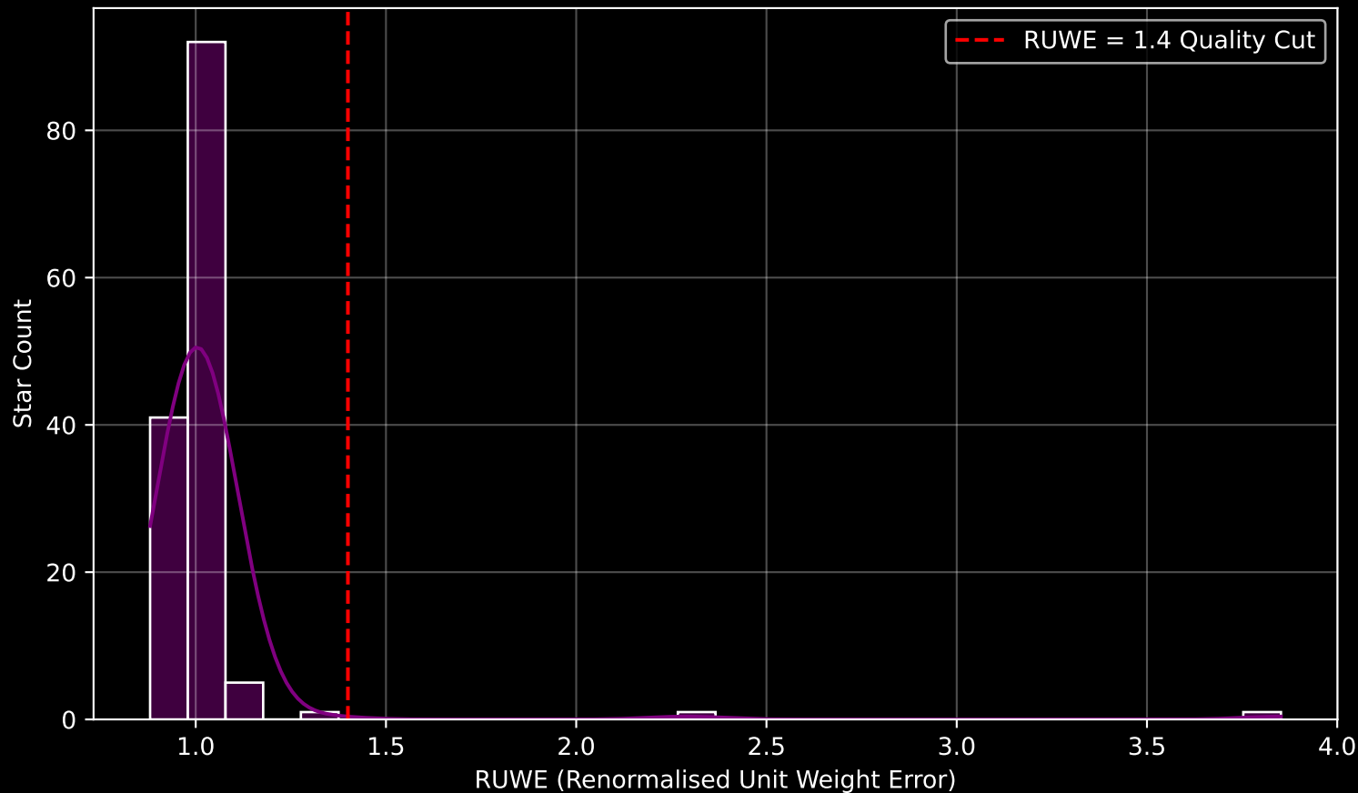
Gaia Cluster: [Berkeley_9] RUWE Distribution (n= 141)
