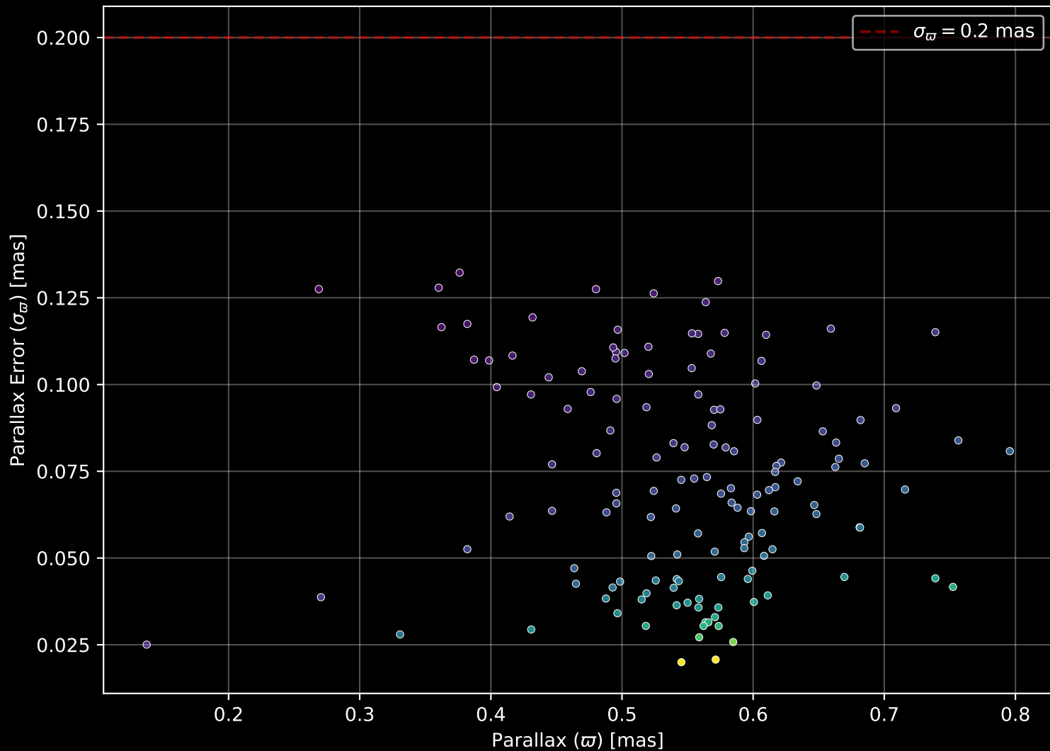
Gaia Cluster: [Berkeley_9] Parallax Quality (n= 141)
