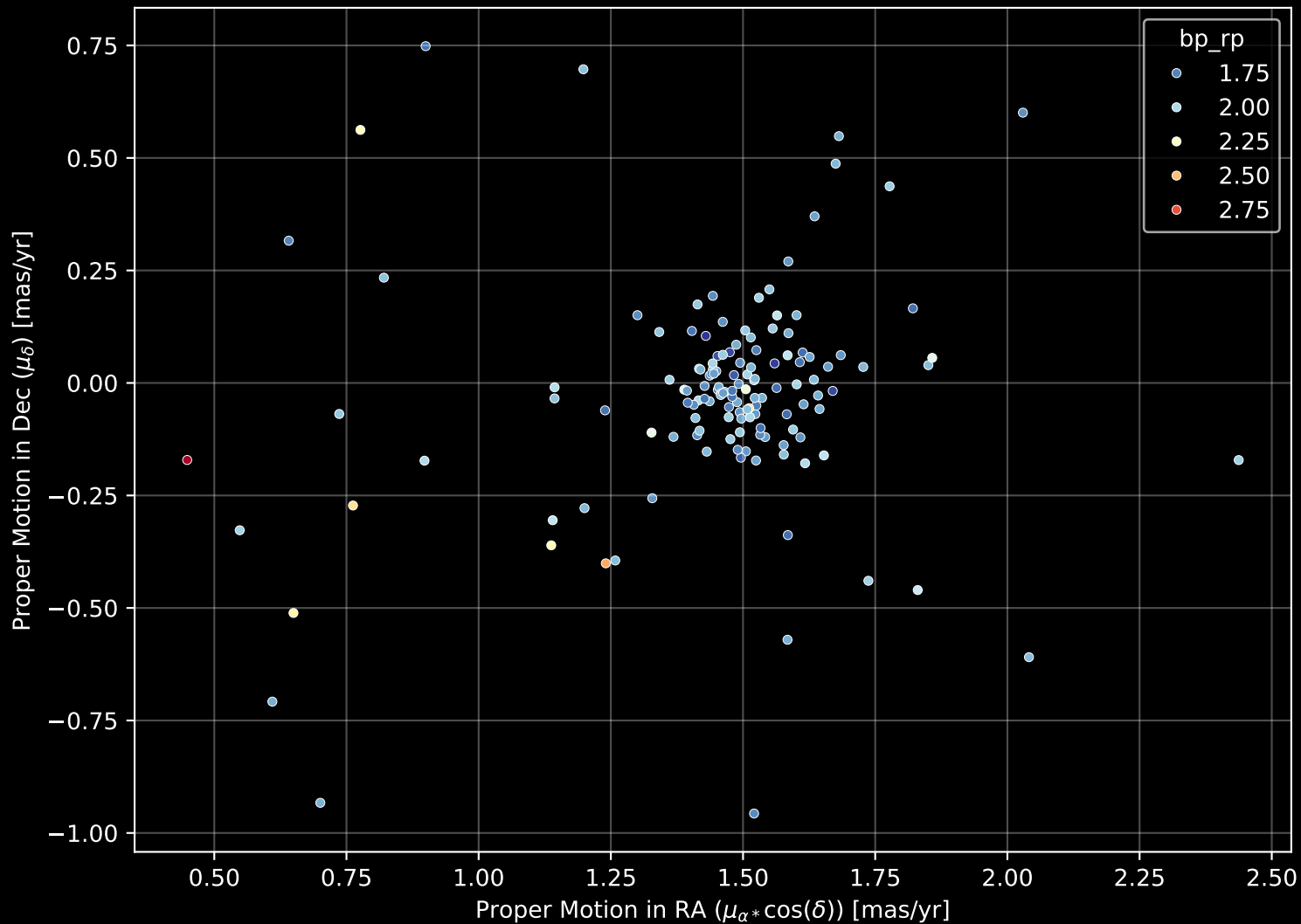
Gaia Cluster: [Berkeley_9] Proper Motion Diagram (n= 141)
