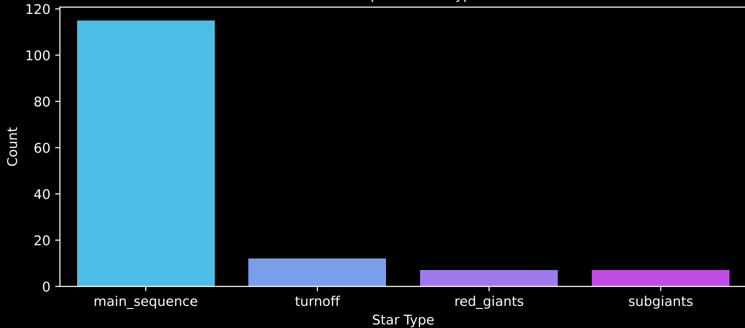
Gaia Cluster: [Berkeley_9] Count plot of Star Type
