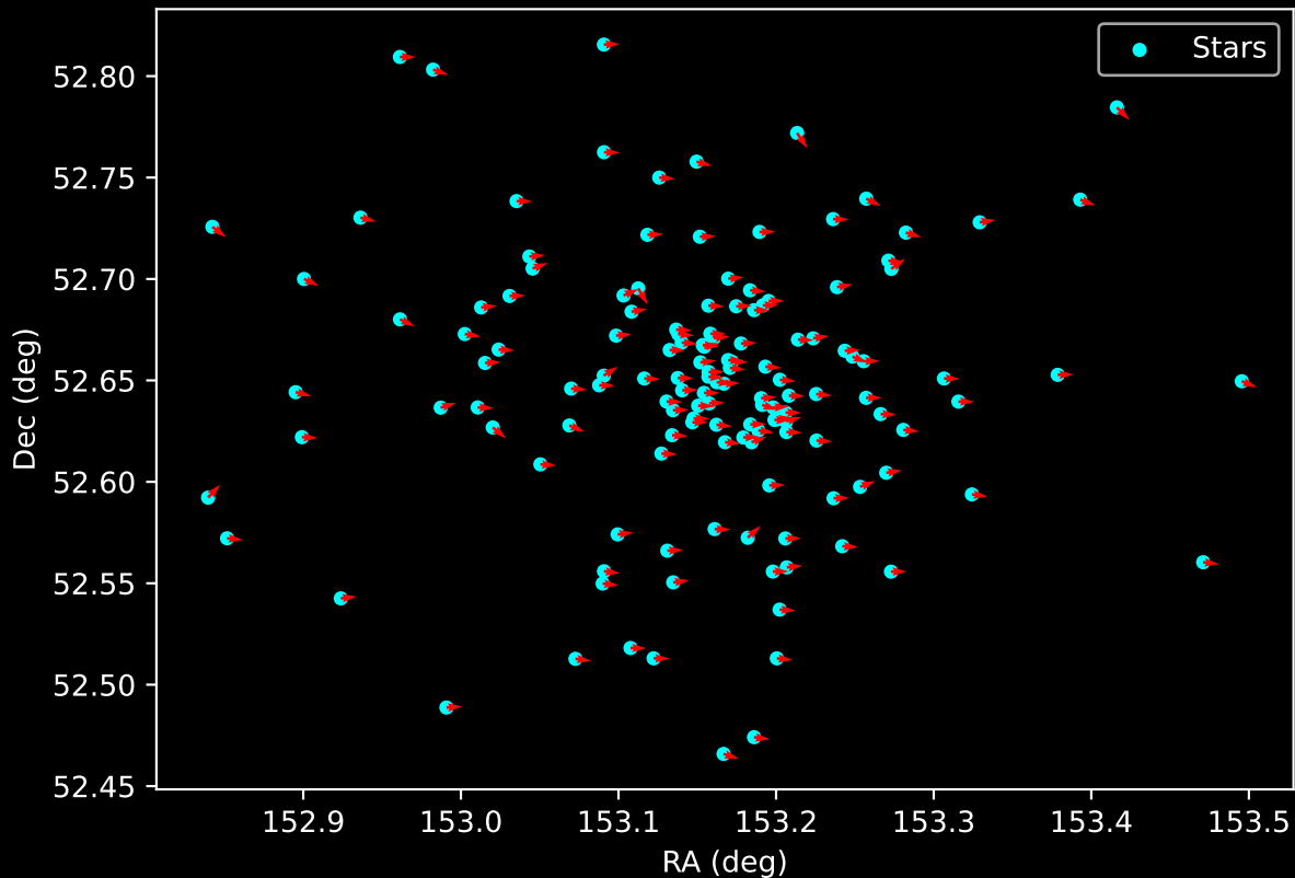
Gaia Cluster: [Berkeley_9] Proper Motion Vectors for Gaia Star Field (n= 141)
