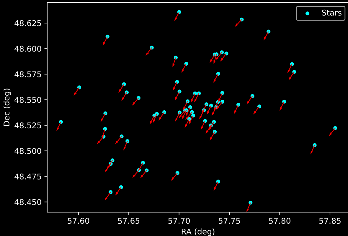
Gaia Cluster: [Berkeley_91] Proper Motion Vectors for Gaia Star Field (n= 66)
