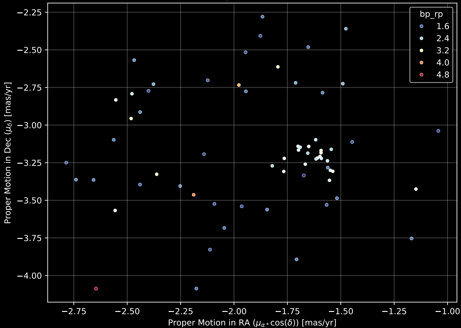
Gaia Cluster: [Berkeley_91] Proper Motion Diagram (n= 66)
