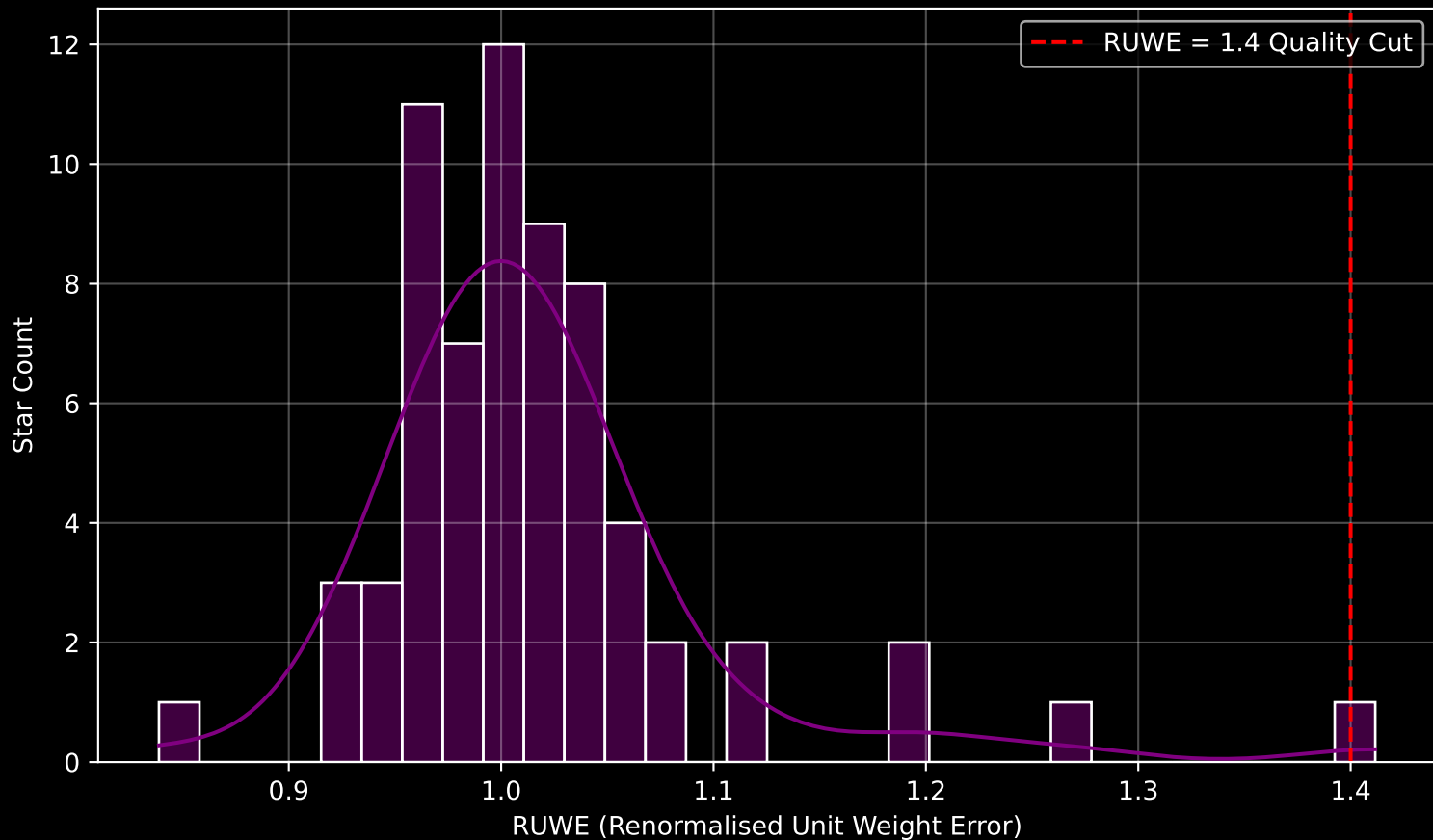
Gaia Cluster: [Berkeley_91] RUWE Distribution (n= 66)
