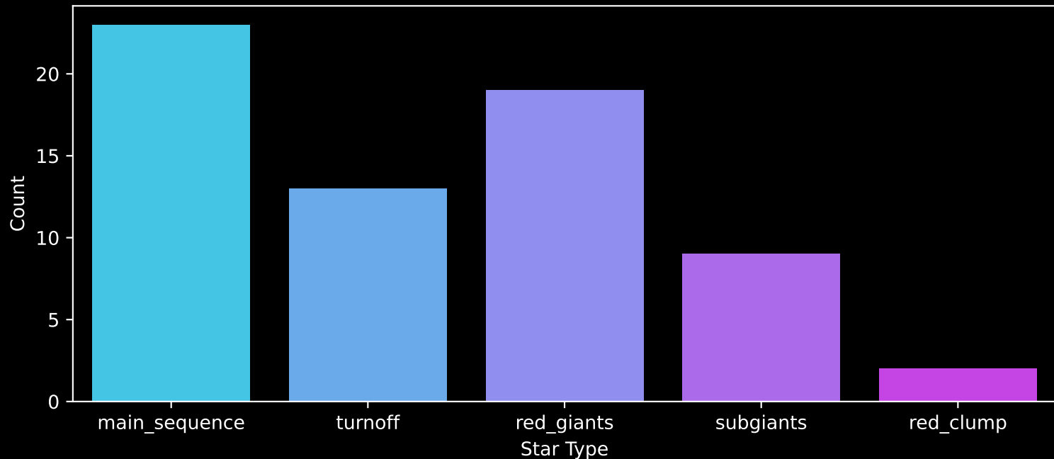
Gaia Cluster: [Berkeley_91] Count plot of Star Type
