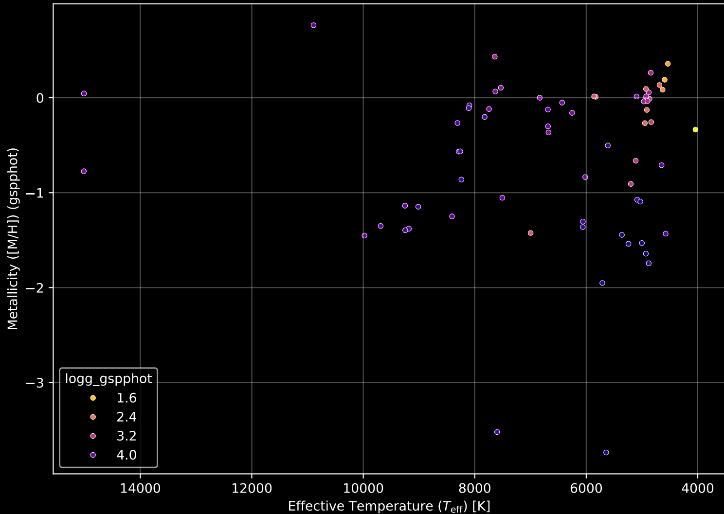
Gaia Cluster: [Berkeley_91] Stellar Population Parameters (n= 66)
