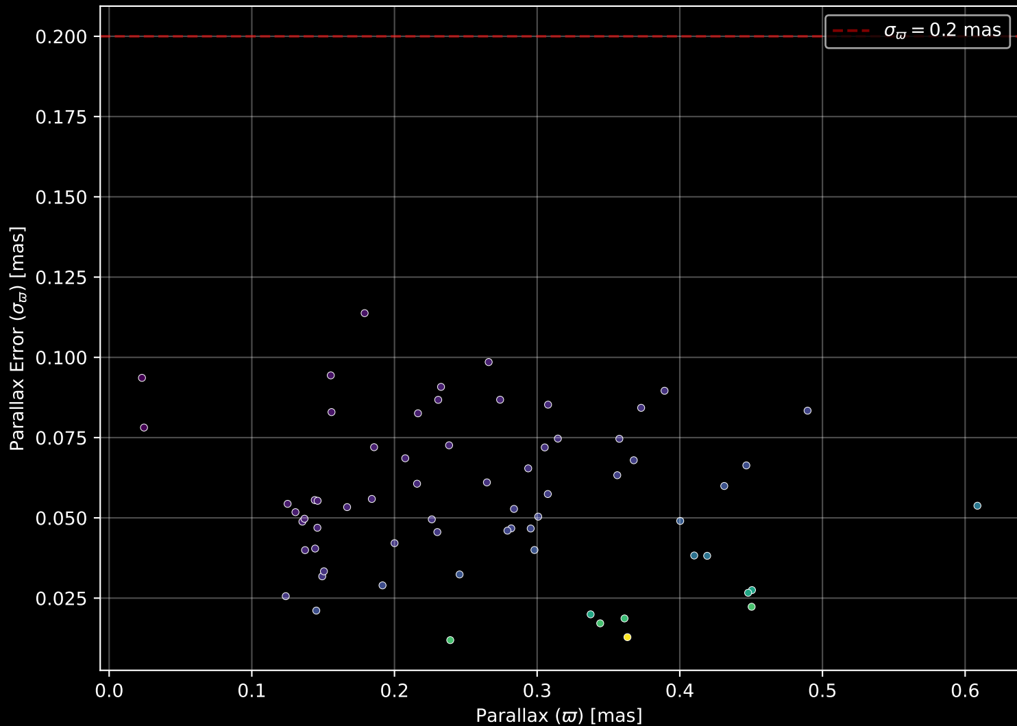
Gaia Cluster: [Berkeley_91] Parallax Quality (n= 66)
