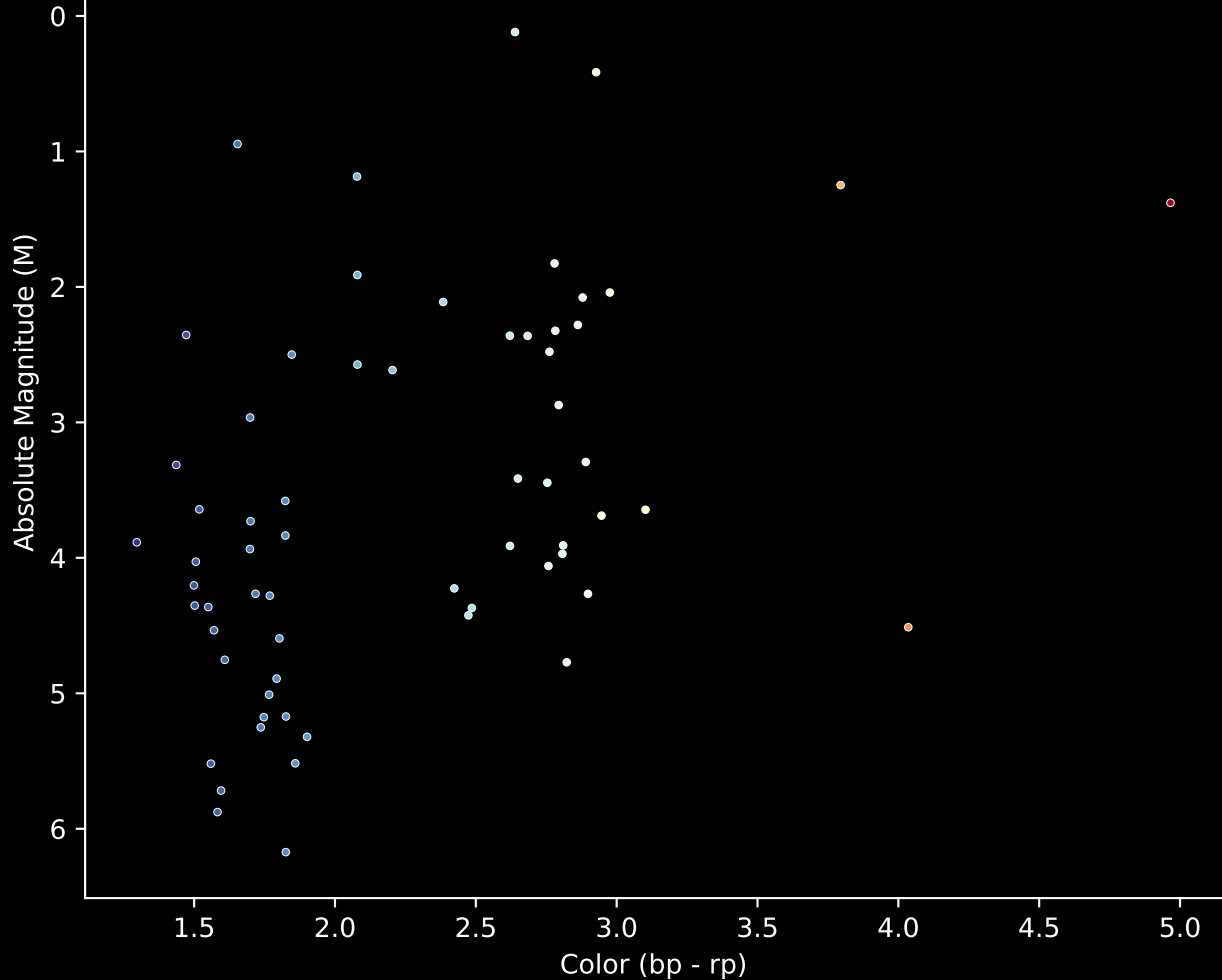
Gaia Cluster: [Berkeley_91] Stars (n=66) Hertzsprung-Russel Diagram
