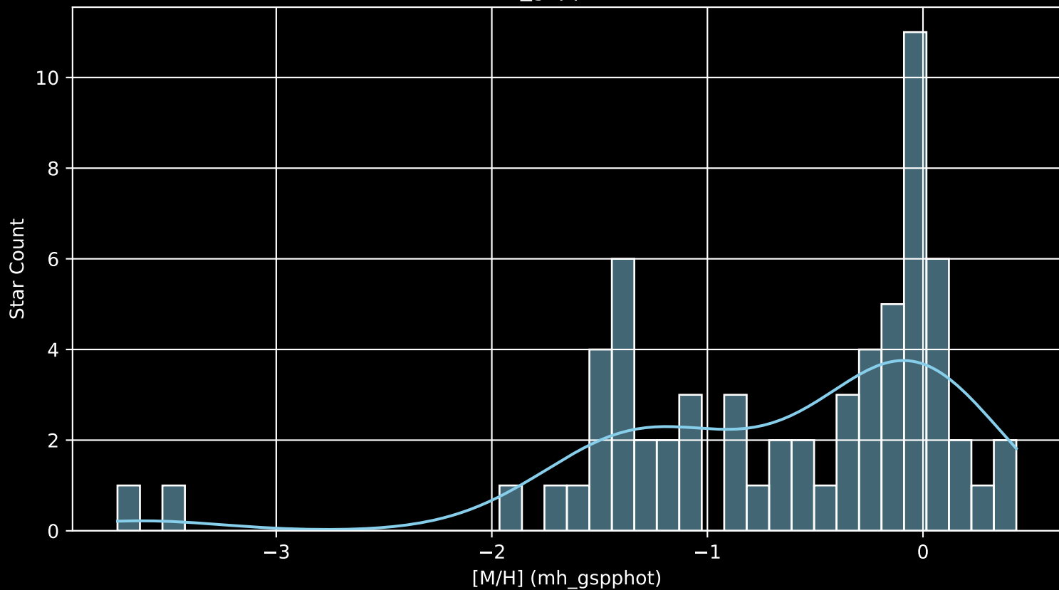
Gaia Cluster: [Berkeley_91 [M/H] (mh_gspphot) (n= 65)
