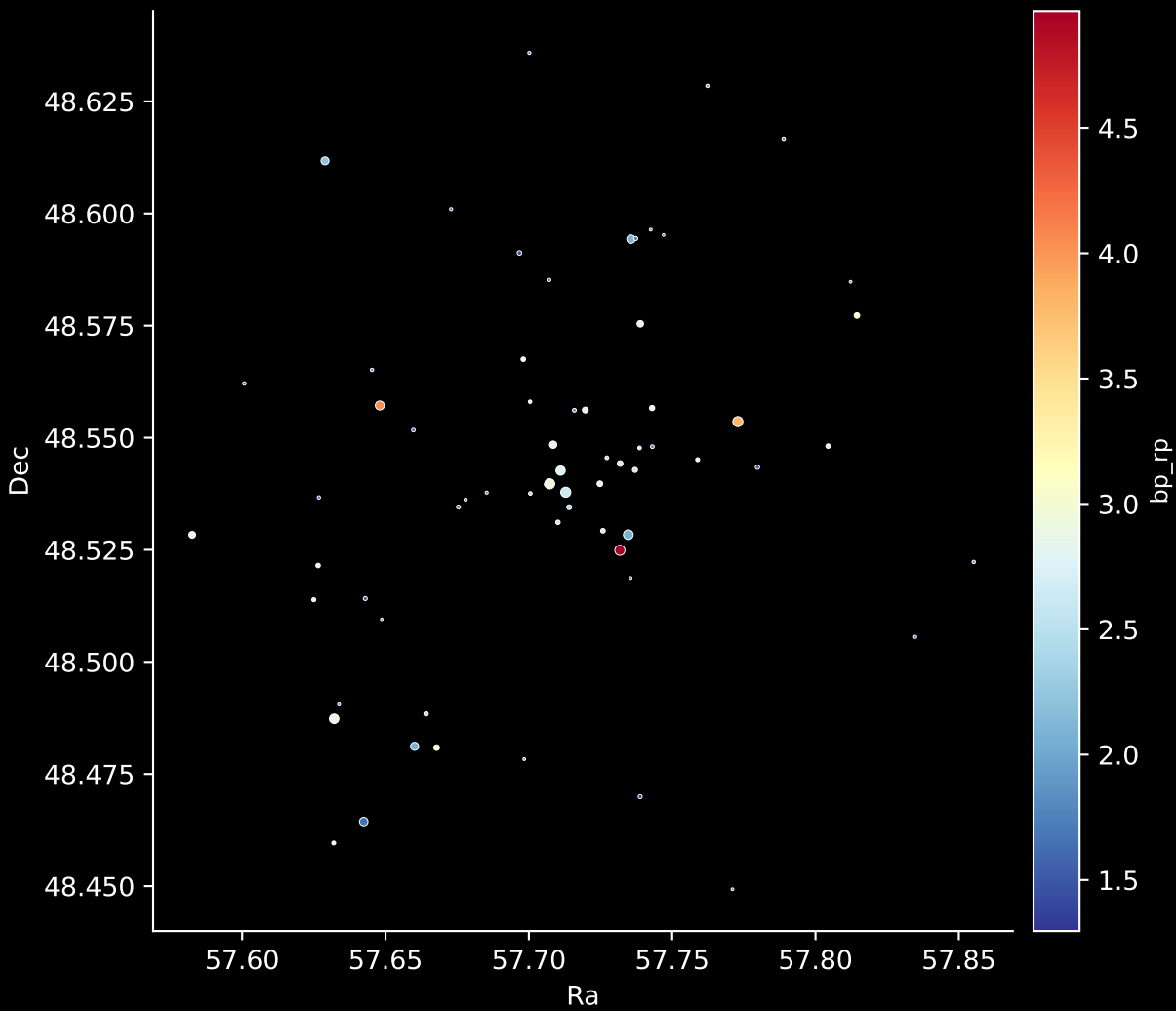
Gaia Cluster: [Berkeley_91] Stars: 66
