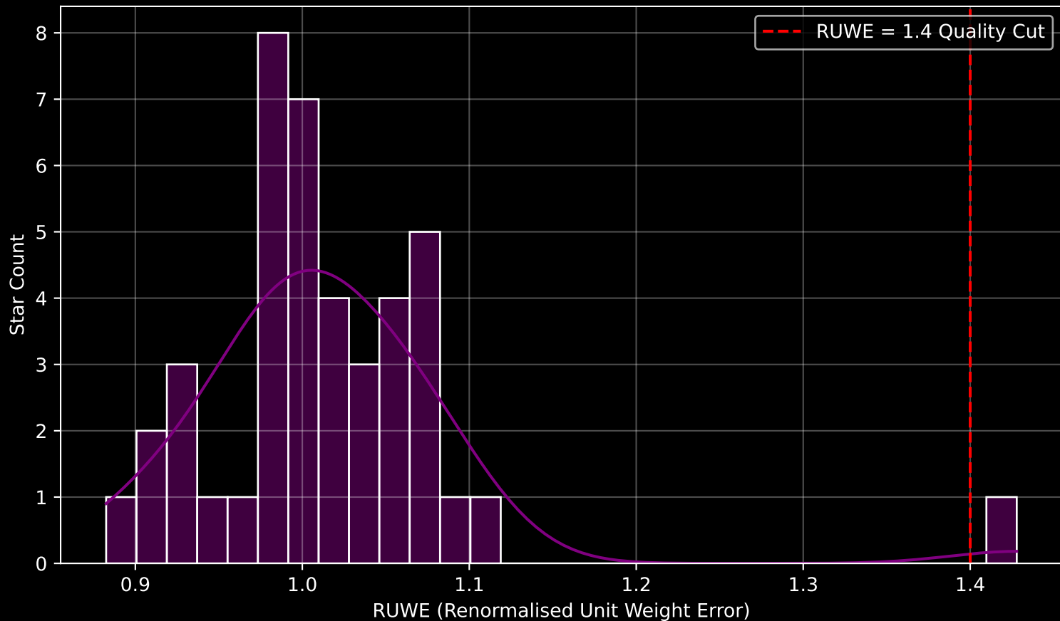
Gaia Cluster: [Berkeley_92] RUWE Distribution (n= 42)
