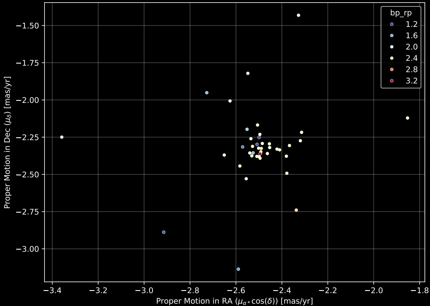
Gaia Cluster: [Berkeley_92] Proper Motion Diagram (n= 42)
