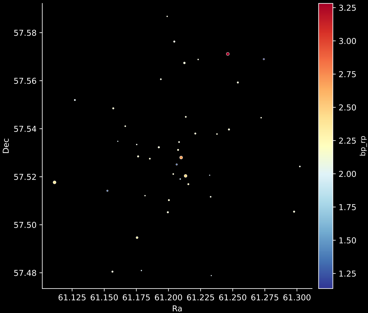
Gaia Cluster: [Berkeley_92] Stars: 42
