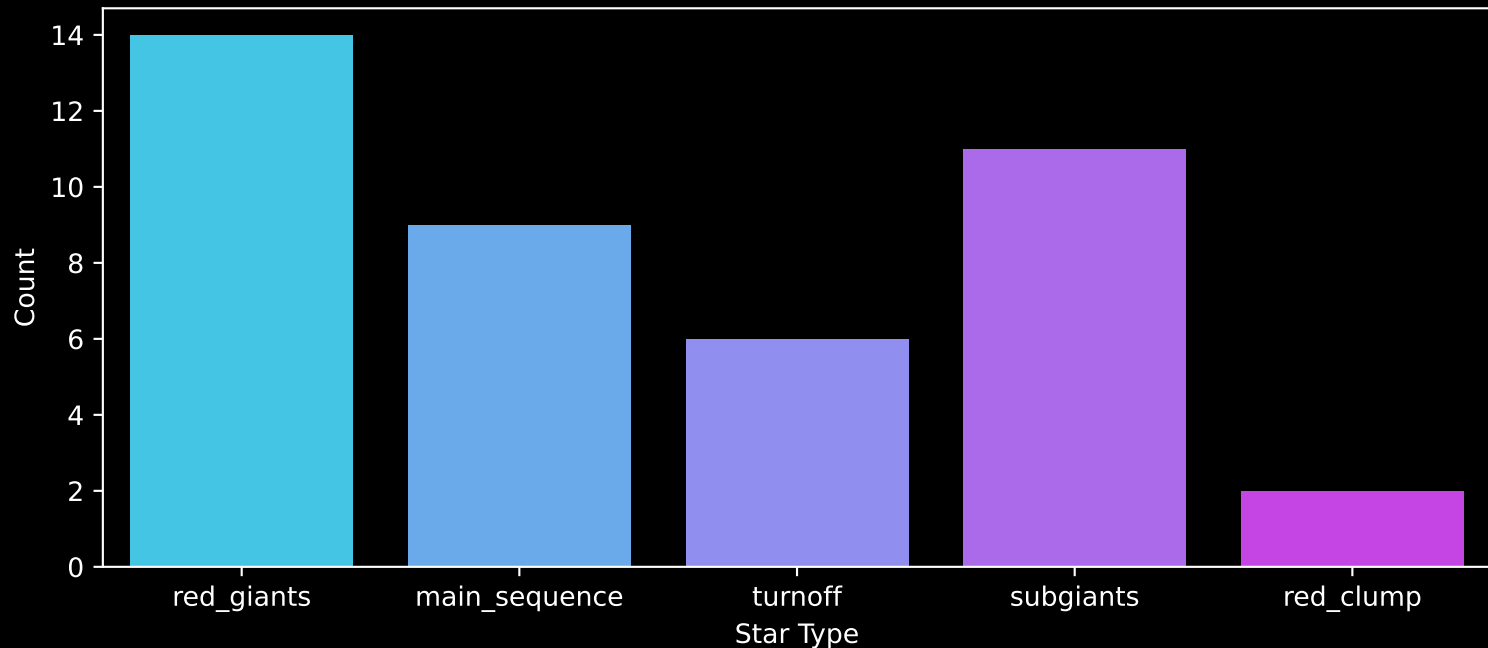
Gaia Cluster: [Berkeley_92] Count plot of Star Type
