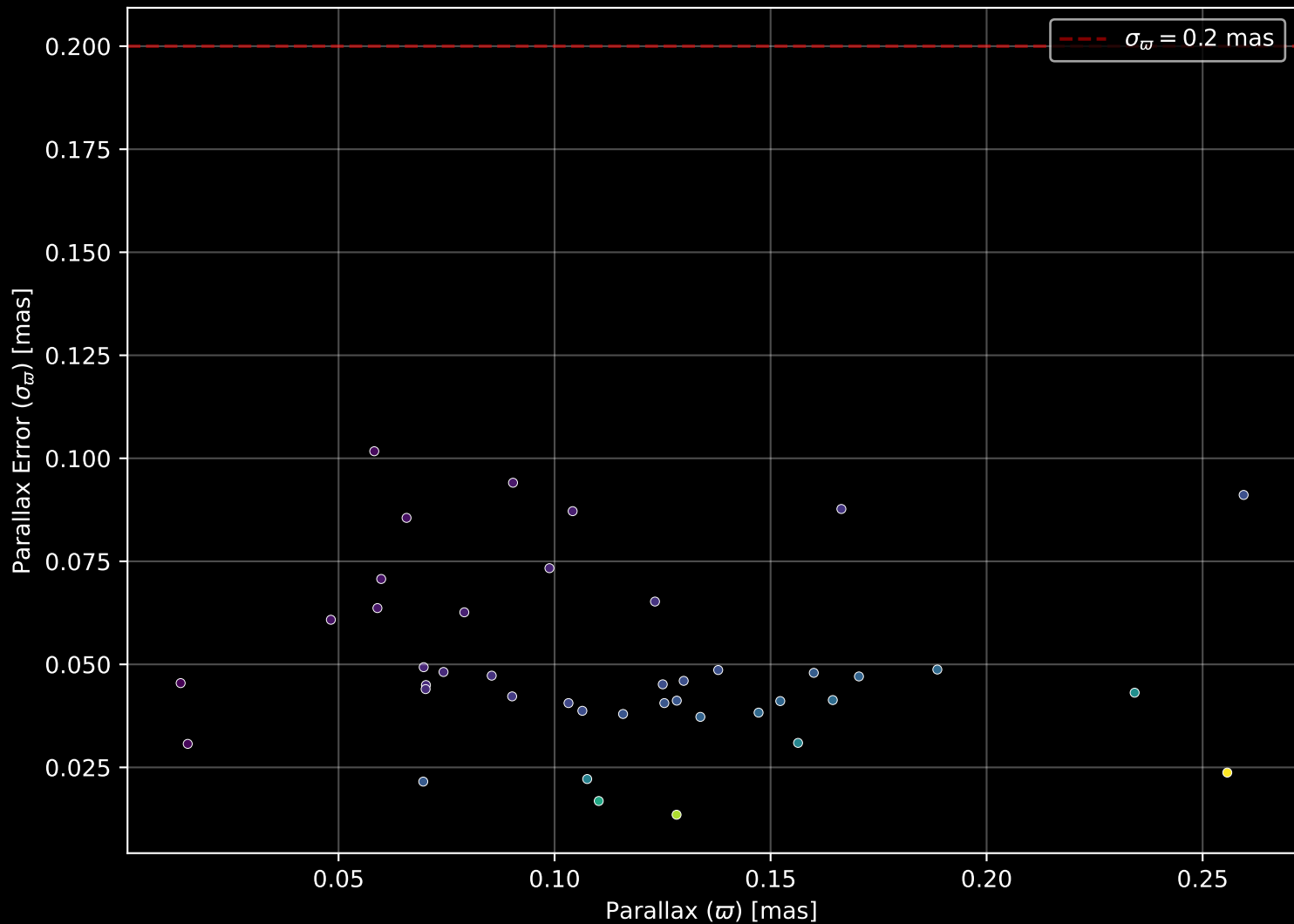
Gaia Cluster: [Berkeley_92] Parallax Quality (n= 42)
