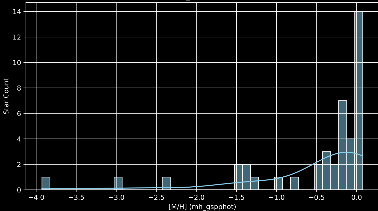
Gaia Cluster: [Berkeley_92 [M/H] (mh_gspphot) (n= 42)
