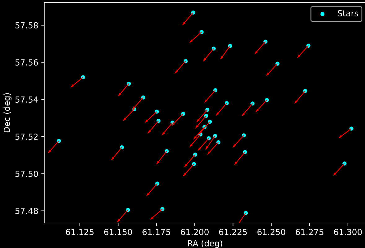
Gaia Cluster: [Berkeley_92] Proper Motion Vectors for Gaia Star Field (n= 42)
