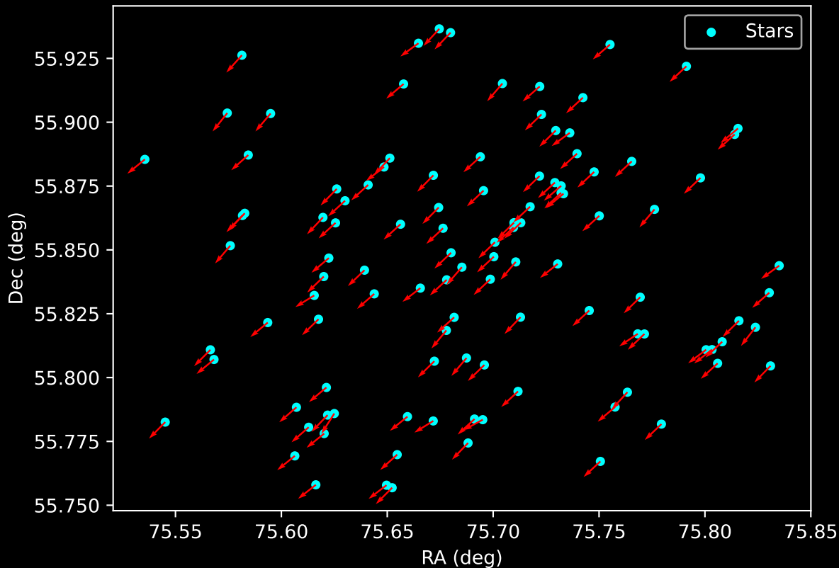
Gaia Cluster: [Berkeley_94] Proper Motion Vectors for Gaia Star Field (n= 109)
