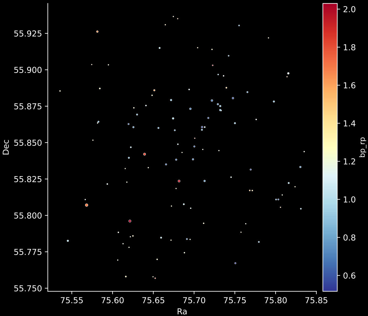
Gaia Cluster: [Berkeley_94] Stars: 109
