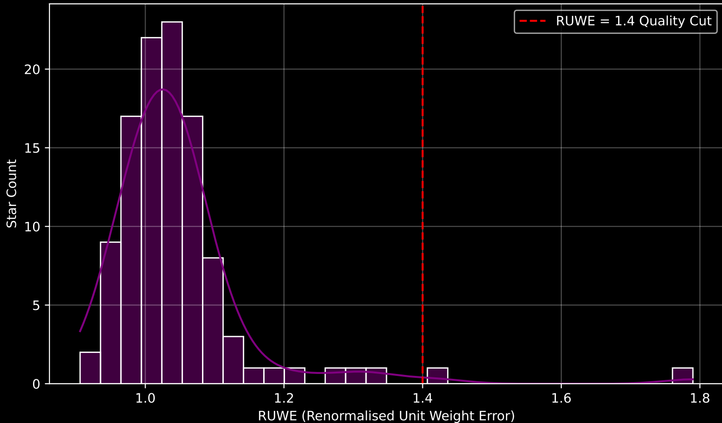
Gaia Cluster: [Berkeley_94] RUWE Distribution (n= 109)
