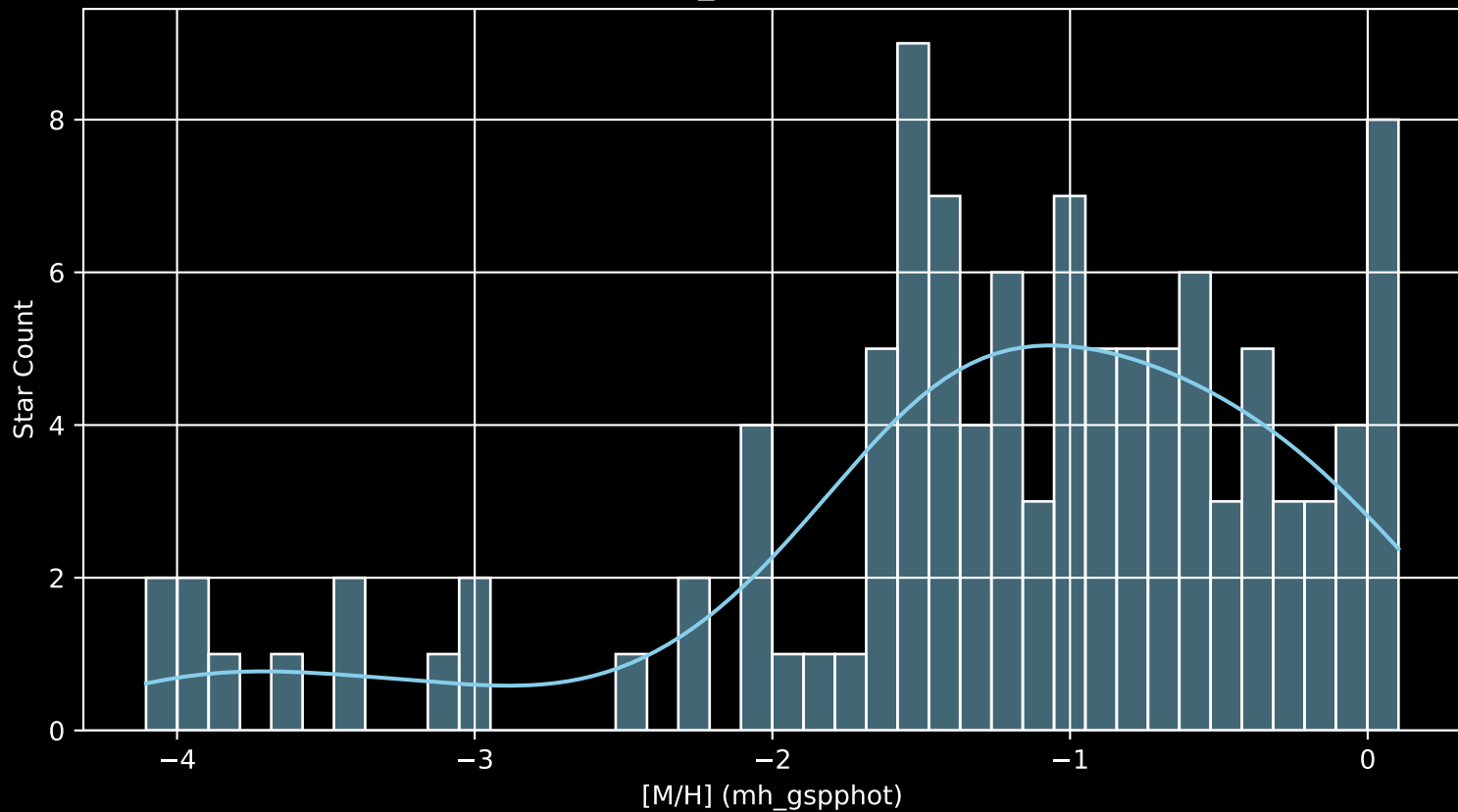
Gaia Cluster: [Berkeley_94 [M/H] (mh_gspphot) (n= 109)
