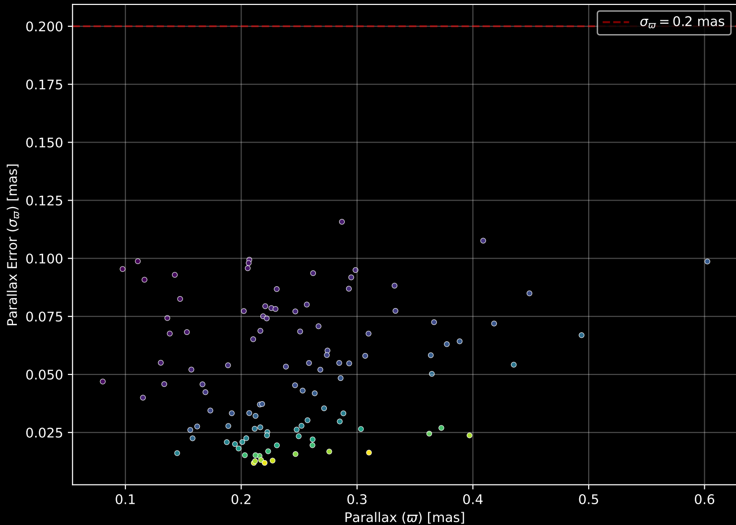
Gaia Cluster: [Berkeley_94] Parallax Quality (n= 109)
