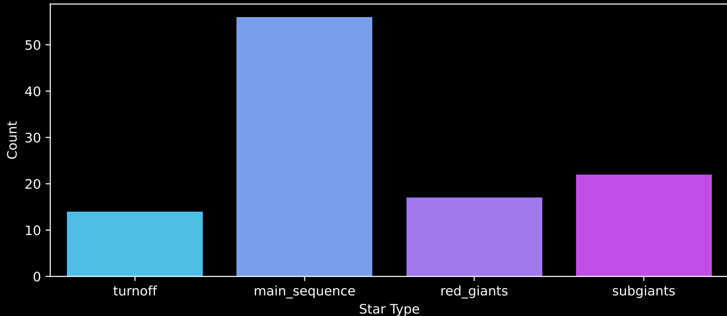
Gaia Cluster: [Berkeley_94] Count plot of Star Type
