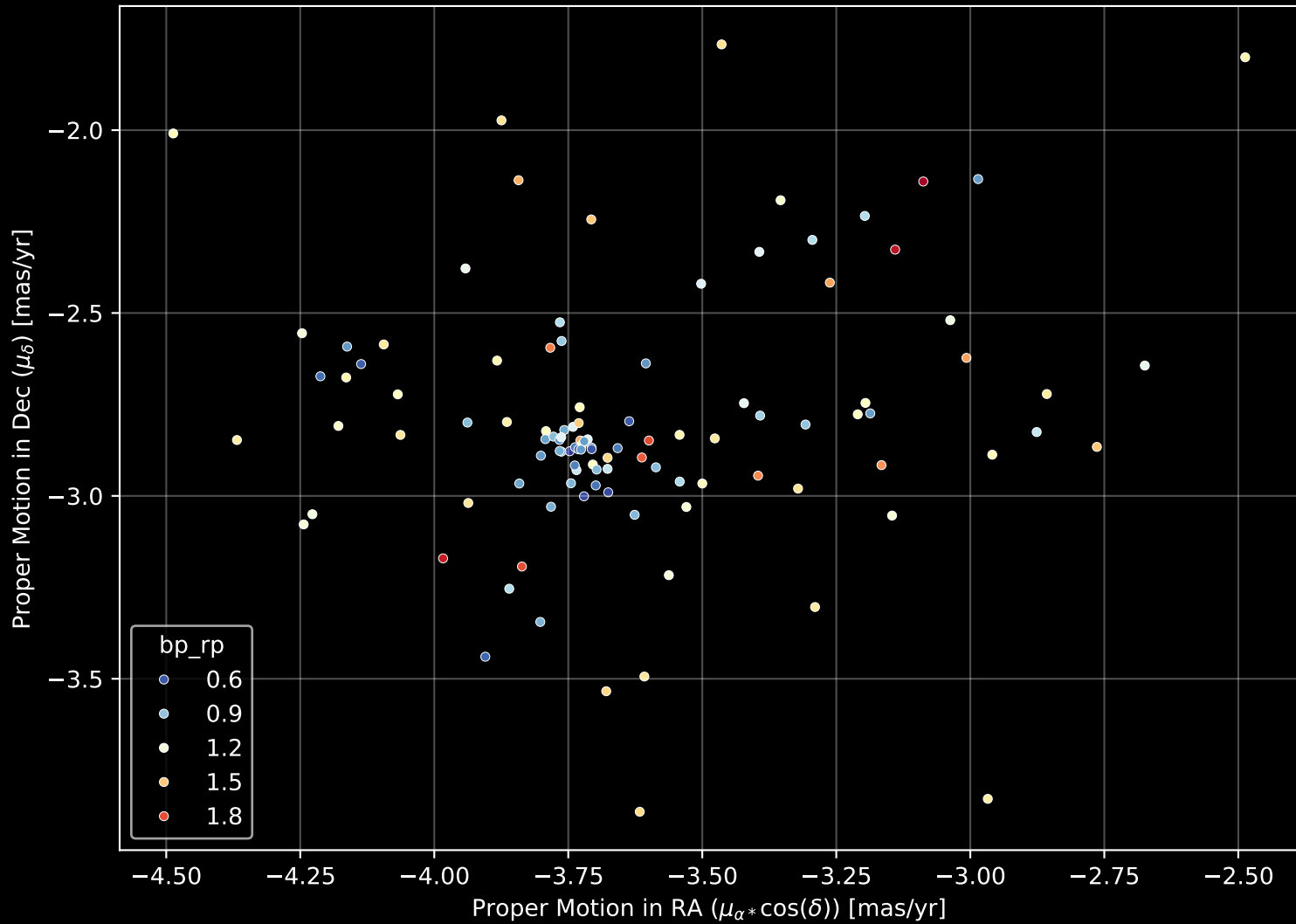
Gaia Cluster: [Berkeley_94] Proper Motion Diagram (n= 109)
