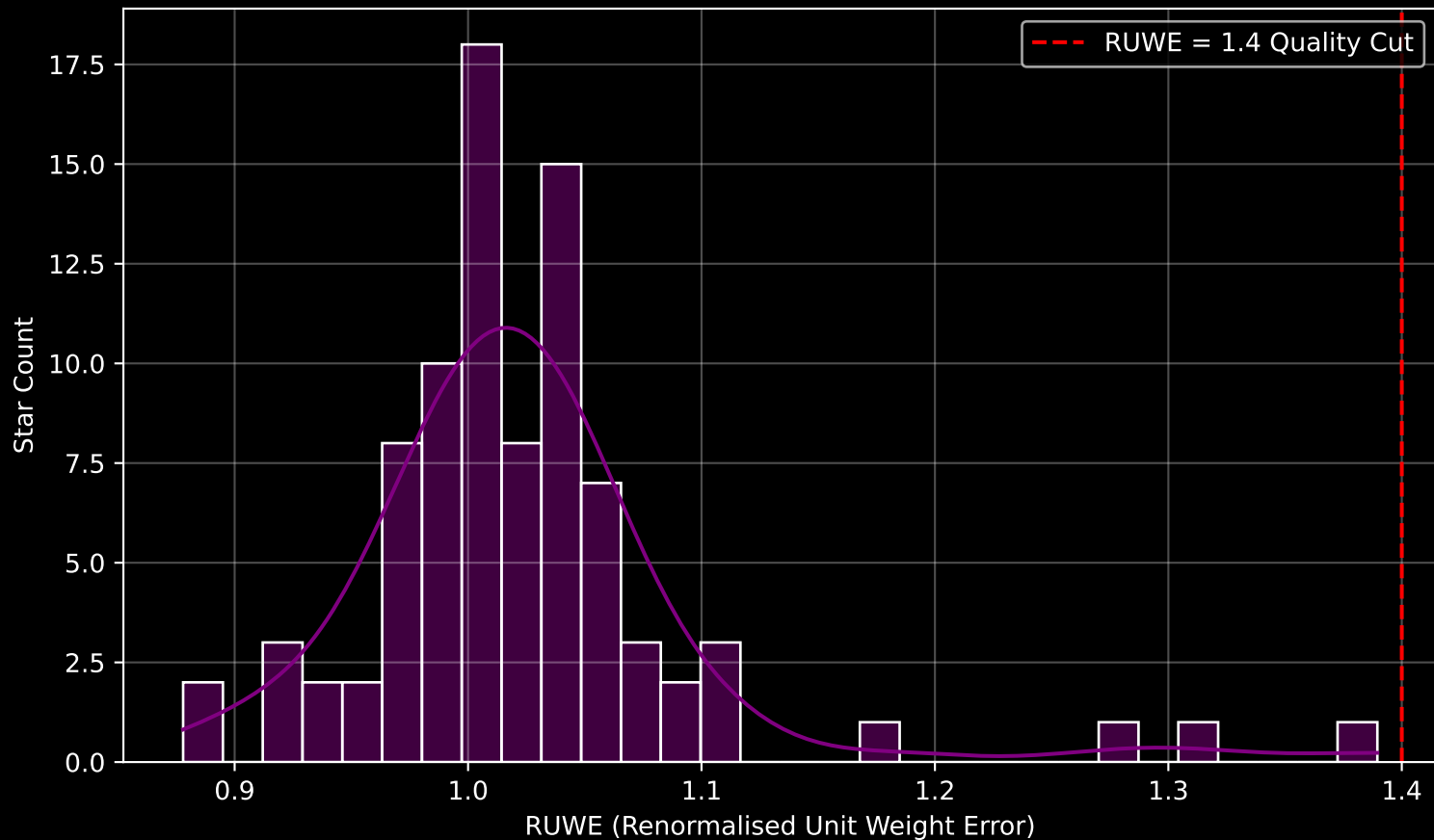
Gaia Cluster: [Berkeley_96] RUWE Distribution (n= 87)
