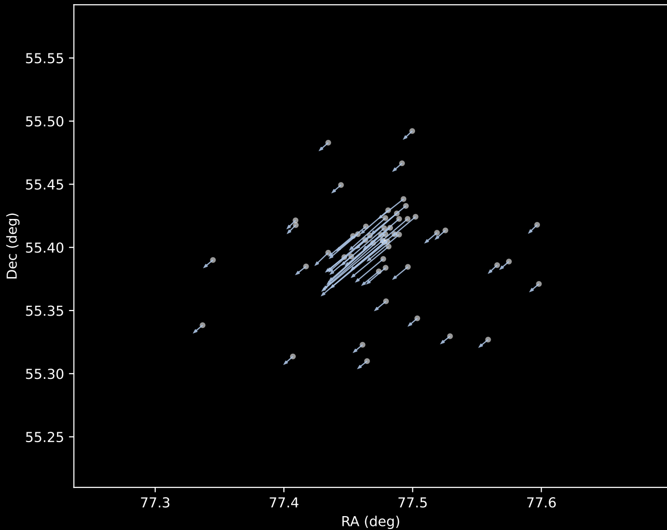
Gaia DR3 Cluster 1 Proper Motion Vectors (n=53)
