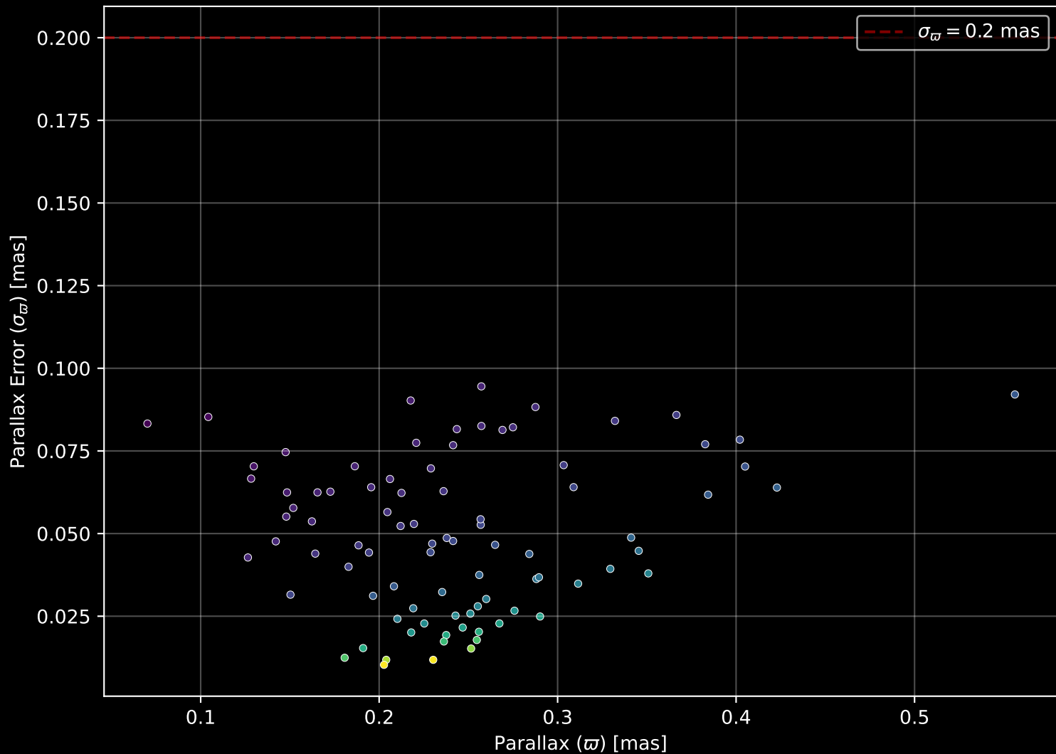
Gaia Cluster: [Berkeley_96] Parallax Quality (n= 87)
