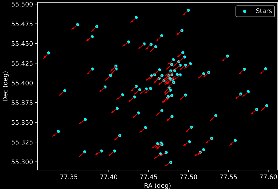
Gaia Cluster: [Berkeley_96] Proper Motion Vectors for Gaia Star Field (n= 87)
