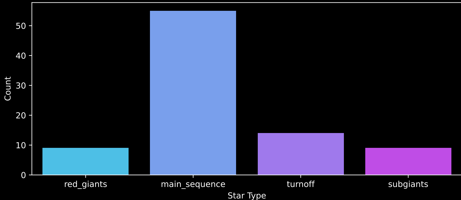
Gaia Cluster: [Berkeley_96] Count plot of Star Type
