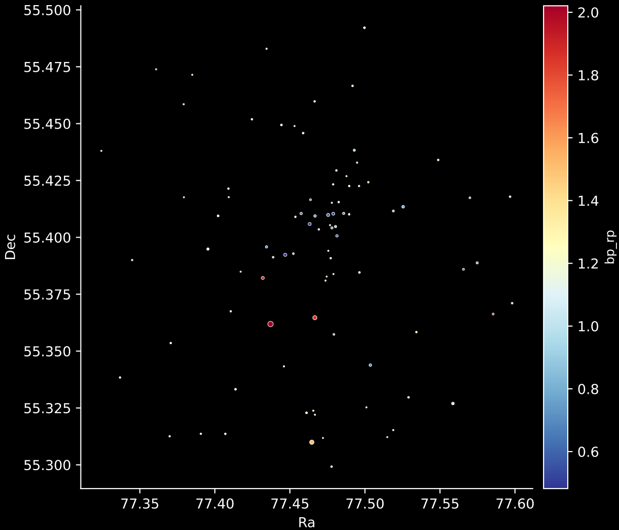
Gaia Cluster: [Berkeley_96] Stars: 87
