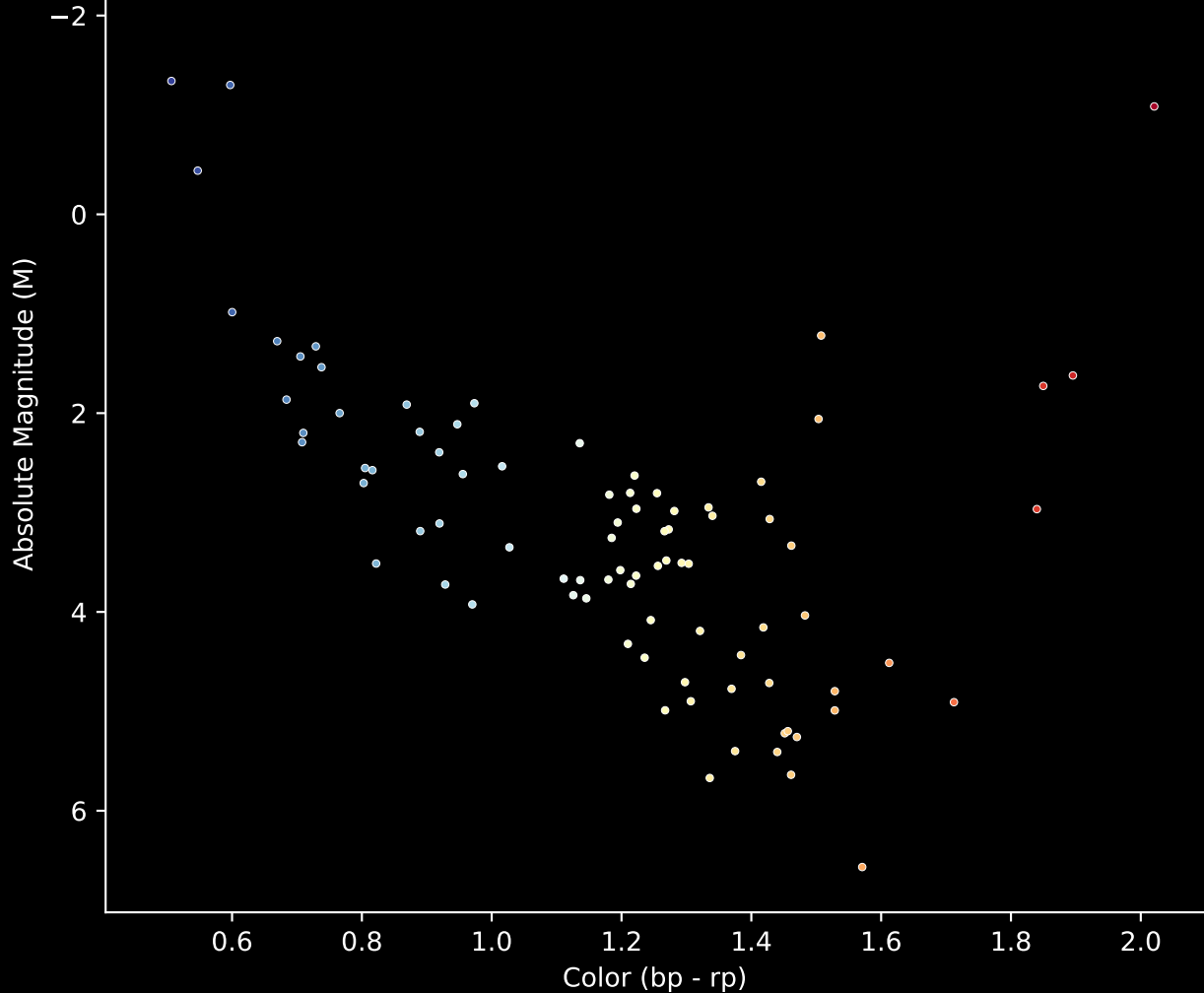
Gaia Cluster: [Berkeley_96] Stars (n= 87) Hertzsprung-Russel Diagram
