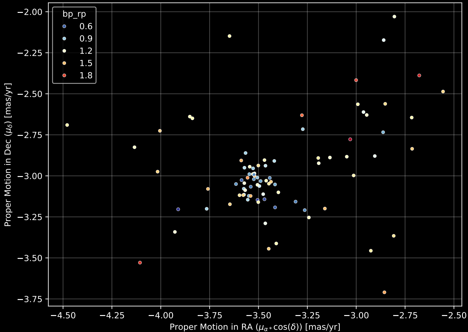
Gaia Cluster: [Berkeley_96] Proper Motion Diagram (n= 87)
