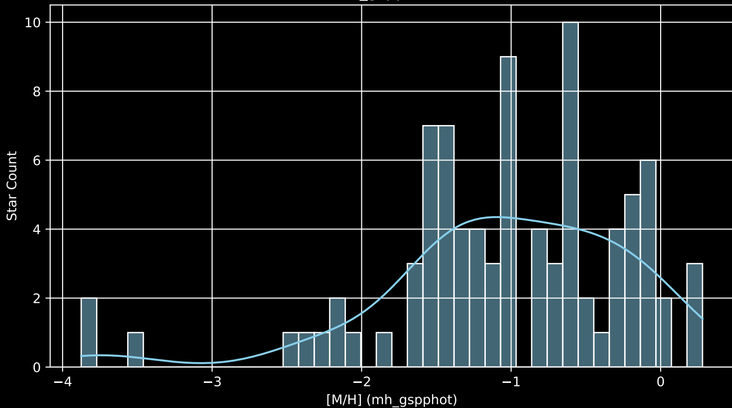
Gaia Cluster: [Berkeley_96 [M/H] (mh_gspphot) (n= 87)
