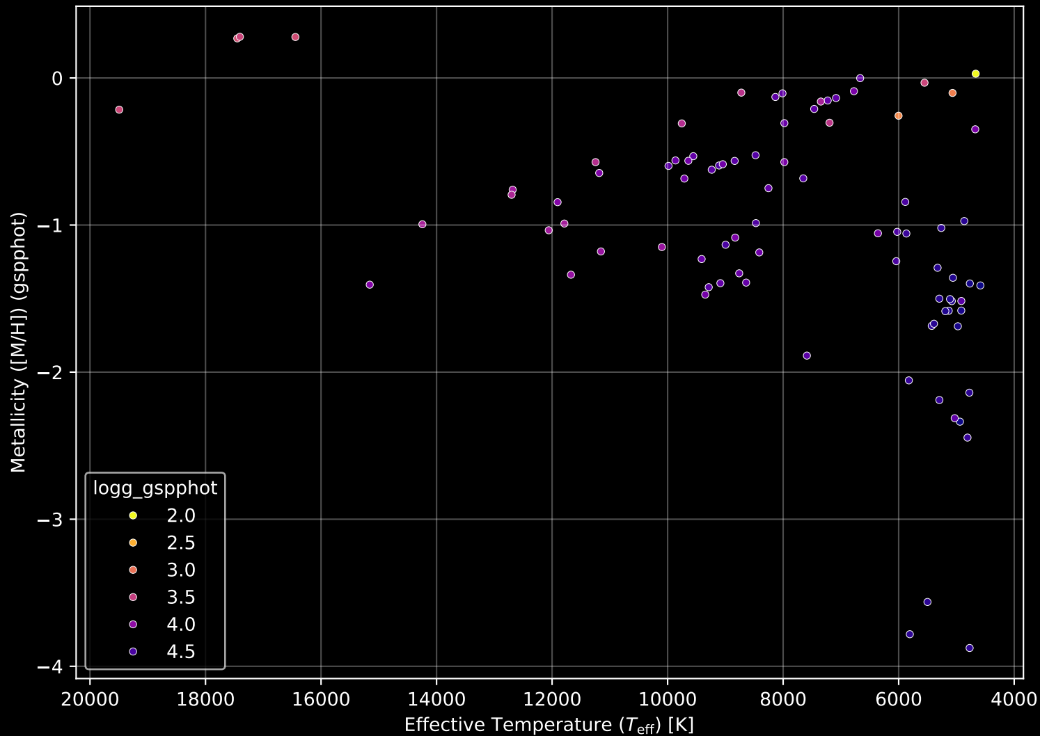
Gaia Cluster: [Berkeley_96] Stellar Population Parameters (n= 87)
