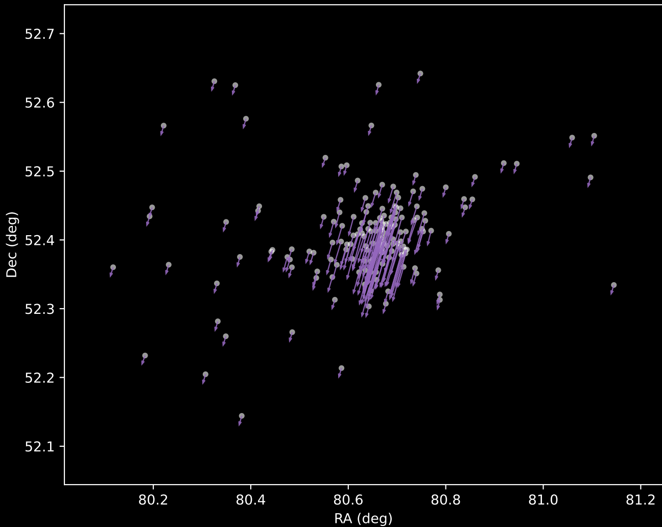
Gaia DR3 Cluster 8 Proper Motion Vectors (n=166)
