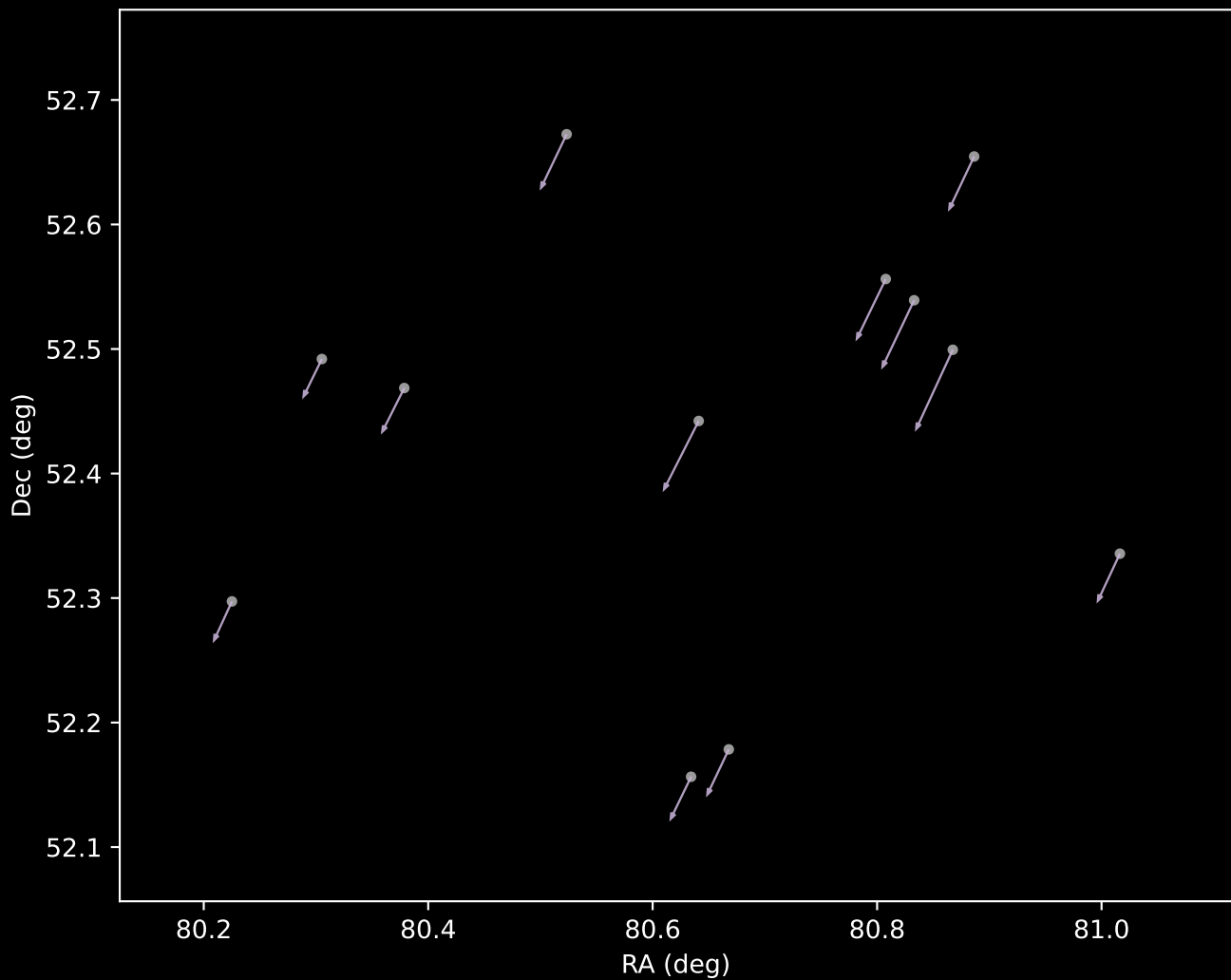
Gaia DR3 Cluster 9 Proper Motion Vectors (n=12)
