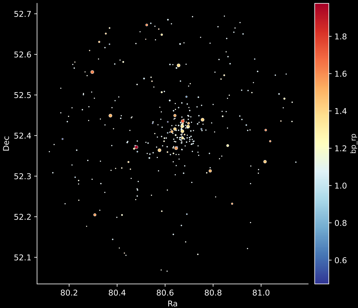
Gaia Cluster: [Berkeley_98] Stars: 328
