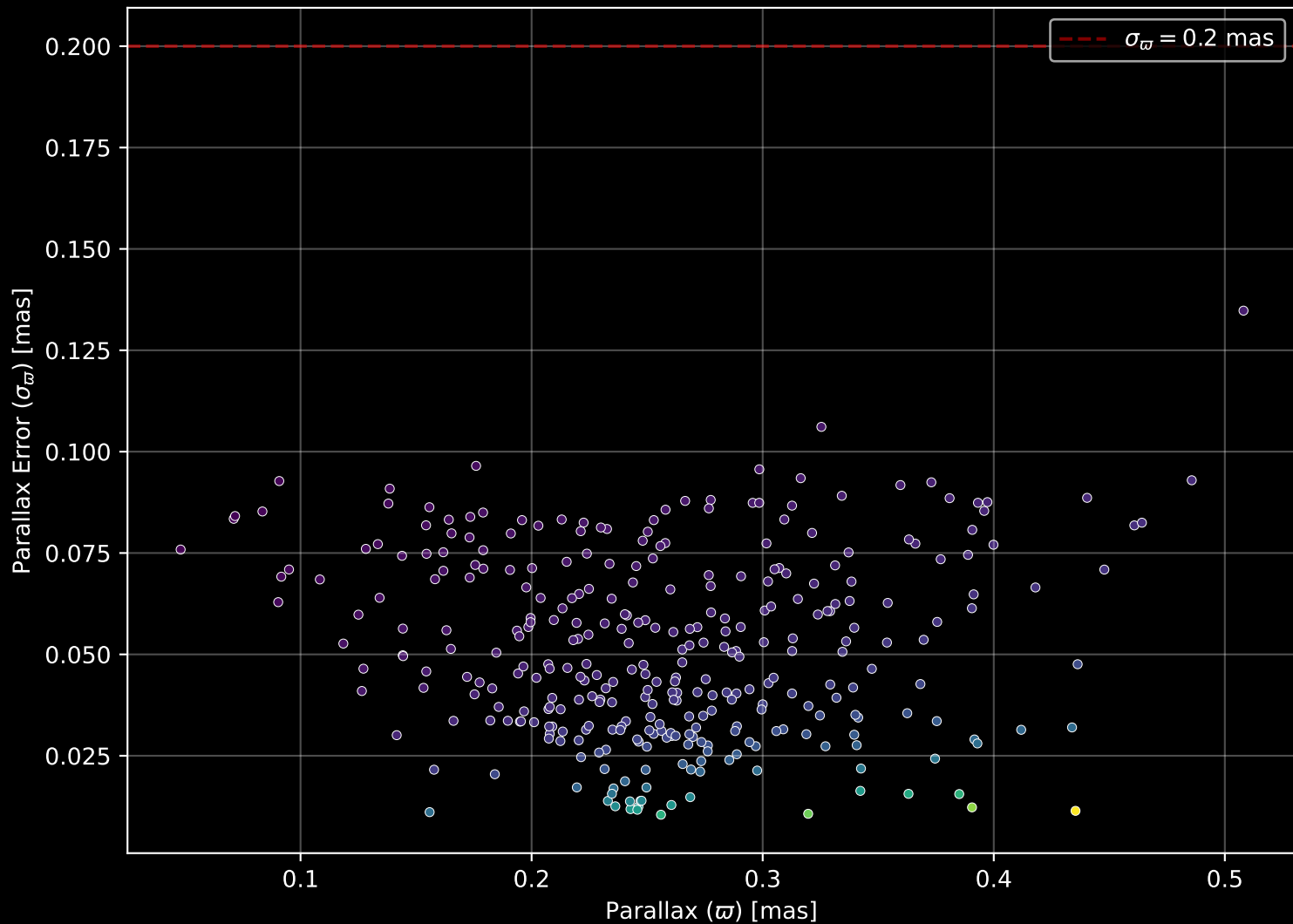
Gaia Cluster: [Berkeley_98] Parallax Quality (n= 328)
