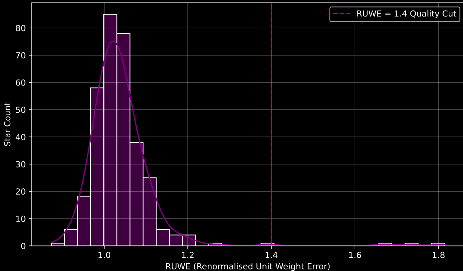
Gaia Cluster: [Berkeley_98] RUWE Distribution (n= 328)
