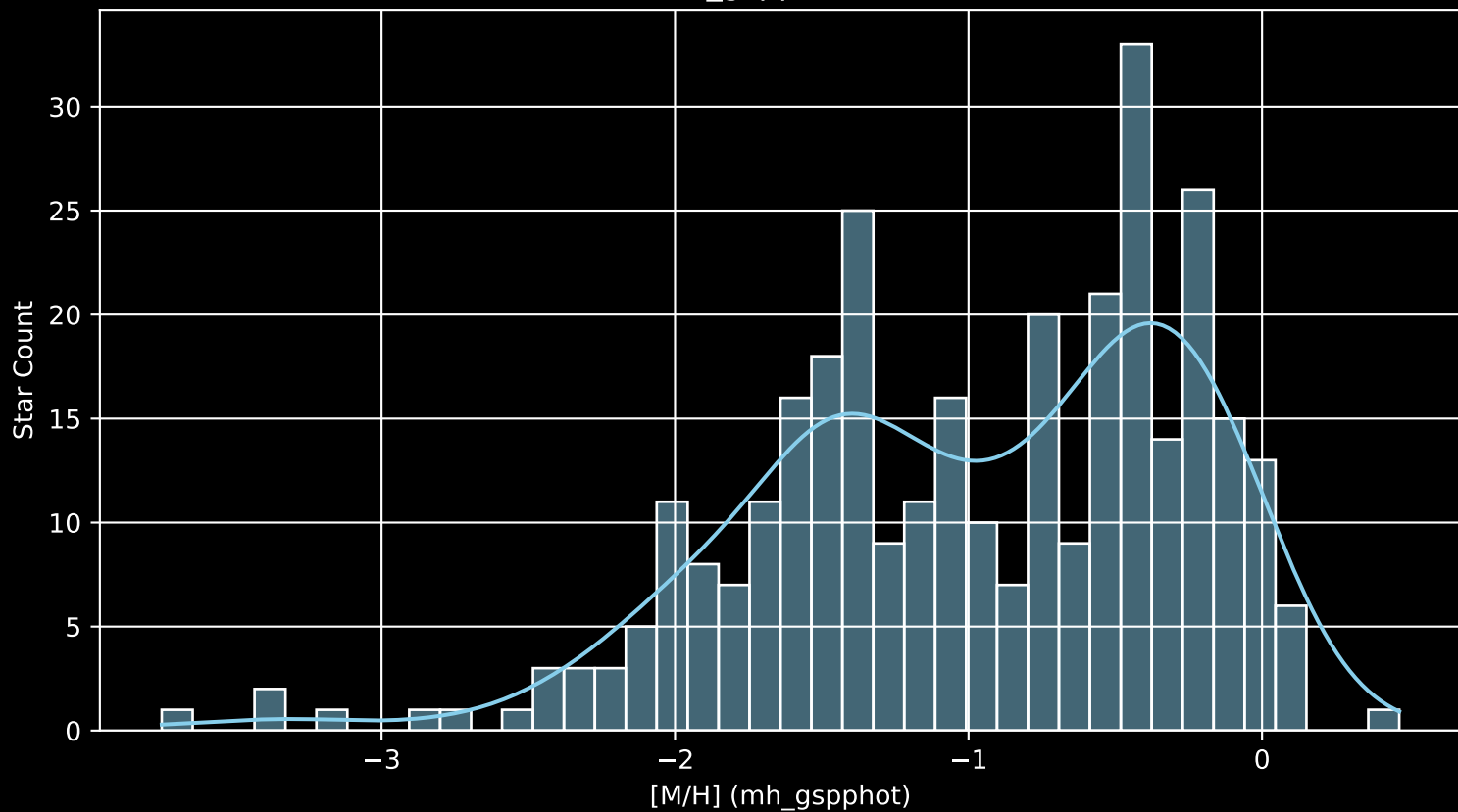
Gaia Cluster: [Berkeley_98 [M/H] (mh_gspphot) (n= 328)
