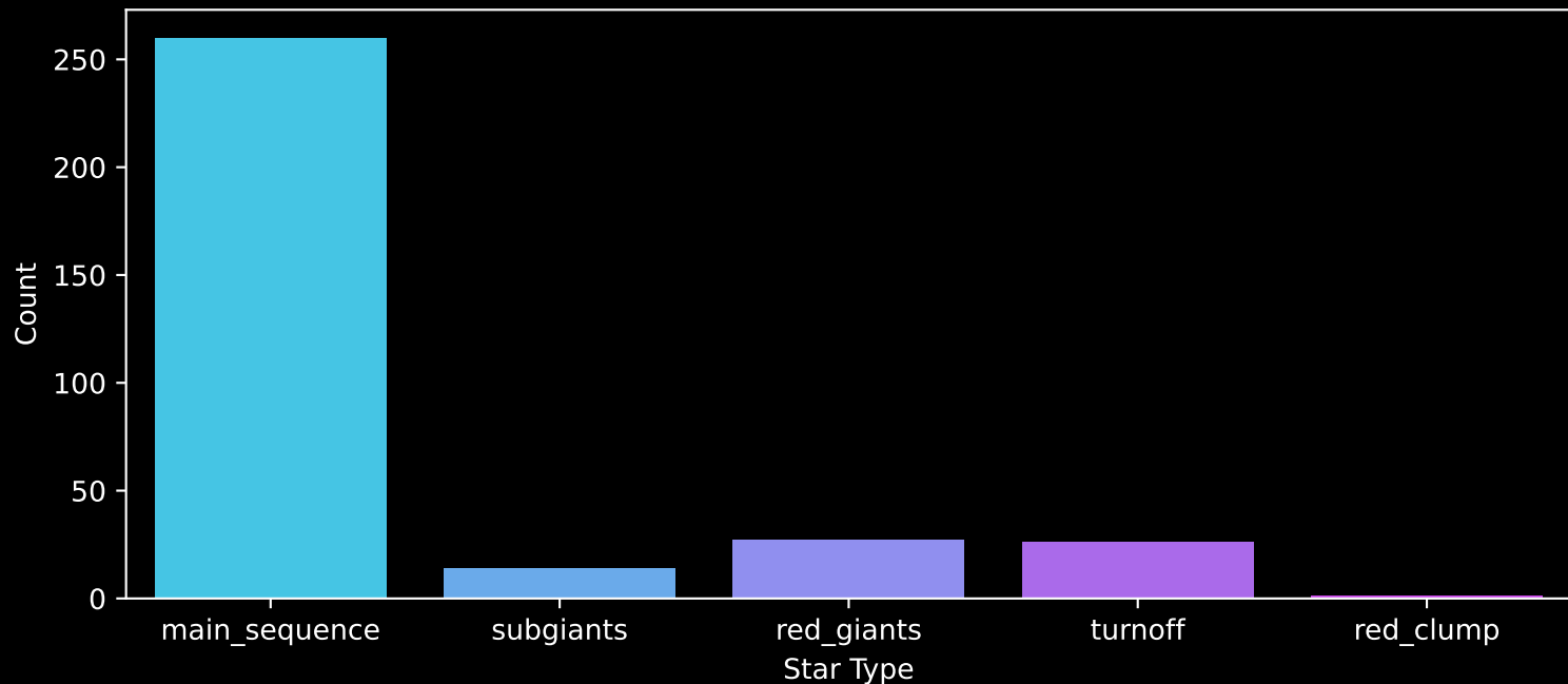
Gaia Cluster: [Berkeley_98] Count plot of Star Type
