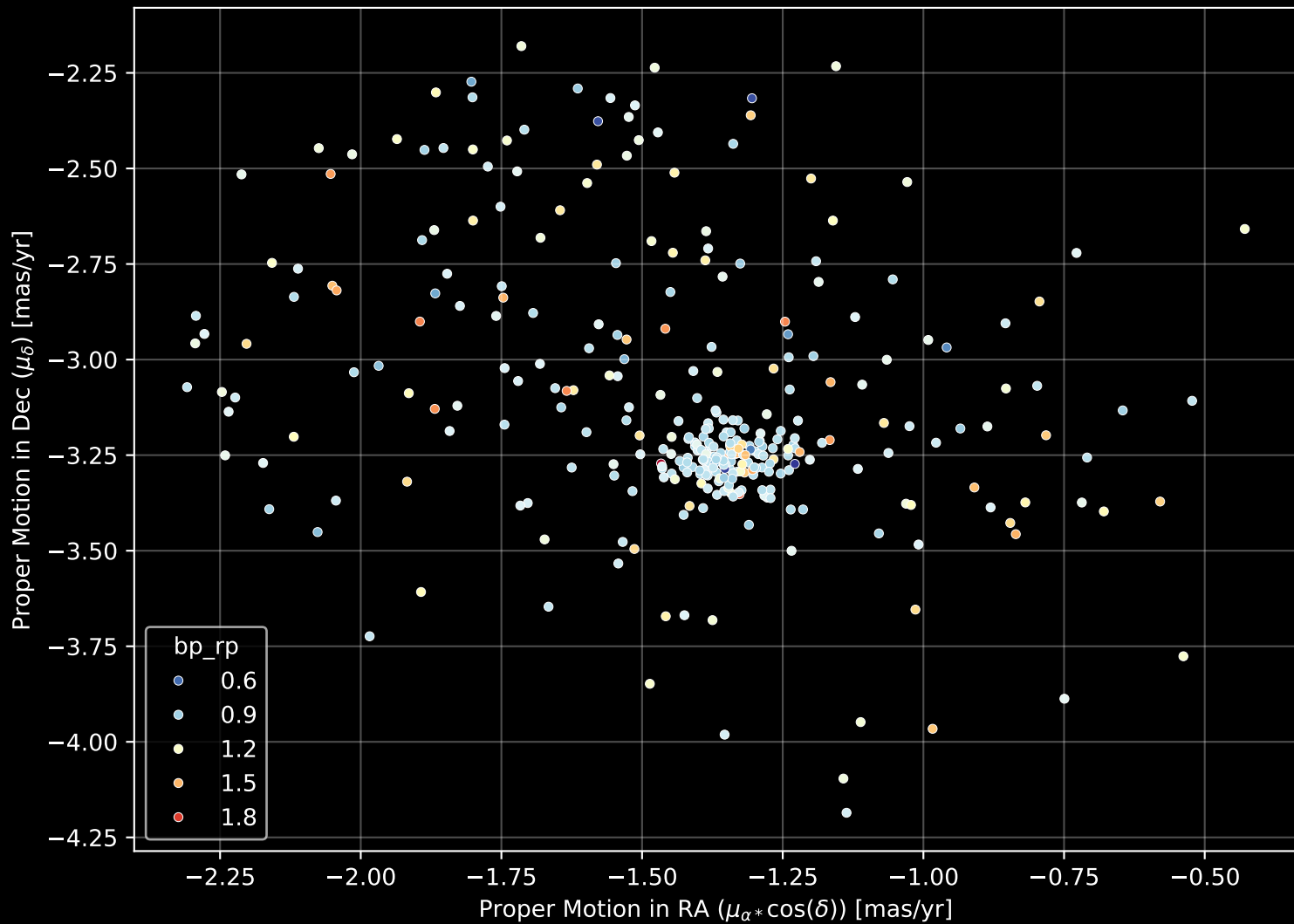
Gaia Cluster: [Berkeley_98] Proper Motion Diagram (n= 328)
