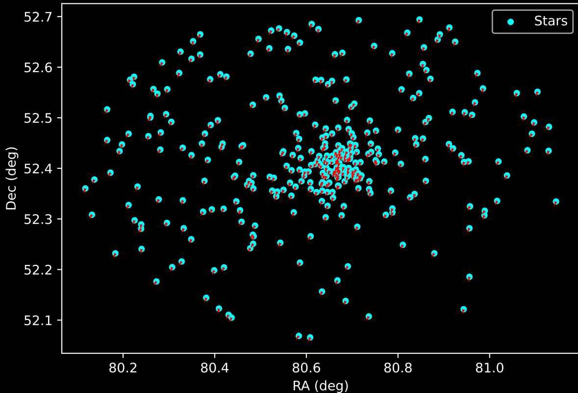
Gaia Cluster: [Berkeley_98] Proper Motion Vectors for Gaia Star Field (n= 328)
