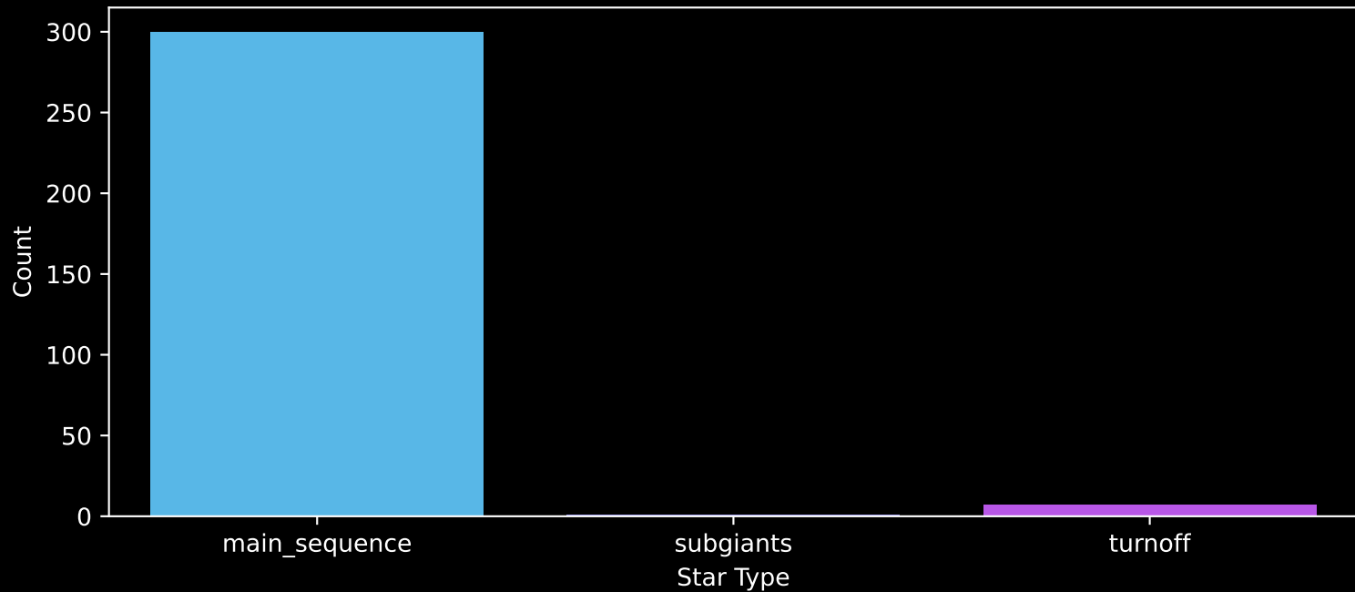
Gaia Cluster: [Blanco_1] Count plot of Star Type
