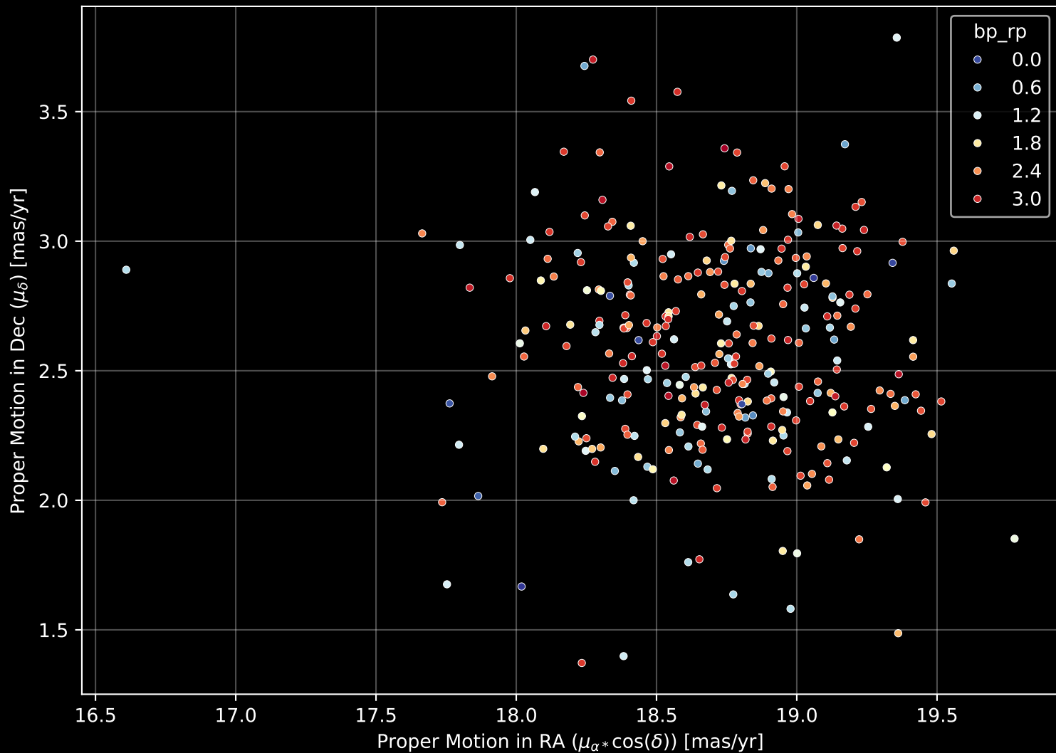
Gaia Cluster: [Blanco_1] Proper Motion Diagram (n= 308)
