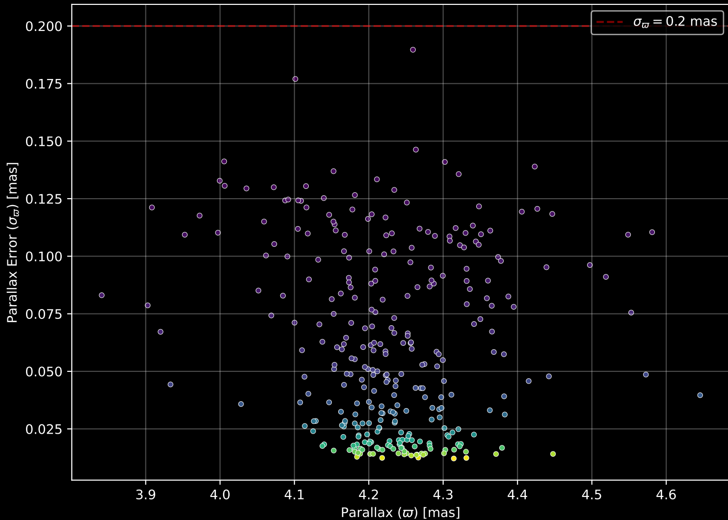
Gaia Cluster: [Blanco_1] Parallax Quality (n= 308)
