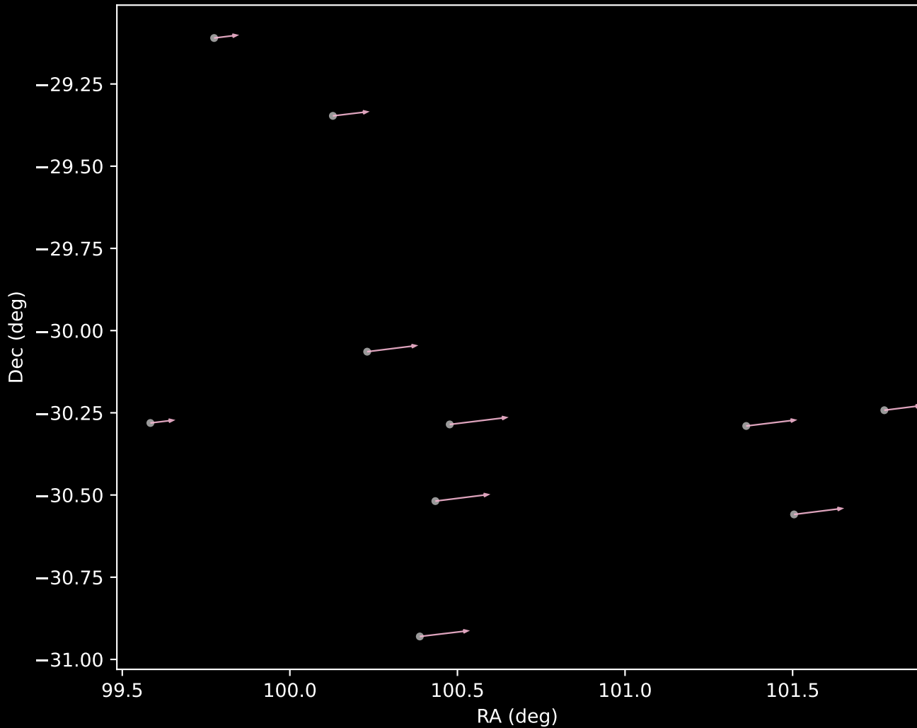
Gaia DR3 Cluster 13 Proper Motion Vectors (n=10)
