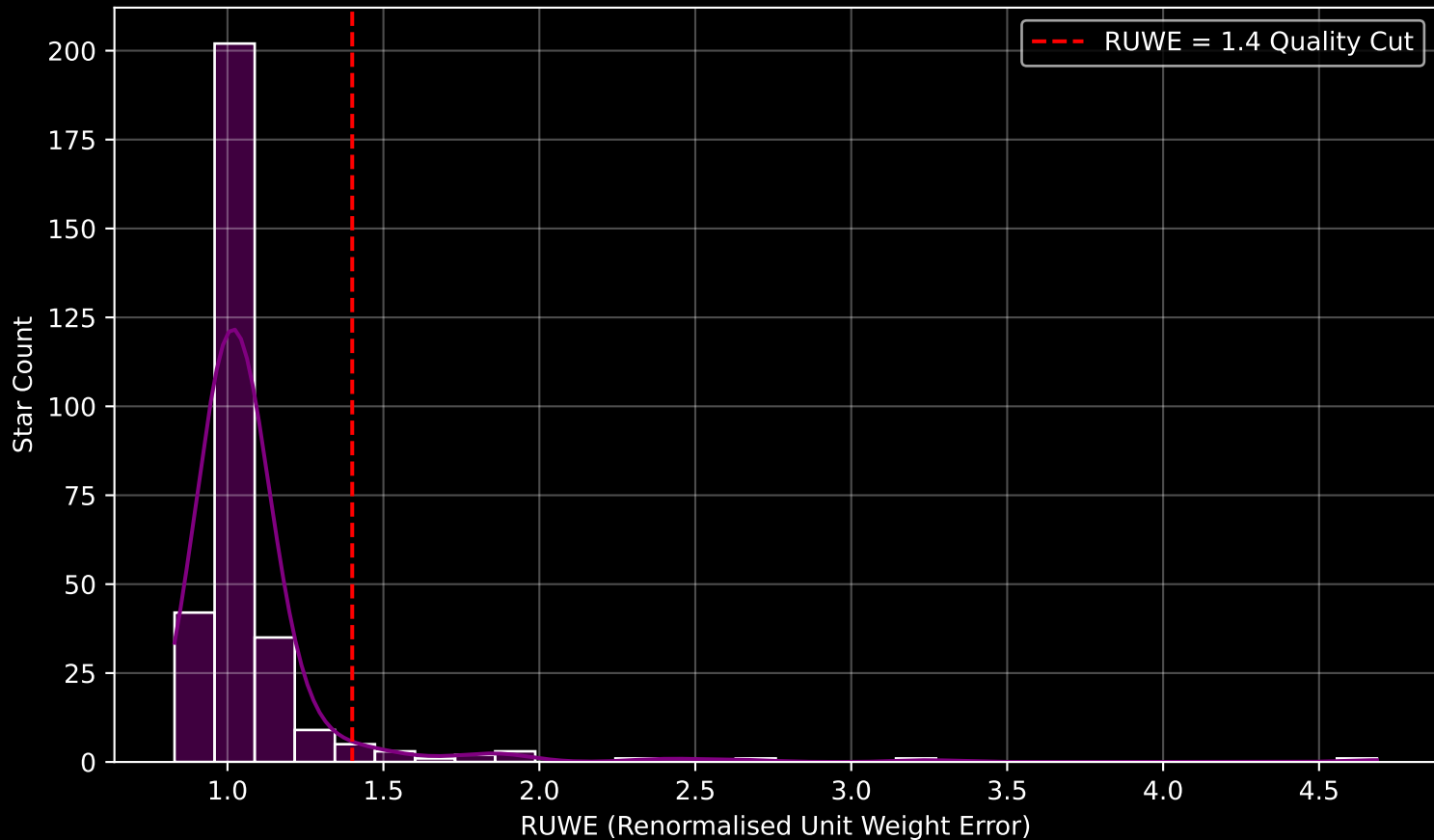
Gaia Cluster: [Blanco_1] RUWE Distribution (n= 307)
