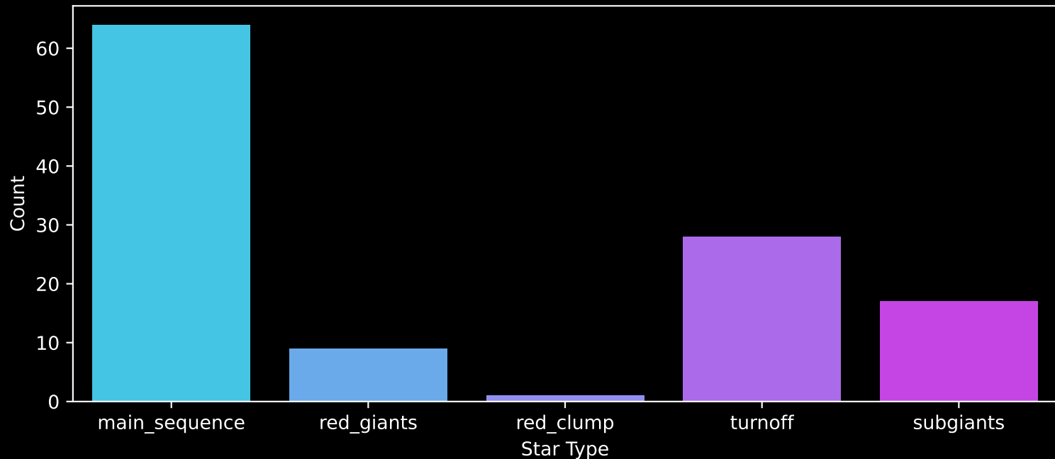
Gaia Cluster: [Bochum_6] Count plot of Star Type
