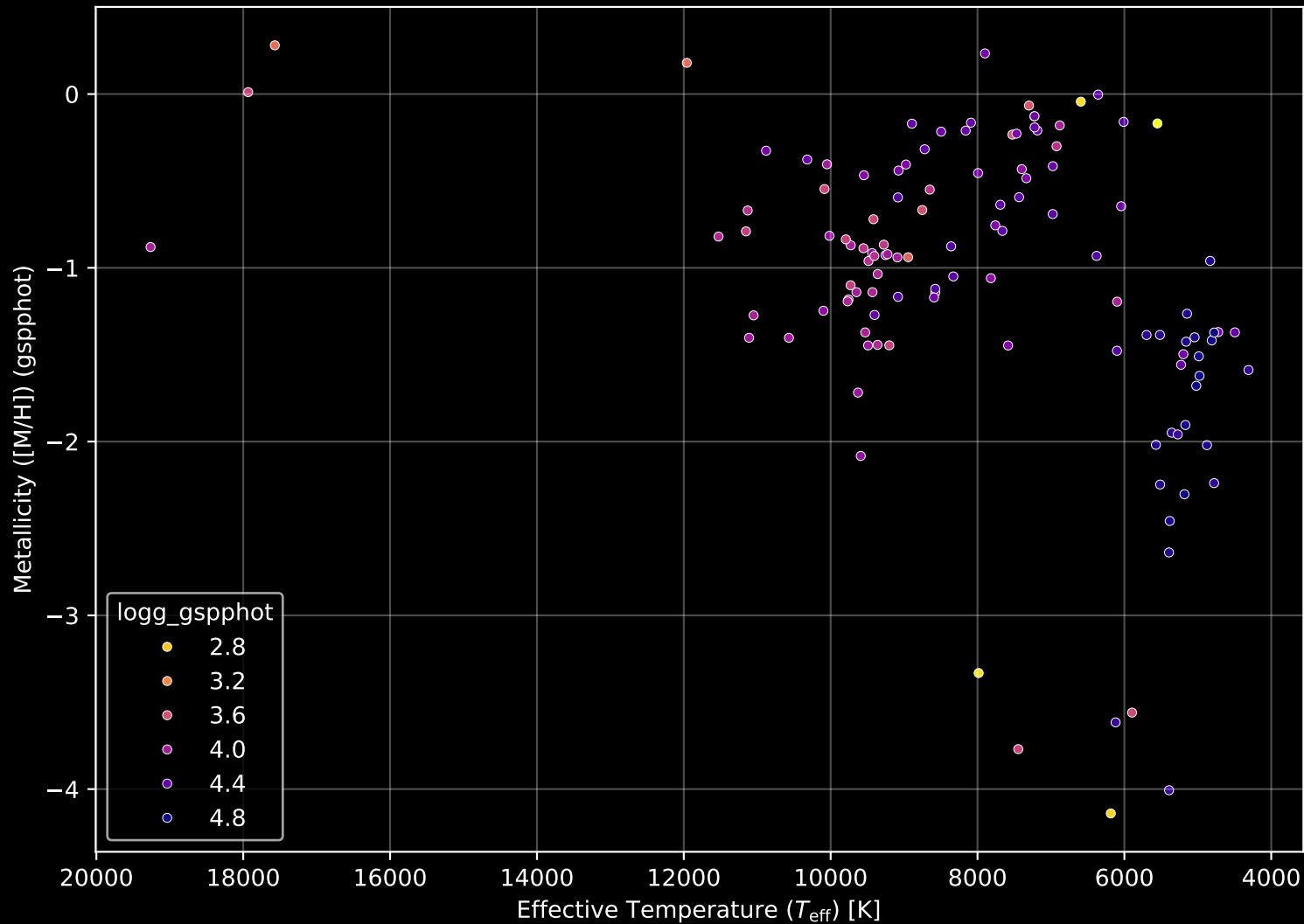
Gaia Cluster: [Bochum_6] Stellar Population Parameters (n= 119)
