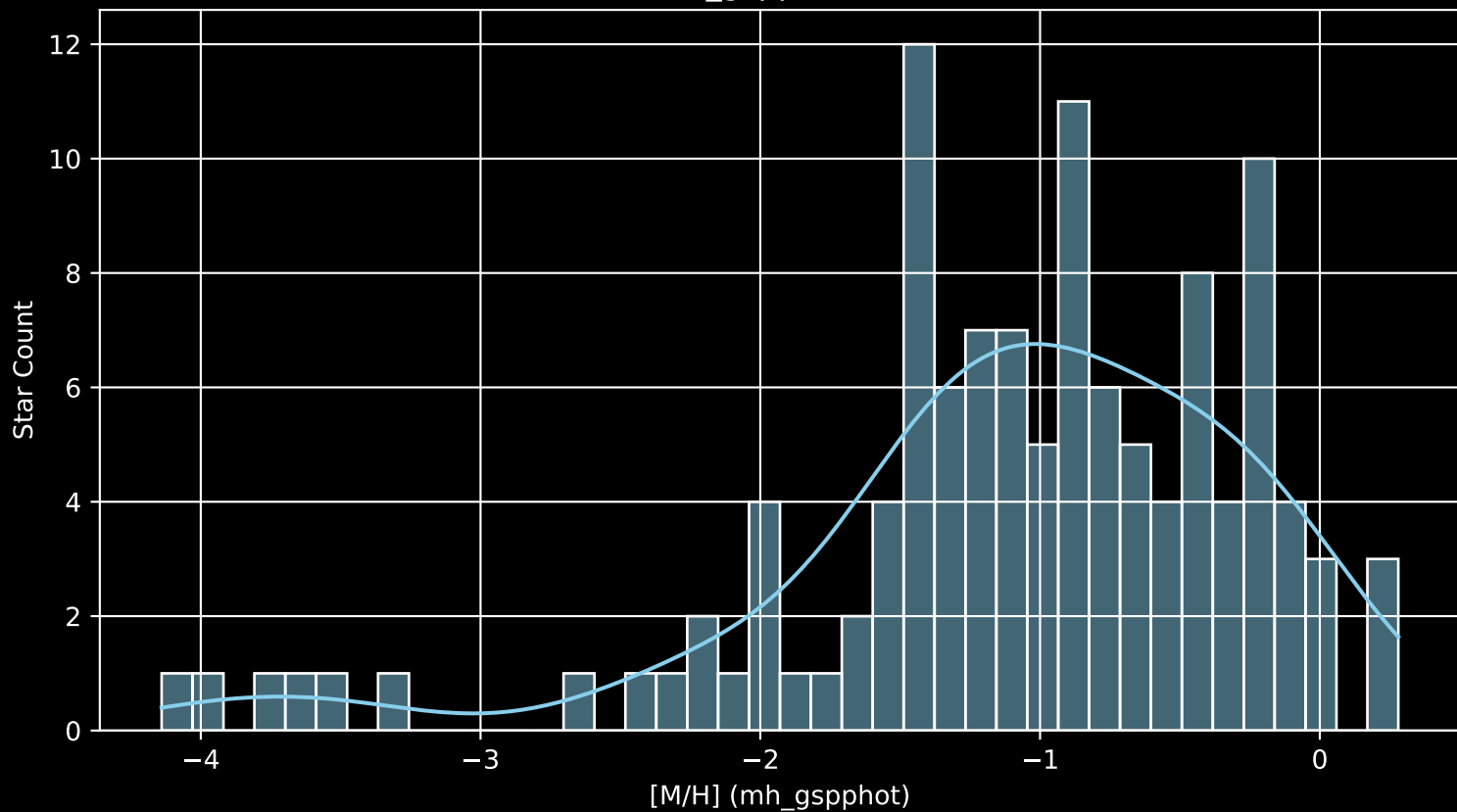
Gaia Cluster: [Bochum_6 [M/H] (mh_gspphot) (n= 119)
