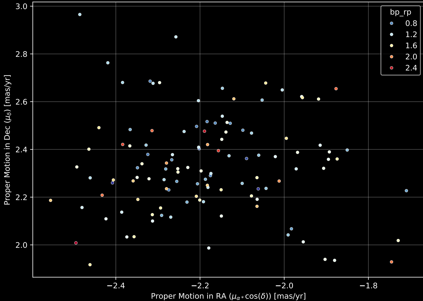
Gaia Cluster: [Bochum_6] Proper Motion Diagram (n= 119)
