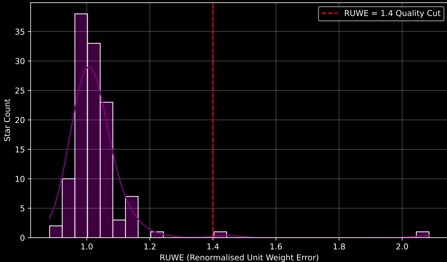
Gaia Cluster: [Bochum_6] RUWE Distribution (n= 119)
