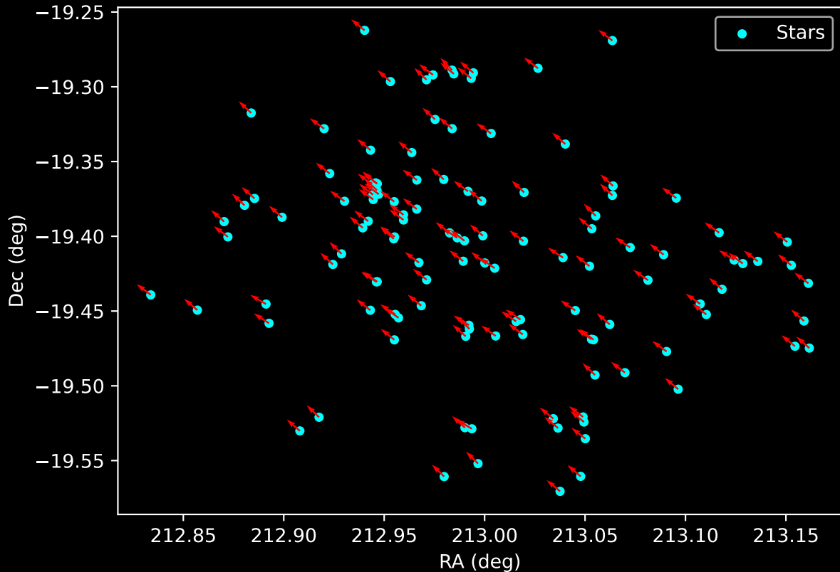
Gaia Cluster: [Bochum_6] Proper Motion Vectors for Gaia Star Field (n= 119)
