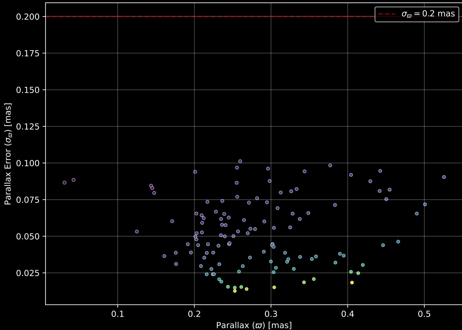
Gaia Cluster: [Bochum_6] Parallax Quality (n= 119)
