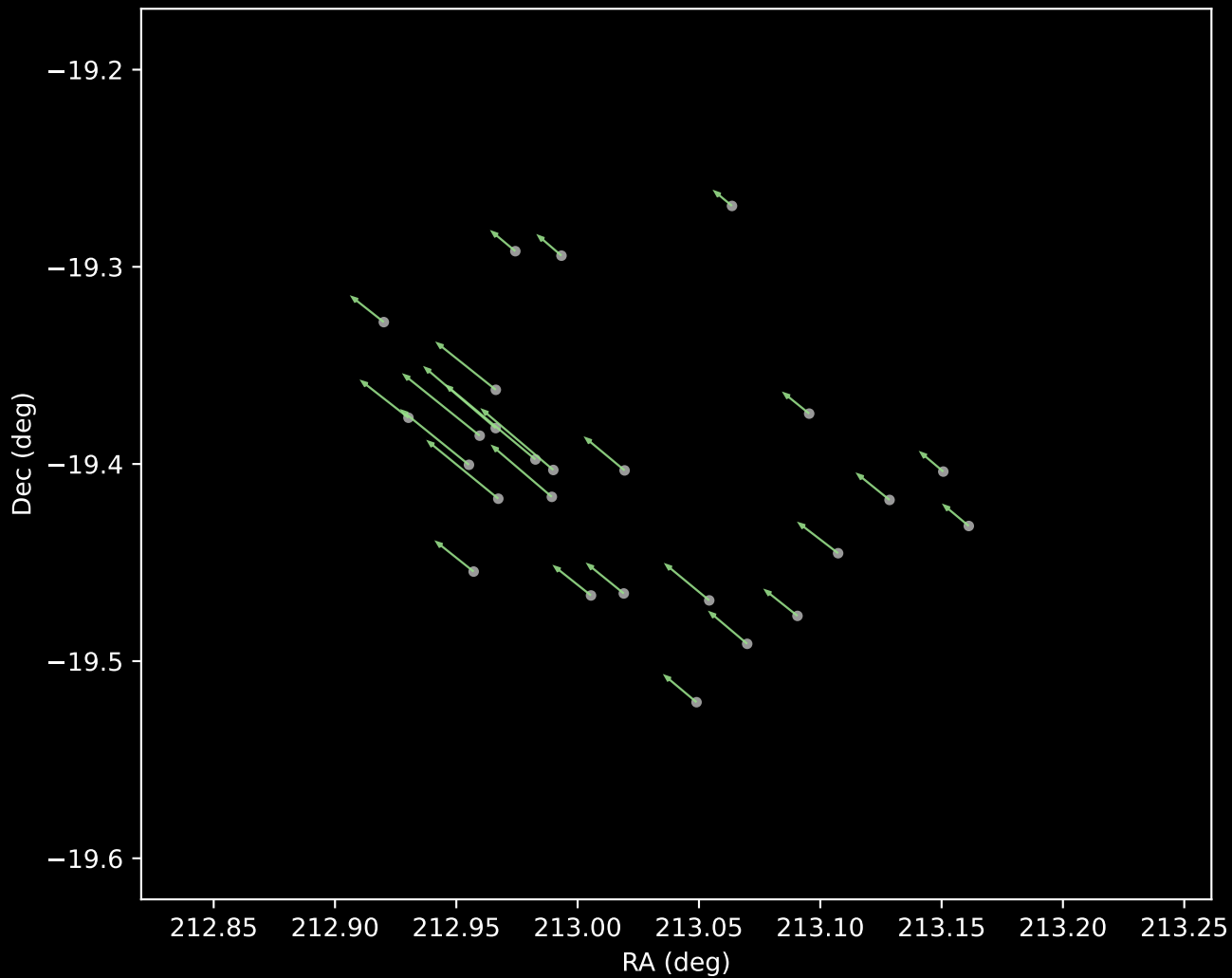
Gaia DR3 Cluster 5 Proper Motion Vectors (n=26)
