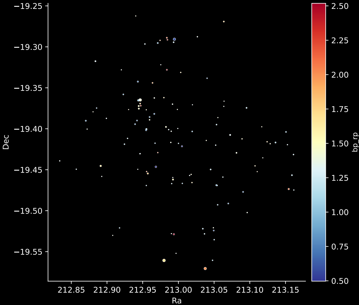
Gaia Cluster: [Bochum_6] Stars: 119
