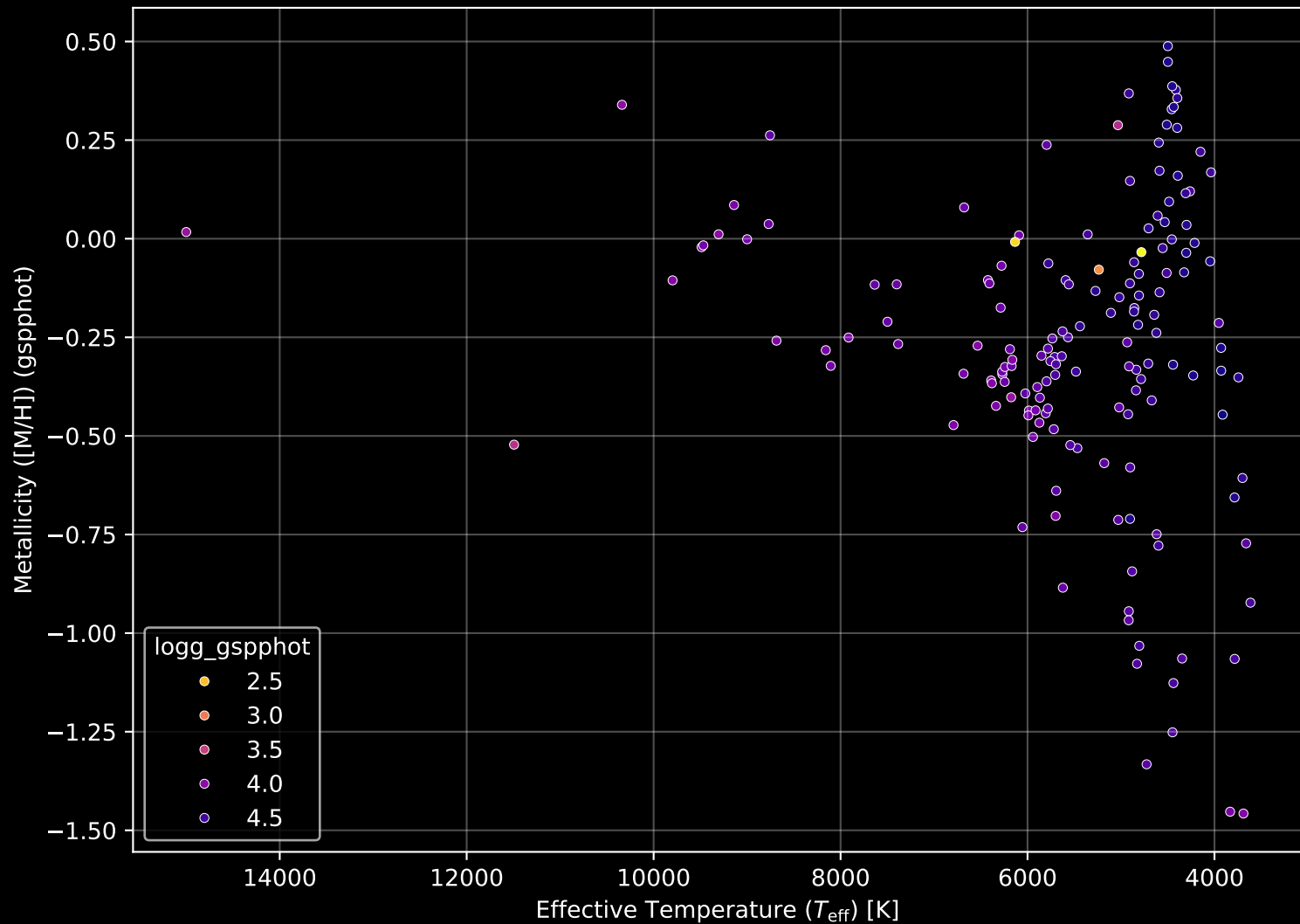
Gaia Cluster: [COIN-Gaia_1] Stellar Population Parameters (n= 159)
