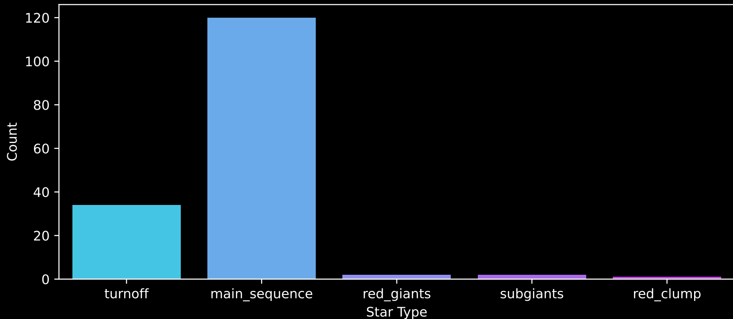
Gaia Cluster: [COIN-Gaia_1] Count plot of Star Type
