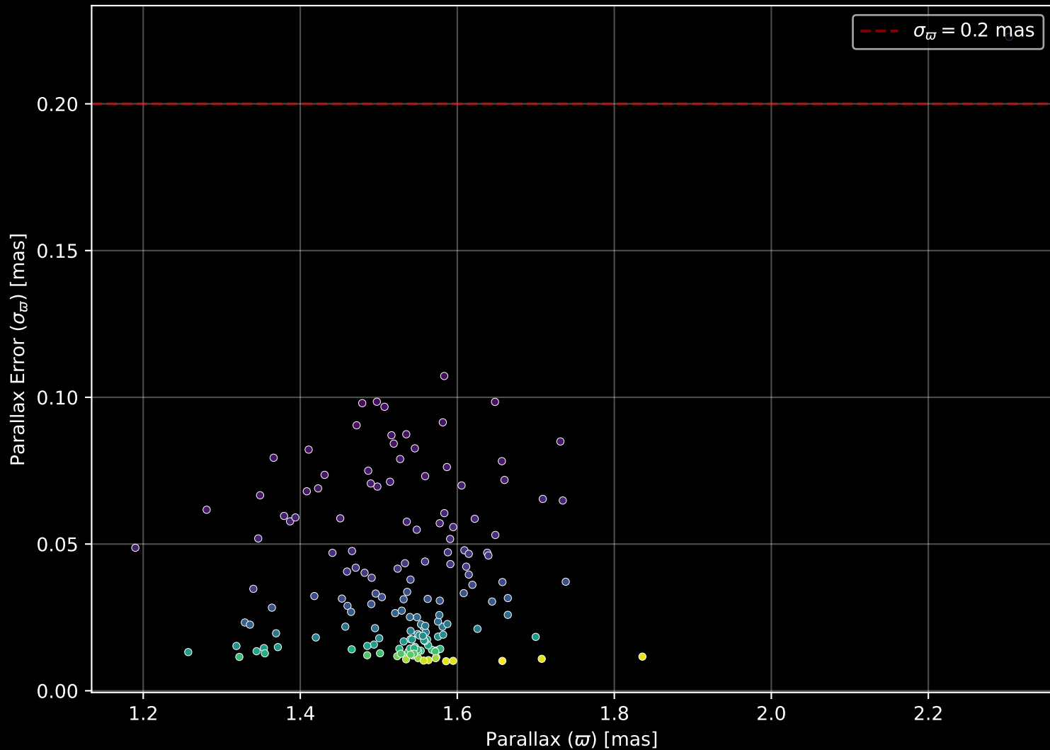
Gaia Cluster: [COIN-Gaia_1] Parallax Quality (n= 159)
