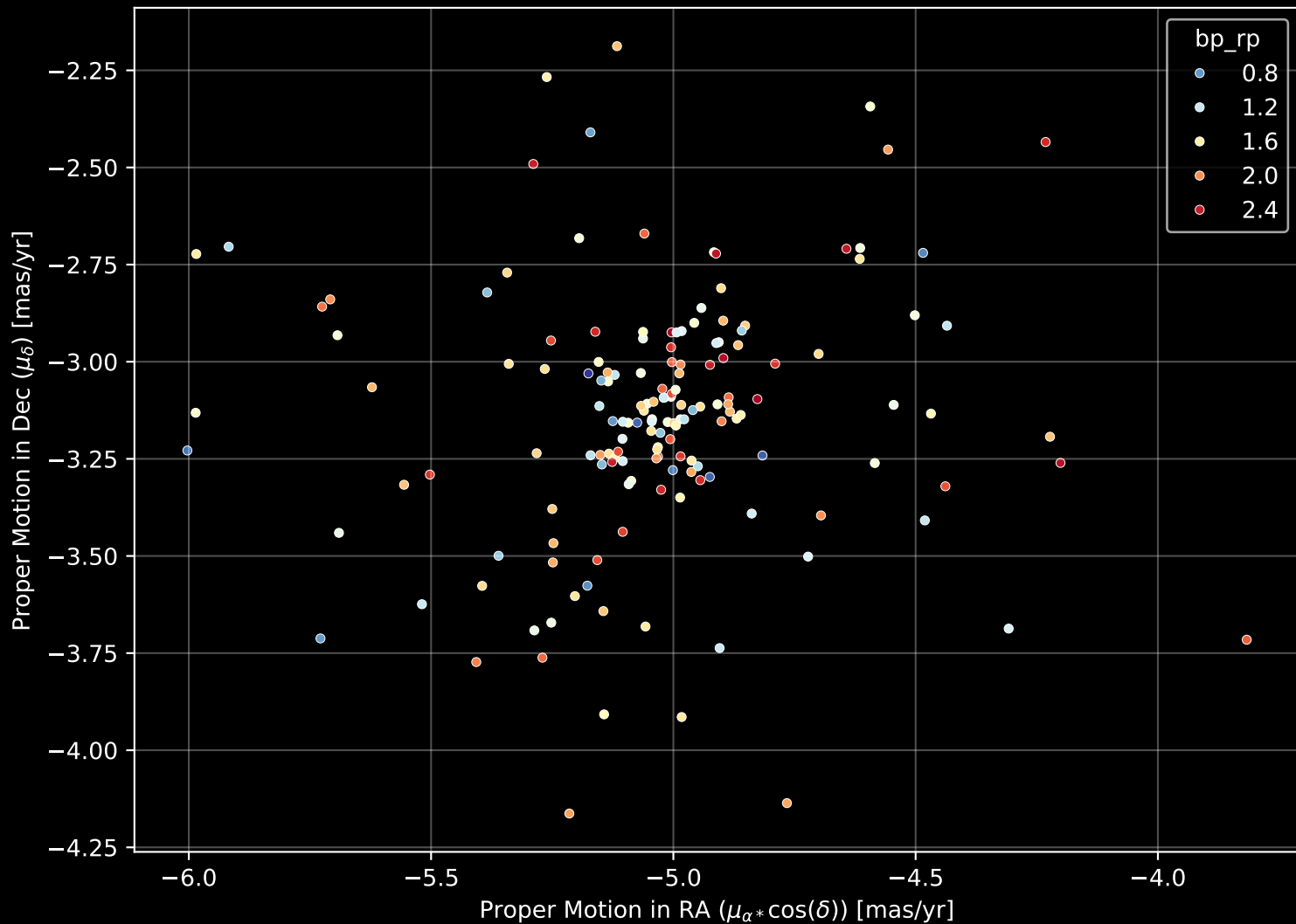
Gaia Cluster: [COIN-Gaia_1] Proper Motion Diagram (n= 159)
