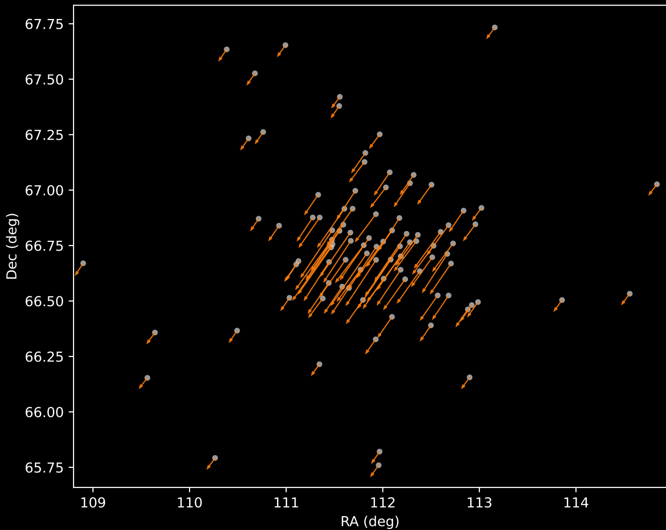
Gaia DR3 Cluster 2 Proper Motion Vectors (n=93)
