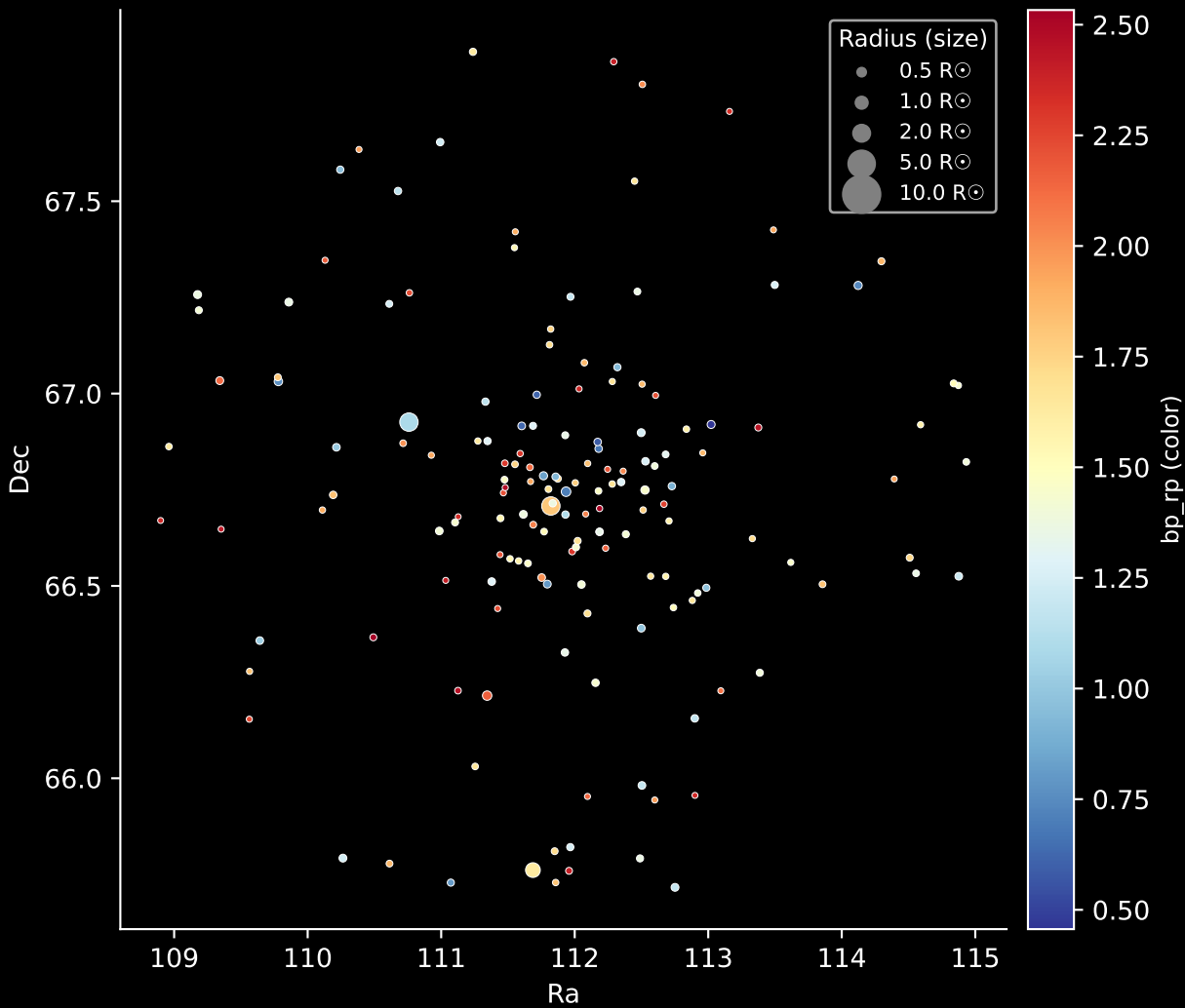
Gaia Cluster: [COIN-Gaia_1] Stars: 159
