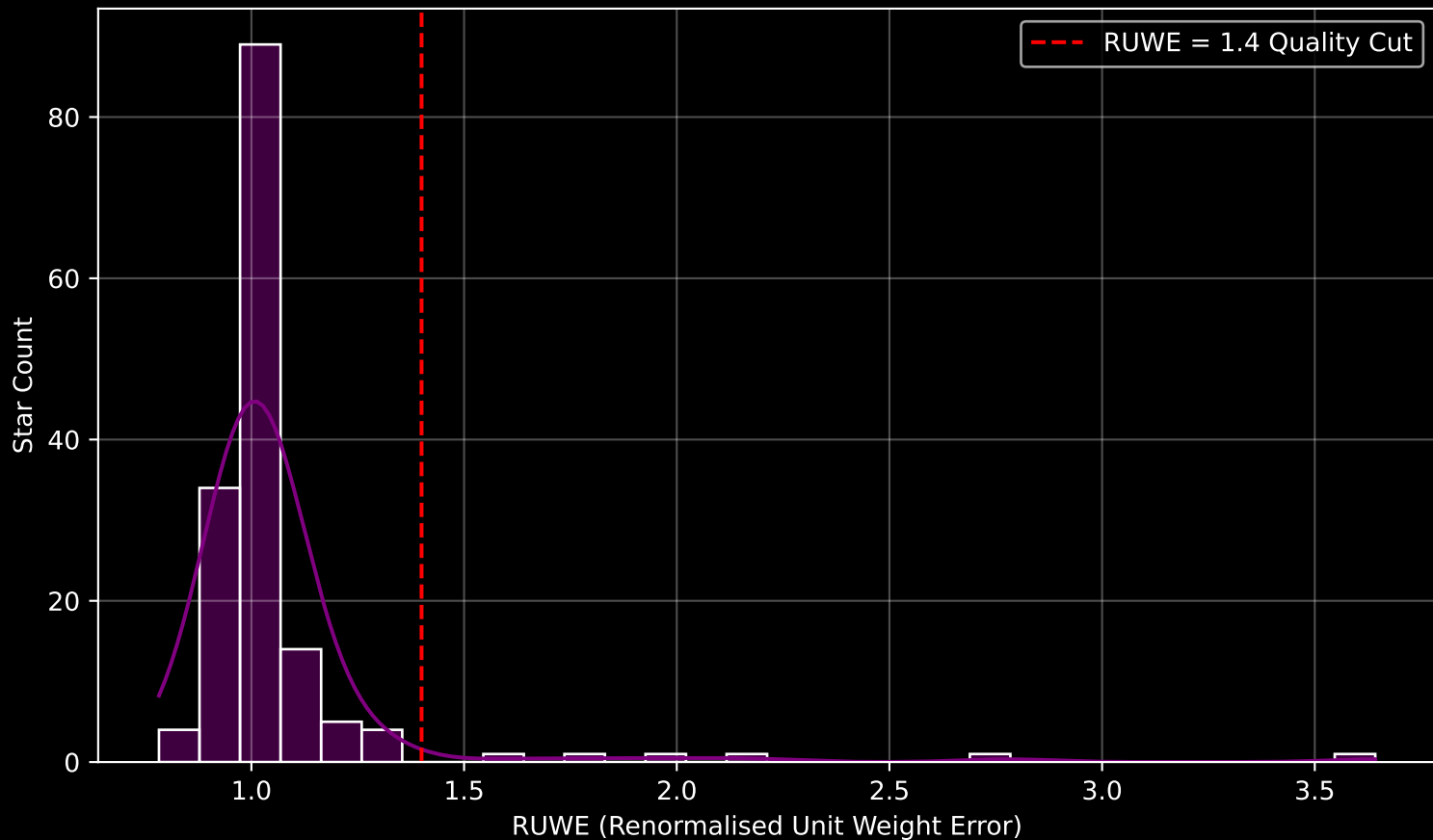
Gaia Cluster: [COIN-Gaia_1] RUWE Distribution (n= 156)
