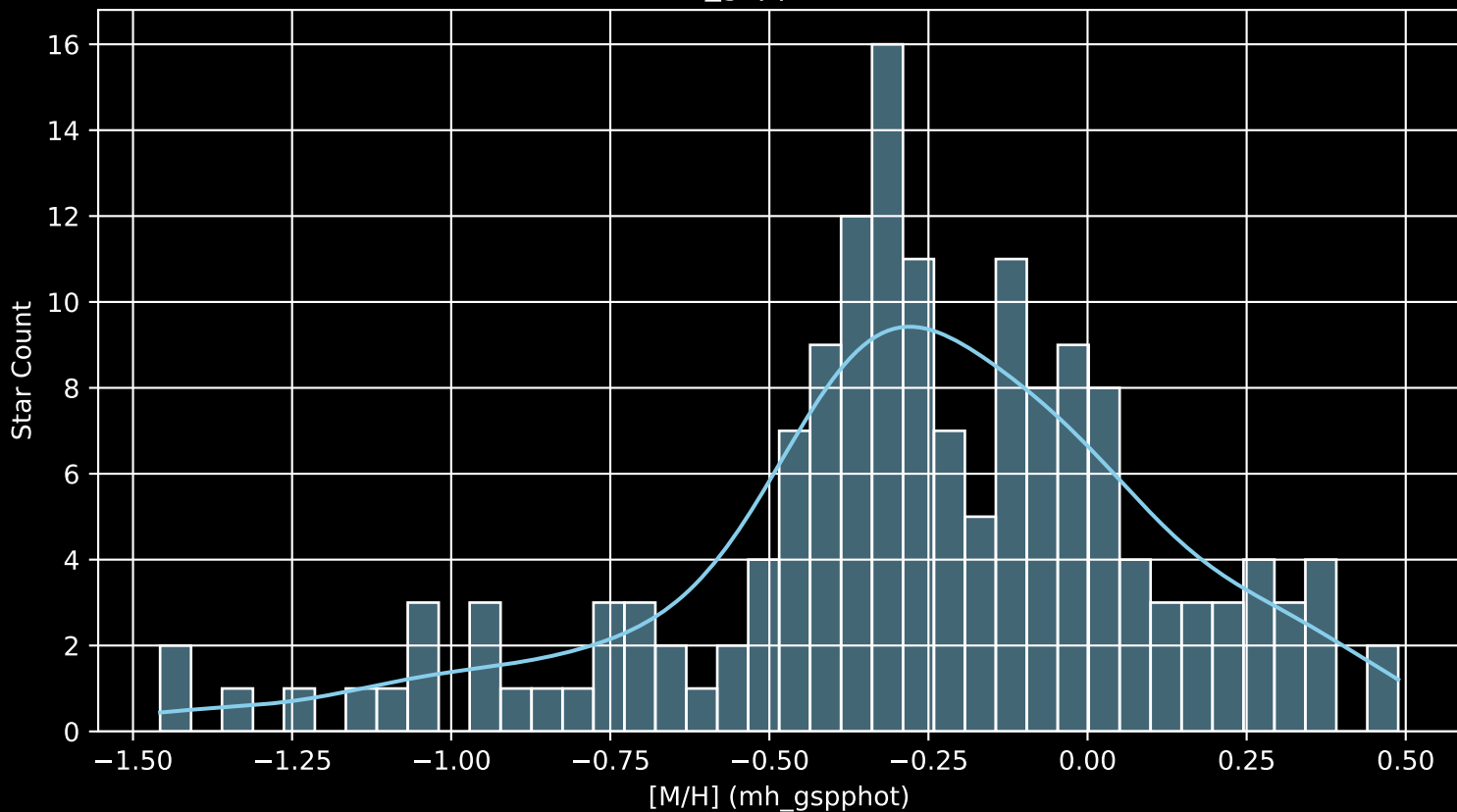
Gaia Cluster: [COIN-Gaia_1 [M/H] (mh_gspphot) (n= 159)
