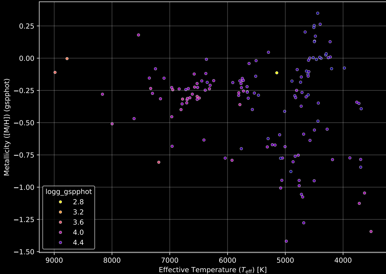
Gaia Cluster: [COIN-Gaia_11] Stellar Population Parameters (n= 144)
