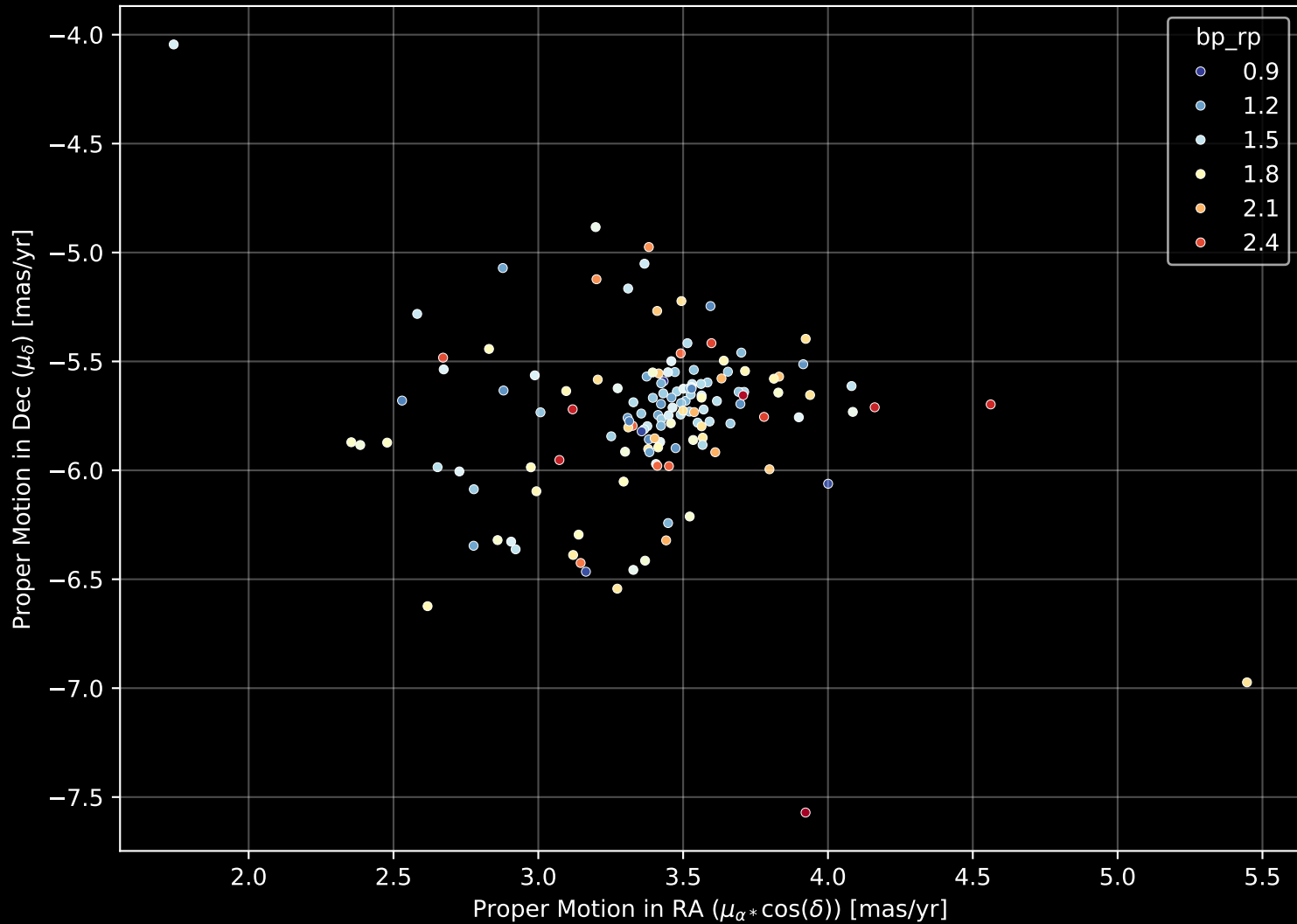
Gaia Cluster: [COIN-Gaia_11] Proper Motion Diagram (n= 144)
