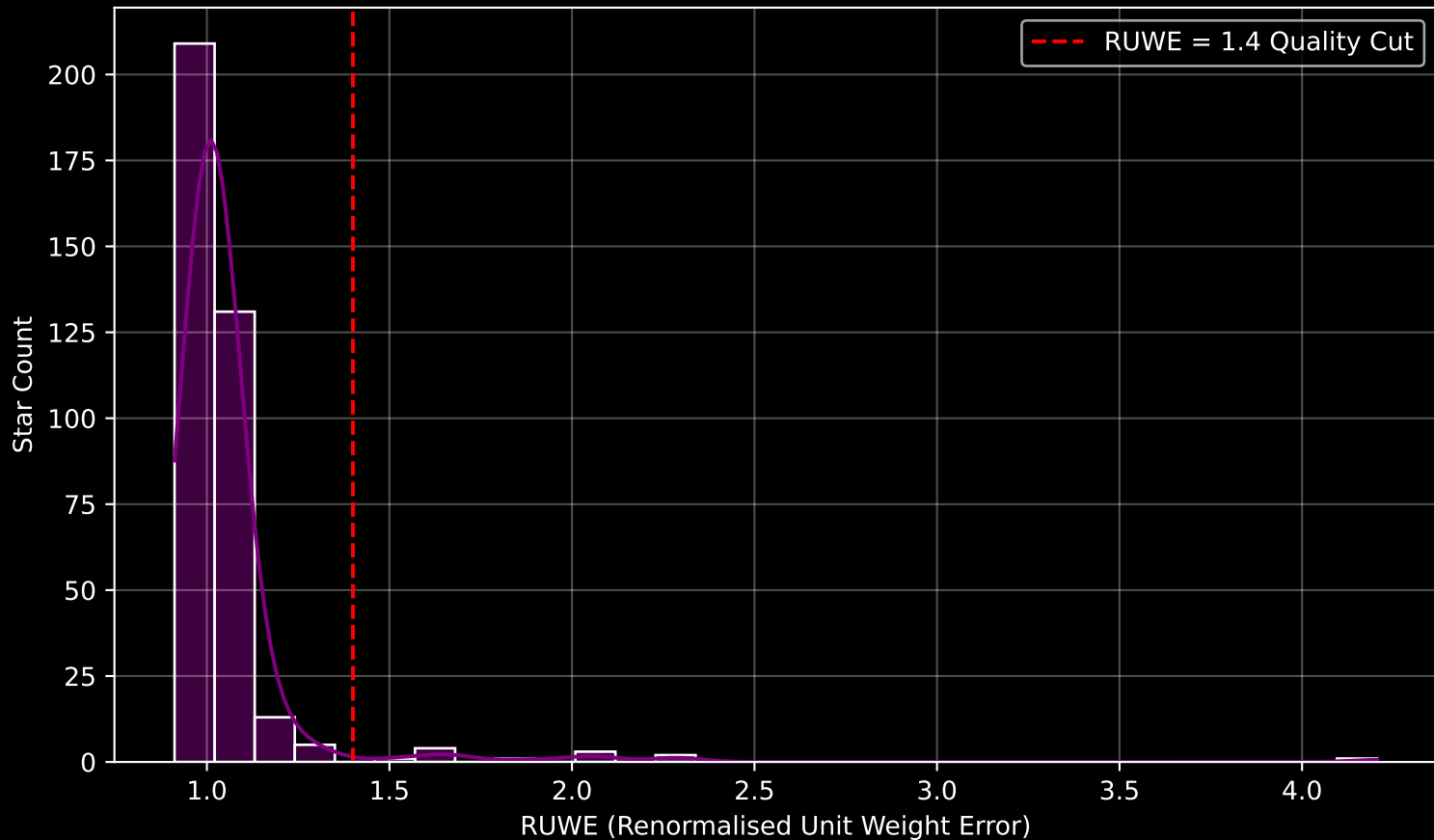
Gaia Cluster: [COIN-Gaia_15] RUWE Distribution (n= 370)
