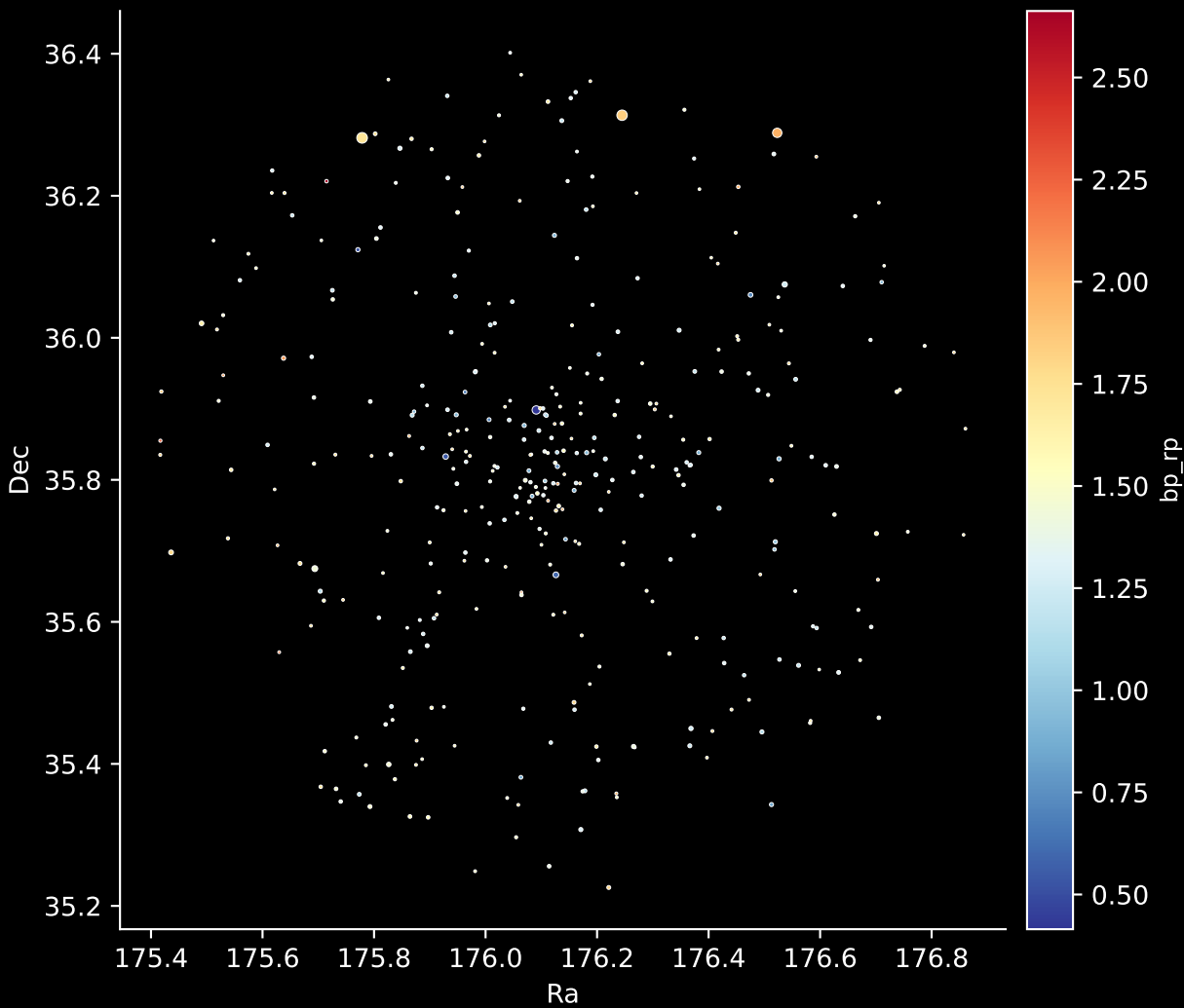
Gaia Cluster: [COIN-Gaia_15] Stars: 370
