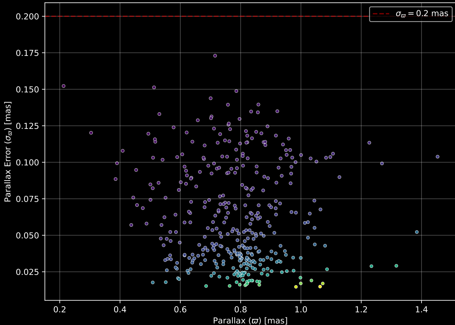
Gaia Cluster: [COIN-Gaia_15] Parallax Quality (n= 370)
