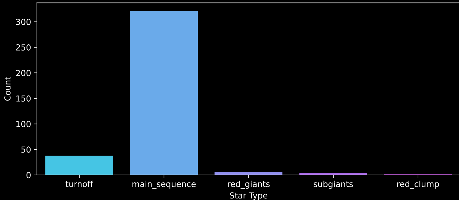
Gaia Cluster: [COIN-Gaia_15] Count plot of Star Type
