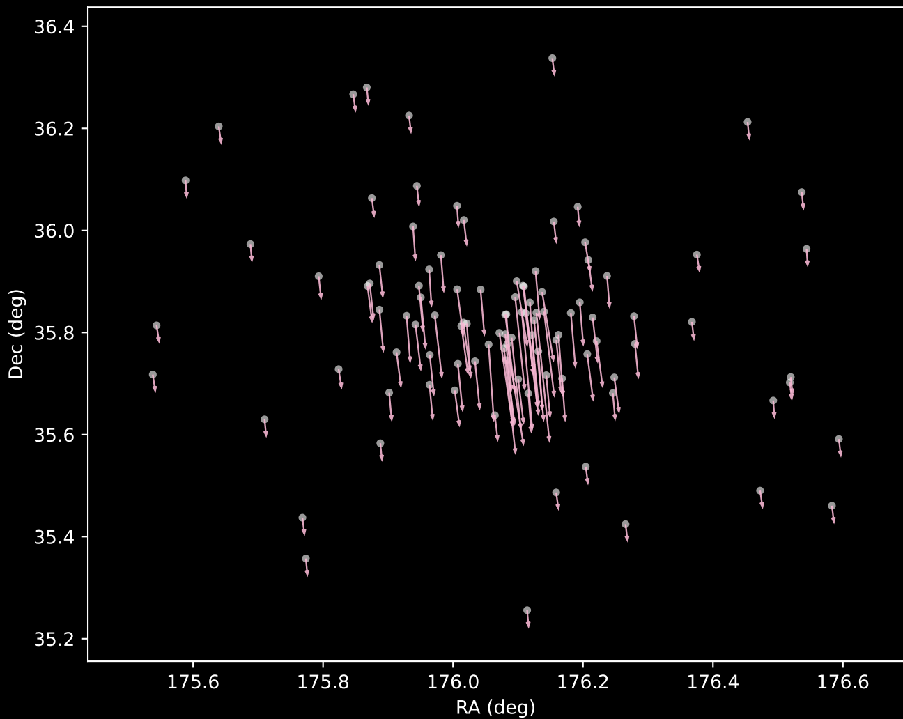
Gaia DR3 Cluster 13 Proper Motion Vectors (n=102)
