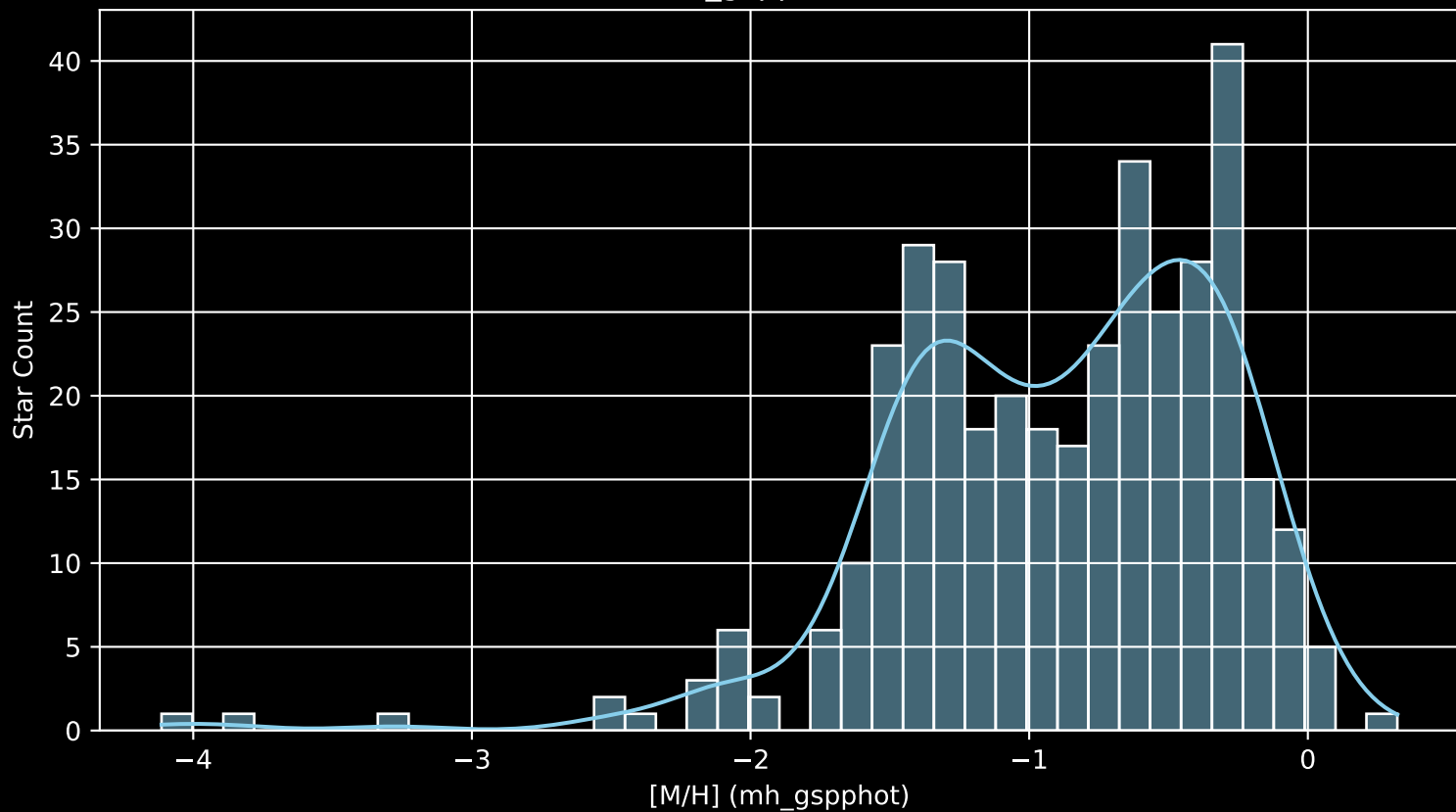
Gaia Cluster: [COIN-Gaia_15 [M/H] (mh_gspphot) (n= 370)
