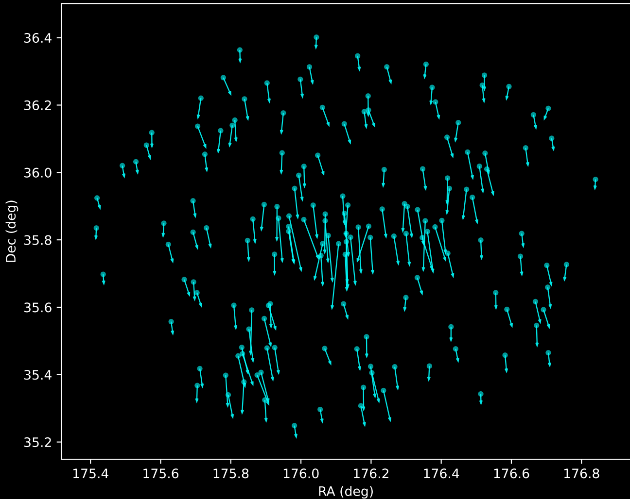
Gaia DR3 Noise Stream Proper Motion Vectors (n=154)
