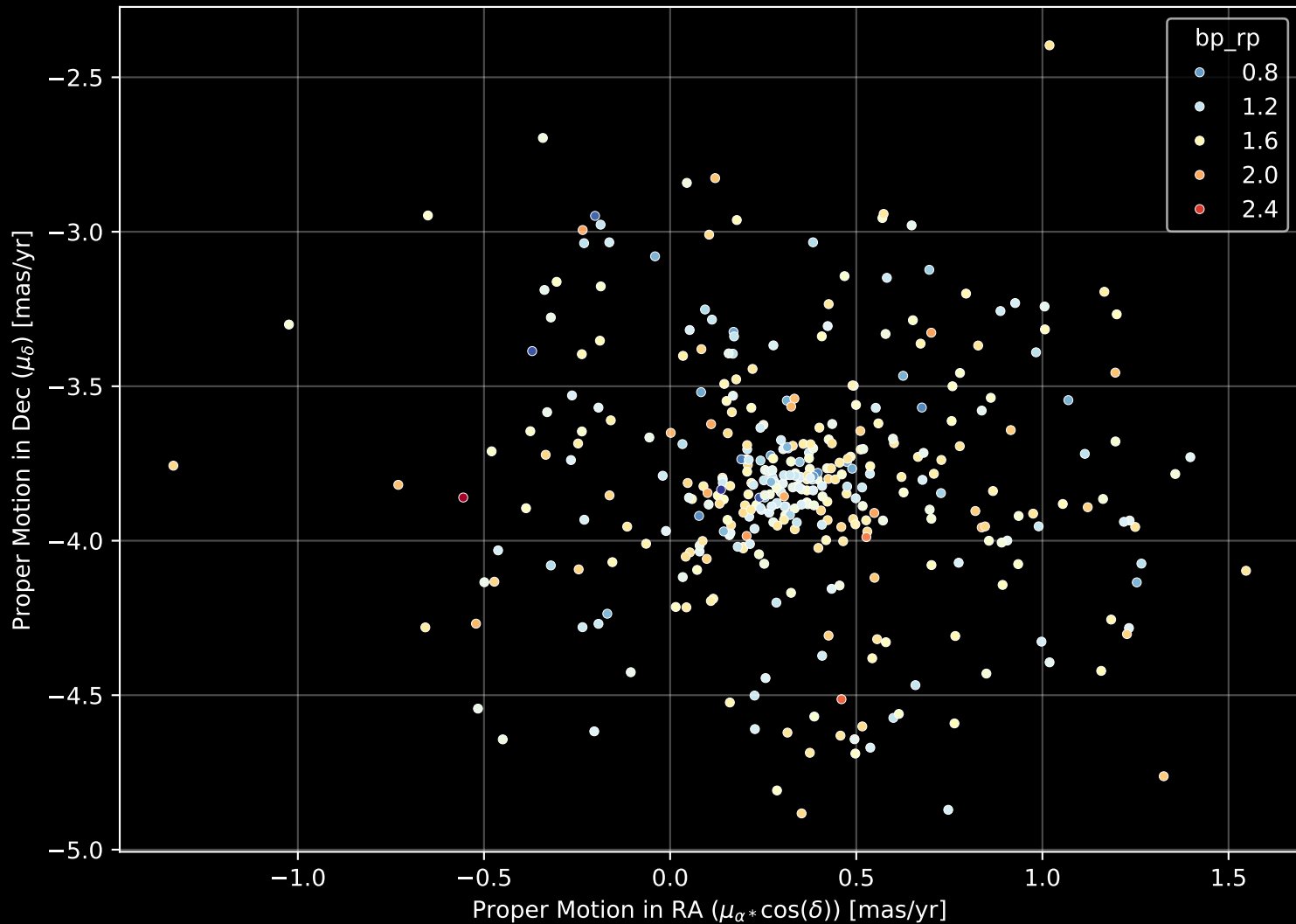
Gaia Cluster: [COIN-Gaia_15] Proper Motion Diagram (n= 370)
