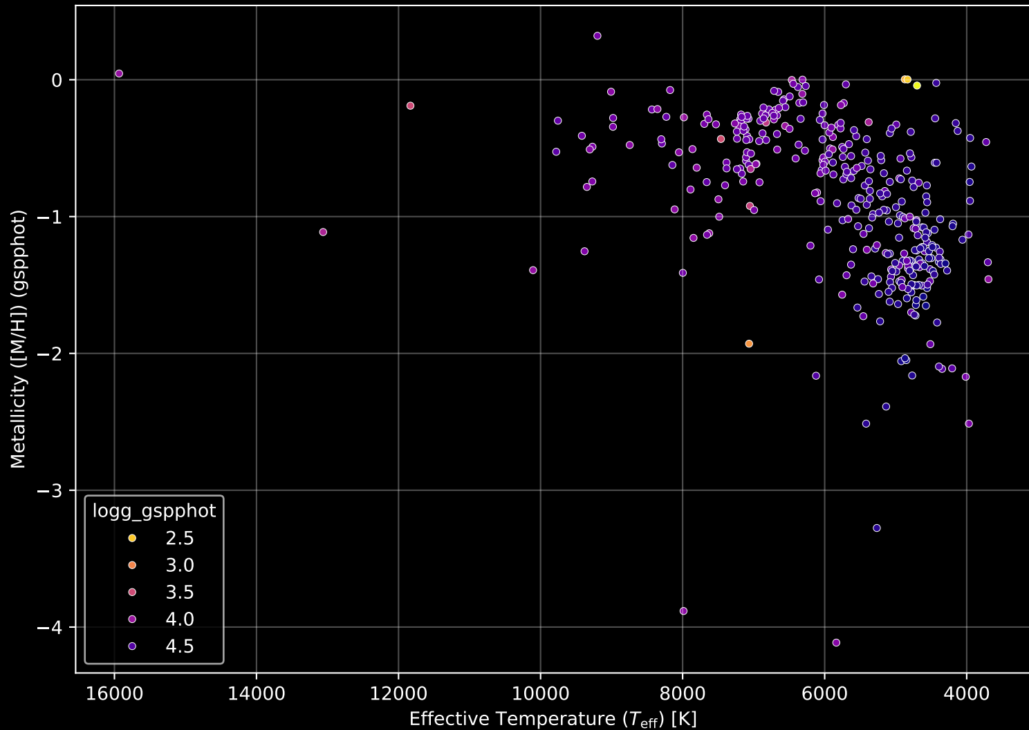
Gaia Cluster: [COIN-Gaia_15] Stellar Population Parameters (n= 370)
