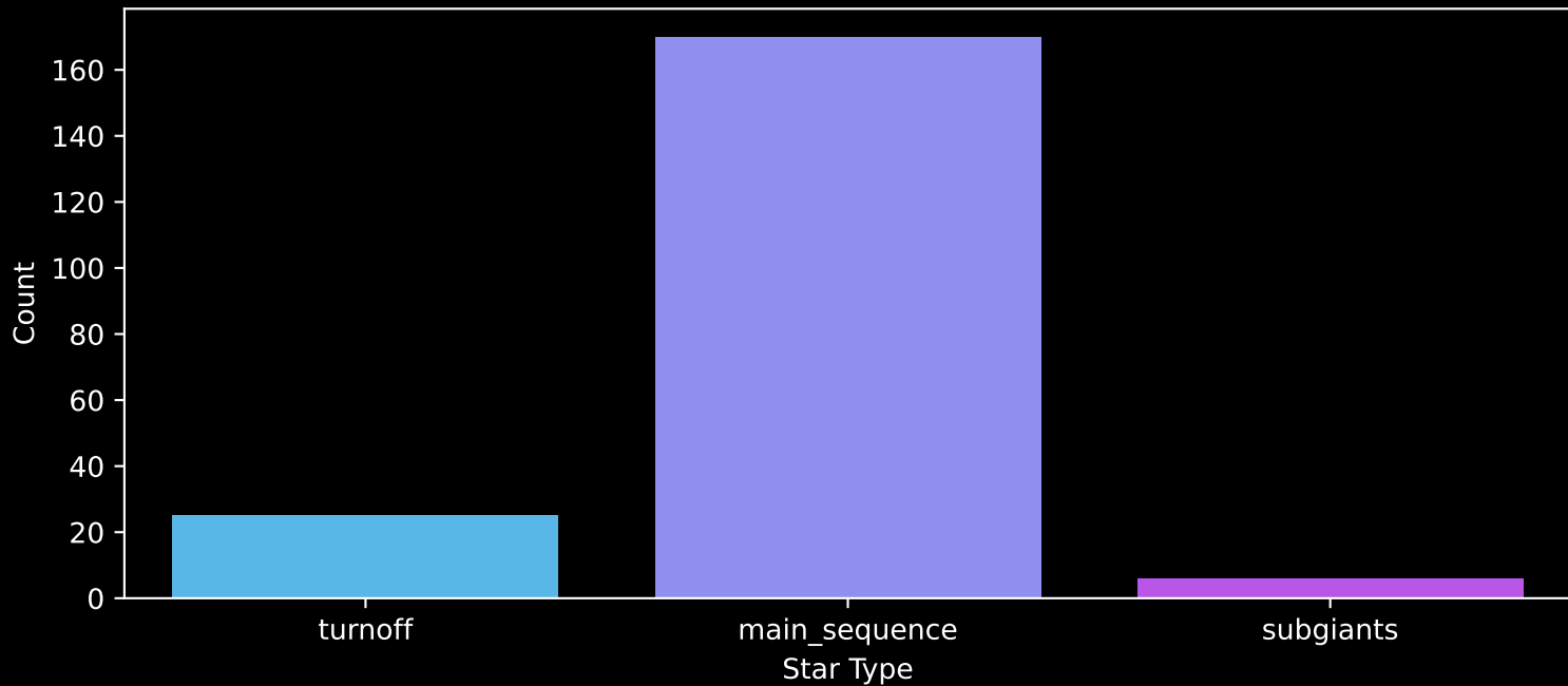
Gaia Cluster: [COIN-Gaia_17] Count plot of Star Type
