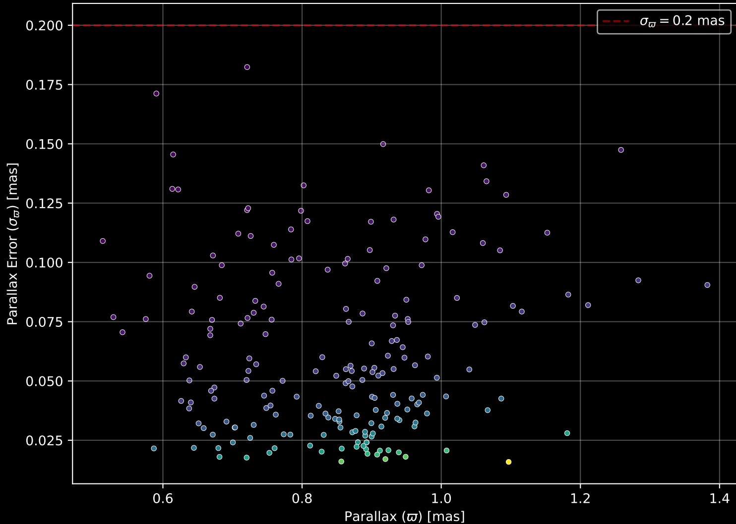
Gaia Cluster: [COIN-Gaia_17] Parallax Quality (n= 201)
