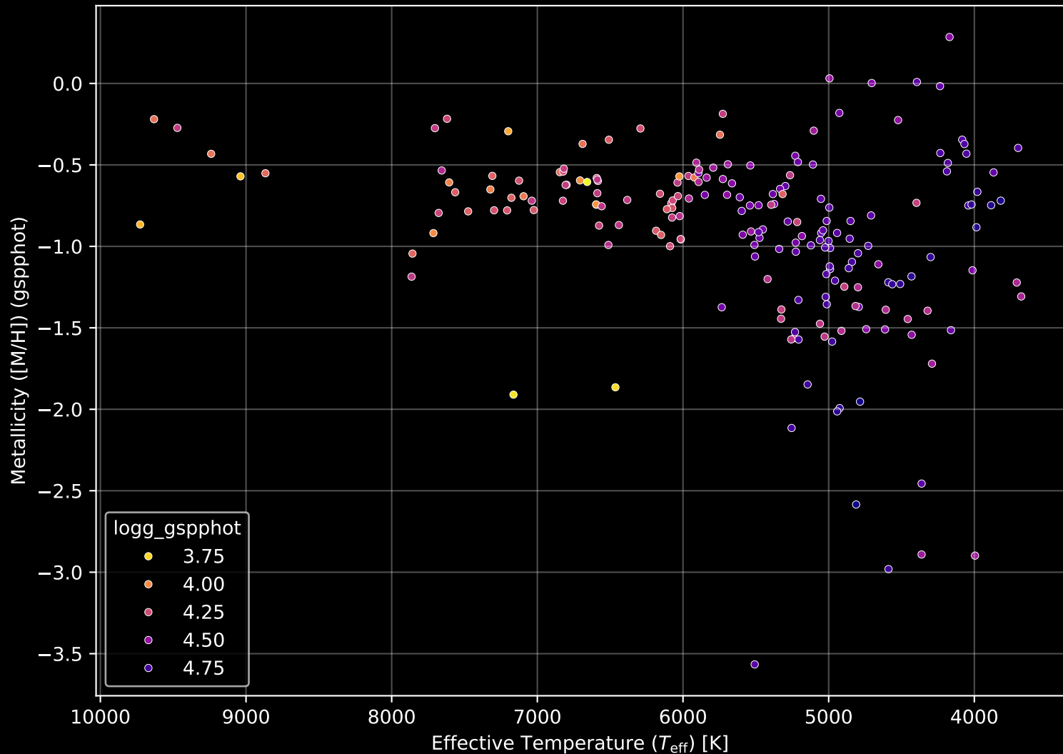
Gaia Cluster: [COIN-Gaia_17] Stellar Population Parameters (n= 201)
