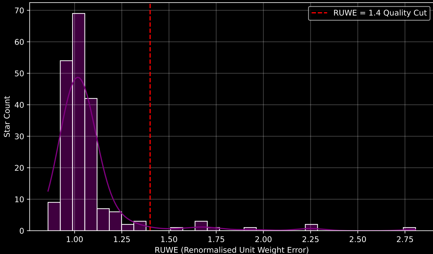
Gaia Cluster: [COIN-Gaia_17] RUWE Distribution (n= 201)
