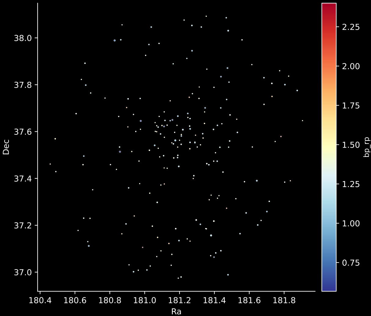
Gaia Cluster: [COIN-Gaia_17] Stars: 201
