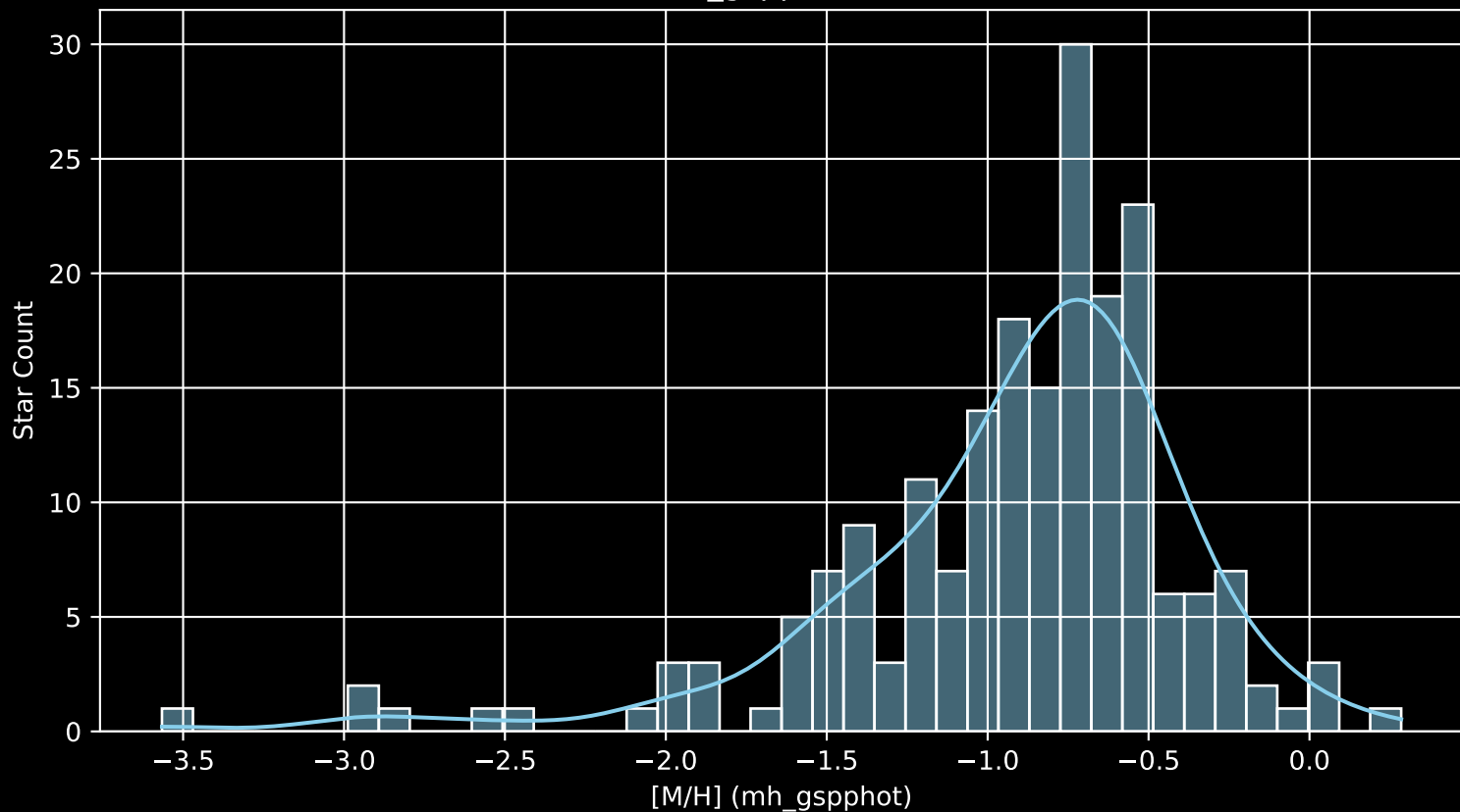
Gaia Cluster: [COIN-Gaia_17 [M/H] (mh_gspphot) (n= 201)
