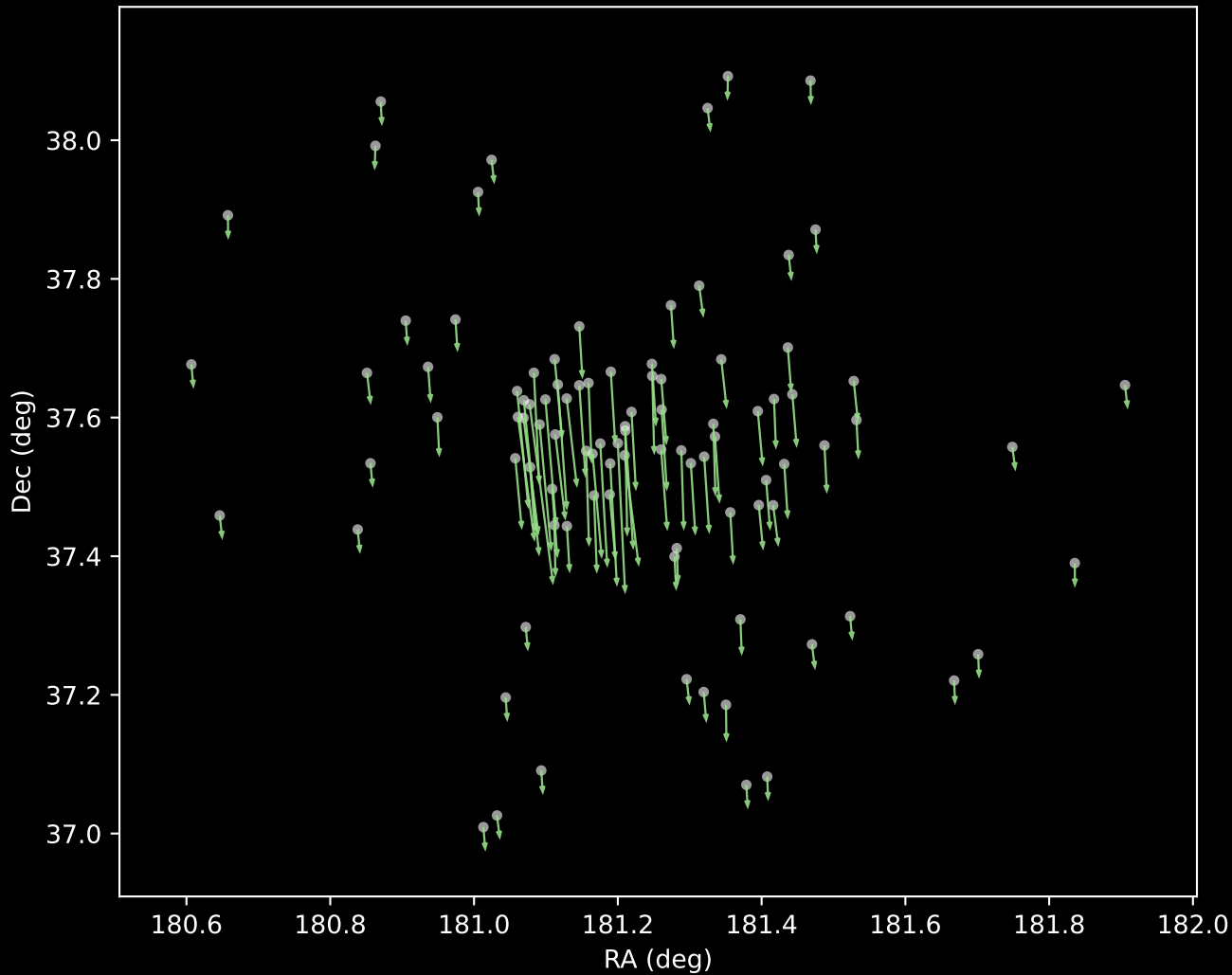
Gaia DR3 Cluster 5 Proper Motion Vectors (n=96)
