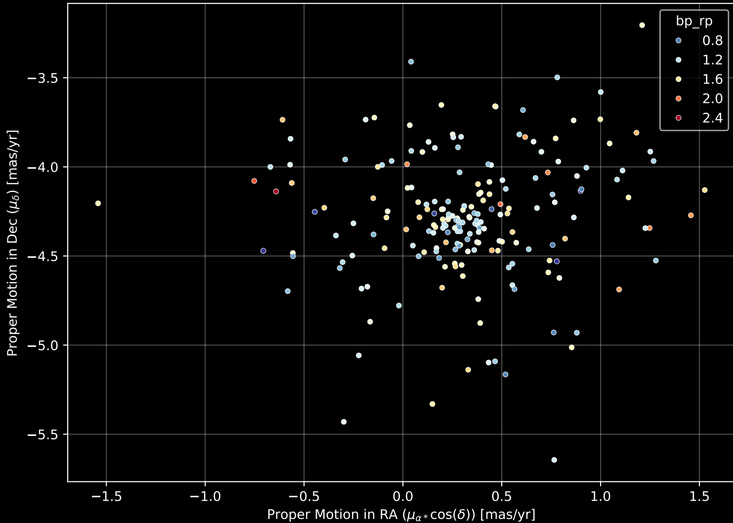
Gaia Cluster: [COIN-Gaia_17] Proper Motion Diagram (n= 201)
