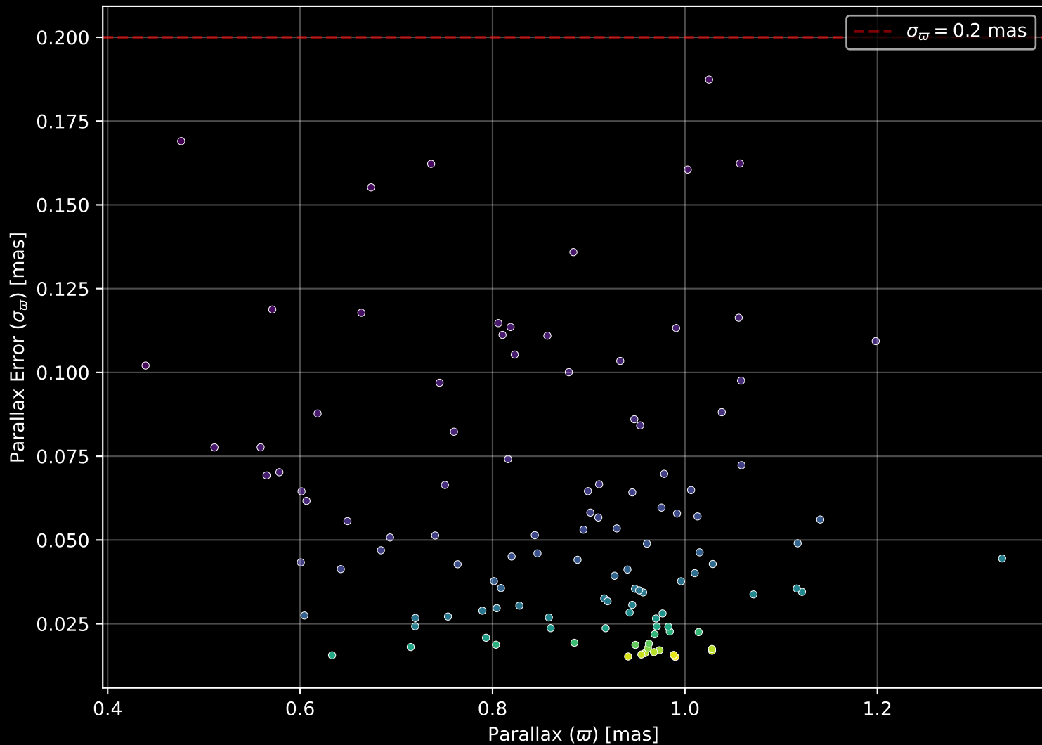
Gaia Cluster: [COIN-Gaia_18] Parallax Quality (n= 115)
