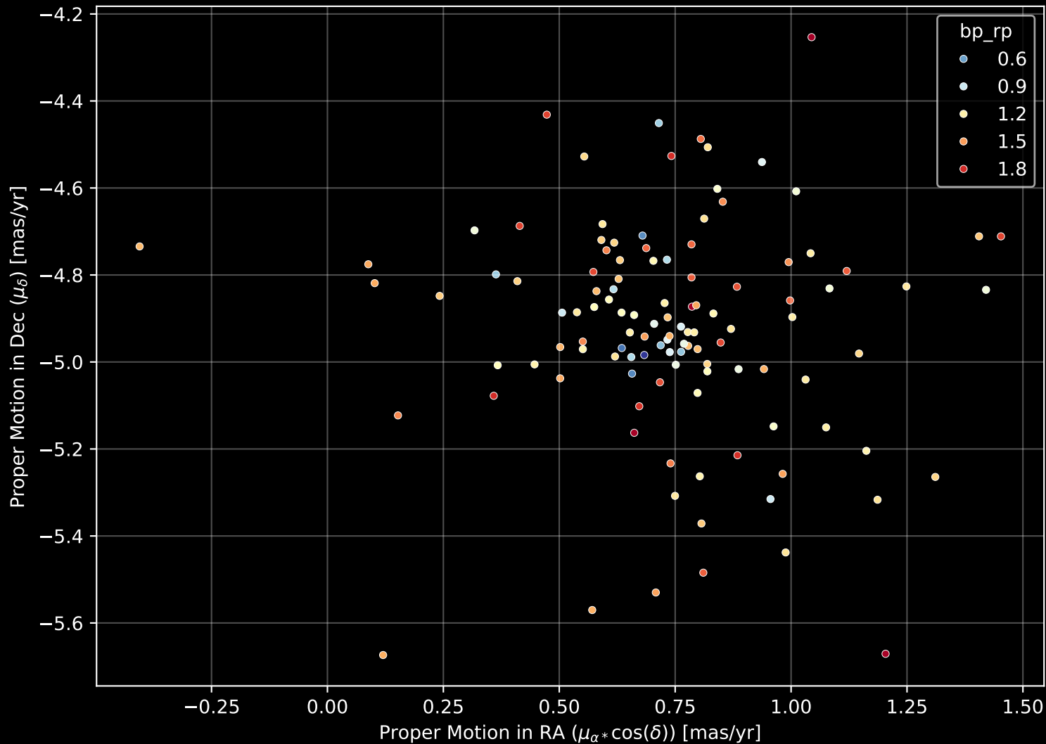
Gaia Cluster: [COIN-Gaia_18] Proper Motion Diagram (n= 115)
