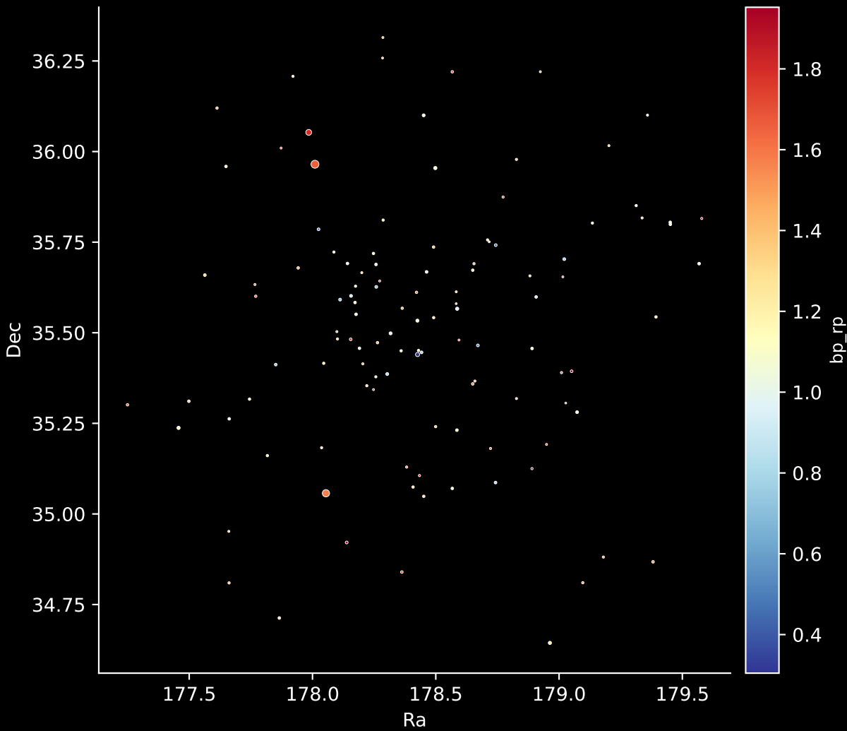
Gaia Cluster: [COIN-Gaia_18] Stars: 115
