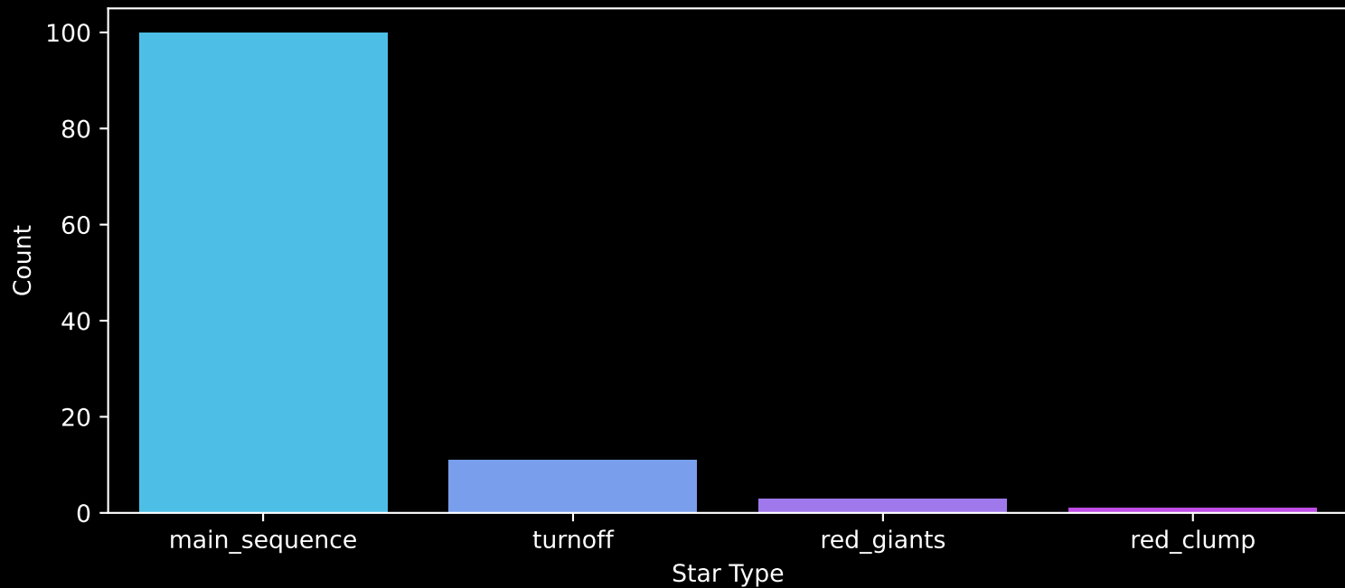
Gaia Cluster: [COIN-Gaia_18] Count plot of Star Type
