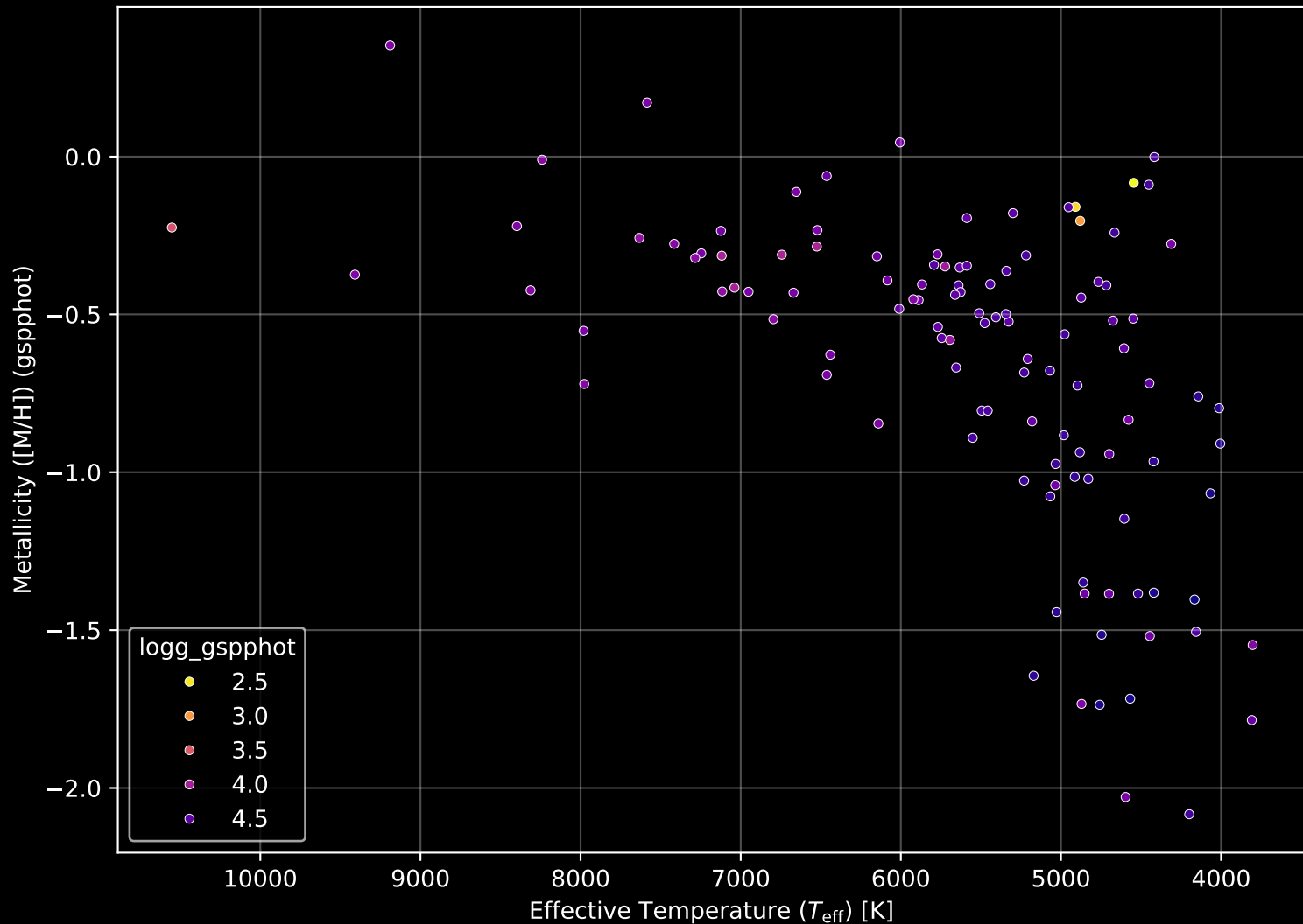
Gaia Cluster: [COIN-Gaia_18] Stellar Population Parameters (n= 115)
