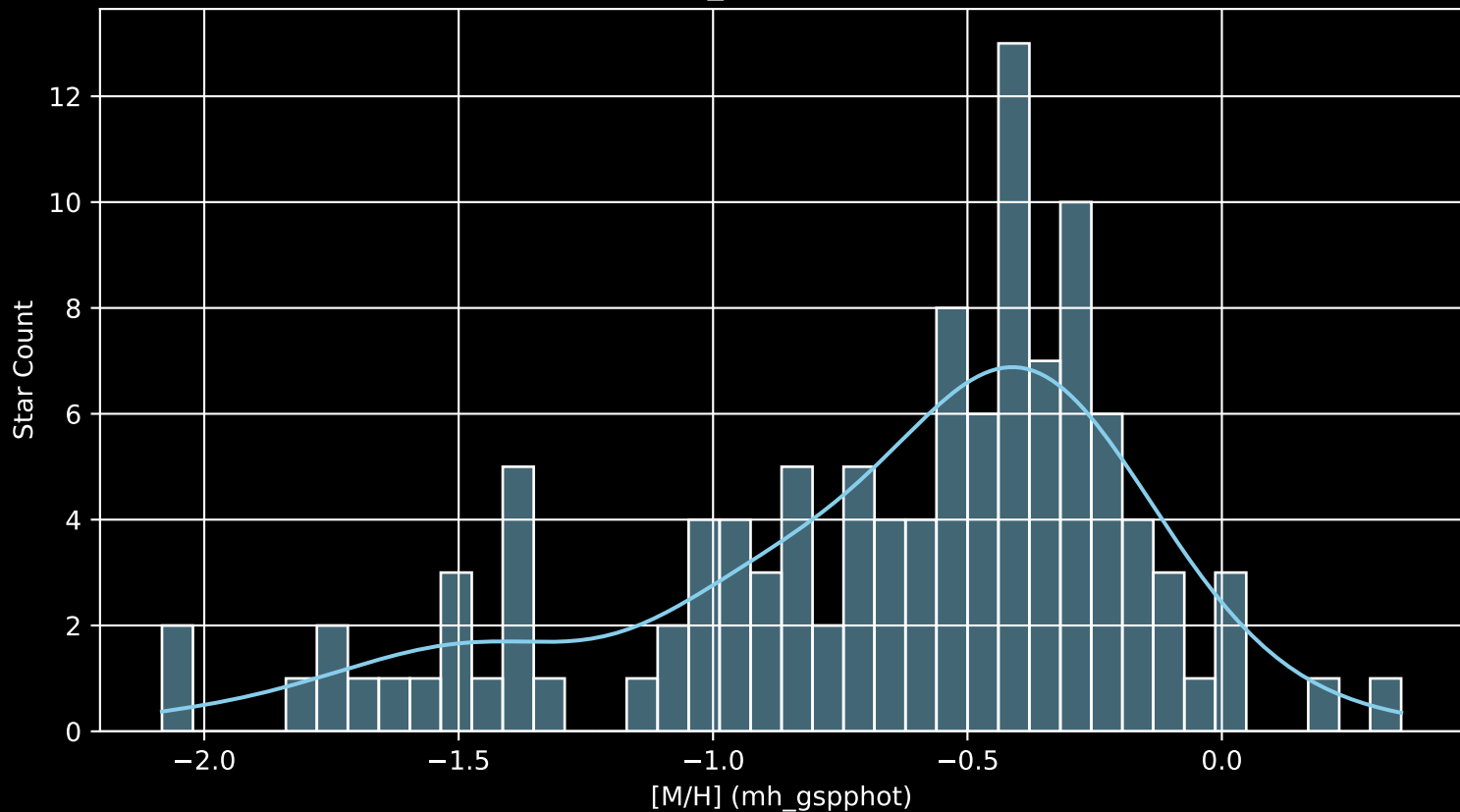
Gaia Cluster: [COIN-Gaia_18 [M/H] (mh_gspphot) (n= 115)
