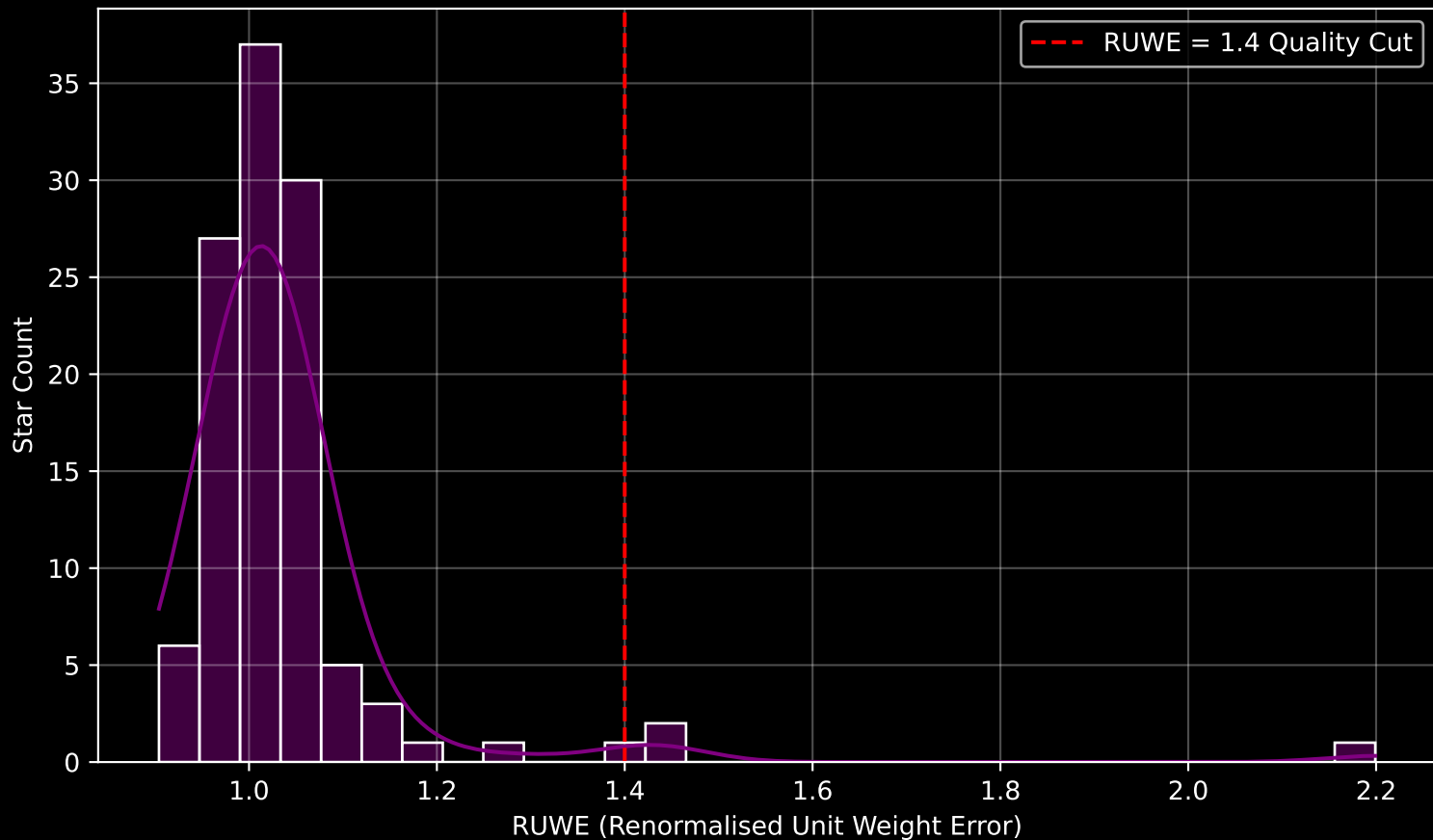
Gaia Cluster: [COIN-Gaia_18] RUWE Distribution (n= 114)
