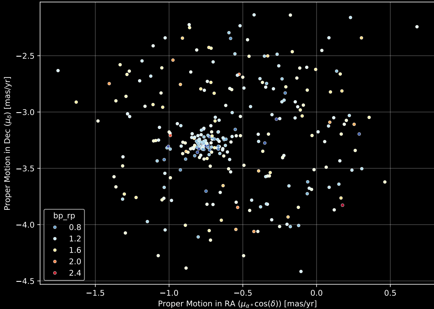
Gaia Cluster: [COIN-Gaia_22] Proper Motion Diagram (n= 302)
