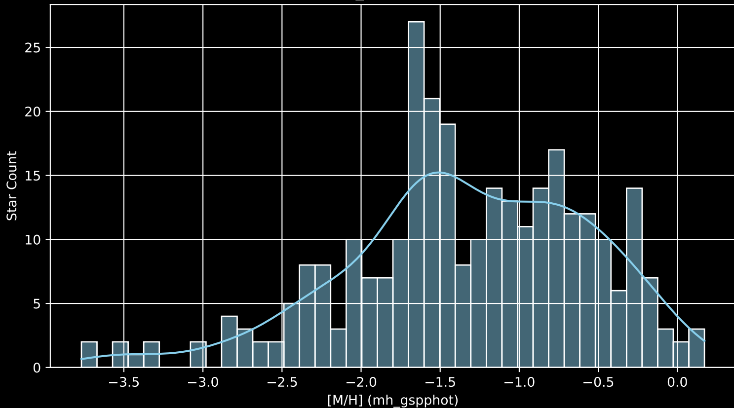
Gaia Cluster: [COIN-Gaia_22 [M/H] (mh_gspphot) (n= 301)
