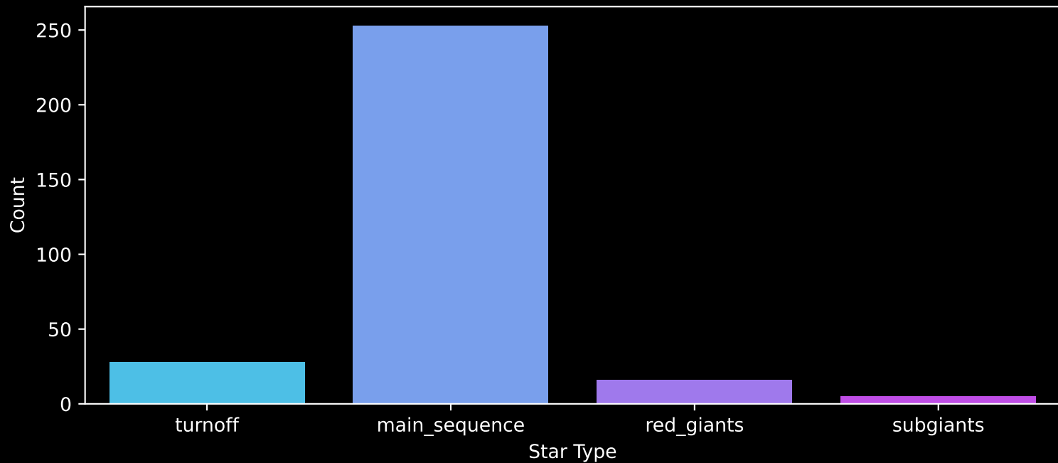
Gaia Cluster: [COIN-Gaia_22] Count plot of Star Type
