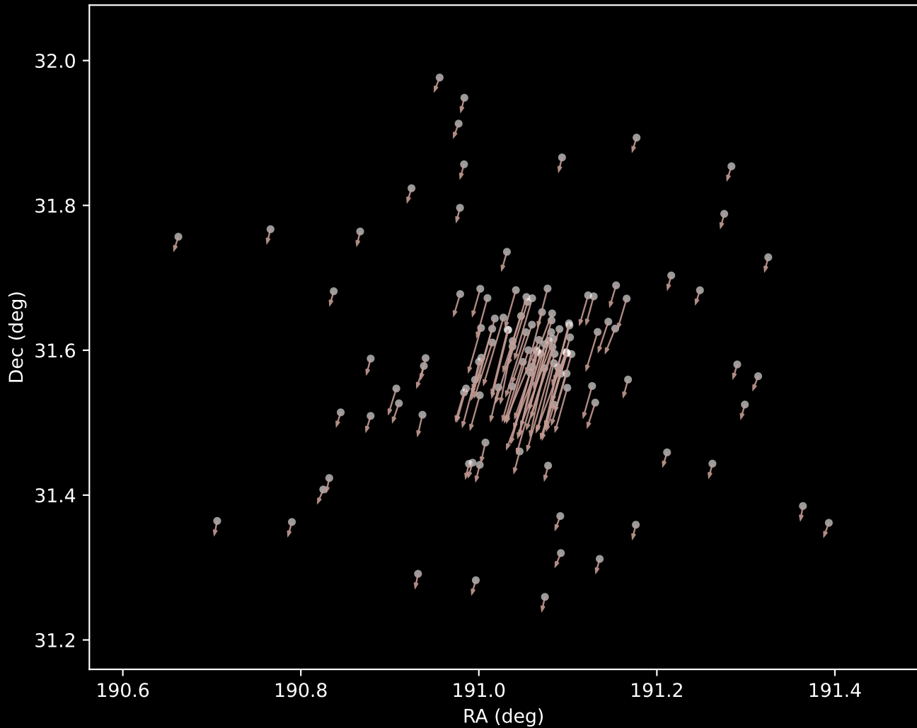
Gaia DR3 Cluster 11 Proper Motion Vectors (n=120)
