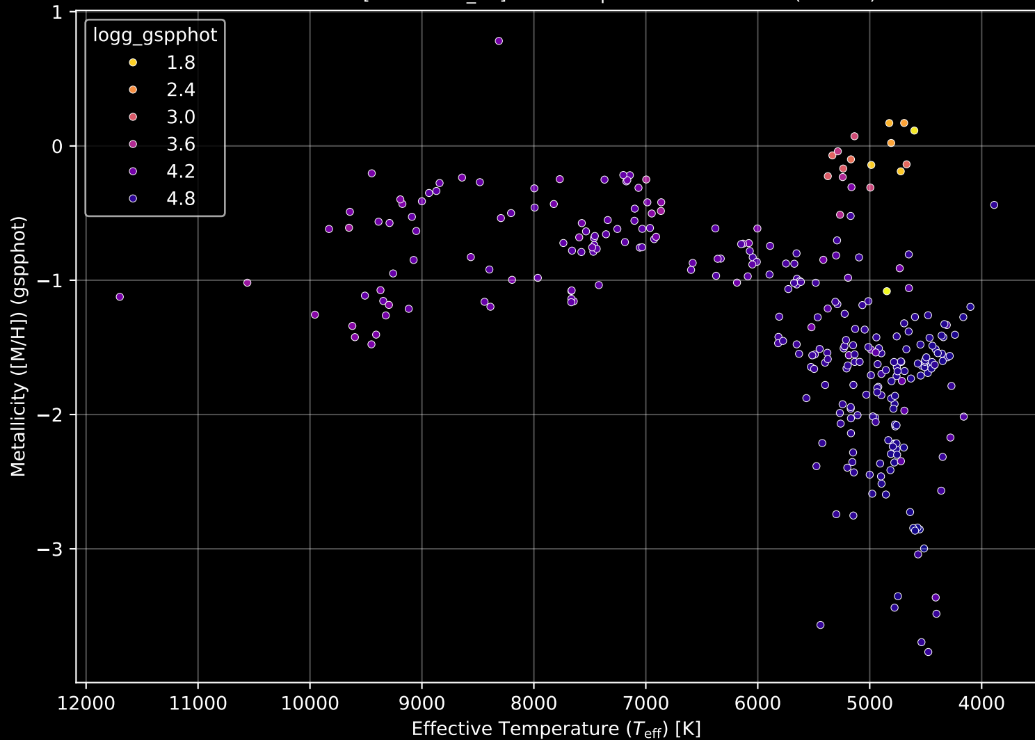
Gaia Cluster: [COIN-Gaia_22] Stellar Population Parameters (n= 302)
