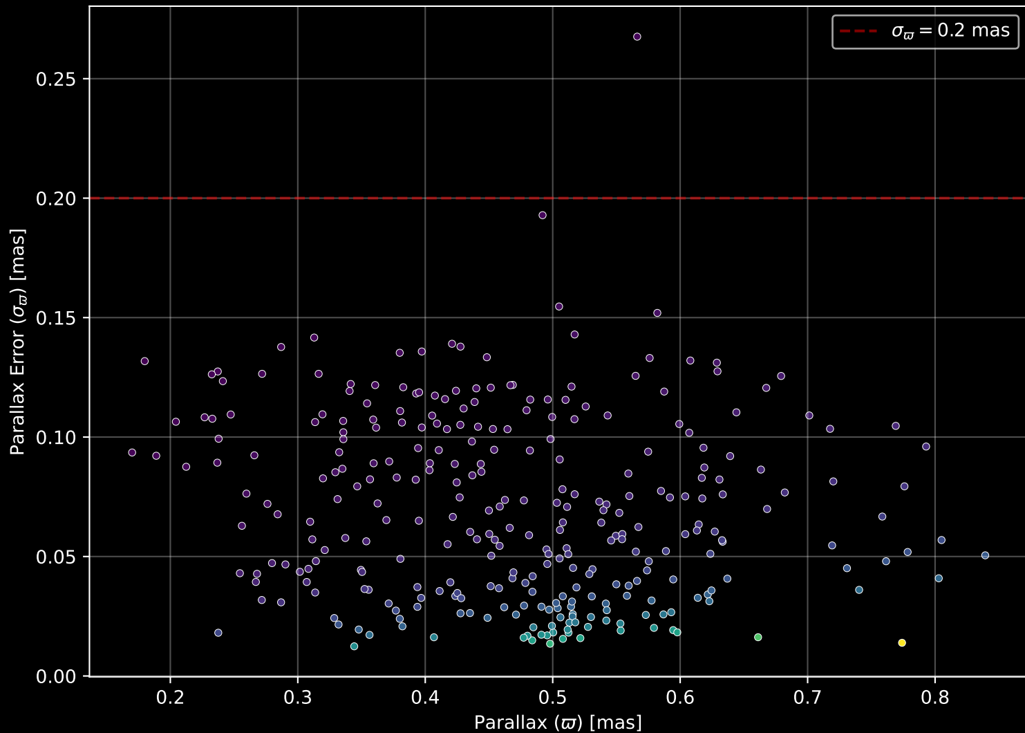
Gaia Cluster: [COIN-Gaia_22] Parallax Quality (n= 302)
