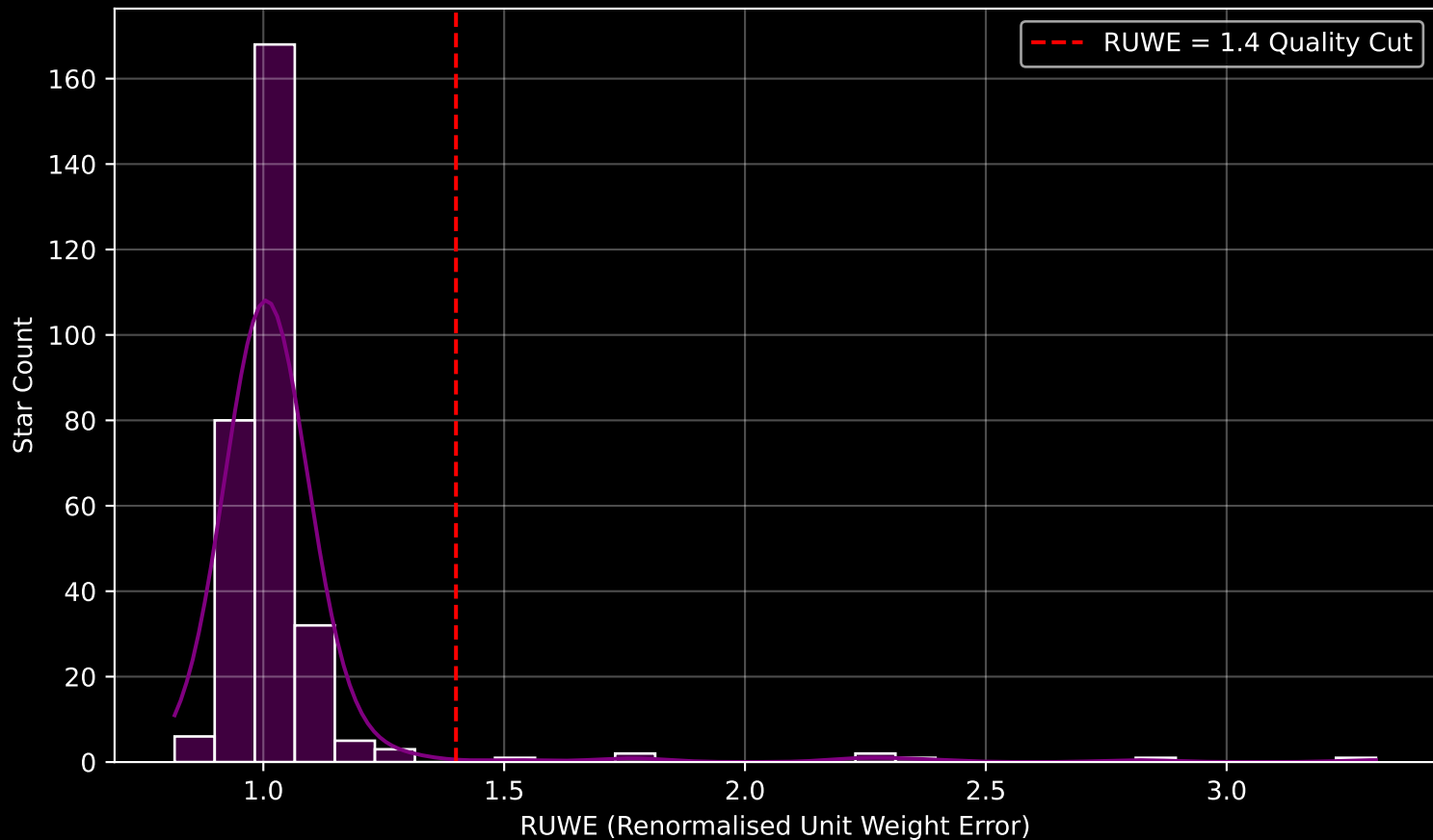
Gaia Cluster: [COIN-Gaia_22] RUWE Distribution (n= 302)
