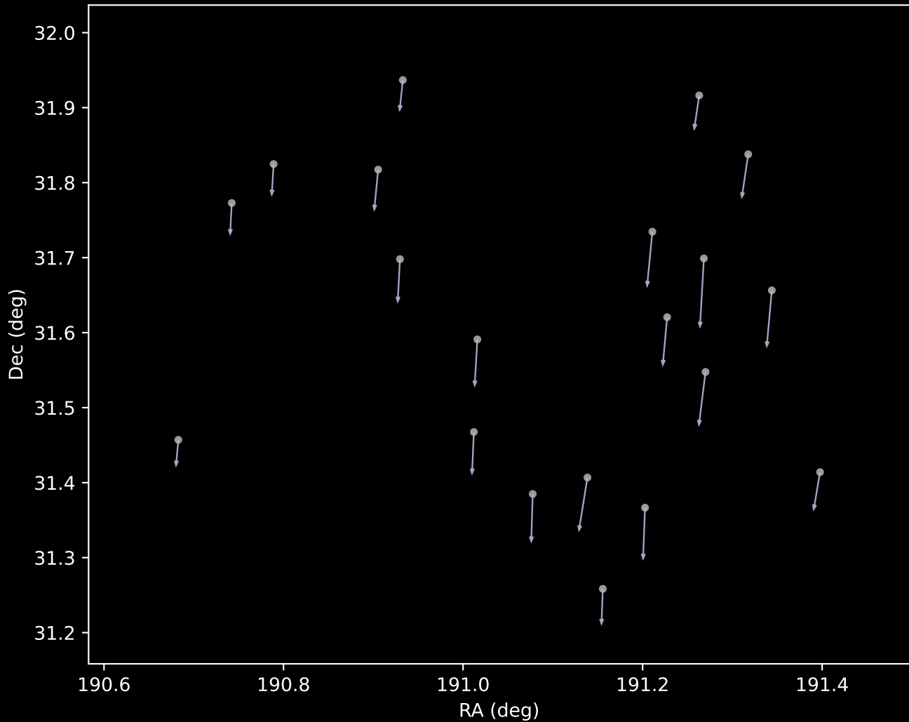
Gaia DR3 Cluster 9 Proper Motion Vectors (n=20)
