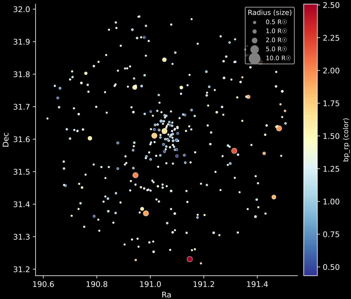
Gaia Cluster: [COIN-Gaia_22] Stars: 302
