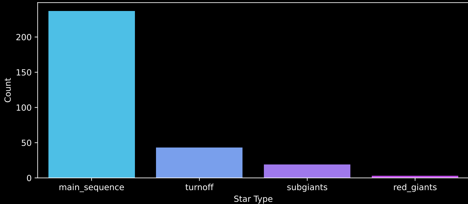
Gaia Cluster: [COIN-Gaia_23] Count plot of Star Type
