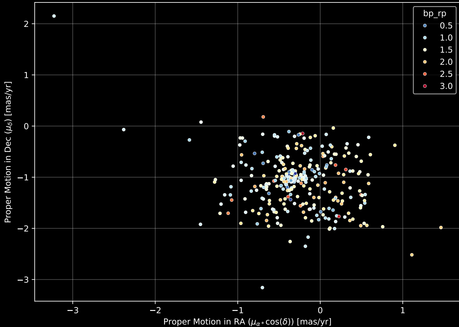
Gaia Cluster: [COIN-Gaia_23] Proper Motion Diagram (n= 302)
