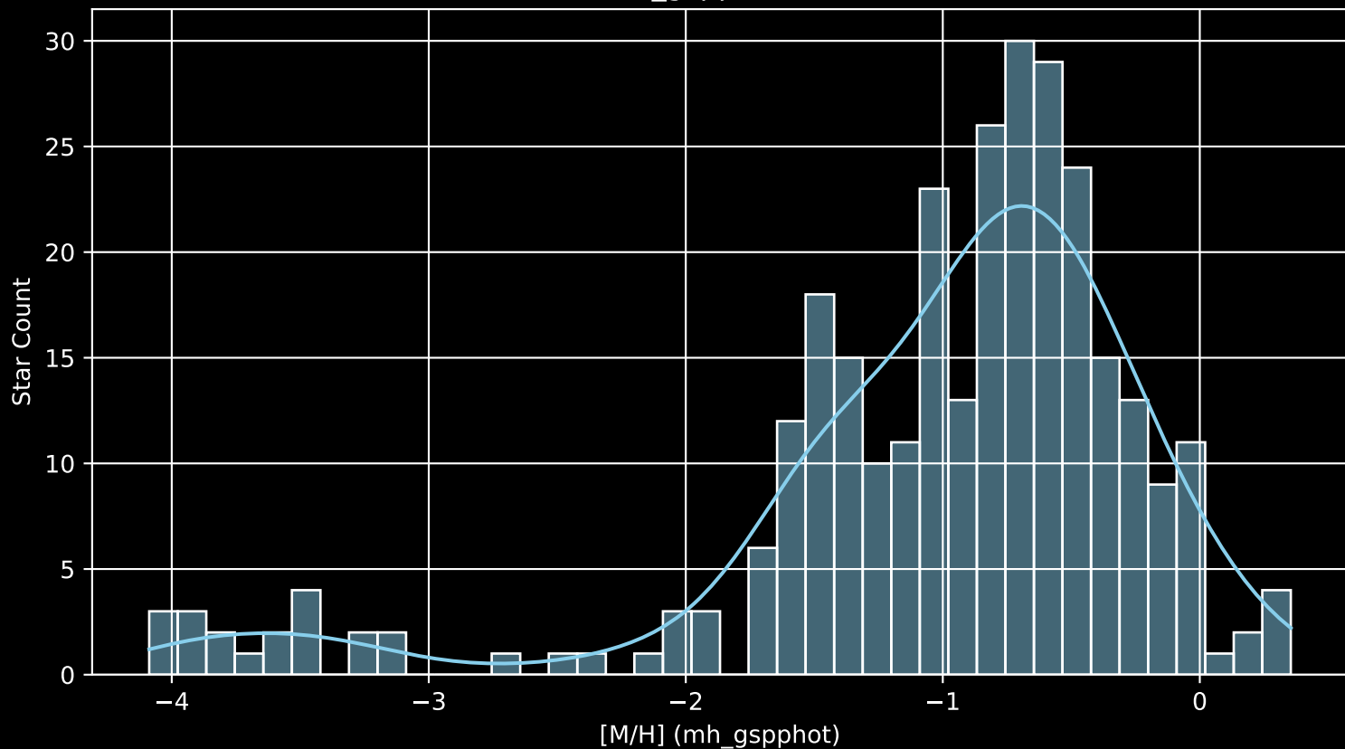
Gaia Cluster: [COIN-Gaia_23 [M/H] (mh_gspphot) (n= 301)
