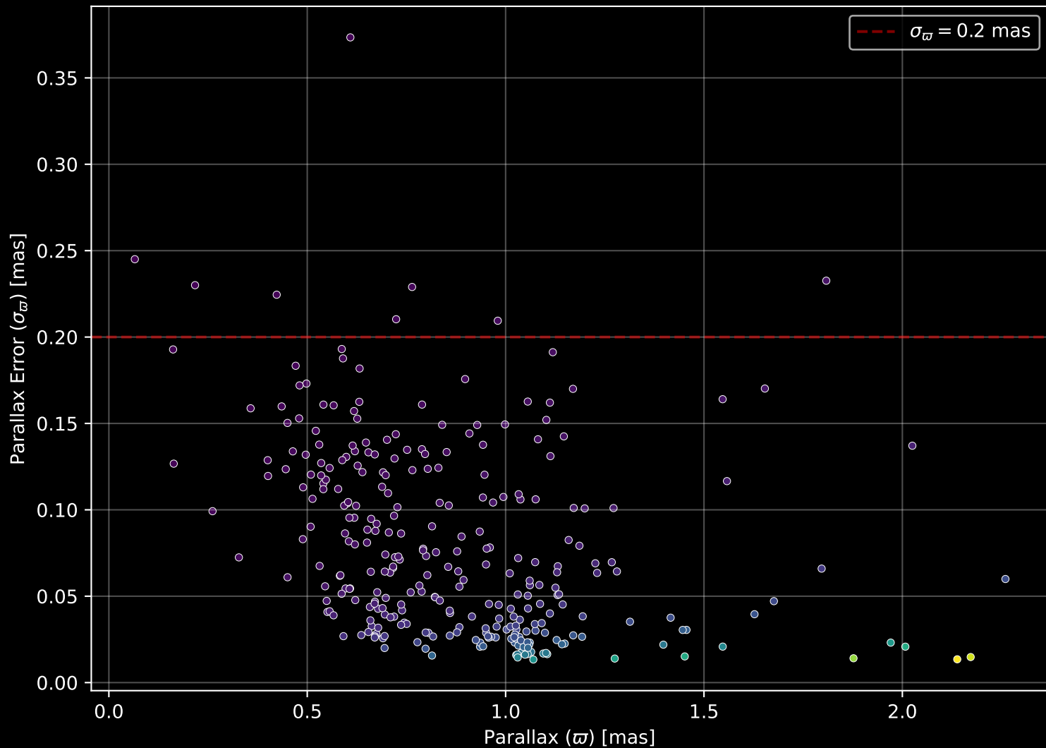
Gaia Cluster: [COIN-Gaia_23] Parallax Quality (n= 302)
