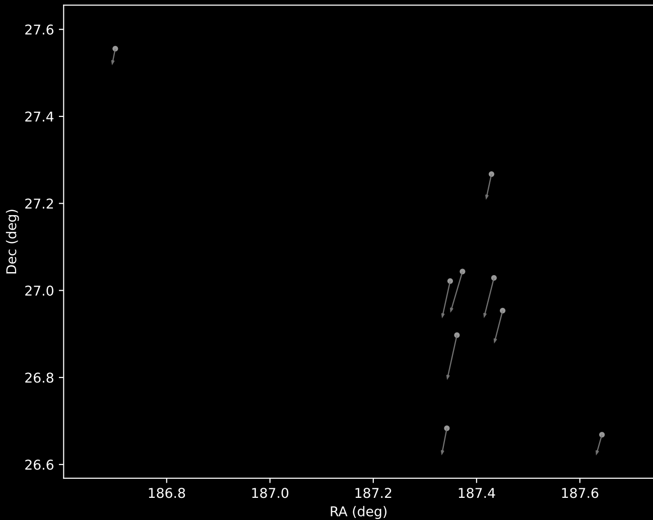
Gaia DR3 Cluster 14 Proper Motion Vectors (n=9)
