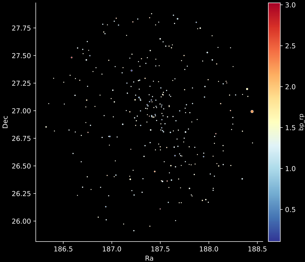
Gaia Cluster: [COIN-Gaia_23] Stars: 302
