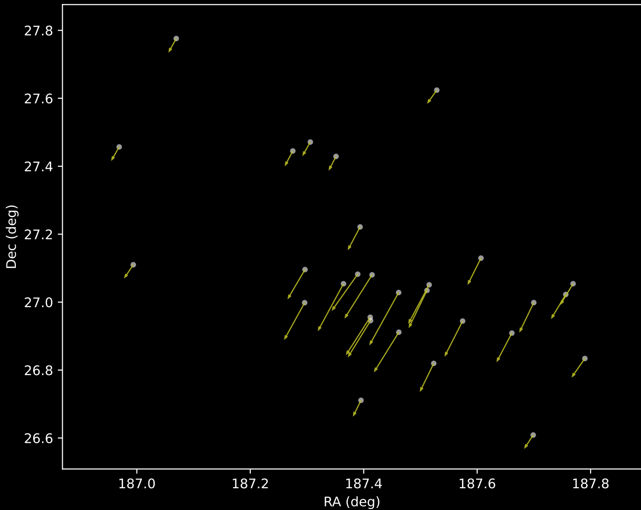
Gaia DR3 Cluster 16 Proper Motion Vectors (n=29)
