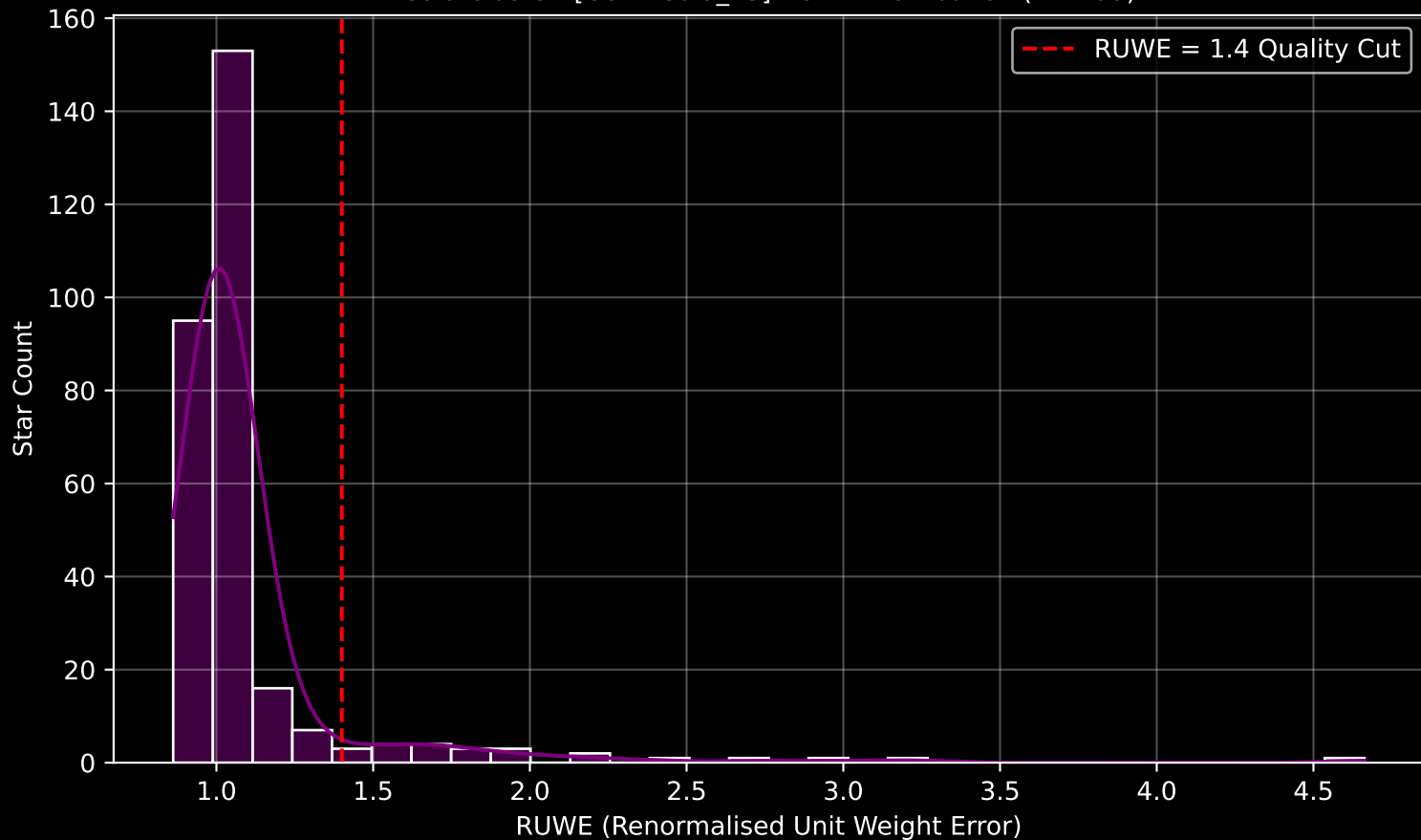
Gaia Cluster: [COIN-Gaia_23] RUWE Distribution (n= 295)
