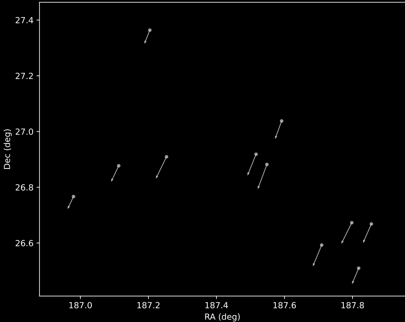
Gaia DR3 Cluster 15 Proper Motion Vectors (n=11)
