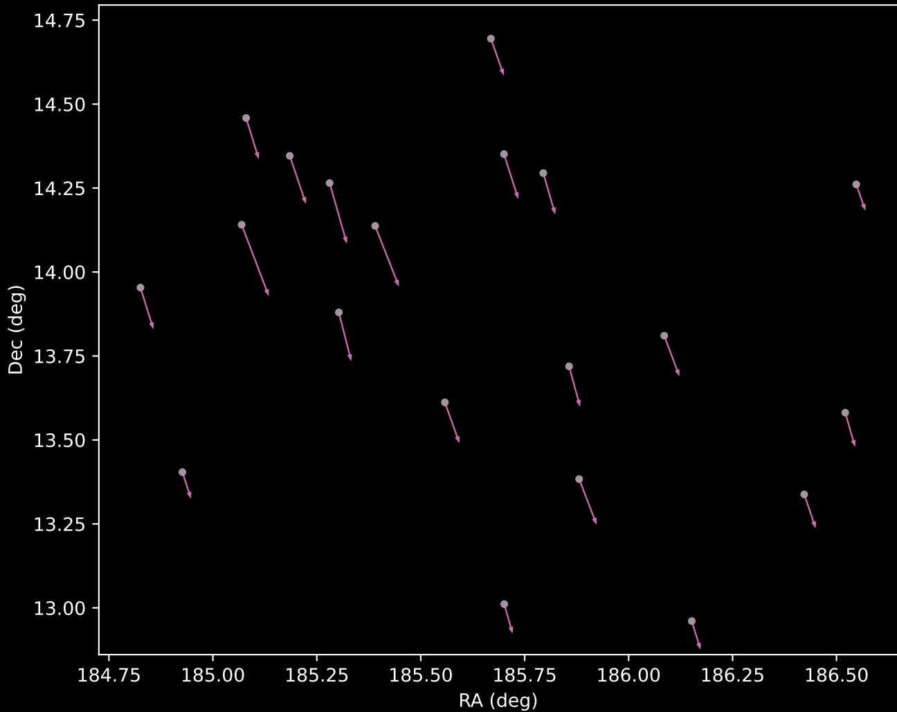
Gaia DR3 Cluster 12 Proper Motion Vectors (n=20)
