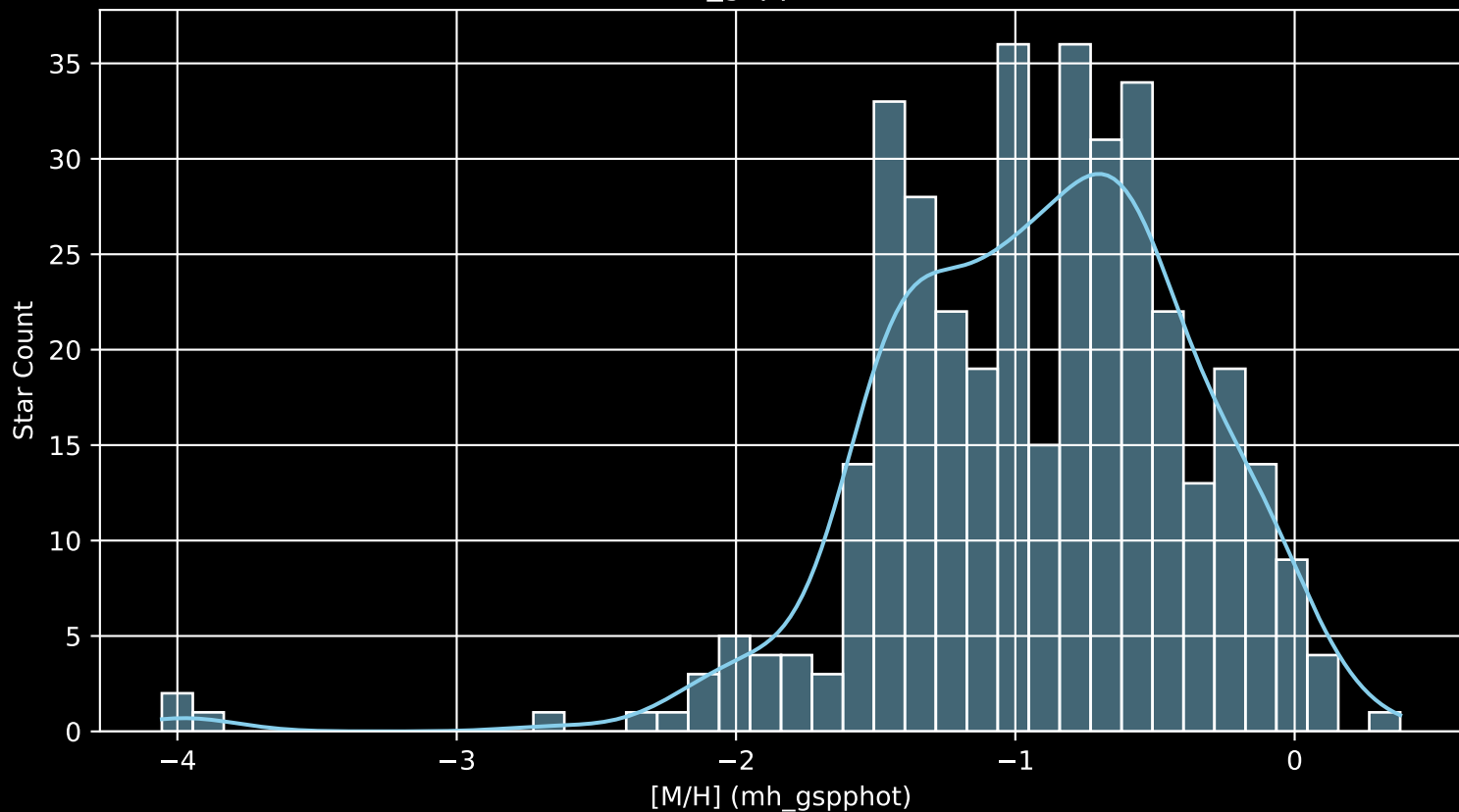
Gaia Cluster: [COIN-Gaia_27 [M/H] (mh_gspphot) (n= 375)
