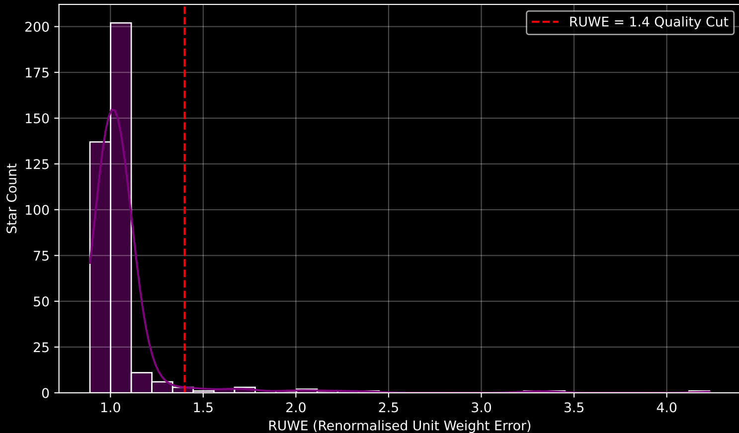
Gaia Cluster: [COIN-Gaia_27] RUWE Distribution (n= 374)
