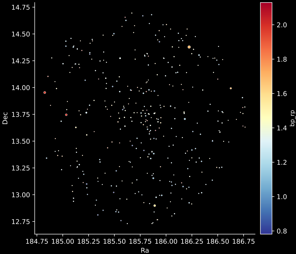
Gaia Cluster: [COIN-Gaia_27] Stars: 375
