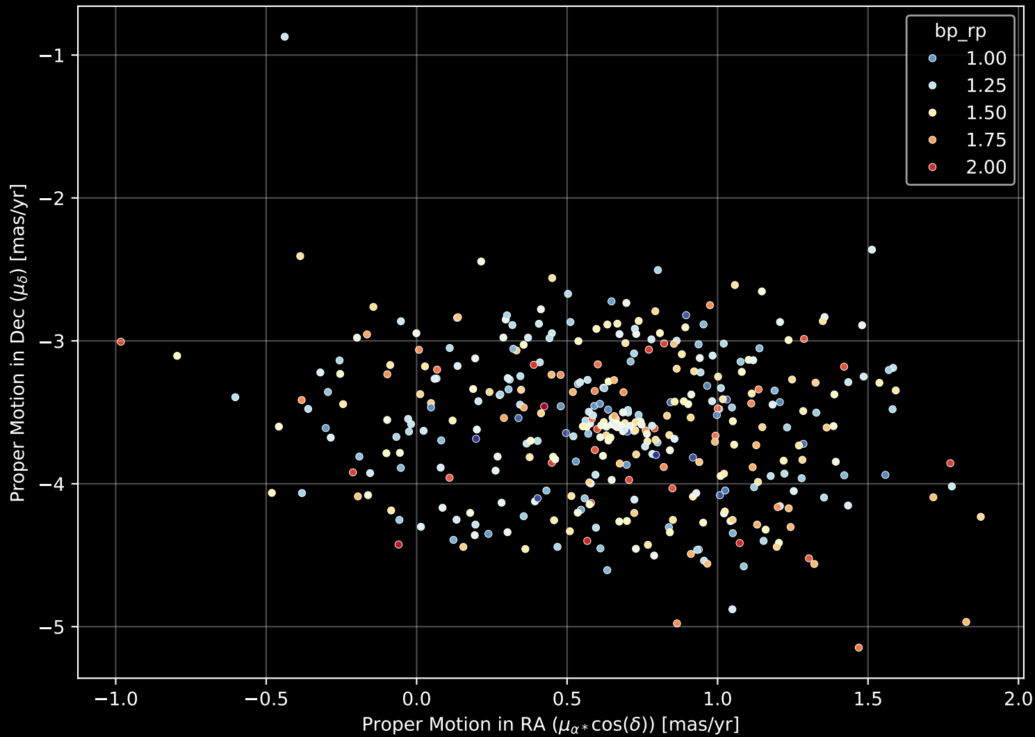
Gaia Cluster: [COIN-Gaia_27] Proper Motion Diagram (n= 375)
