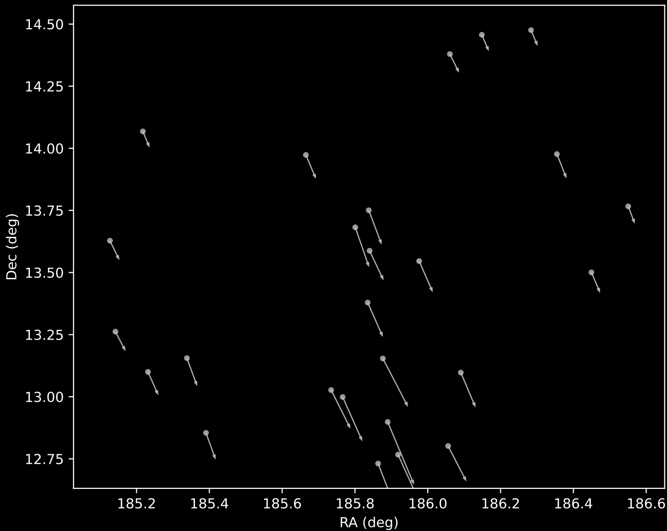
Gaia DR3 Cluster 15 Proper Motion Vectors (n=26)
