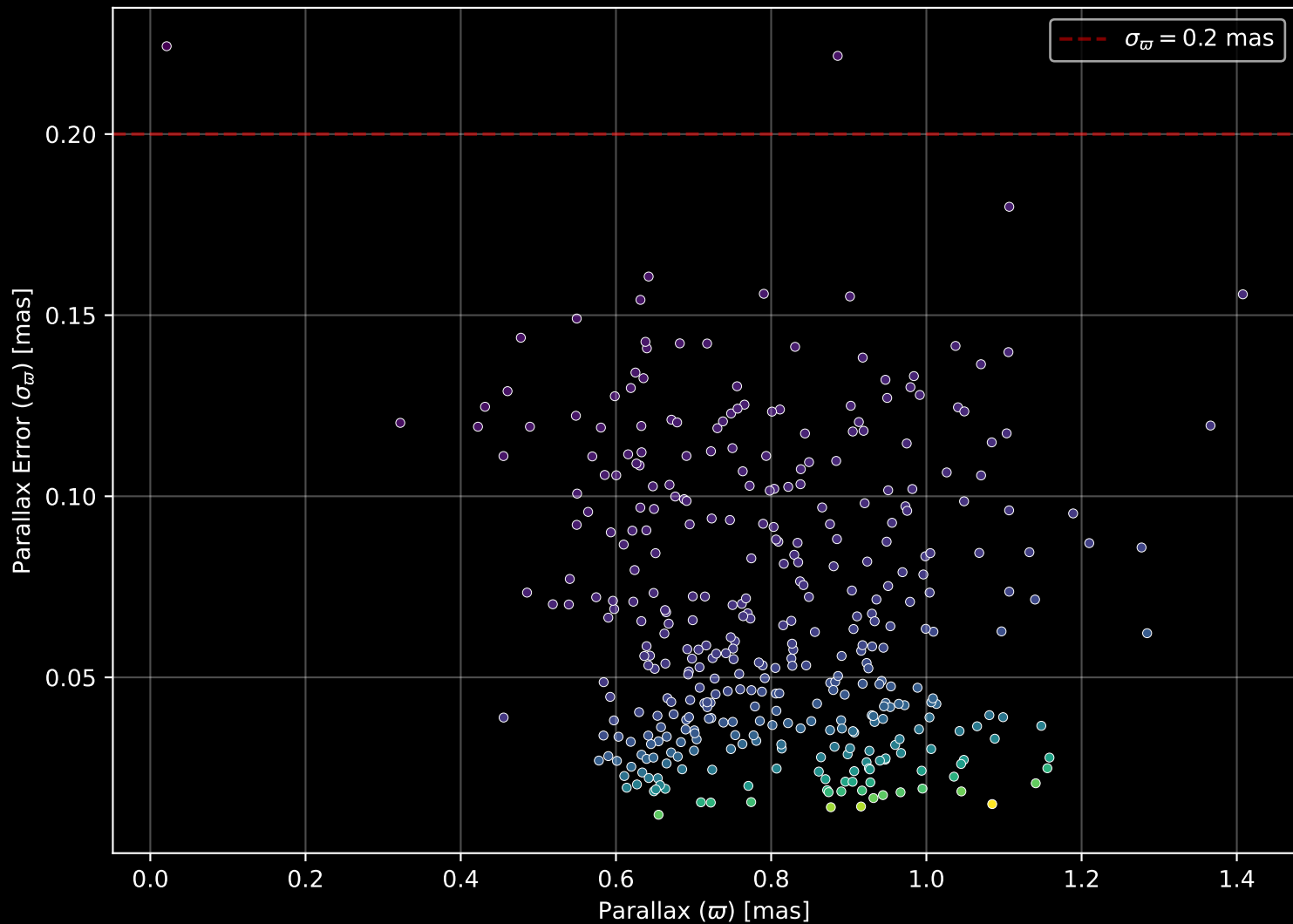
Gaia Cluster: [COIN-Gaia_27] Parallax Quality (n= 375)
