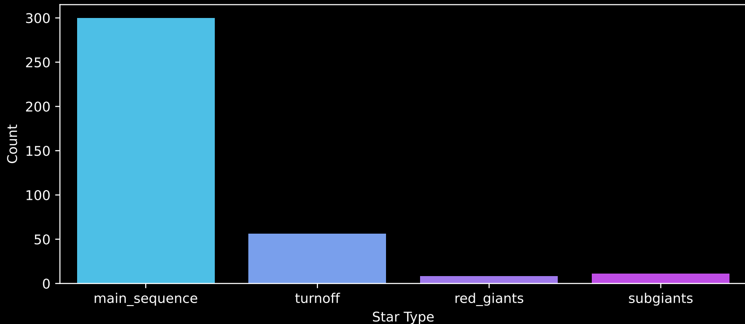
Gaia Cluster: [COIN-Gaia_27] Count plot of Star Type
