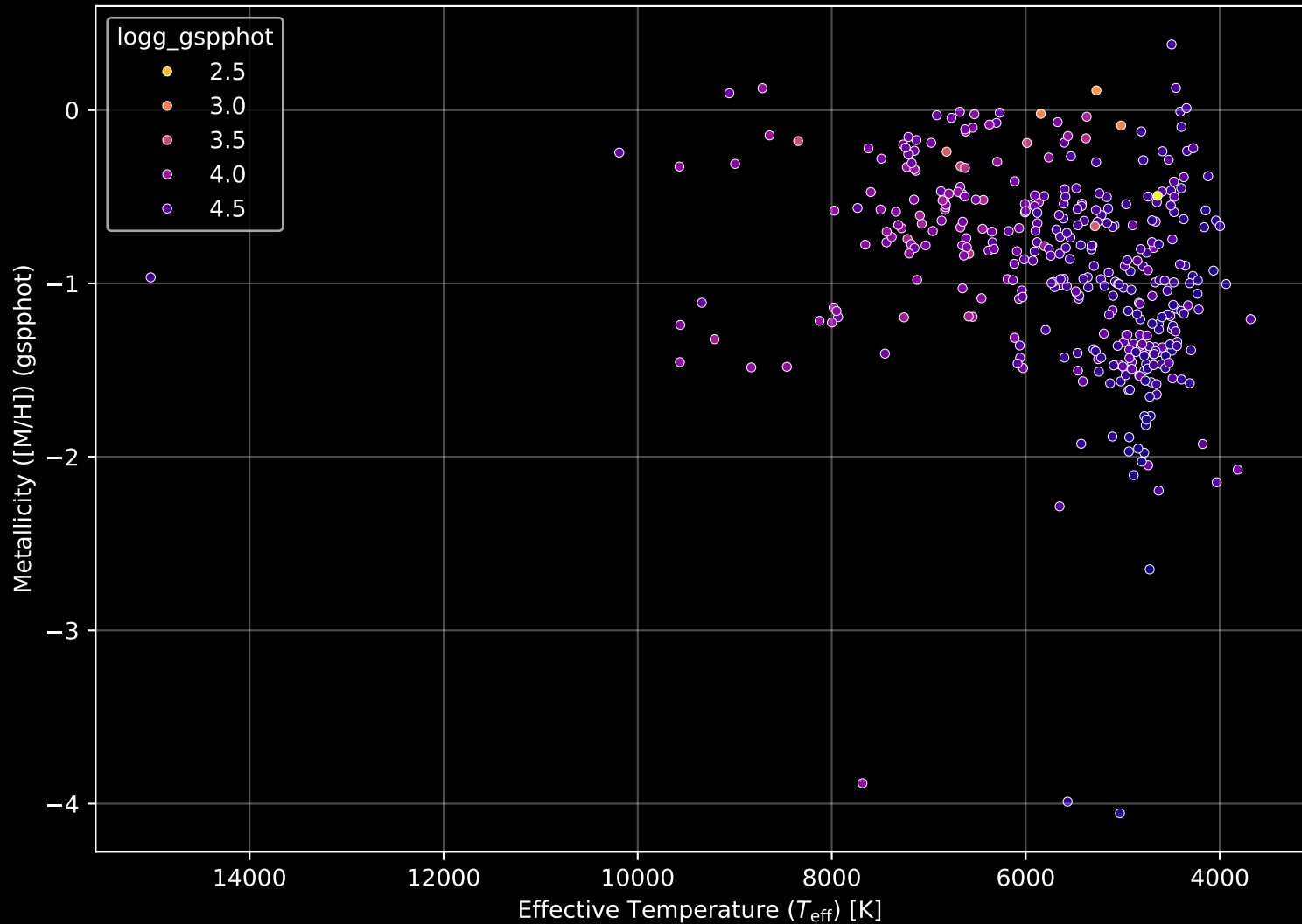
Gaia Cluster: [COIN-Gaia_27] Stellar Population Parameters (n= 375)
