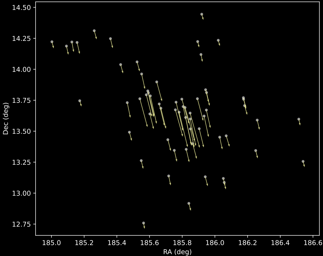
Gaia DR3 Cluster 17 Proper Motion Vectors (n=61)
