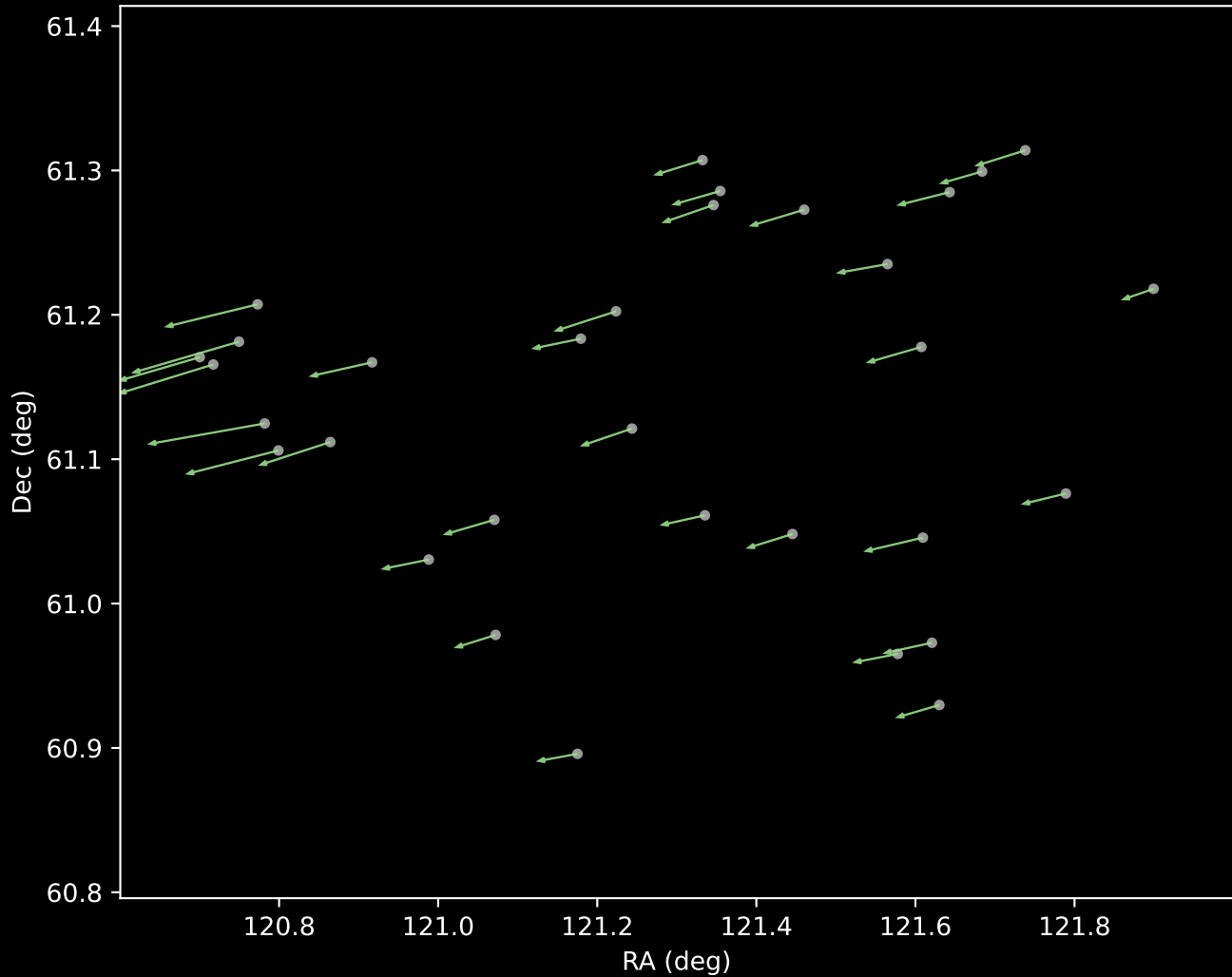
Gaia DR3 Cluster 5 Proper Motion Vectors (n=32)
