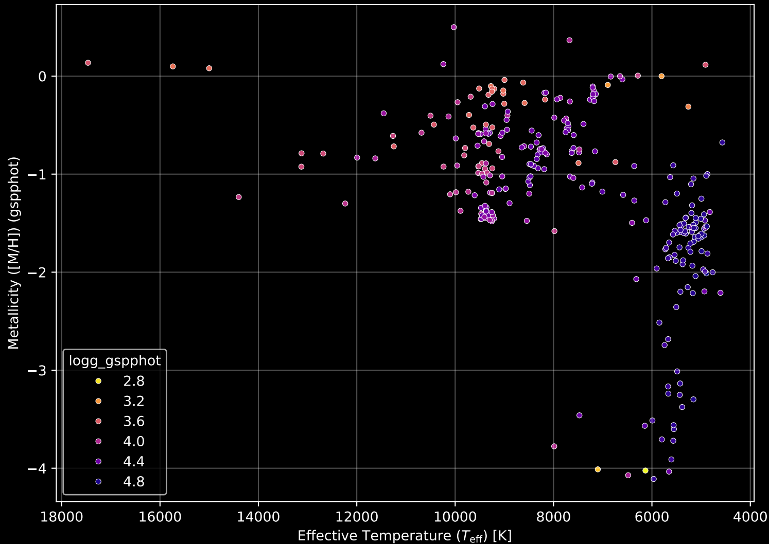
Gaia Cluster: [COIN-Gaia_31] Stellar Population Parameters (n= 294)
