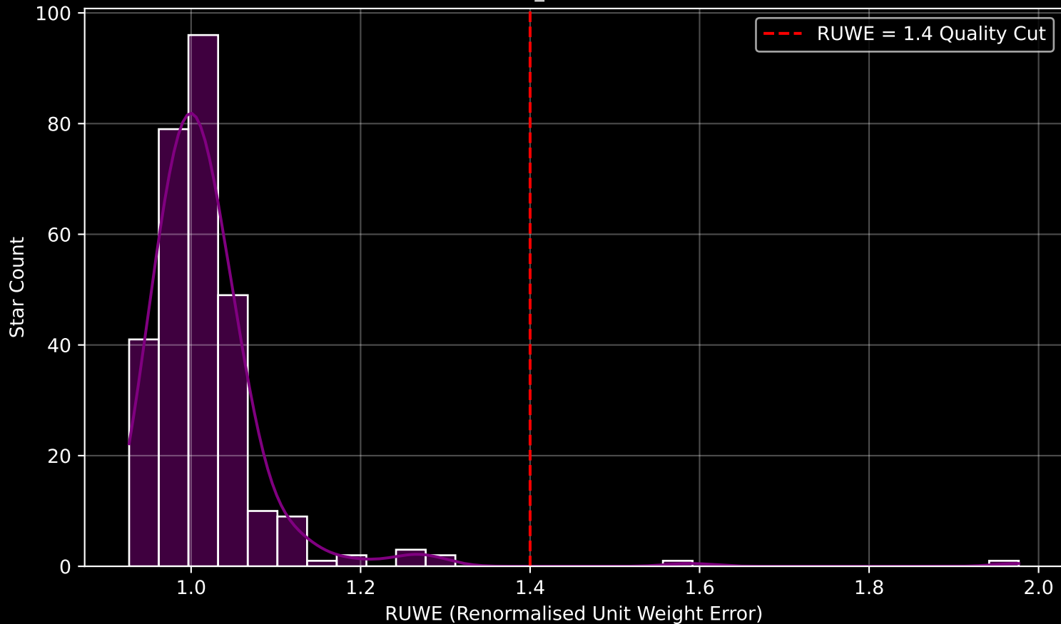
Gaia Cluster: [COIN-Gaia_31] RUWE Distribution (n= 294)
