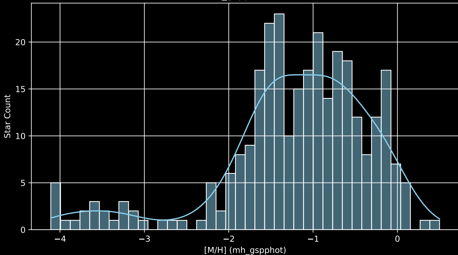
Gaia Cluster: [COIN-Gaia_31 [M/H] (mh_gspphot) (n= 294)
