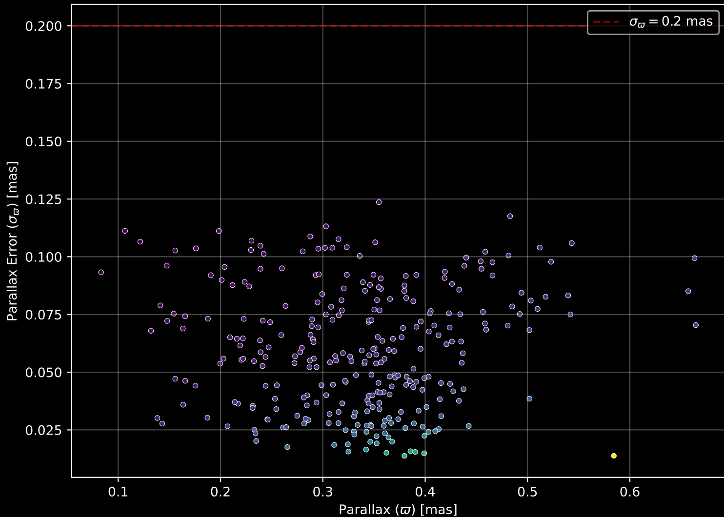
Gaia Cluster: [COIN-Gaia_31] Parallax Quality (n= 294)
