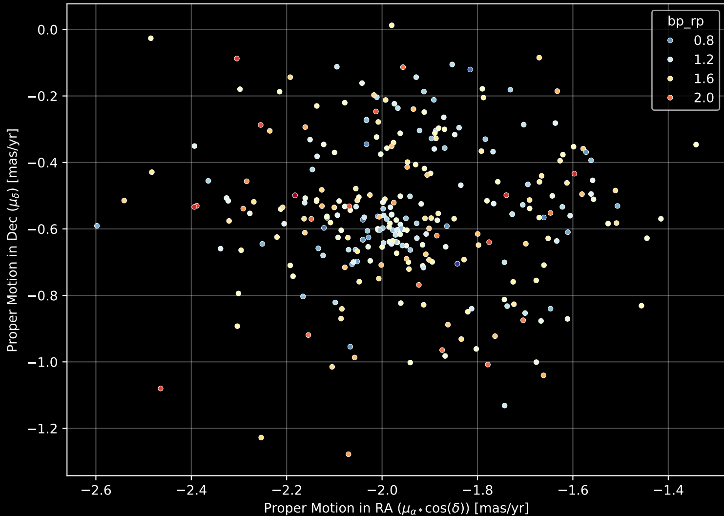
Gaia Cluster: [COIN-Gaia_31] Proper Motion Diagram (n= 294)
