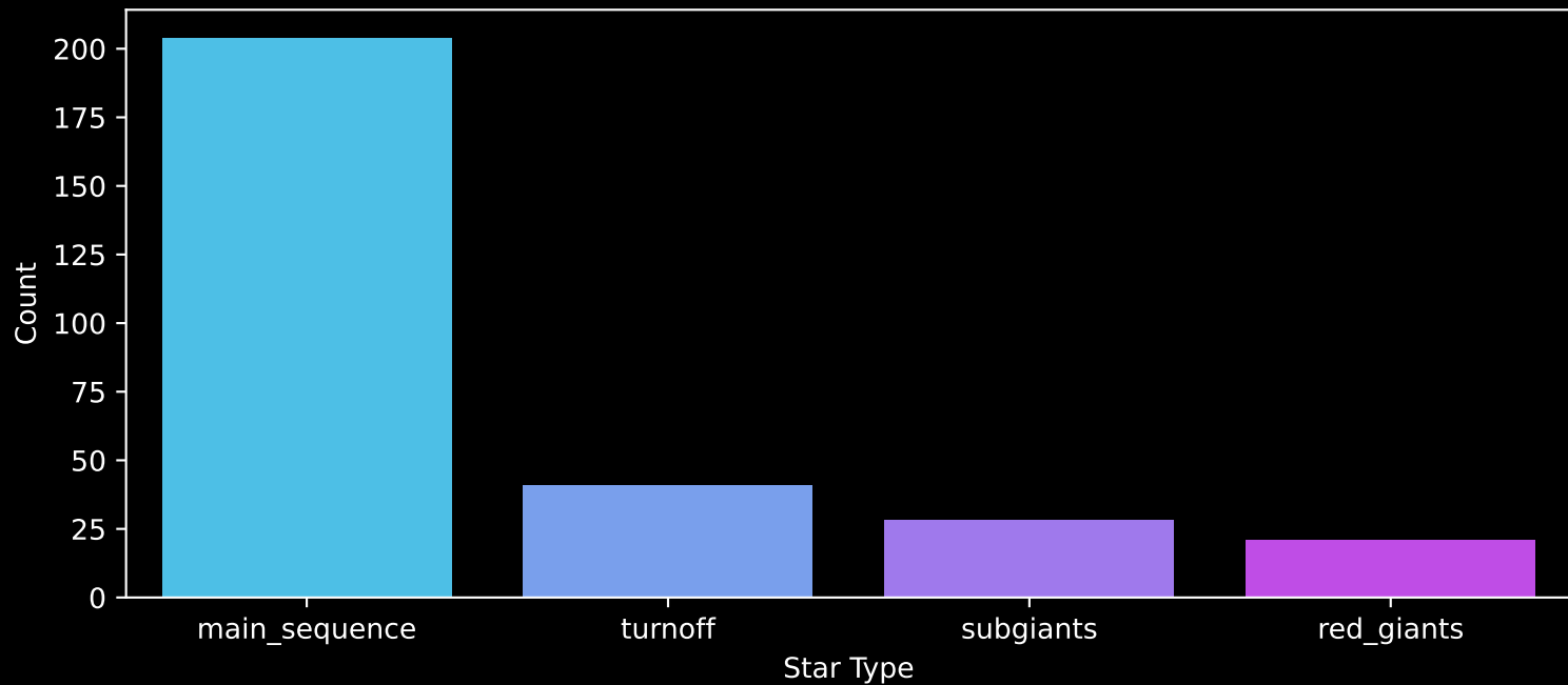
Gaia Cluster: [COIN-Gaia_31] Count plot of Star Type
