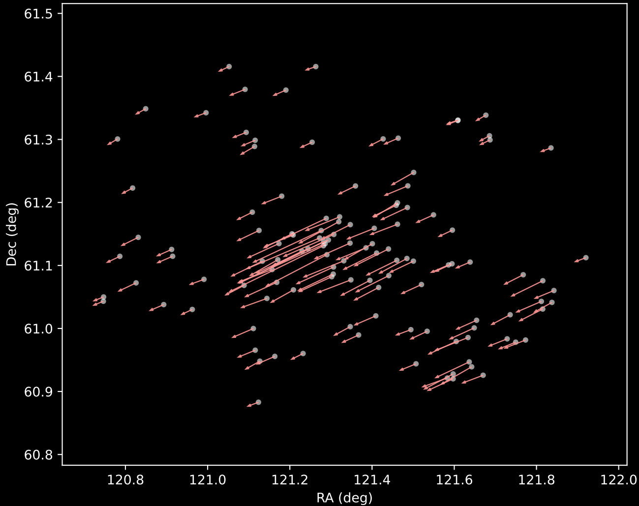
Gaia DR3 Cluster 7 Proper Motion Vectors (n=120)
