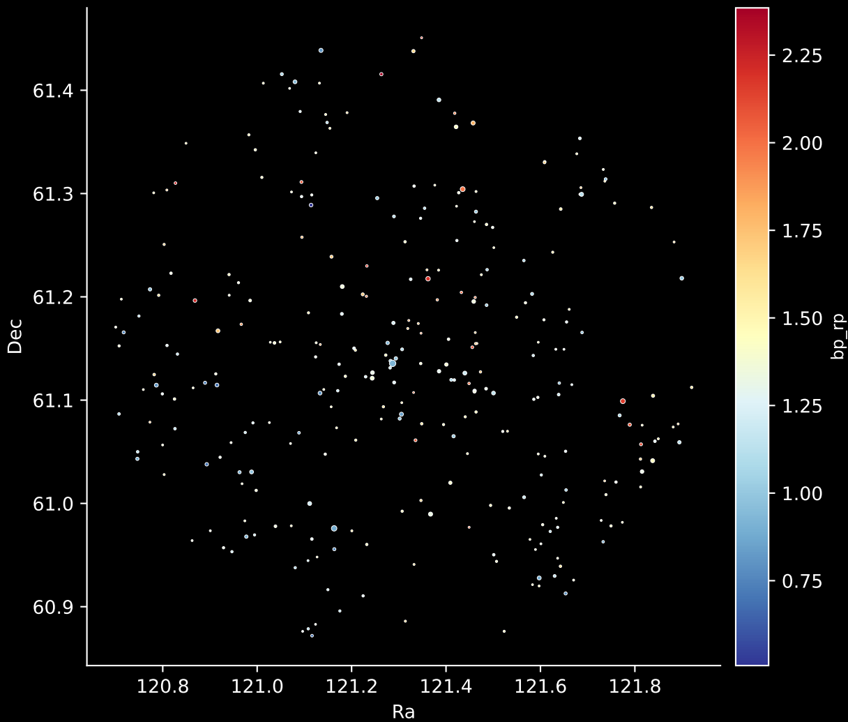
Gaia Cluster: [COIN-Gaia_31] Stars: 294
