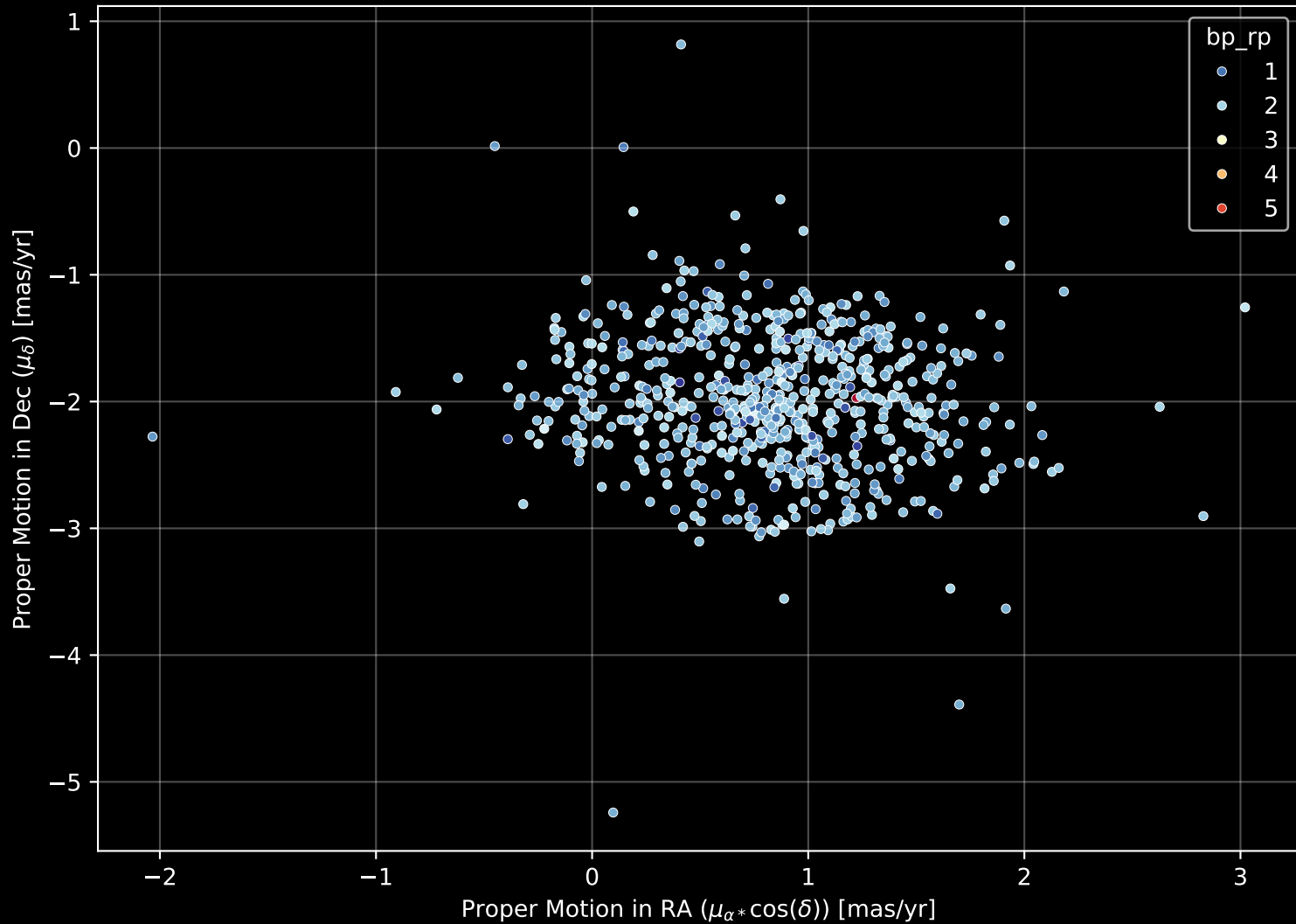
Gaia Cluster: [COIN-Gaia_37] Proper Motion Diagram (n= 685)
