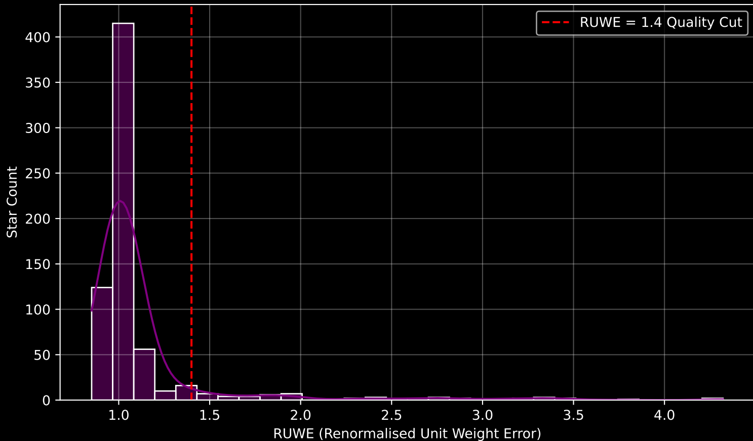
Gaia Cluster: [COIN-Gaia_37] RUWE Distribution (n= 673)
