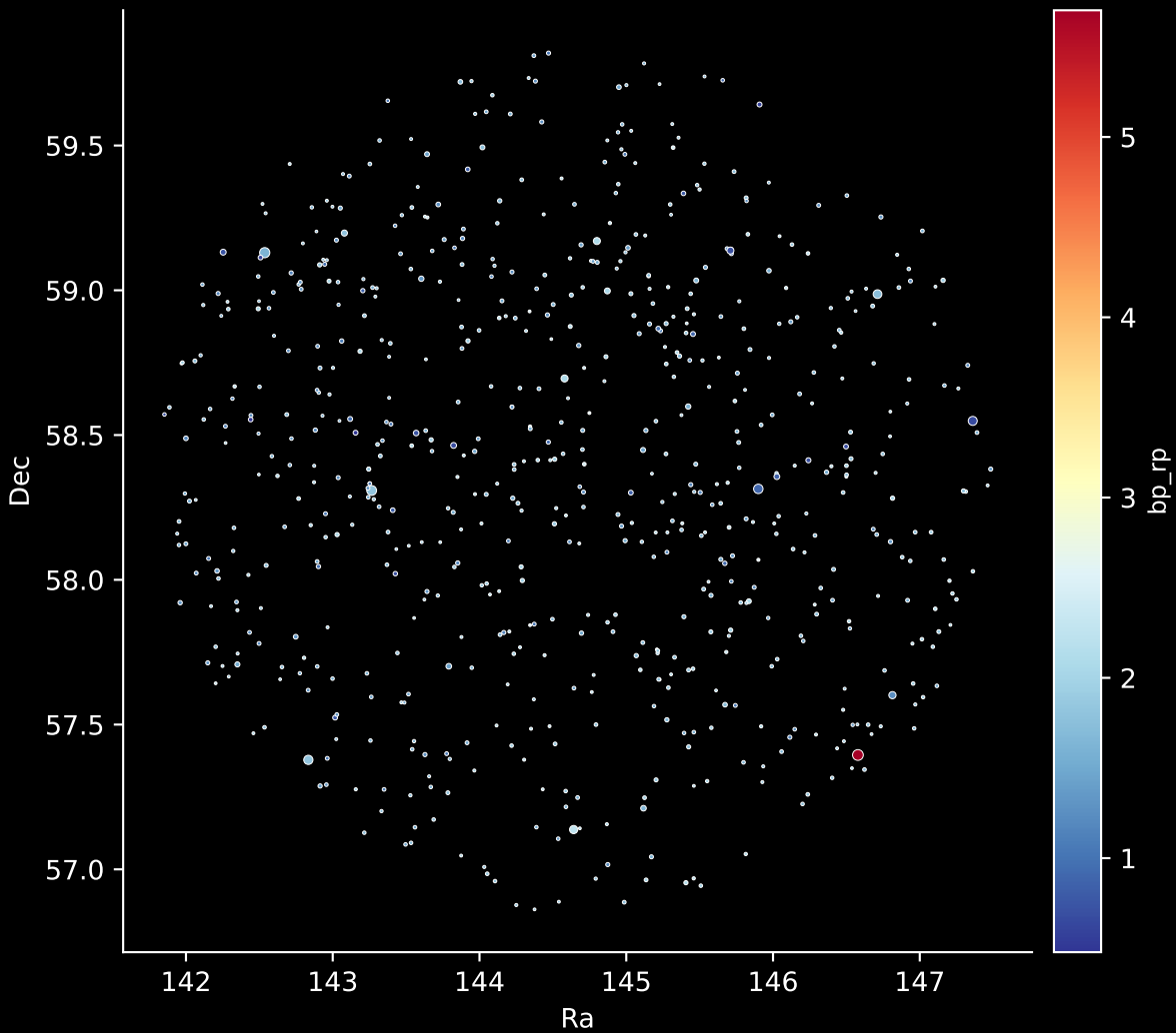
Gaia Cluster: [COIN-Gaia_37] Stars: 685
