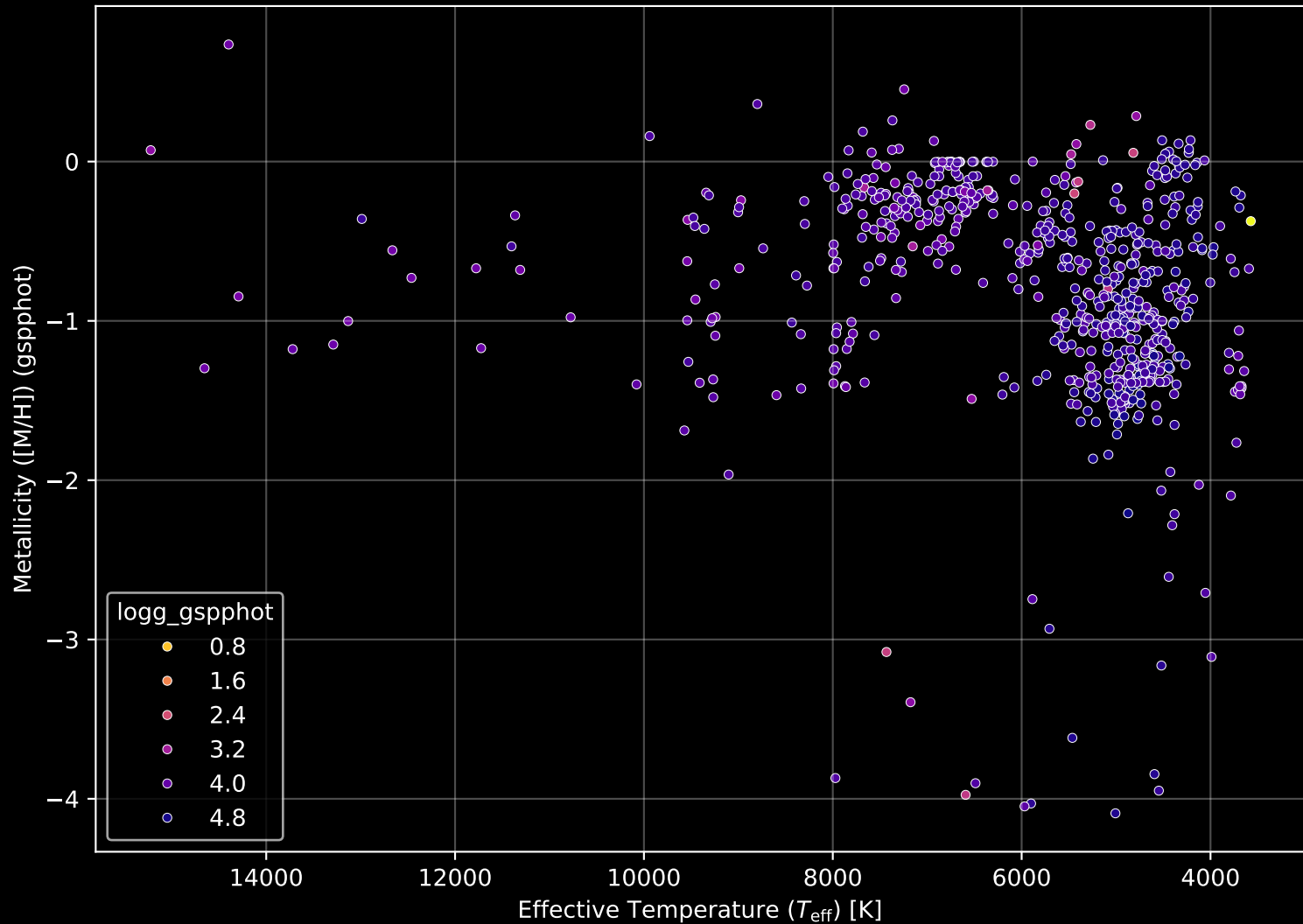
Gaia Cluster: [COIN-Gaia_37] Stellar Population Parameters (n= 685)
