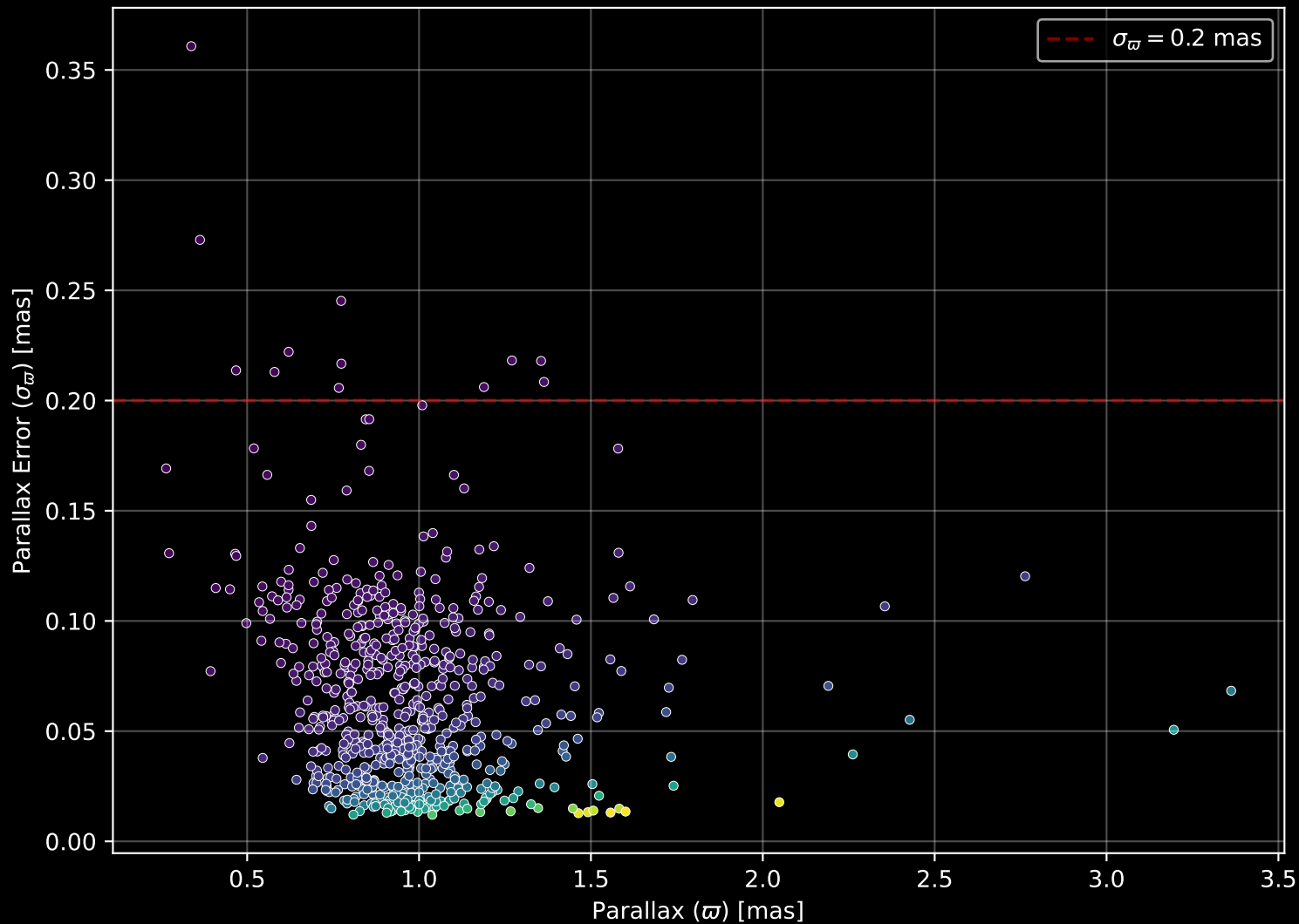
Gaia Cluster: [COIN-Gaia_37] Parallax Quality (n= 685)
