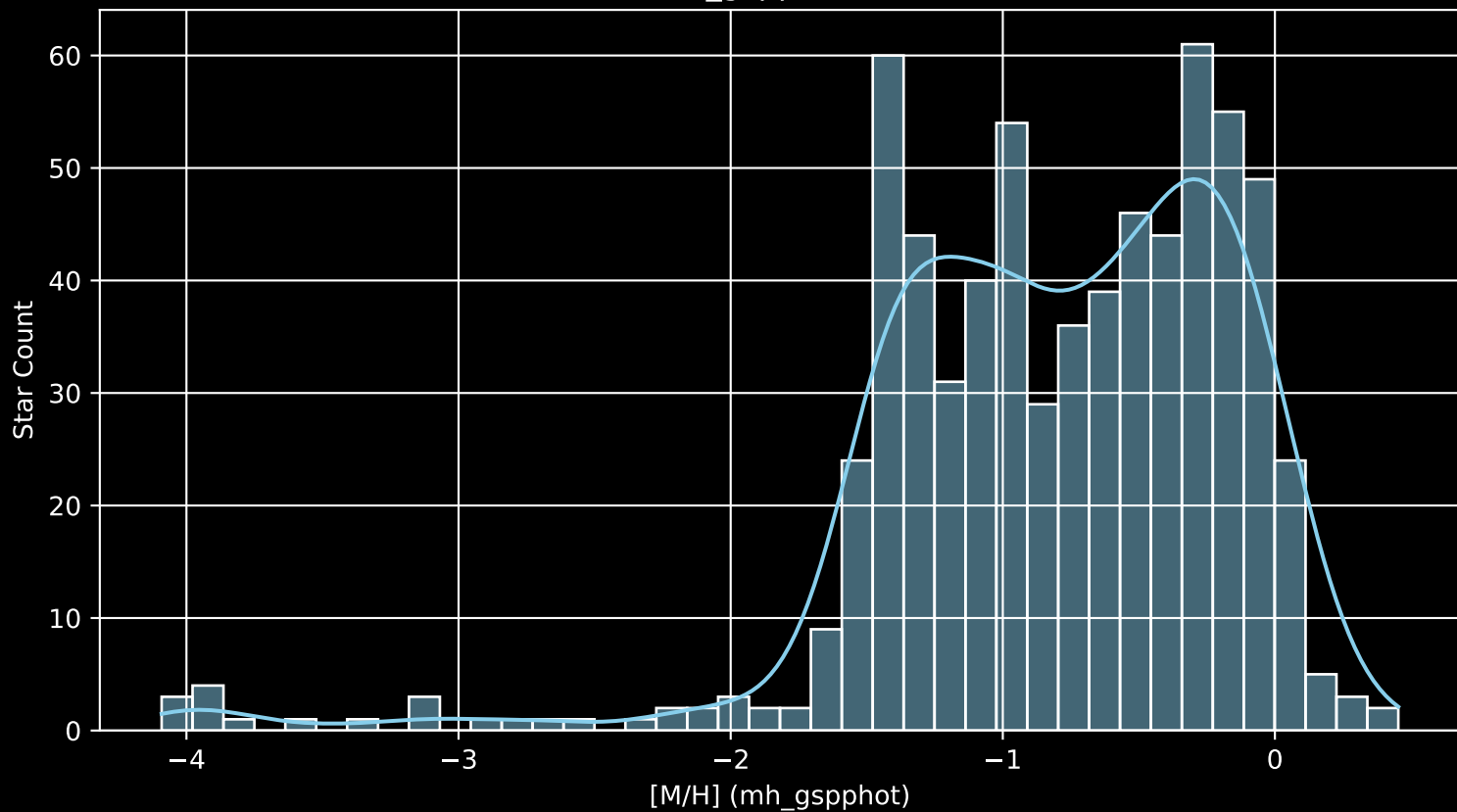
Gaia Cluster: [COIN-Gaia_37 [M/H] (mh_gspphot) (n= 684)
