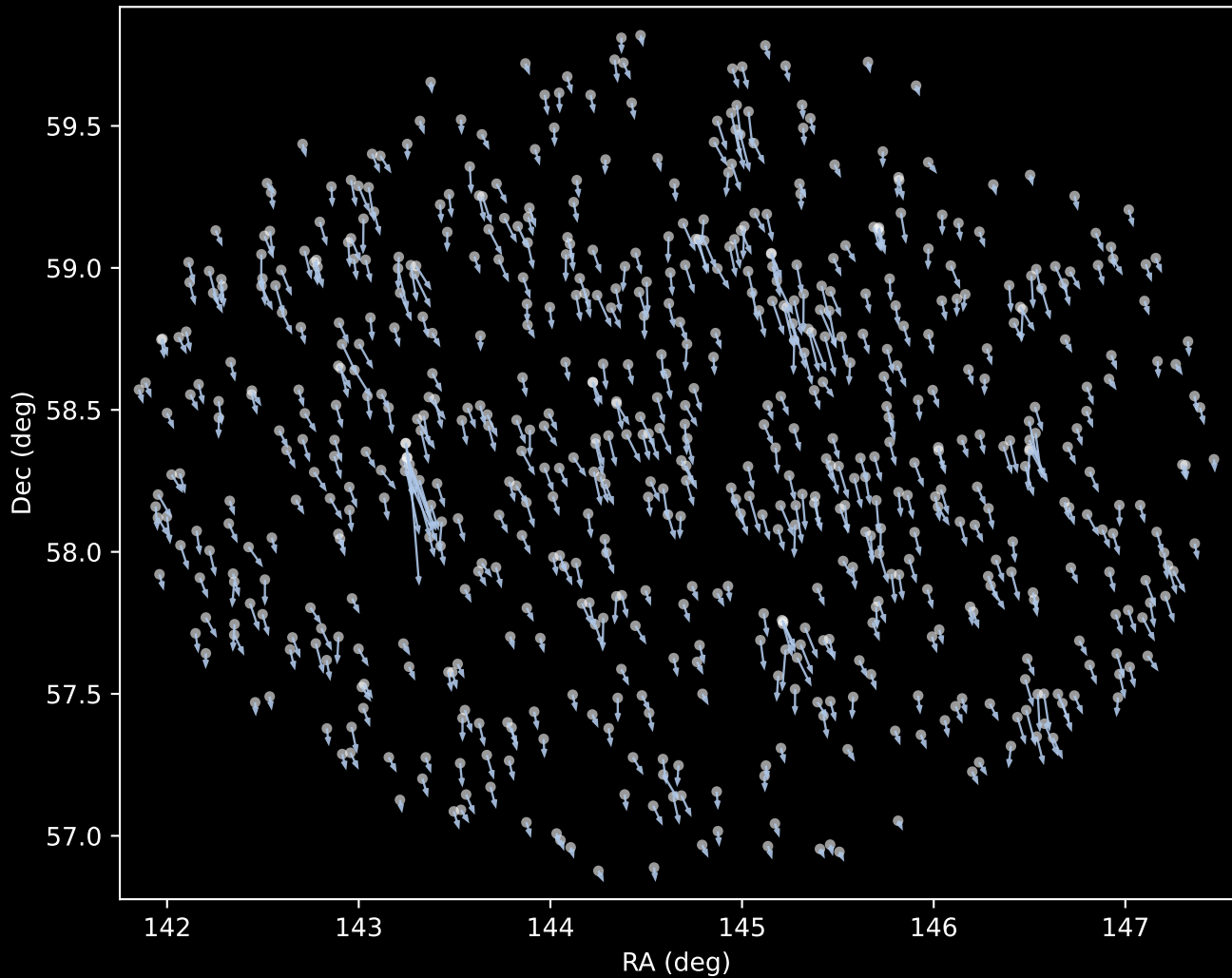
Gaia DR3 Cluster 1 Proper Motion Vectors (n=637)
