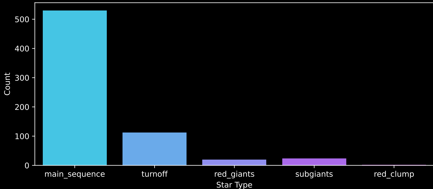
Gaia Cluster: [COIN-Gaia_37] Count plot of Star Type
