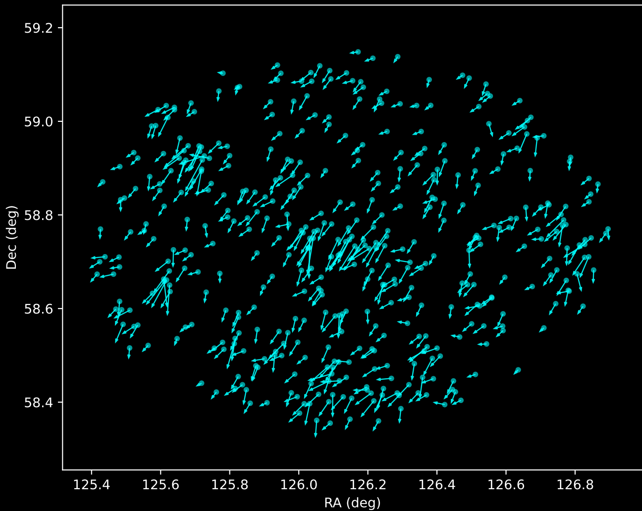
Gaia DR3 Noise Stream Proper Motion Vectors (n=436)
