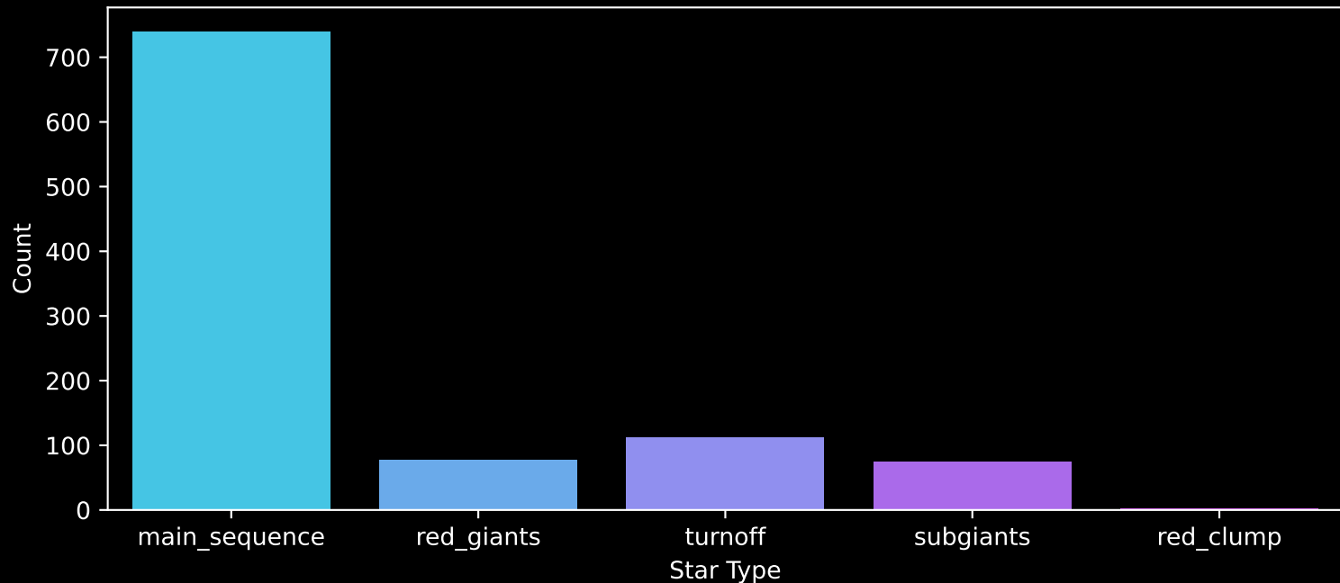
Gaia Cluster: [COIN-Gaia_4] Count plot of Star Type
