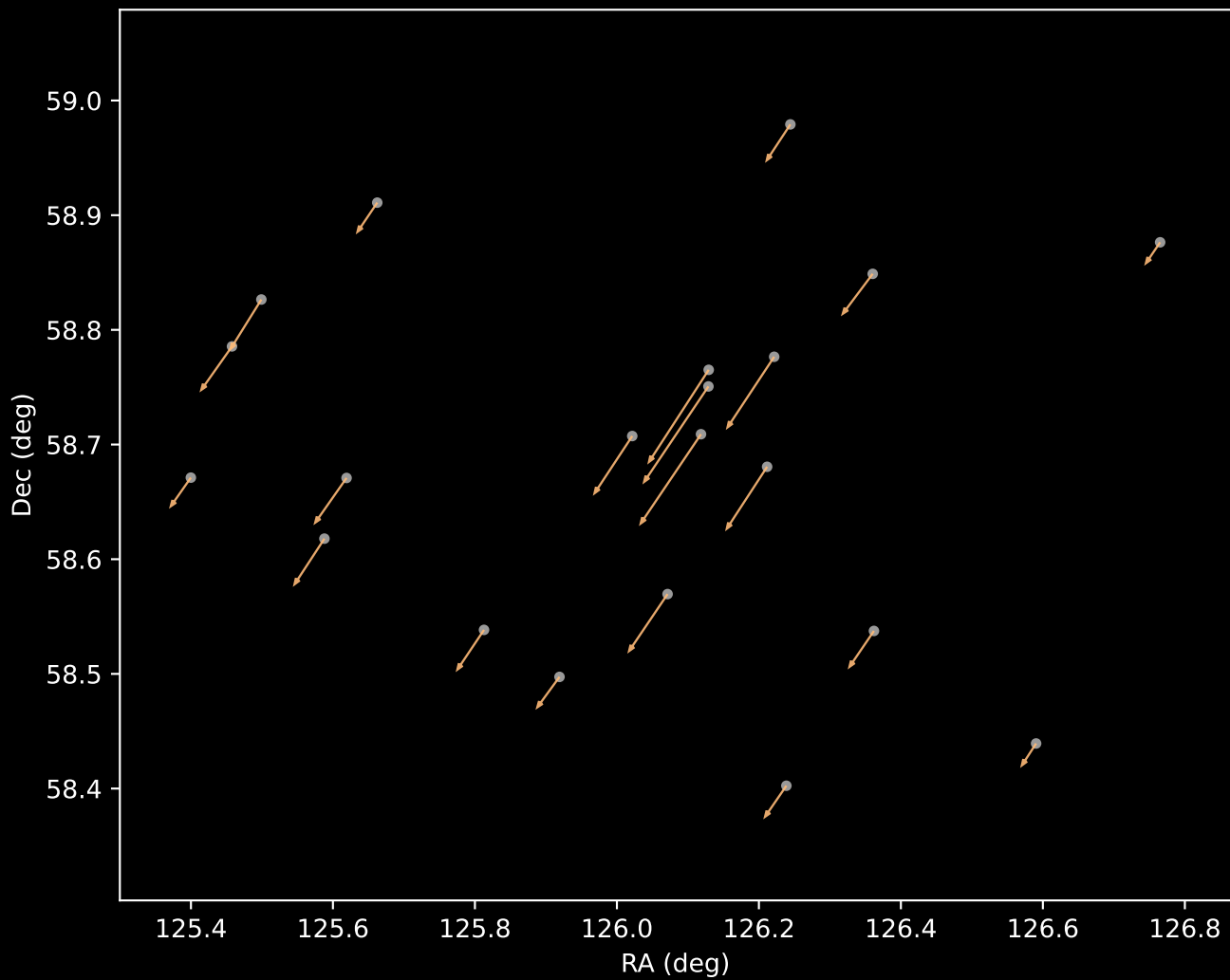
Gaia DR3 Cluster 43 Proper Motion Vectors (n=21)
