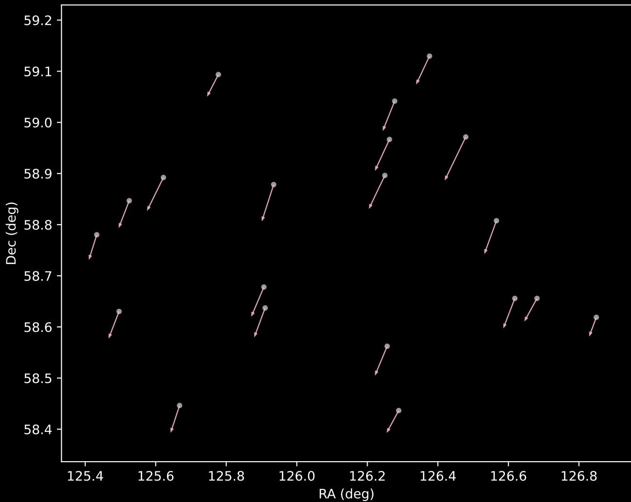
Gaia DR3 Cluster 33 Proper Motion Vectors (n=20)
