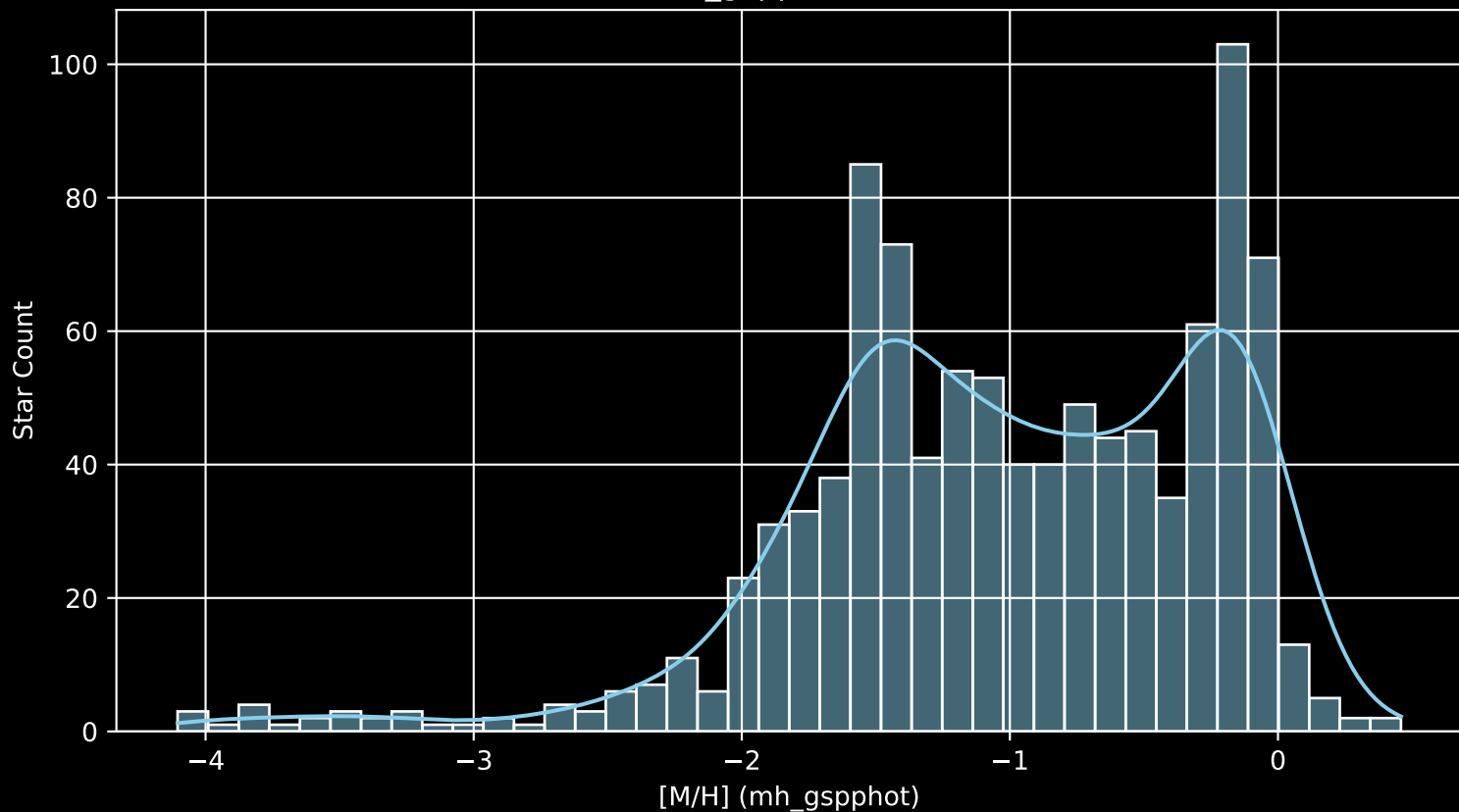
Gaia Cluster: [COIN-Gaia_4 [M/H] (mh_gspphot) (n= 1002)
