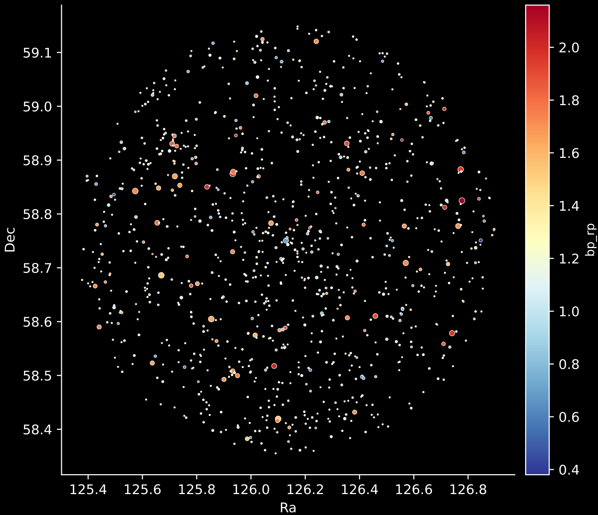
Gaia Cluster: [COIN-Gaia_4] Stars: 1005
