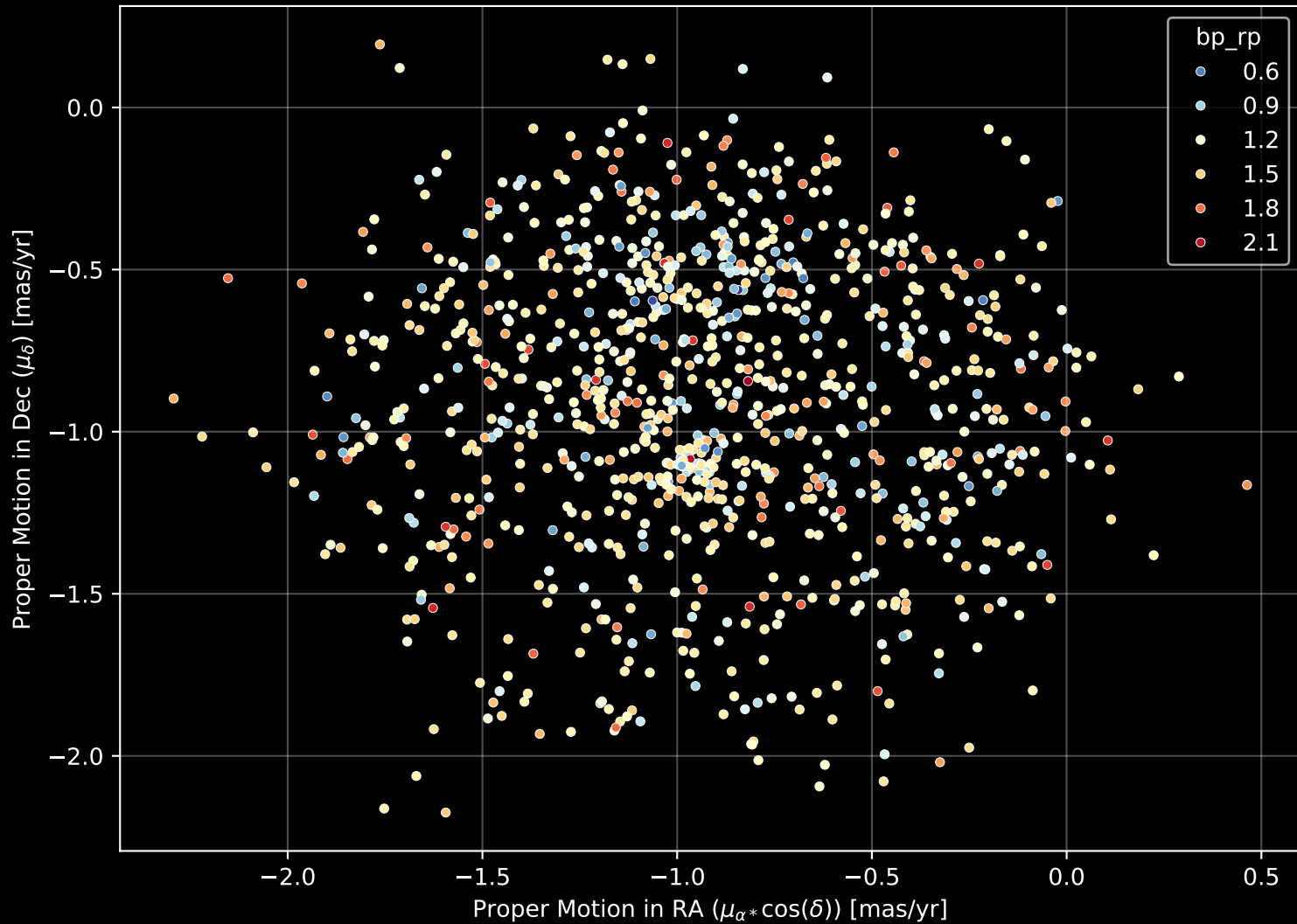
Gaia Cluster: [COIN-Gaia_4] Proper Motion Diagram (n= 1005)
