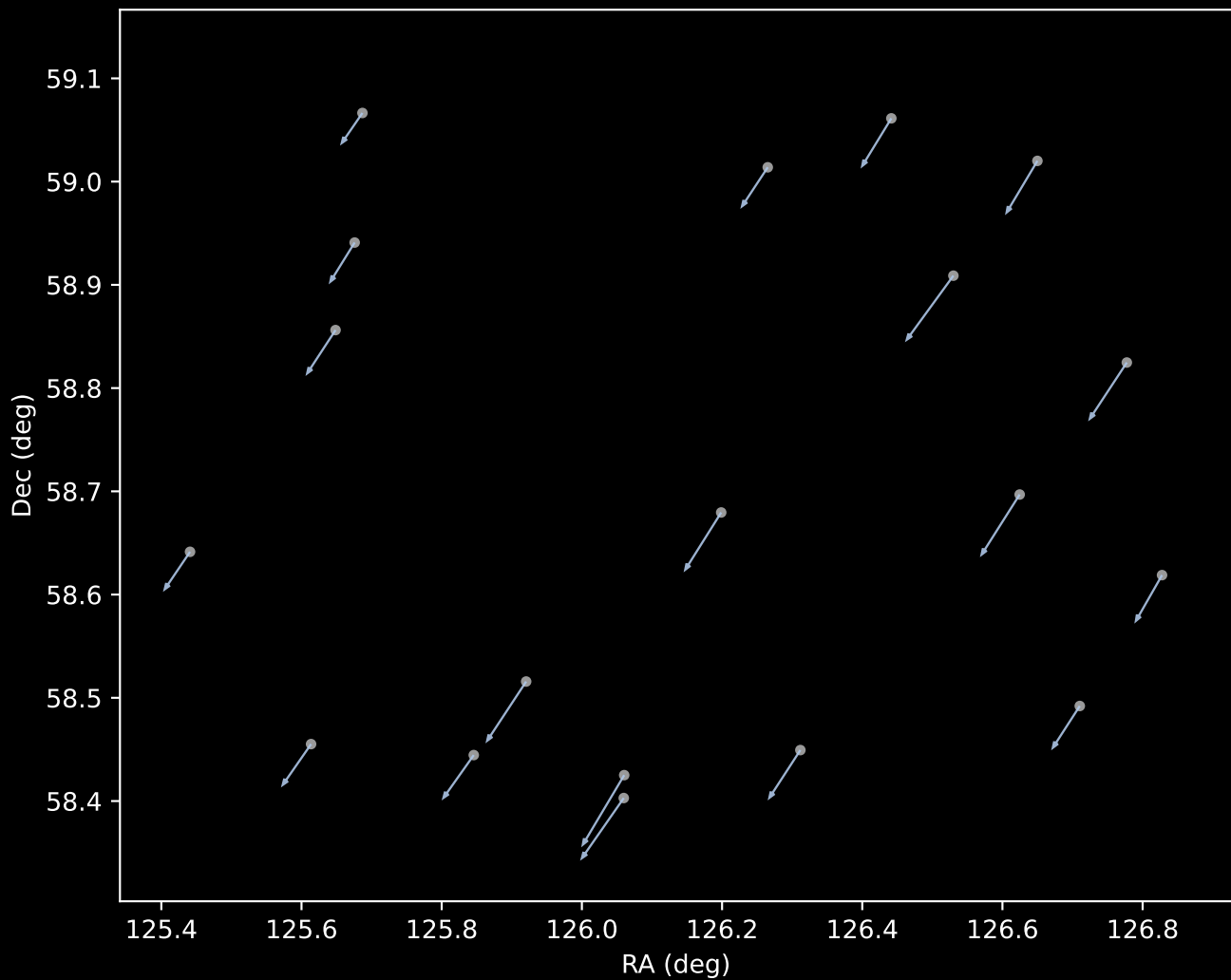
Gaia DR3 Cluster 41 Proper Motion Vectors (n=19)
