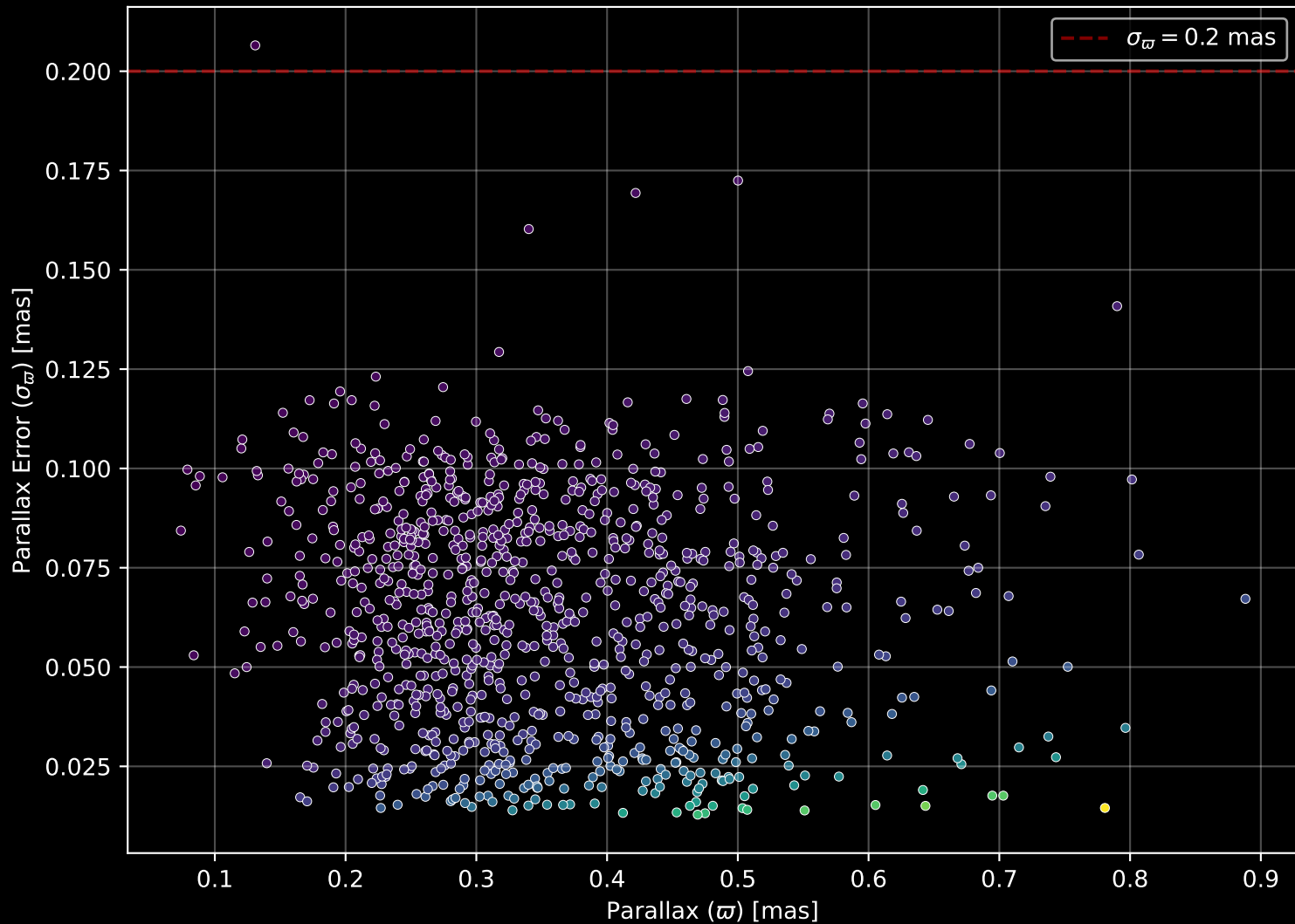
Gaia Cluster: [COIN-Gaia_4] Parallax Quality (n= 1005)
