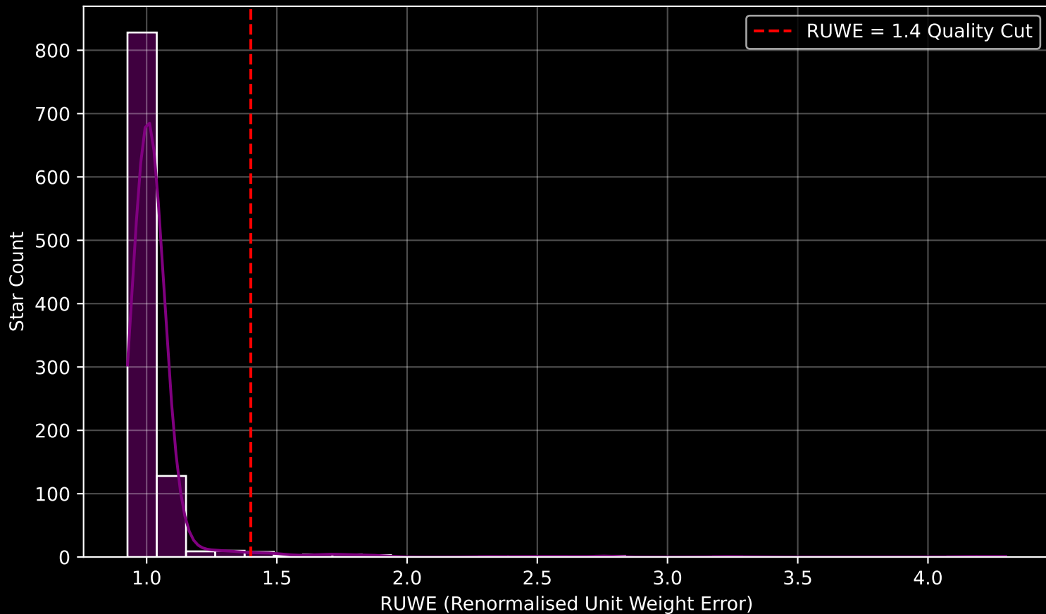
Gaia Cluster: [COIN-Gaia_4] RUWE Distribution (n= 1004)
