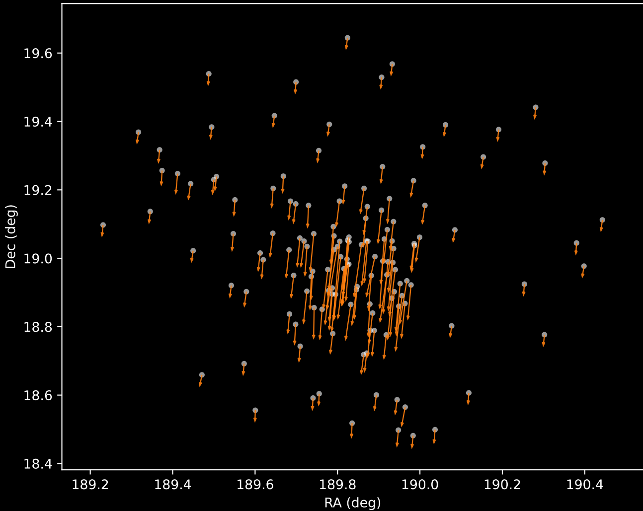
Gaia DR3 Cluster 2 Proper Motion Vectors (n=136)
