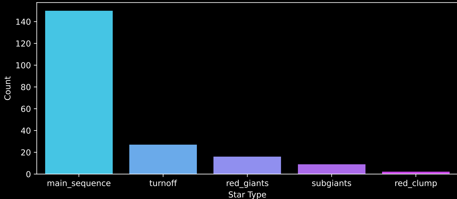
Gaia Cluster: [COIN-Gaia_41] Count plot of Star Type
