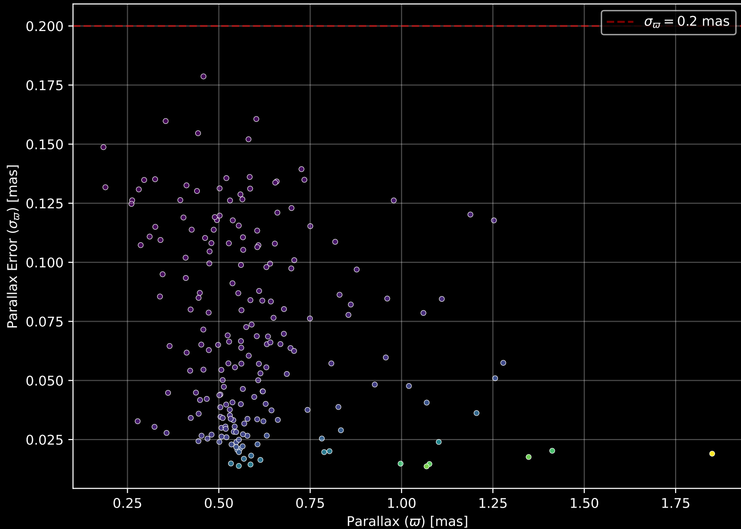
Gaia Cluster: [COIN-Gaia_41] Parallax Quality (n= 204)
