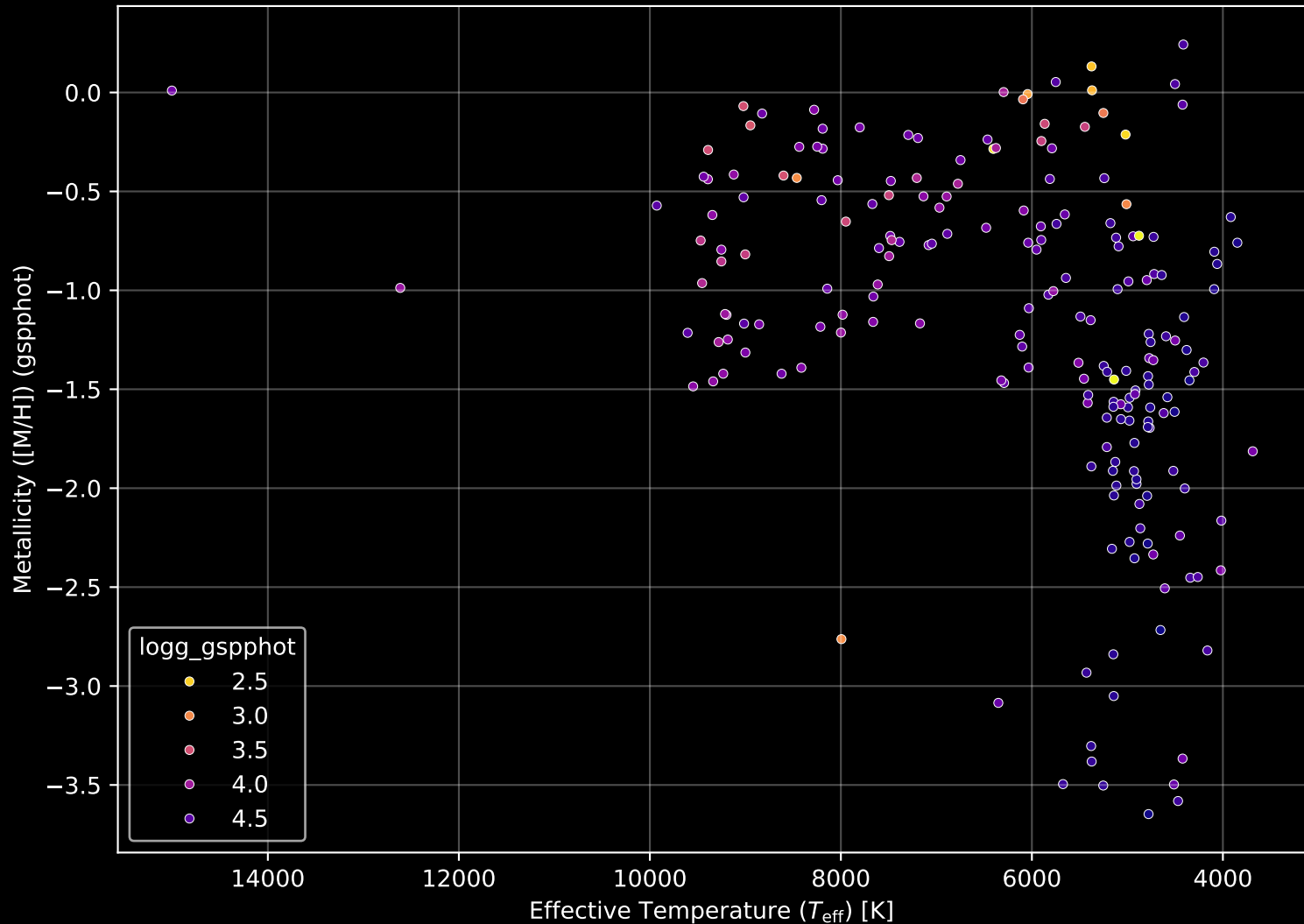
Gaia Cluster: [COIN-Gaia_41] Stellar Population Parameters (n= 204)
