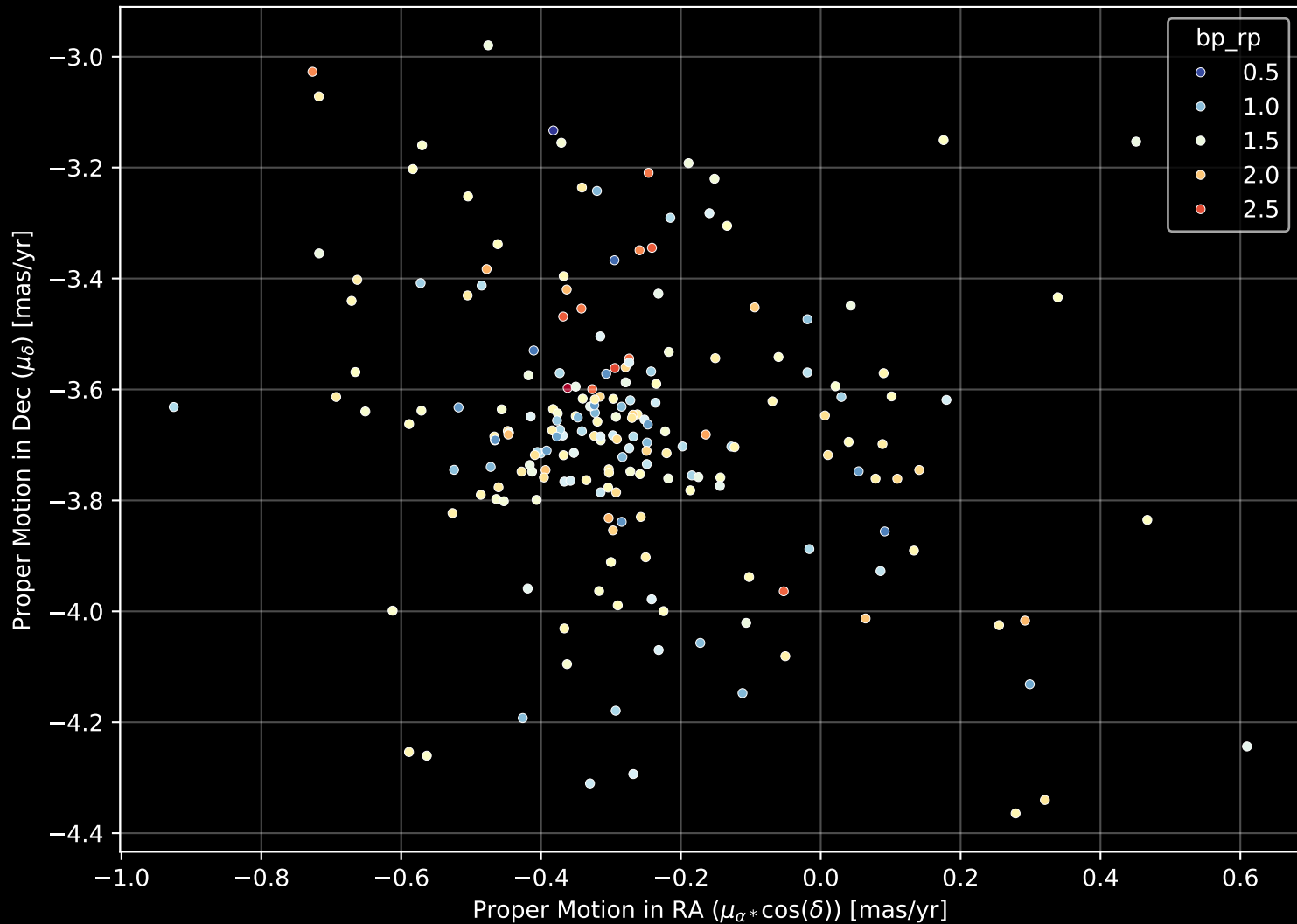
Gaia Cluster: [COIN-Gaia_41] Proper Motion Diagram (n= 204)
