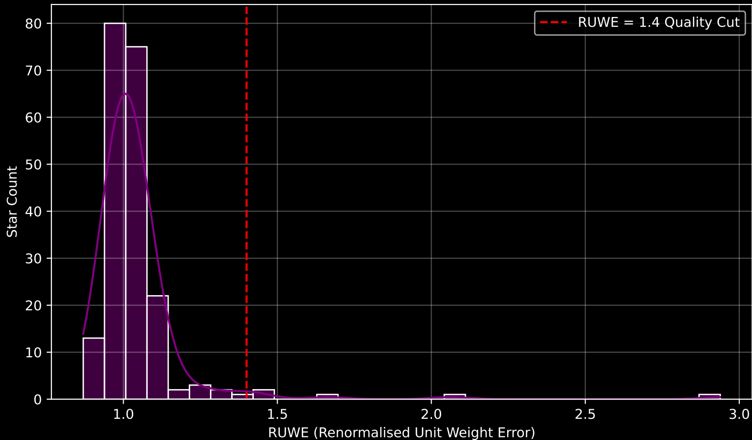
Gaia Cluster: [COIN-Gaia_41] RUWE Distribution (n= 203)
