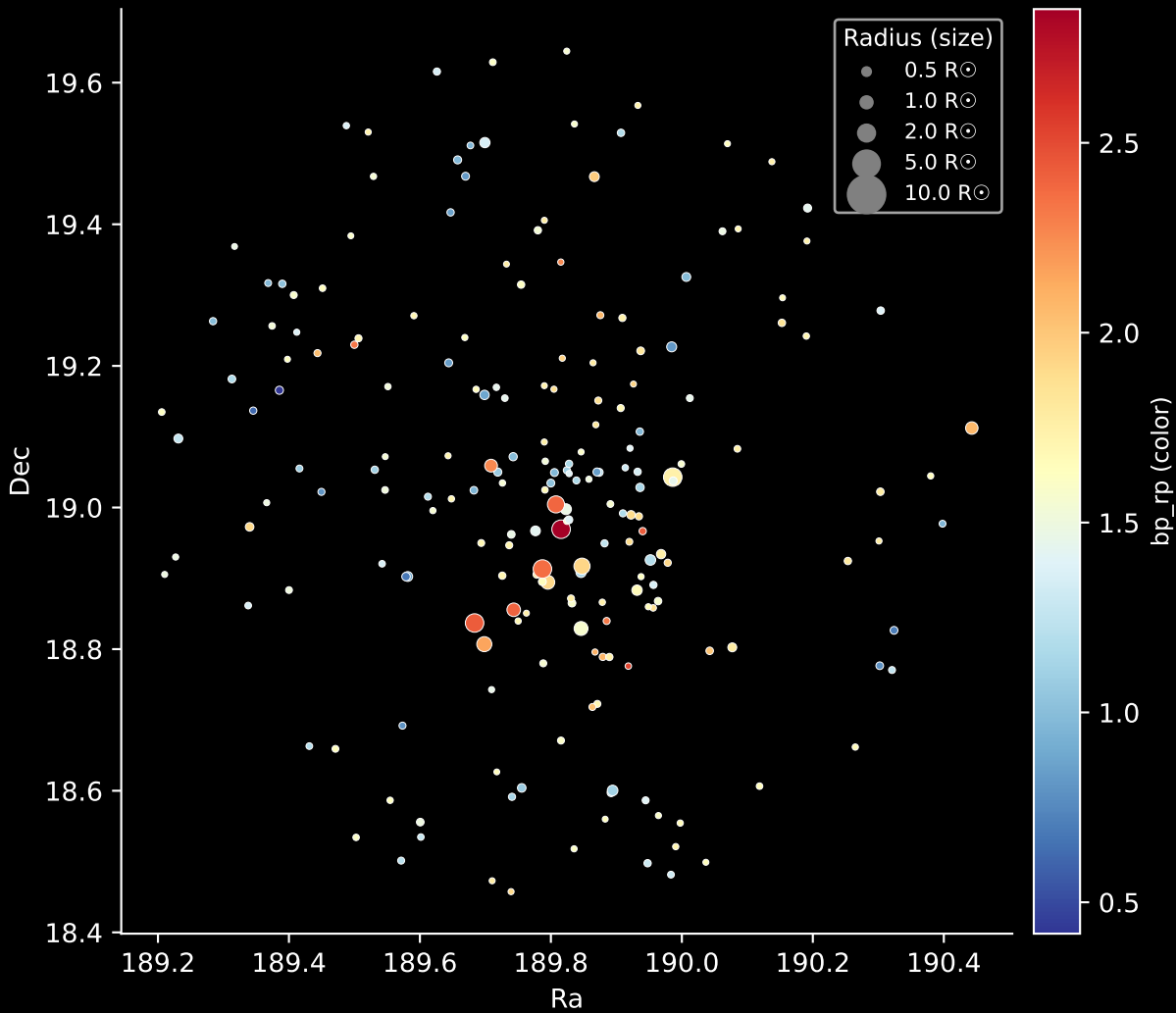
Gaia Cluster: [COIN-Gaia_41] Stars: 204
