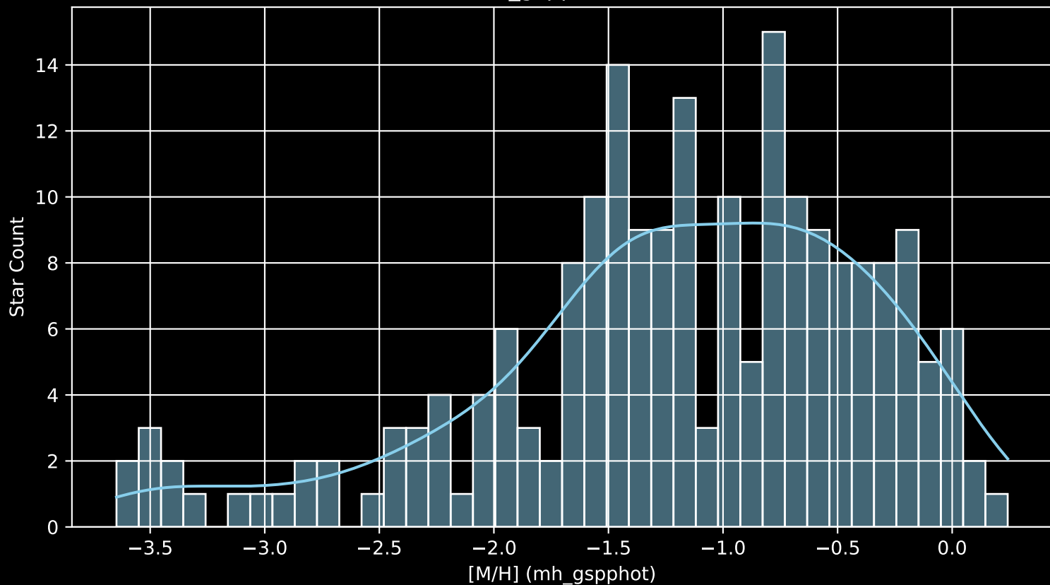
Gaia Cluster: [COIN-Gaia_41 [M/H] (mh_gspphot) (n= 204)
