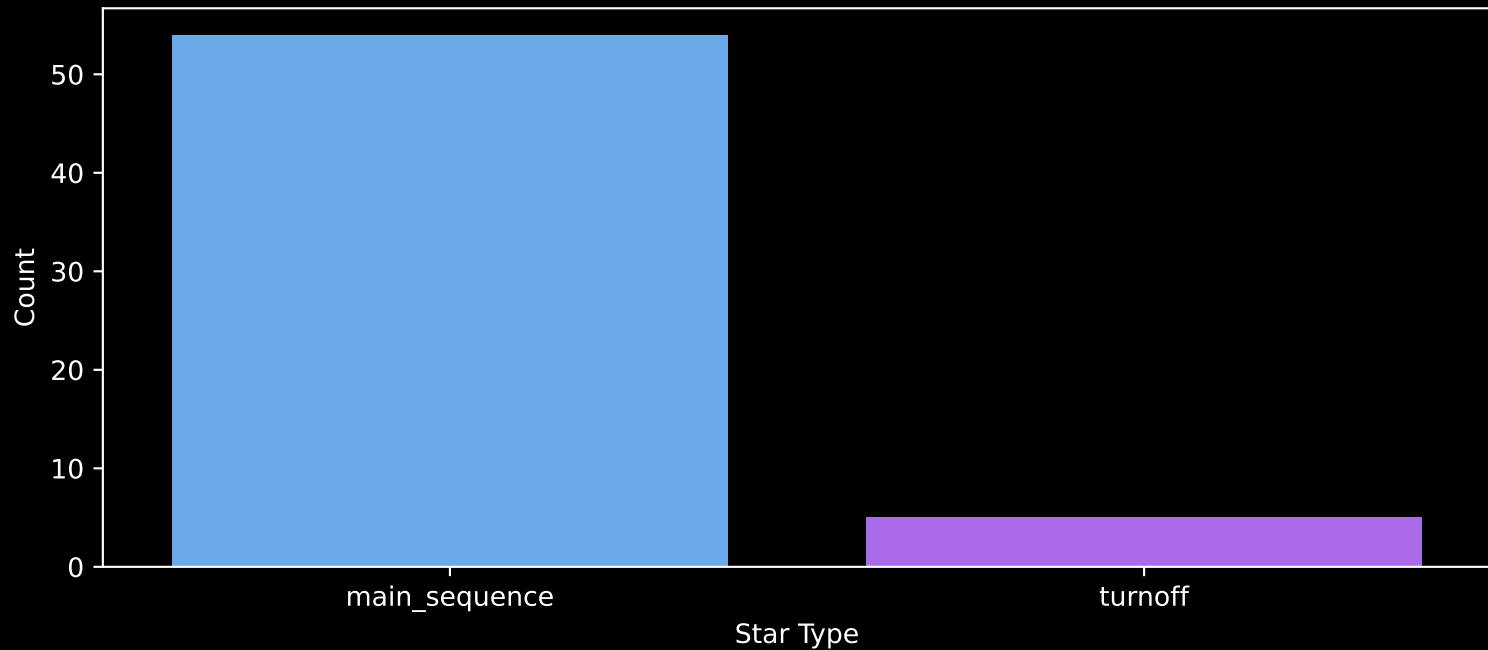
Gaia Cluster: [COIN-Gaia_5] Count plot of Star Type
