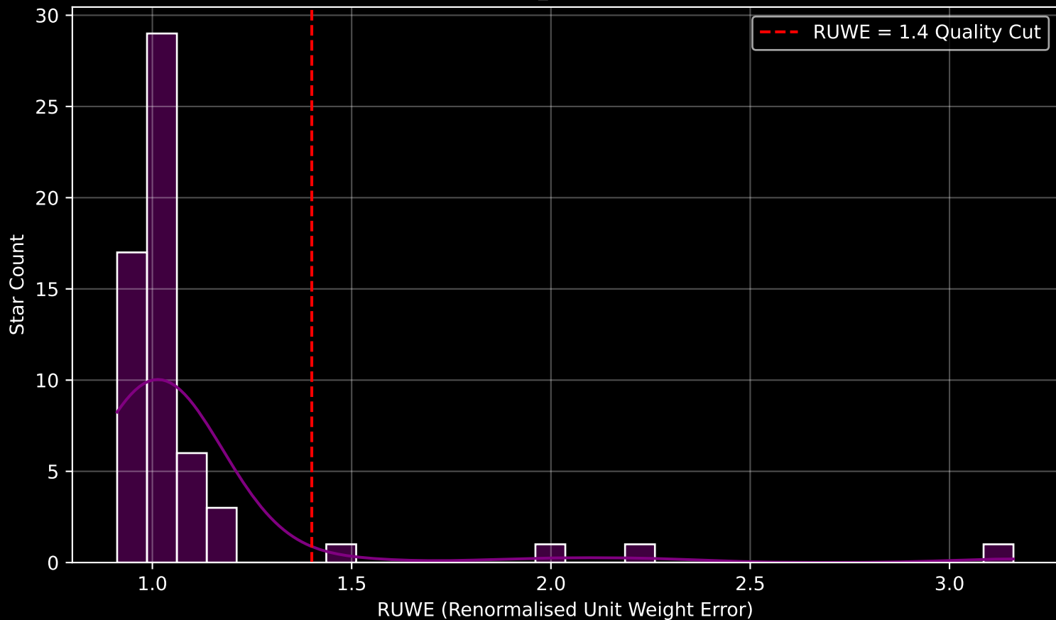
Gaia Cluster: [COIN-Gaia_5] RUWE Distribution (n= 59)
