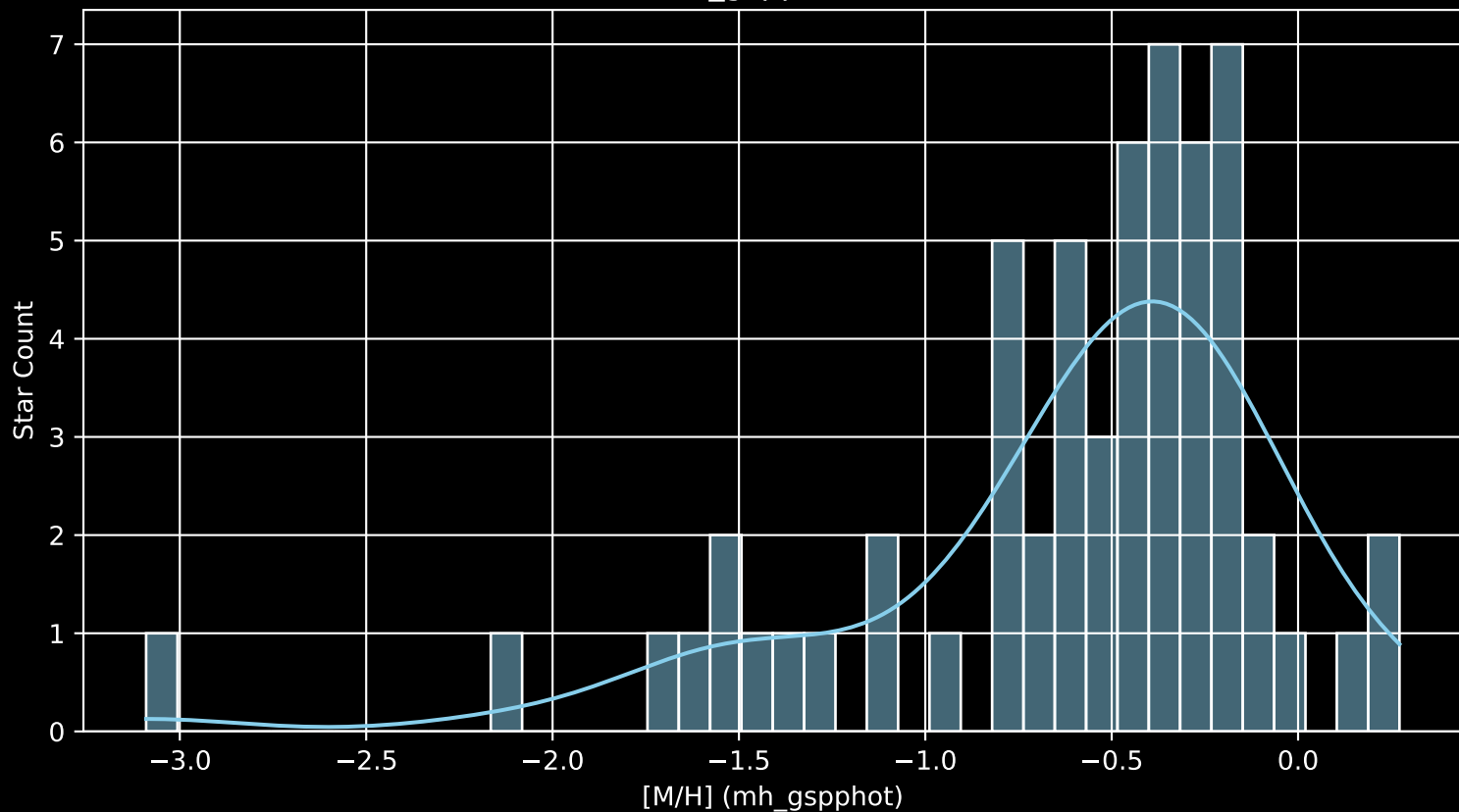
Gaia Cluster: [COIN-Gaia_5 [M/H] (mh_gspphot) (n= 59)
