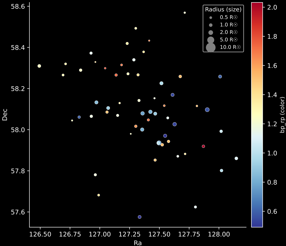
Gaia Cluster: [COIN-Gaia_5] Stars: 59
