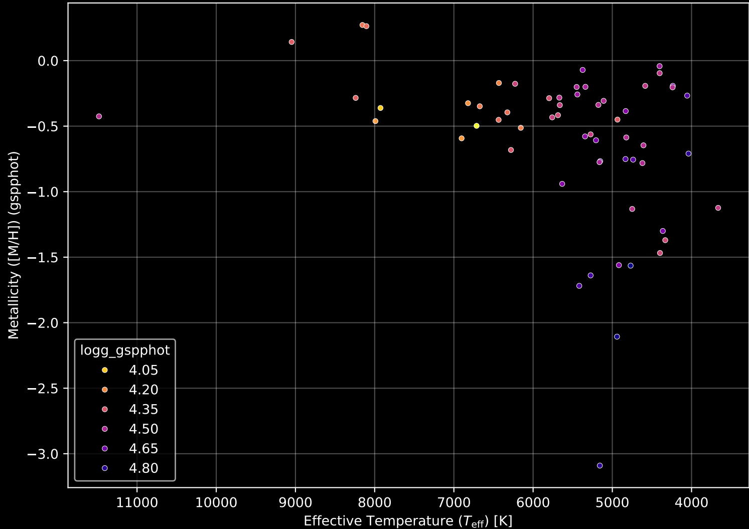
Gaia Cluster: [COIN-Gaia_5] Stellar Population Parameters (n= 59)
