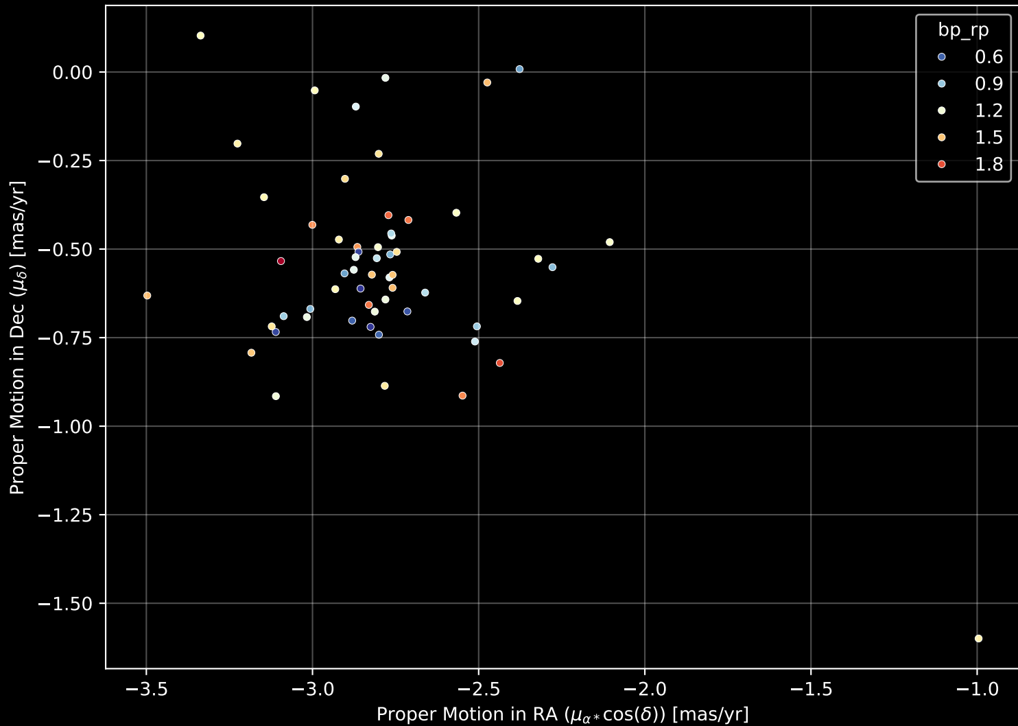
Gaia Cluster: [COIN-Gaia_5] Proper Motion Diagram (n= 59)
