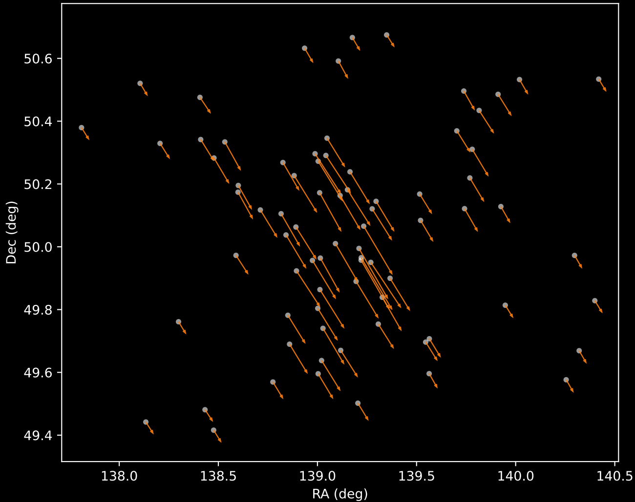
Gaia DR3 Cluster 2 Proper Motion Vectors (n=77)
