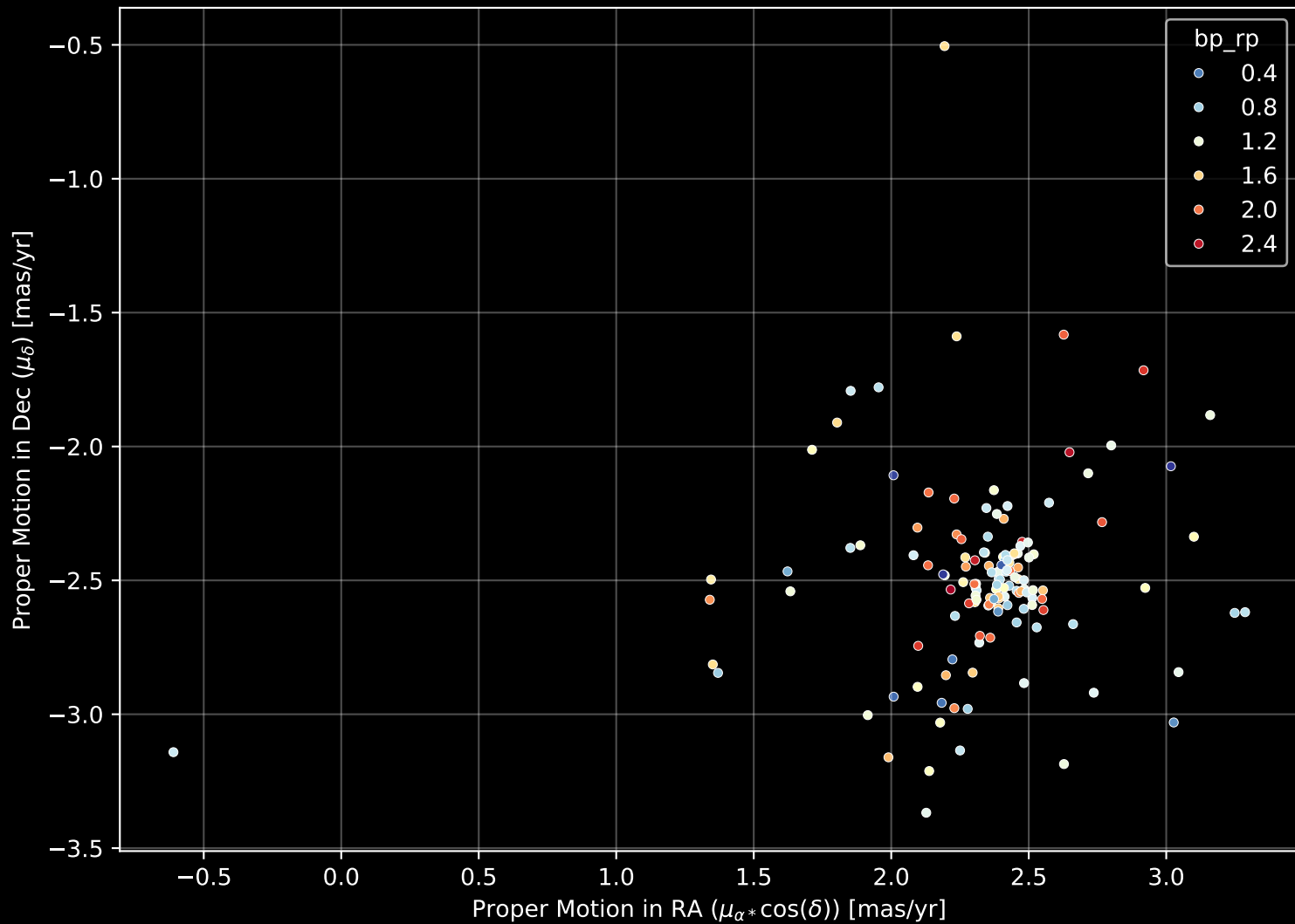
Gaia Cluster: [COIN-Gaia_8] Proper Motion Diagram (n= 143)
