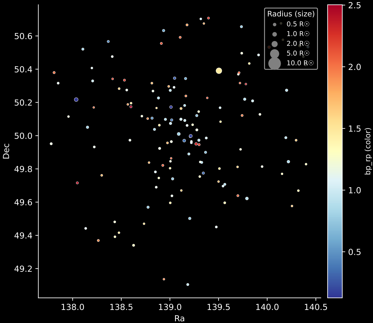
Gaia Cluster: [COIN-Gaia_8] Stars: 143
