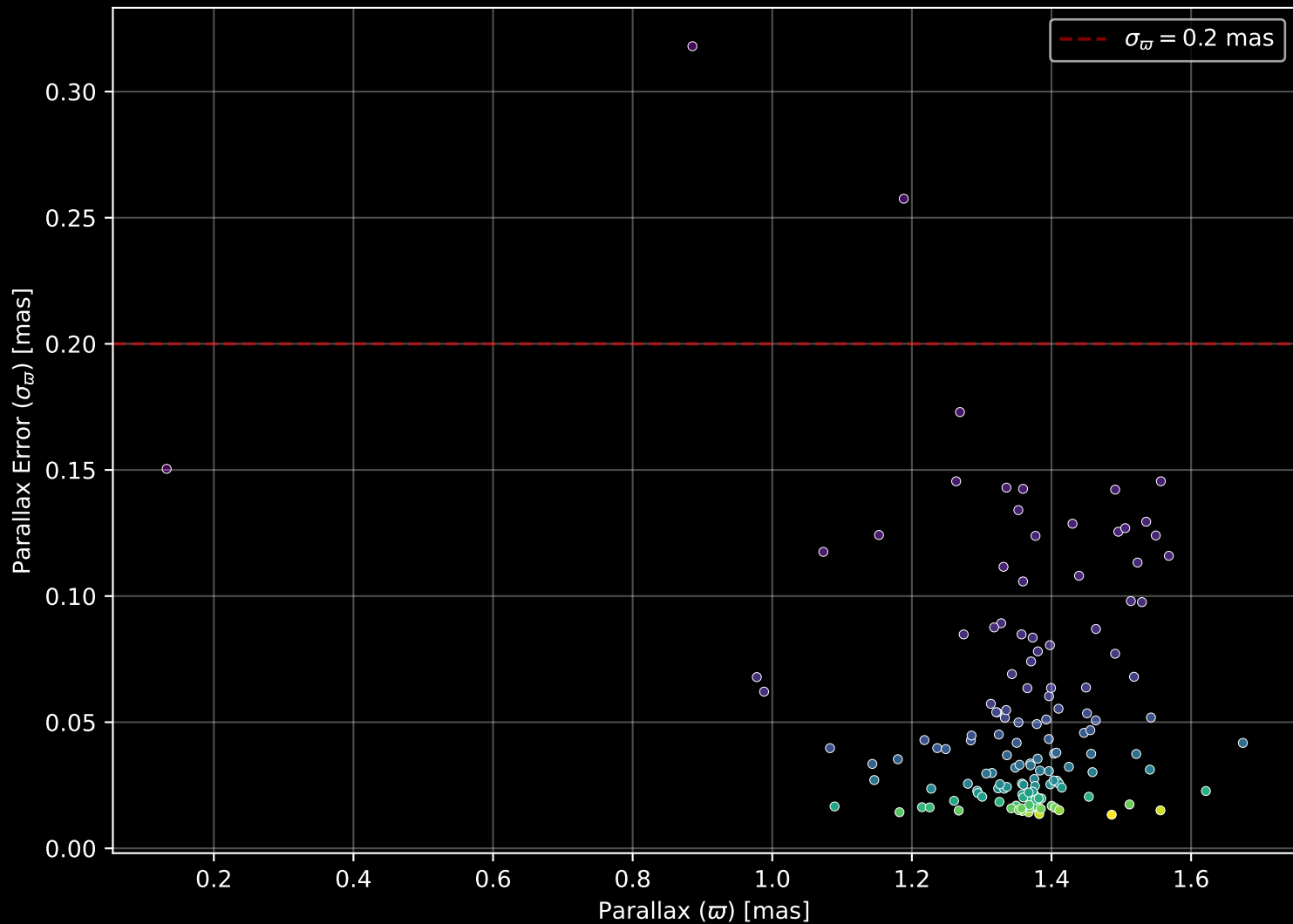
Gaia Cluster: [COIN-Gaia_8] Parallax Quality (n= 143)
