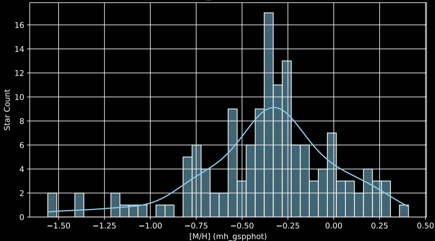
Gaia Cluster: [COIN-Gaia_8 [M/H] (mh_gspphot) (n= 143)
