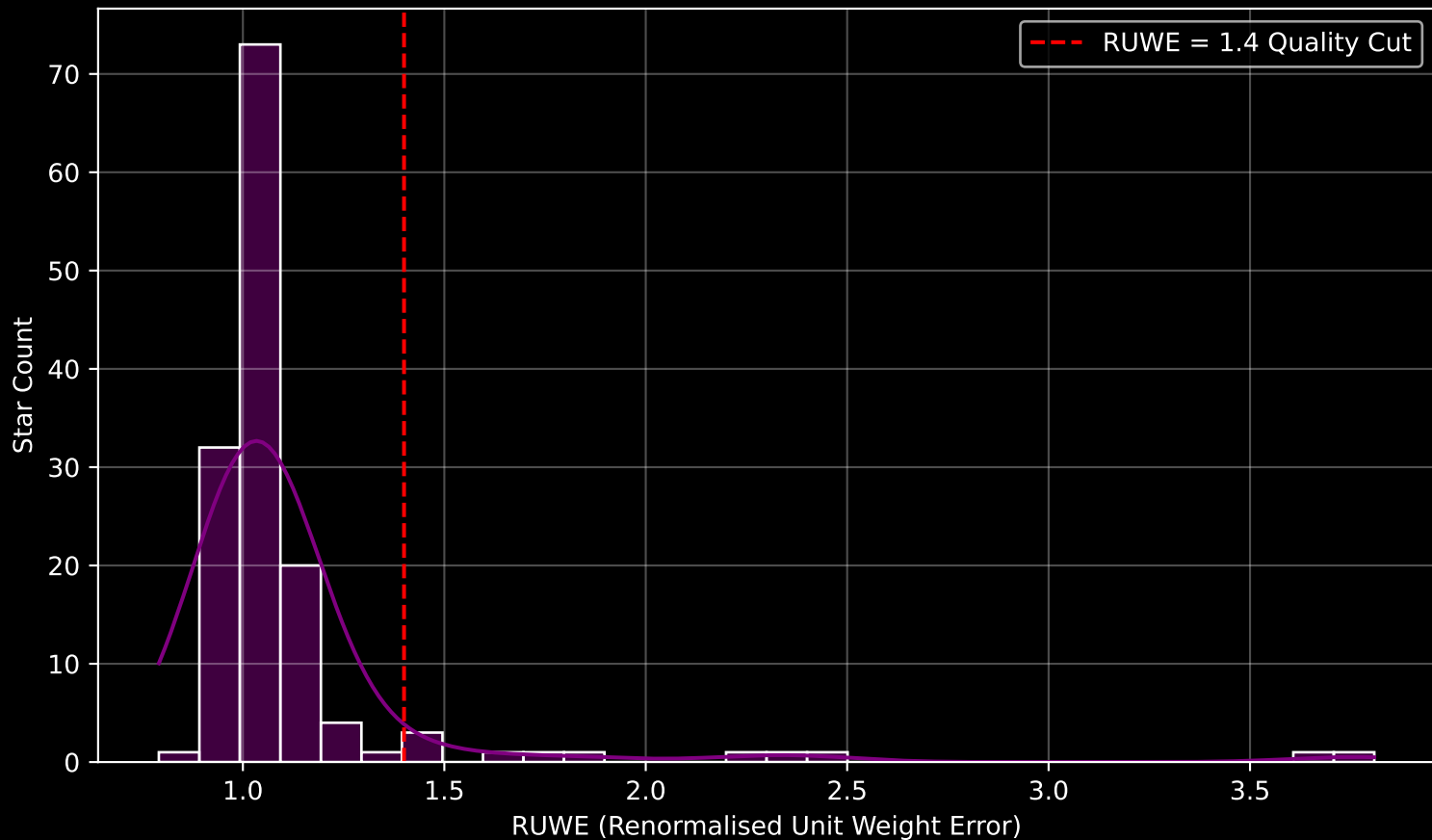
Gaia Cluster: [COIN-Gaia_8] RUWE Distribution (n= 142)
