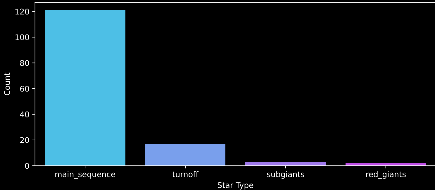
Gaia Cluster: [COIN-Gaia_8] Count plot of Star Type
