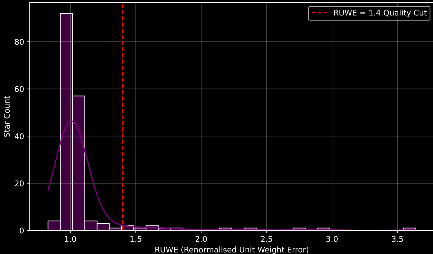
Gaia Cluster: [COIN-Gaia_9] RUWE Distribution (n= 173)
