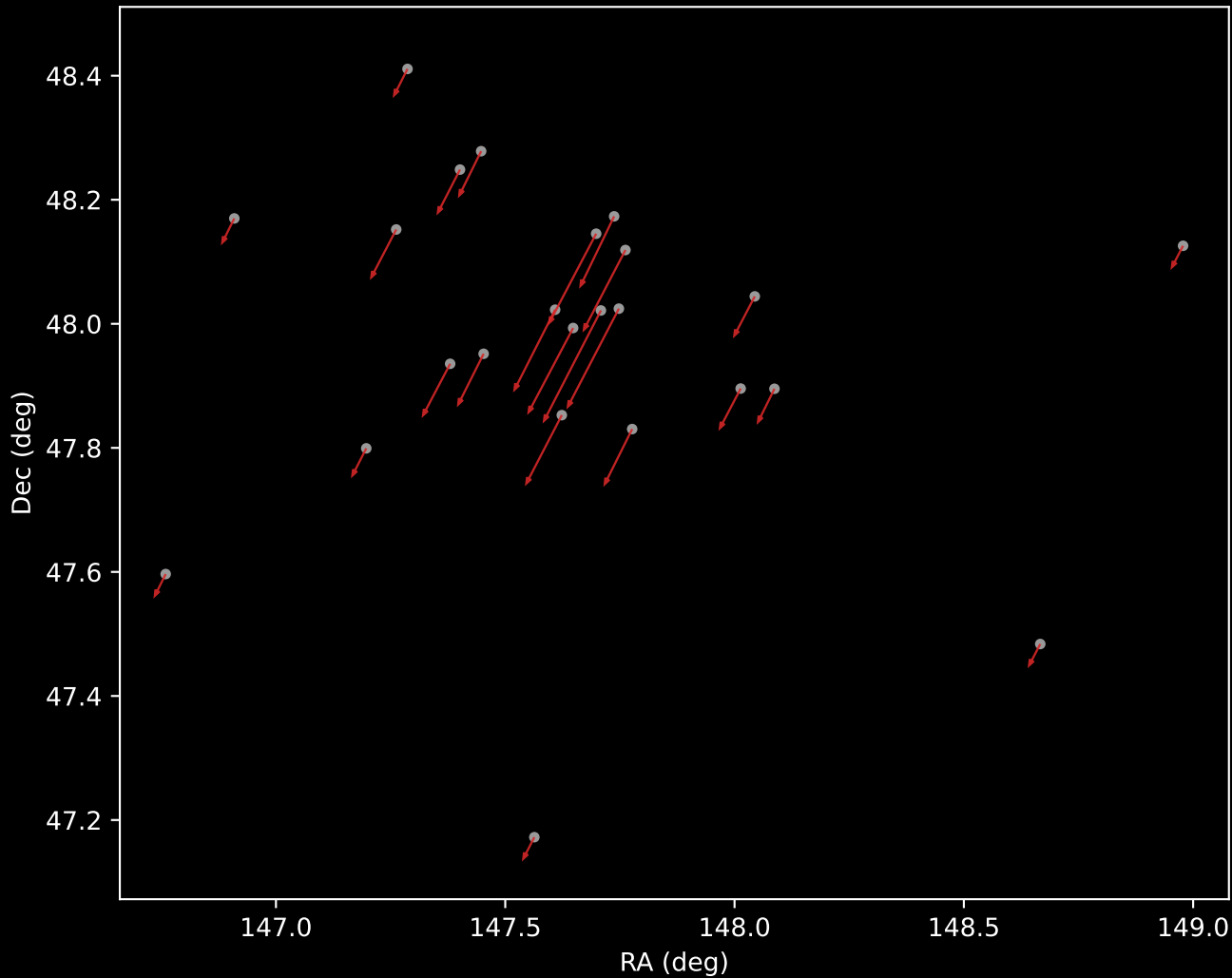
Gaia DR3 Cluster 6 Proper Motion Vectors (n=24)
