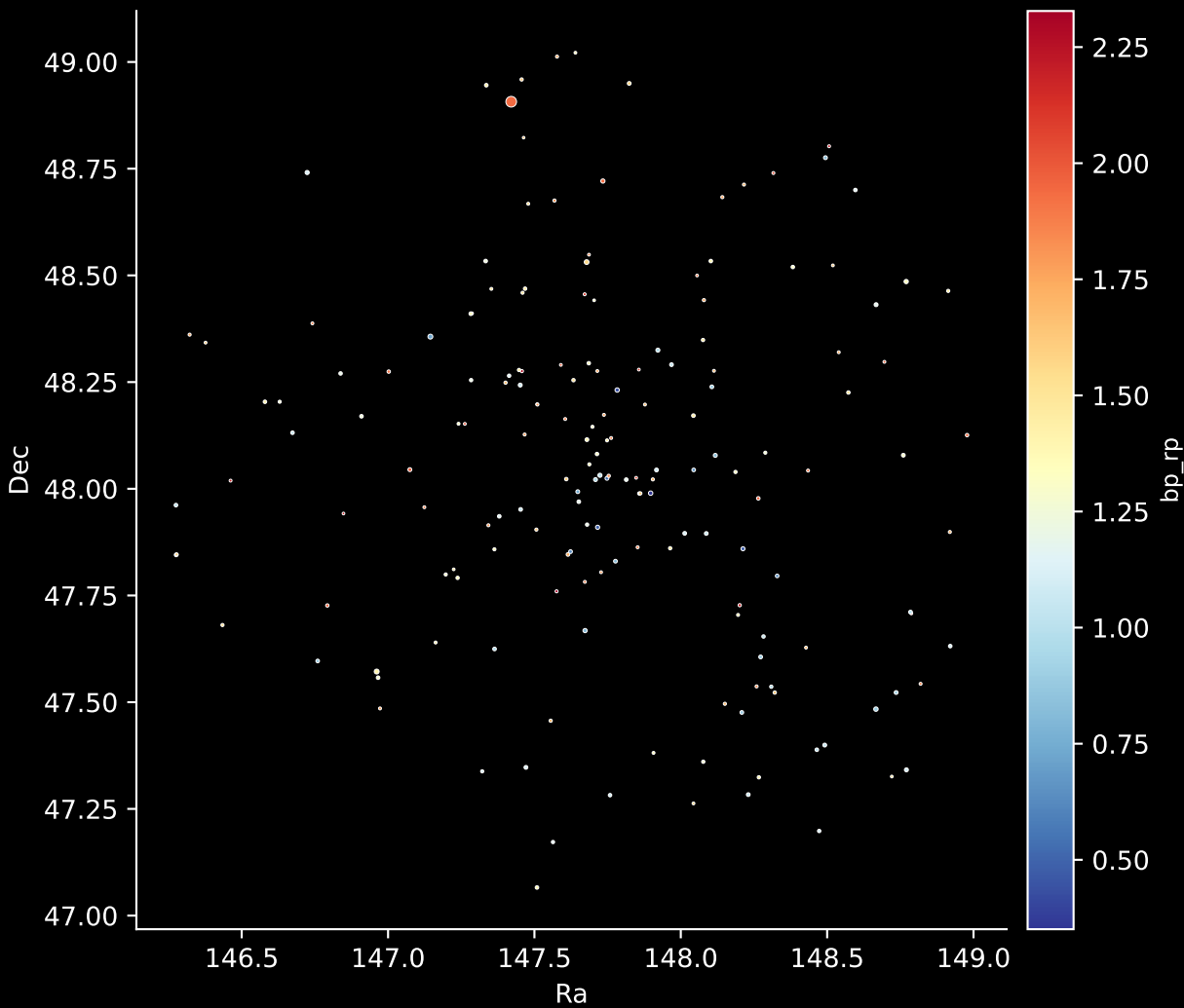
Gaia Cluster: [COIN-Gaia_9] Stars: 173
