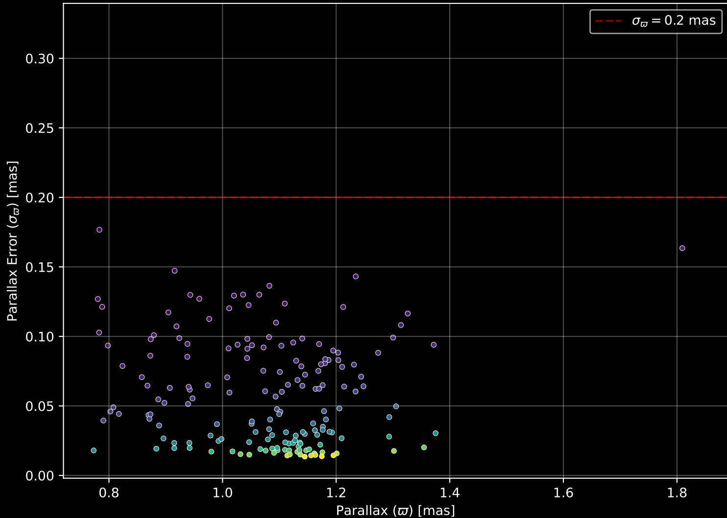
Gaia Cluster: [COIN-Gaia_9] Parallax Quality (n= 173)
