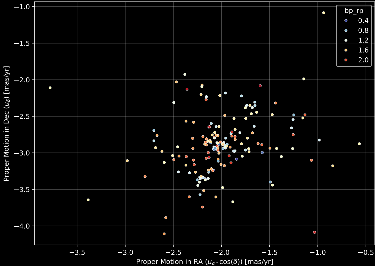
Gaia Cluster: [COIN-Gaia_9] Proper Motion Diagram (n= 173)
