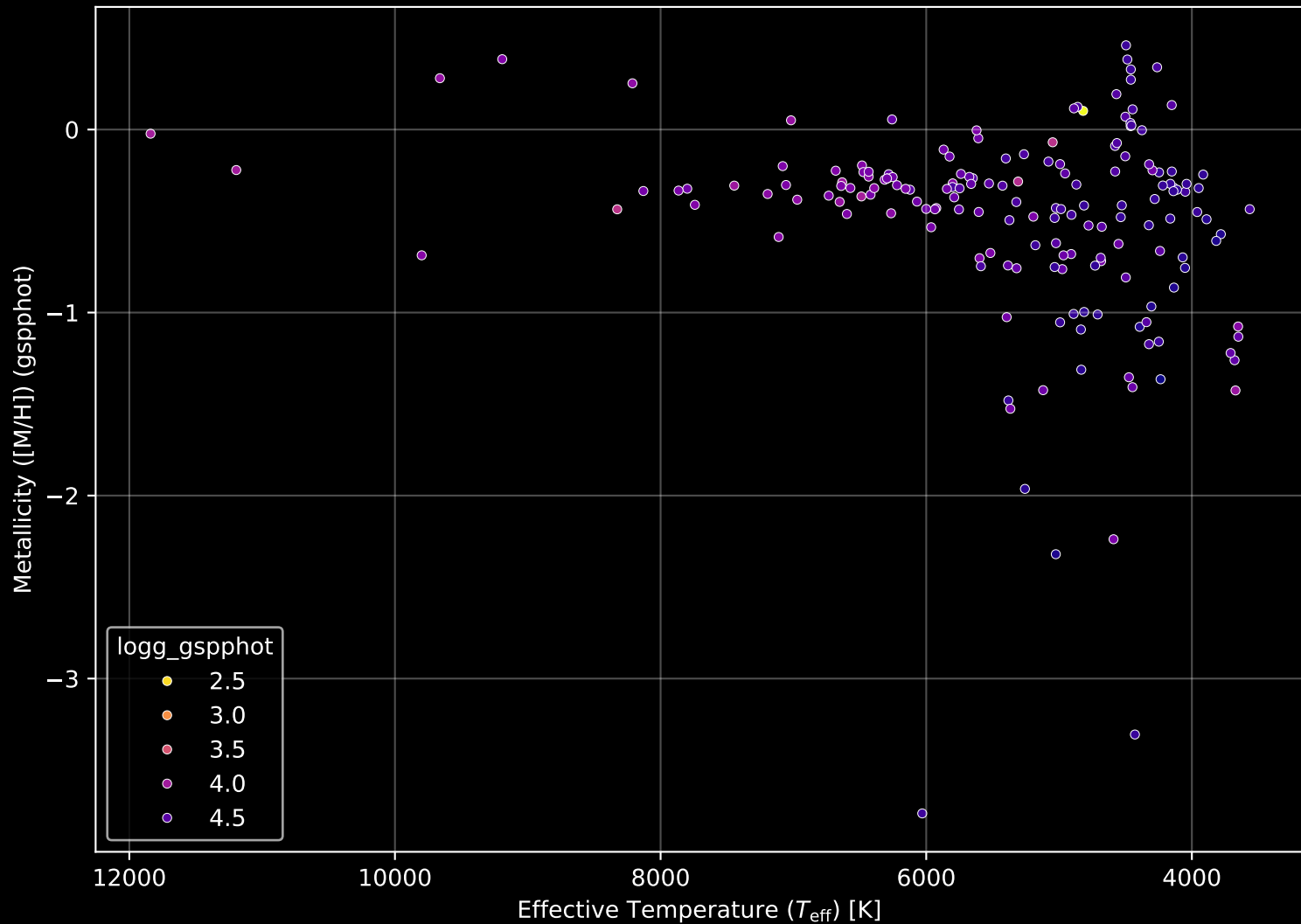
Gaia Cluster: [COIN-Gaia_9] Stellar Population Parameters (n= 173)
