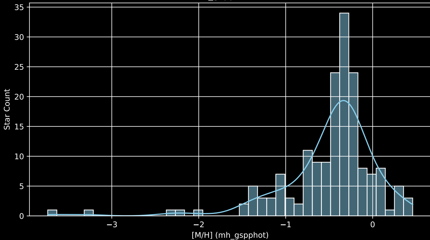
Gaia Cluster: [COIN-Gaia_9 [M/H] (mh_gspphot) (n= 173)
