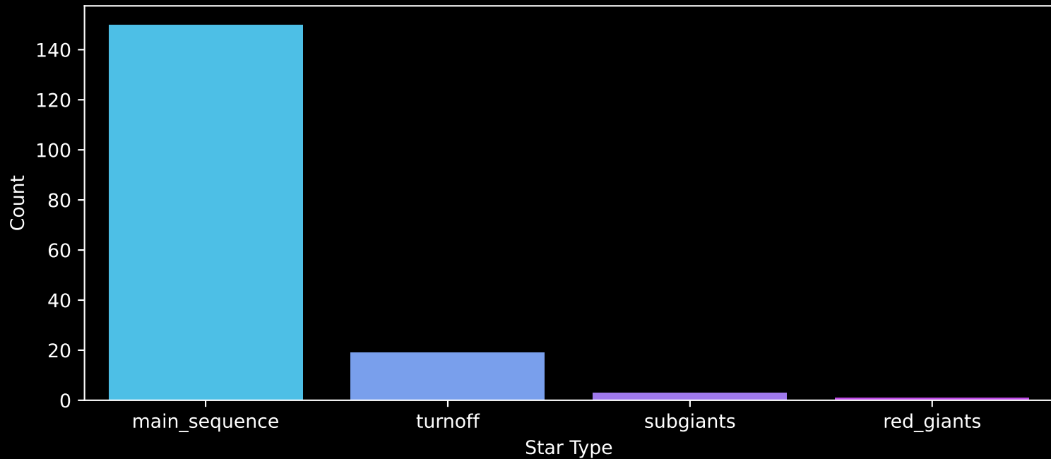
Gaia Cluster: [COIN-Gaia_9] Count plot of Star Type
