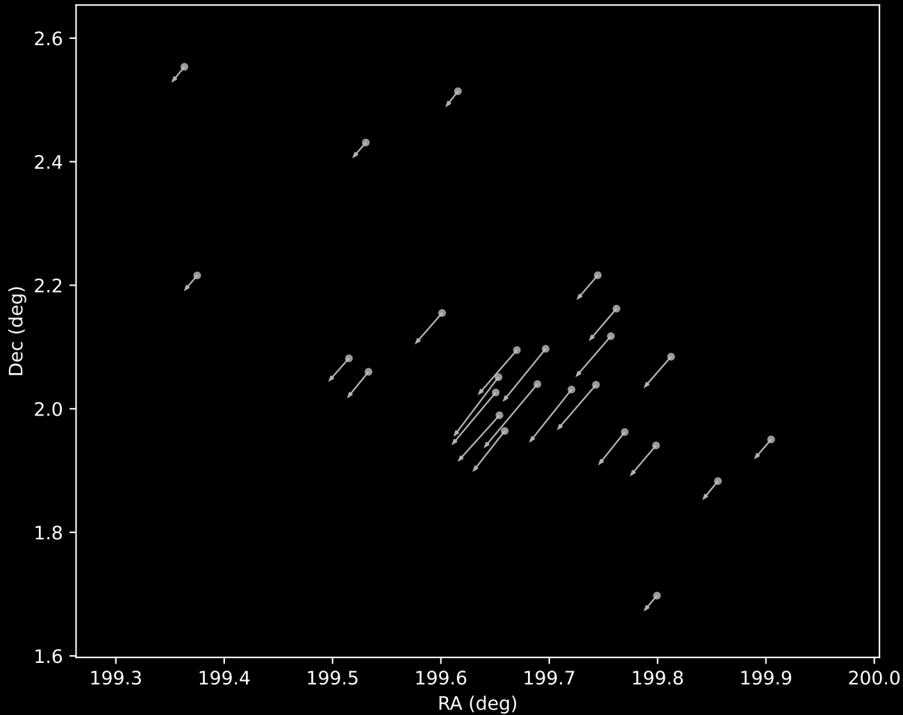
Gaia DR3 Cluster 15 Proper Motion Vectors (n=25)
