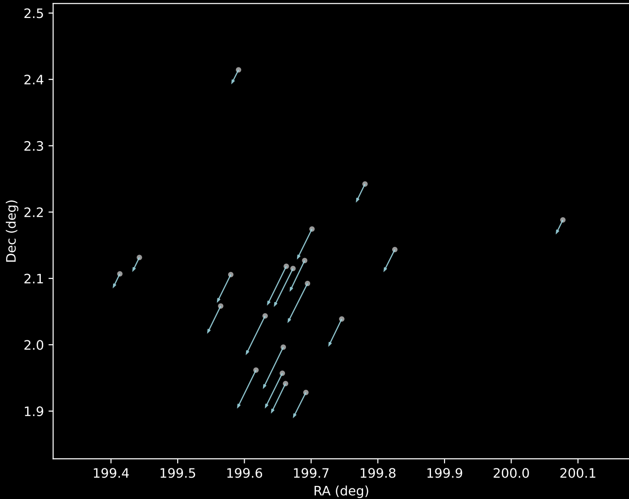
Gaia DR3 Cluster 39 Proper Motion Vectors (n=20)
