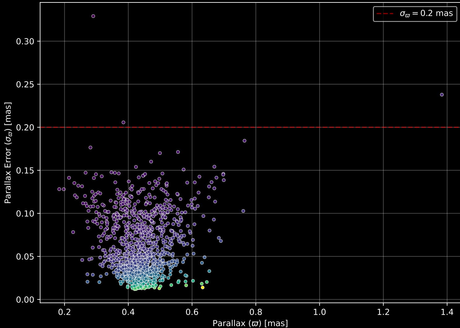
Gaia Cluster: [Collinder_110] Parallax Quality (n= 1168)
