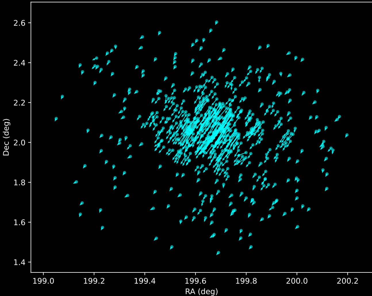
Gaia DR3 Noise Stream Proper Motion Vectors (n=546)
