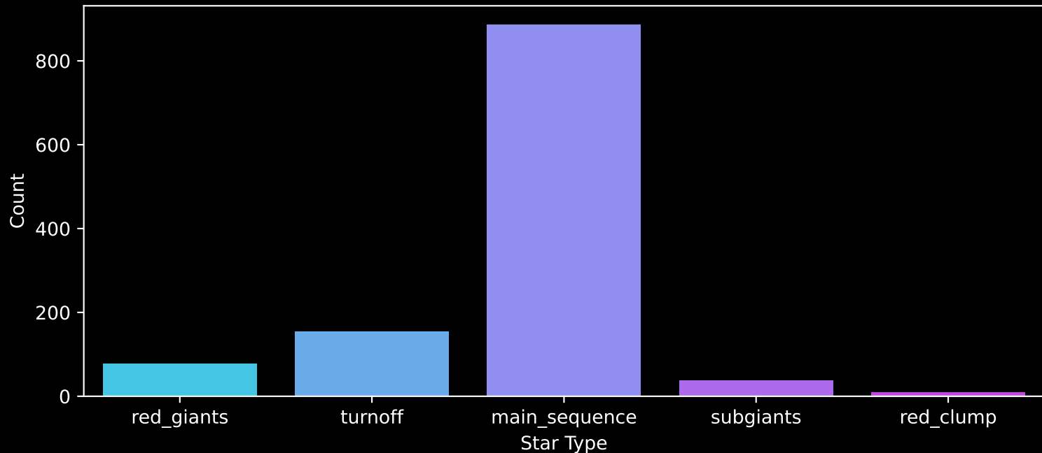
Gaia Cluster: [Collinder_110] Count plot of Star Type
