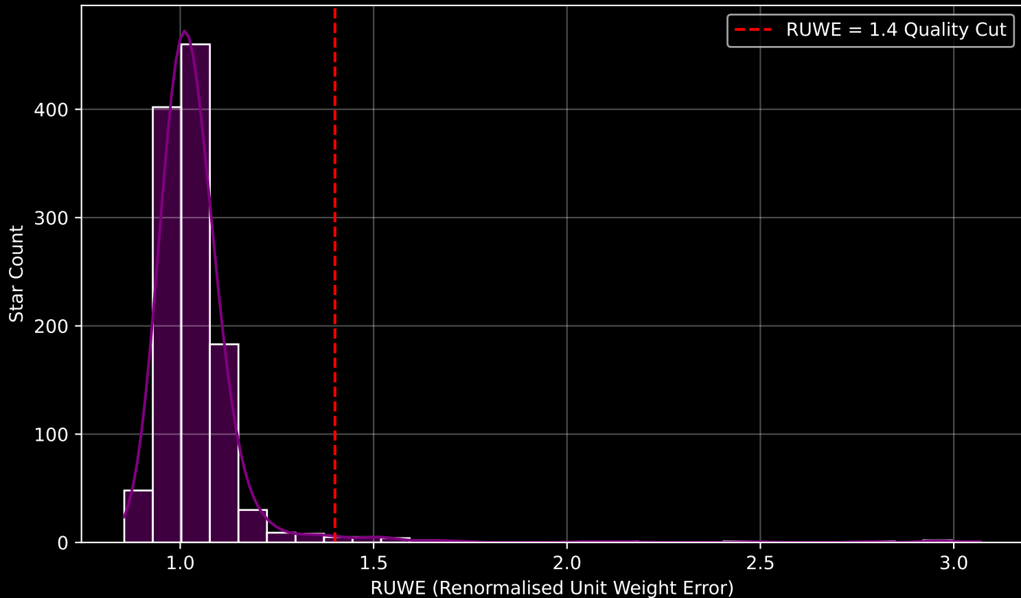
Gaia Cluster: [Collinder_110] RUWE Distribution (n= 1164)
