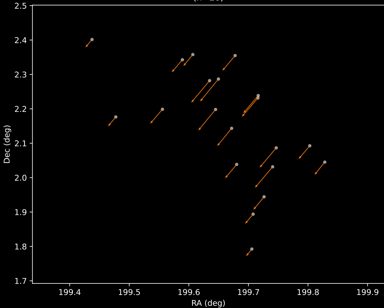
Gaia DR3 Cluster 42 Proper Motion Vectors (n=20)
