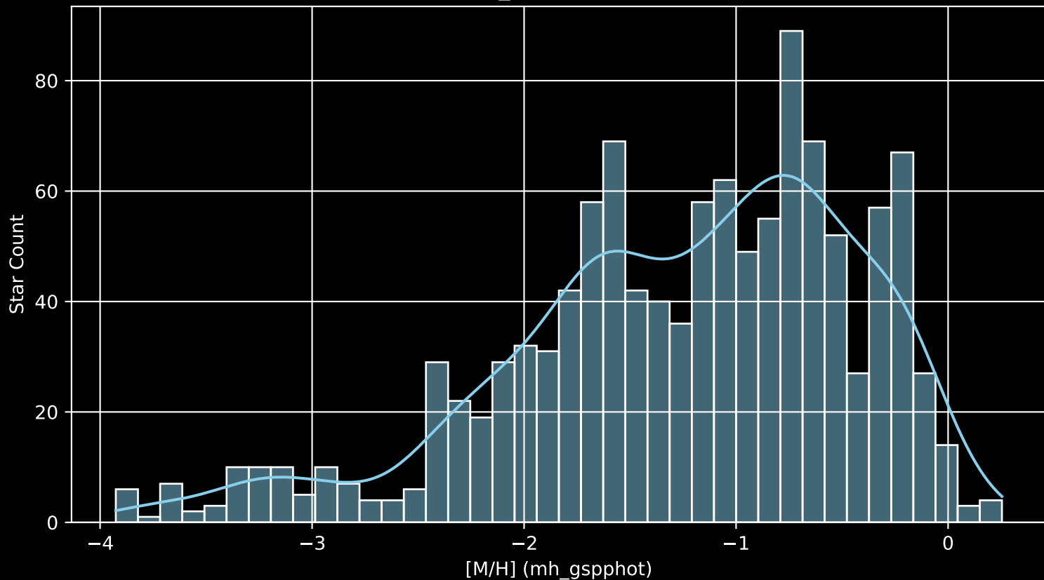
Gaia Cluster: [Collinder_110 [M/H] (mh_gspphot) (n= 1167)
