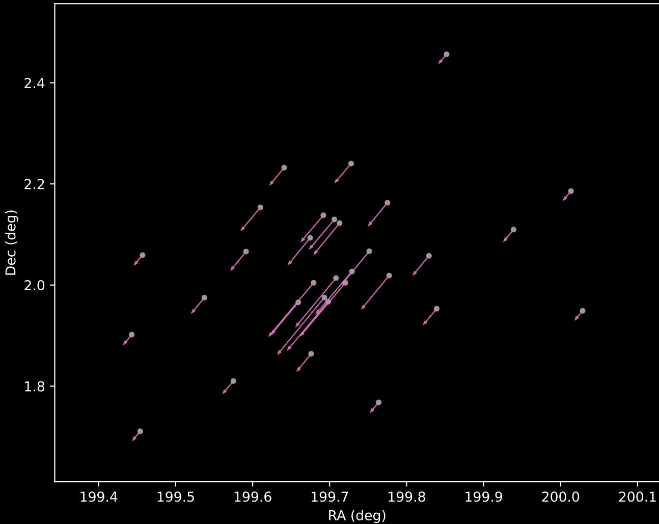
Gaia DR3 Cluster 52 Proper Motion Vectors (n=31)
