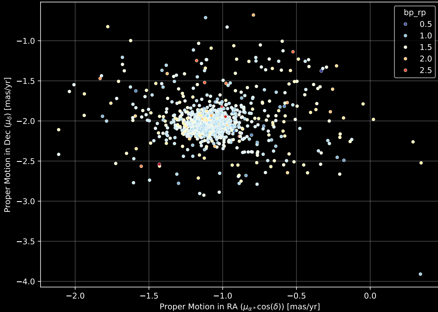
Gaia Cluster: [Collinder_110] Proper Motion Diagram (n= 1168)
