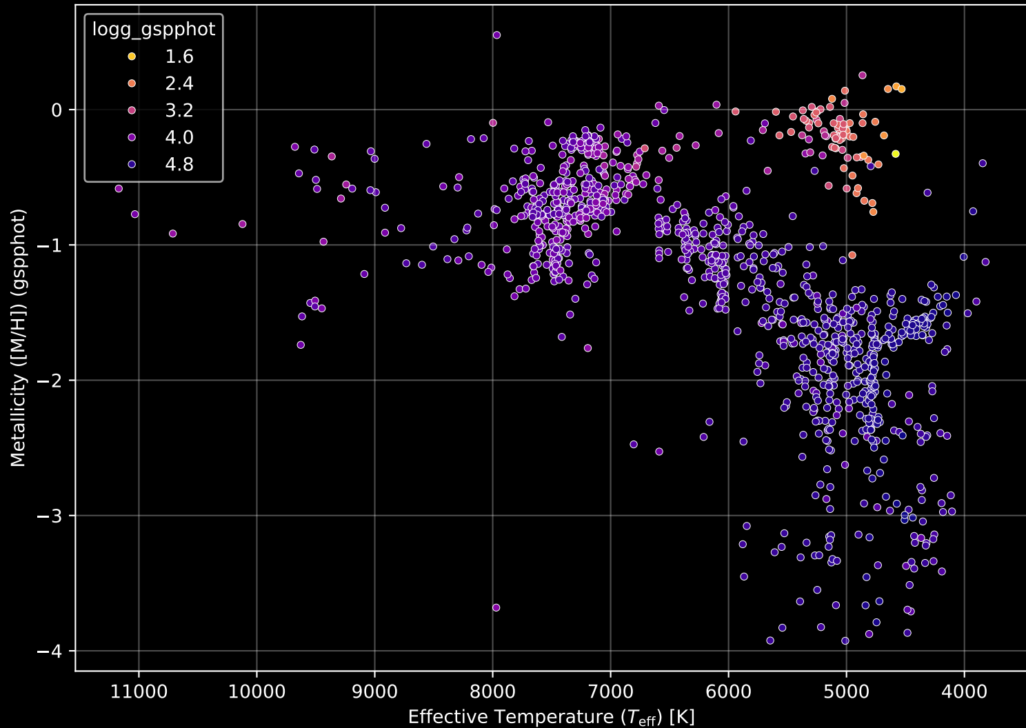
Gaia Cluster: [Collinder_110] Stellar Population Parameters (n= 1168)
