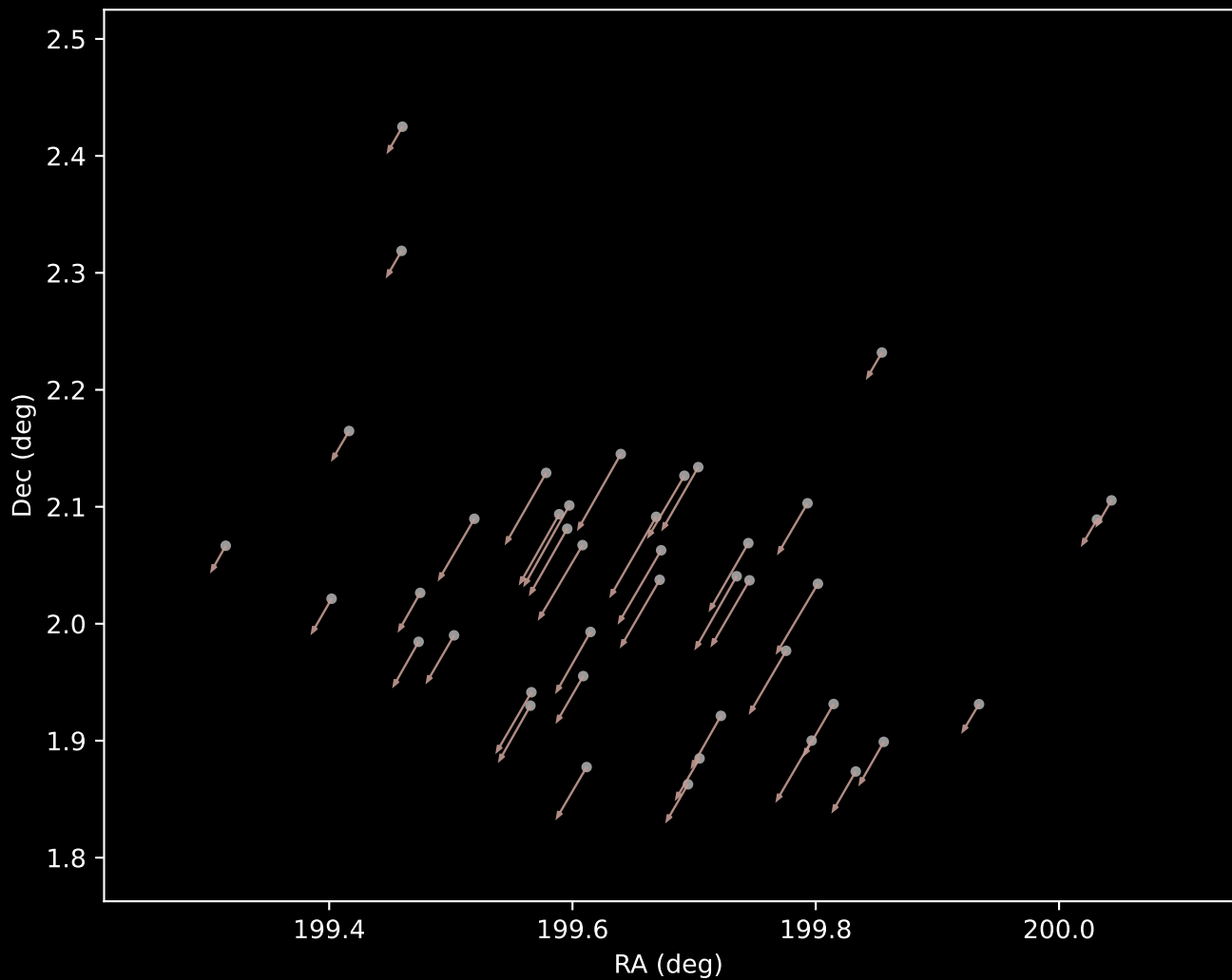
Gaia DR3 Cluster 51 Proper Motion Vectors (n=42)
