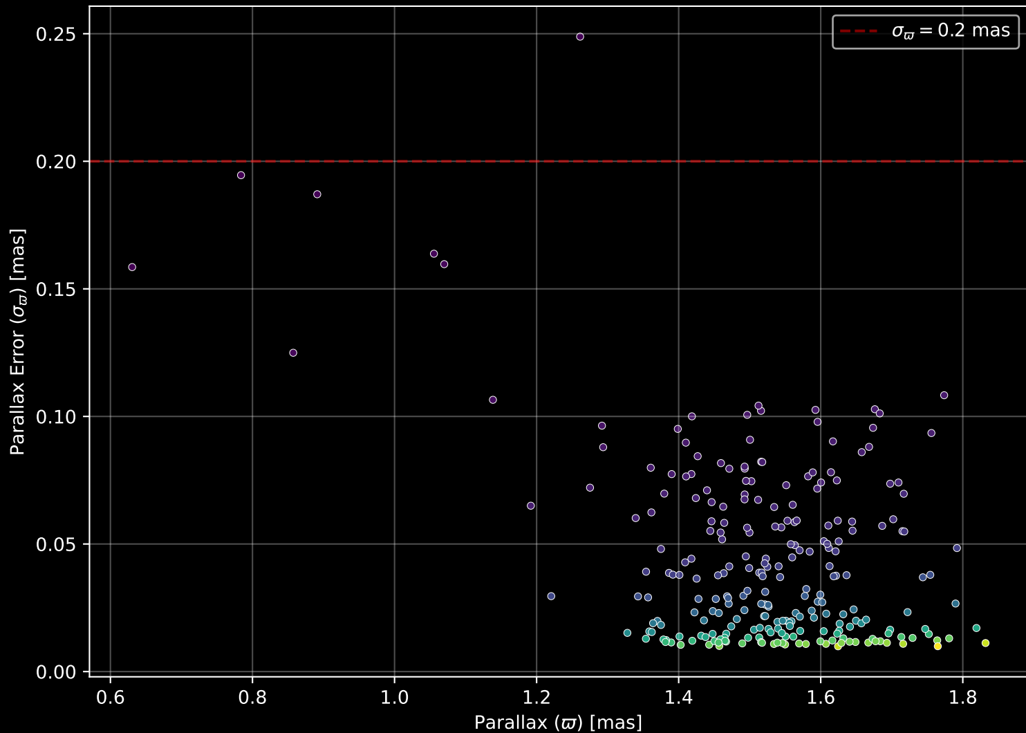
Gaia Cluster: [Collinder_132] Parallax Quality (n= 245)
