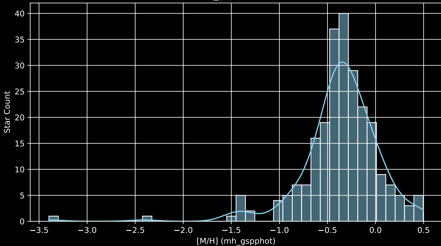
Gaia Cluster: [Collinder_132 [M/H] (mh_gspphot) (n= 244)
