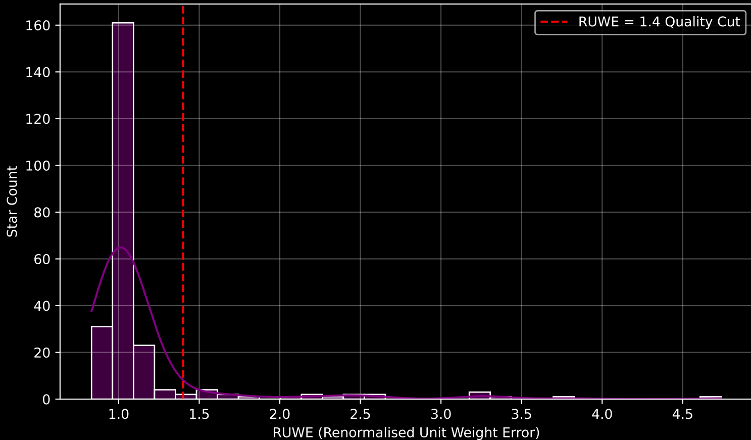
Gaia Cluster: [Collinder_132] RUWE Distribution (n= 242)
