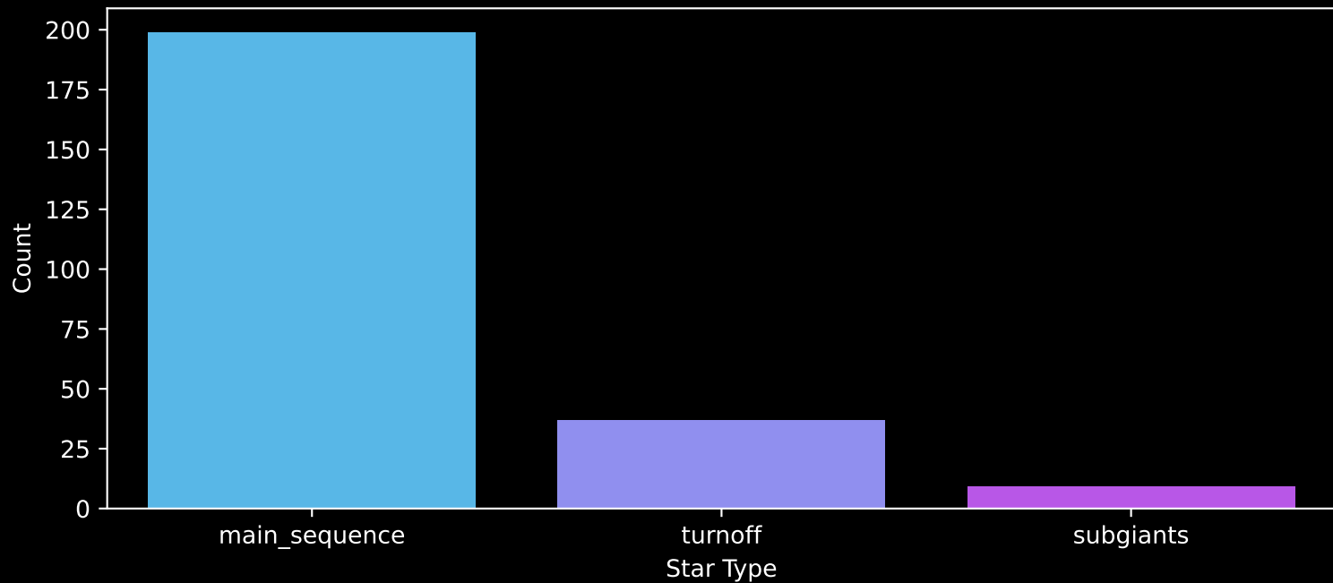
Gaia Cluster: [Collinder_132] Count plot of Star Type
