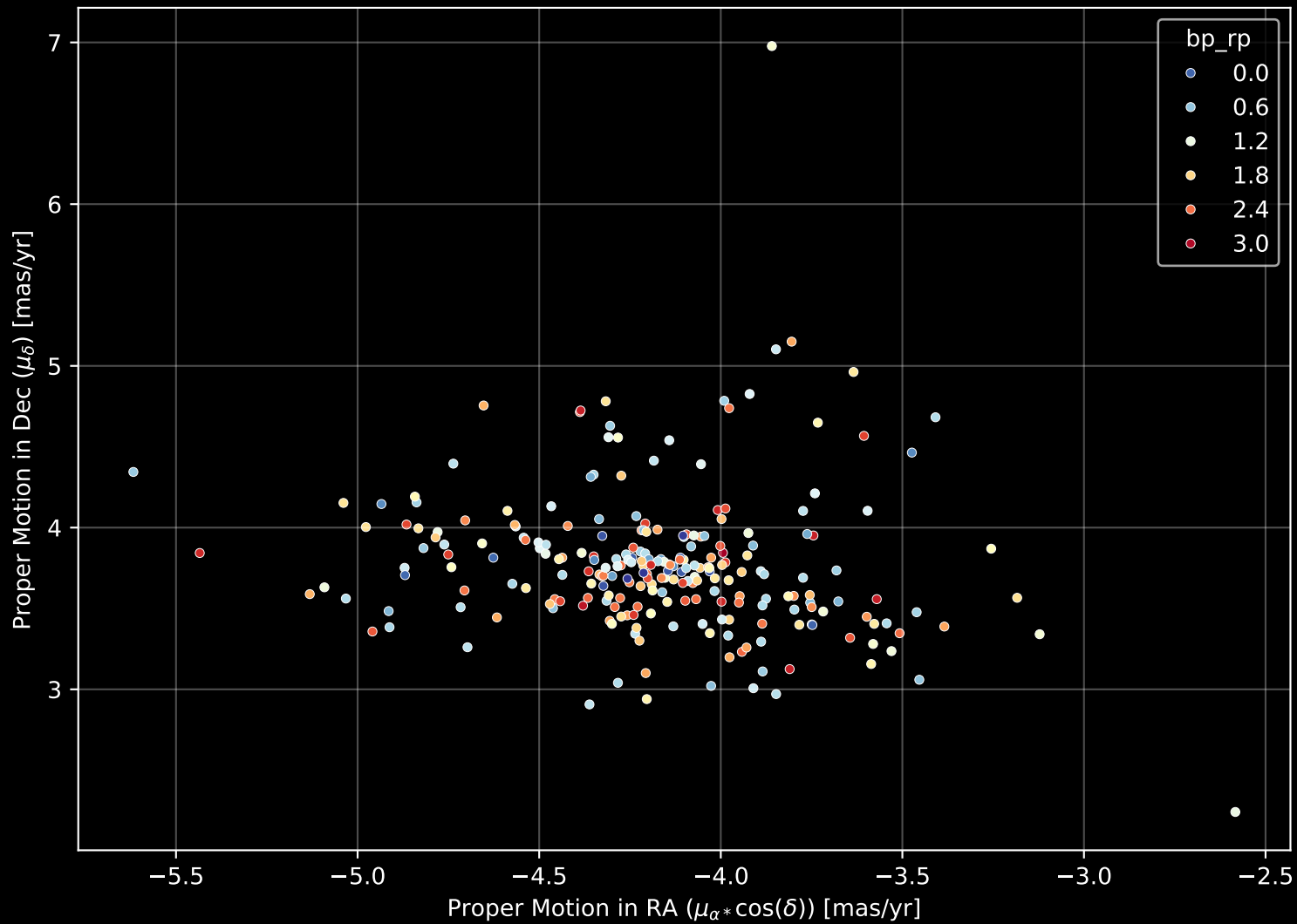
Gaia Cluster: [Collinder_132] Proper Motion Diagram (n= 245)
