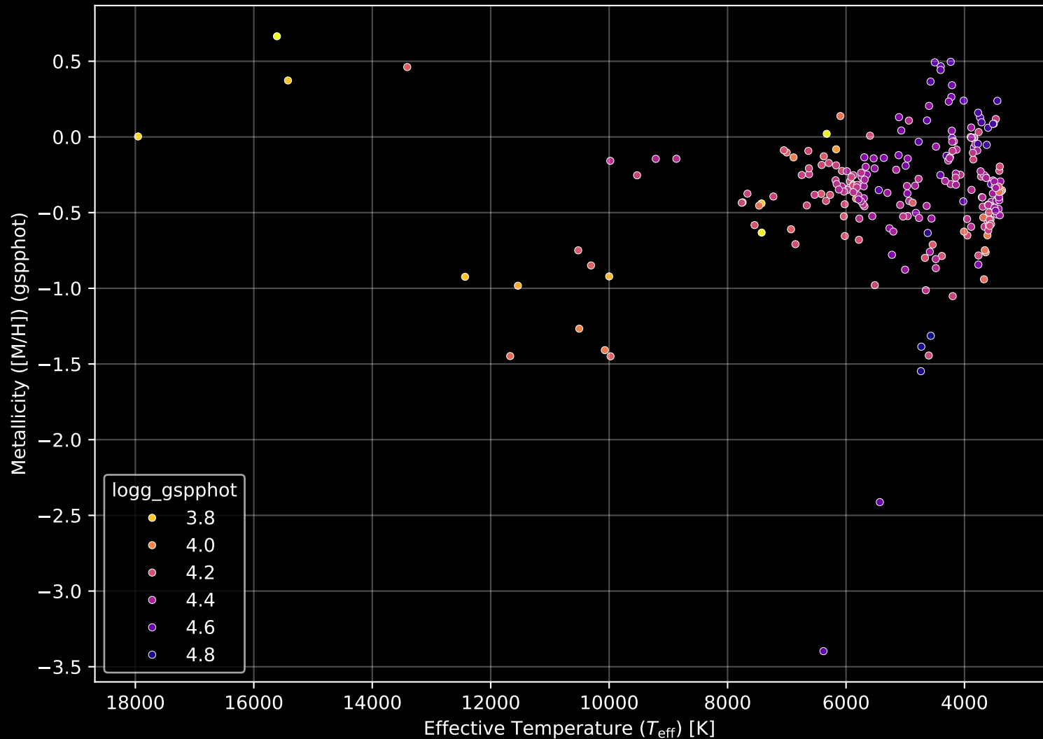
Gaia Cluster: [Collinder_132] Stellar Population Parameters (n= 245)
