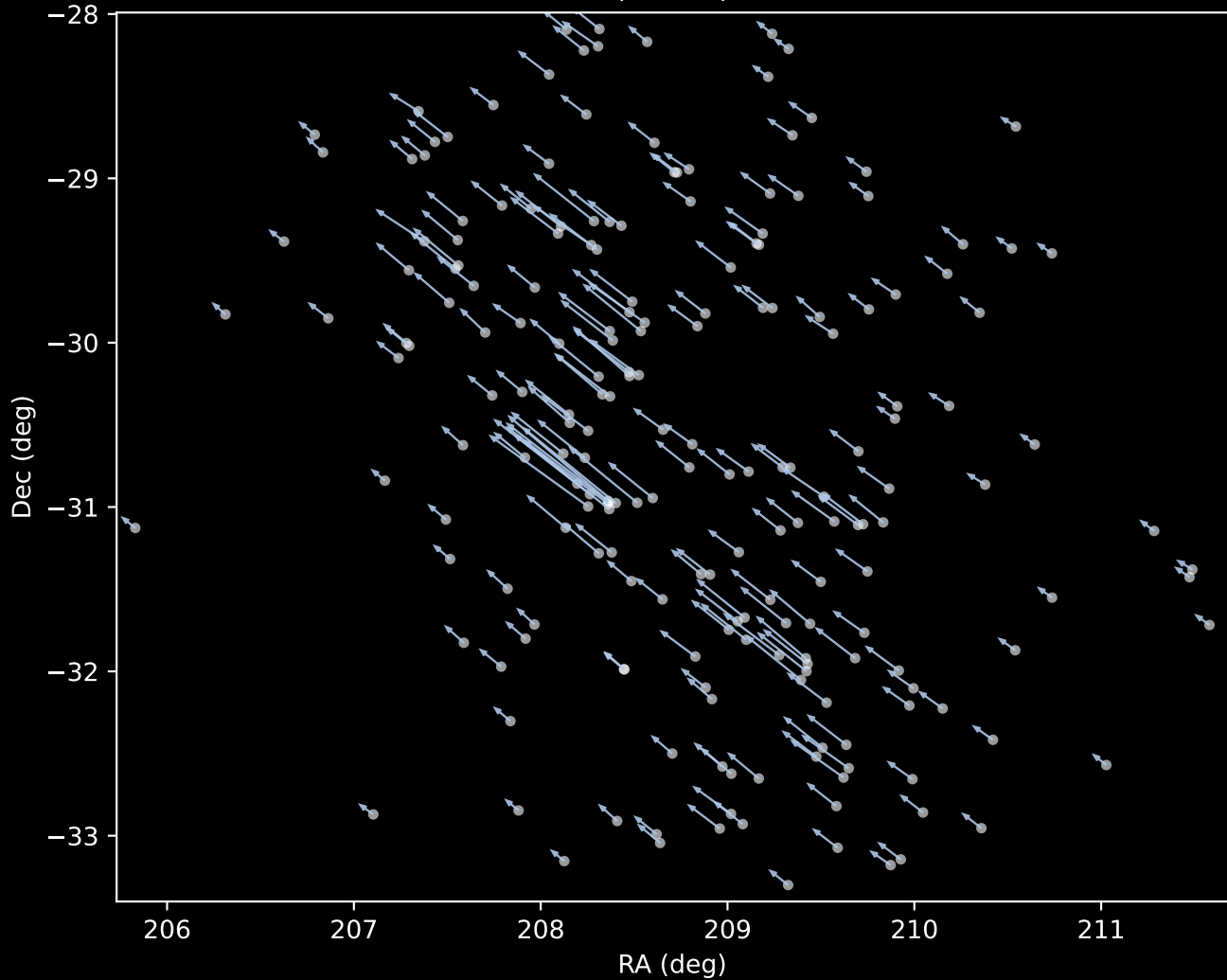
Gaia DR3 Cluster 1 Proper Motion Vectors (n=205)
