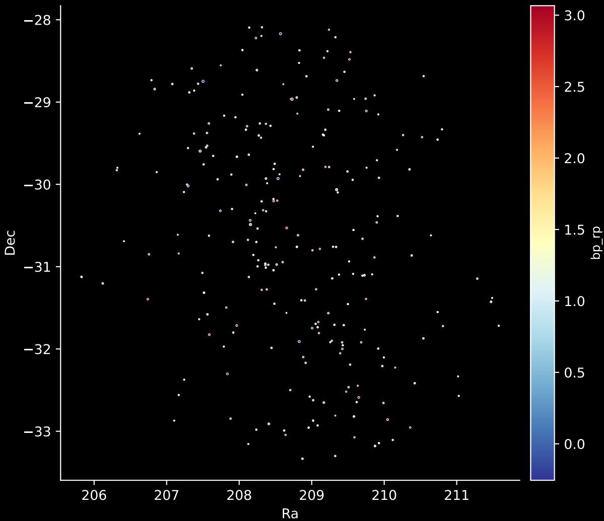
Gaia Cluster: [Collinder_132] Stars: 245
