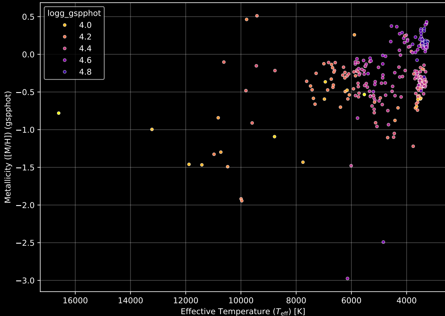
Gaia Cluster: [Collinder_135] Stellar Population Parameters (n= 321)
