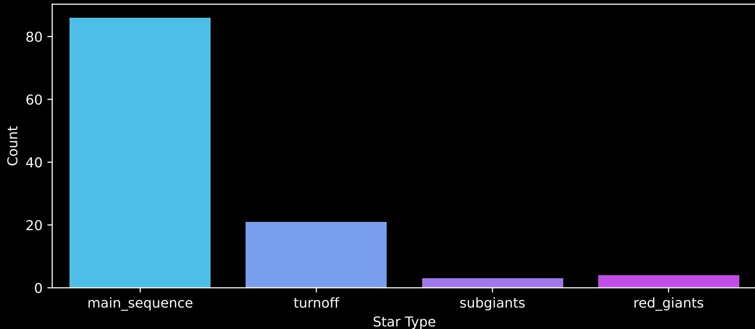
Gaia Cluster: [Collinder_185] Count plot of Star Type
