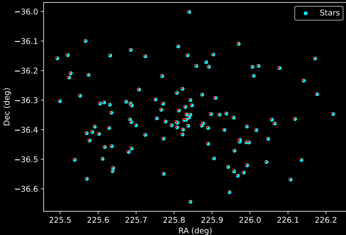
Gaia Cluster: [Collinder_185] Proper Motion Vectors for Gaia Star Field (n= 114)
