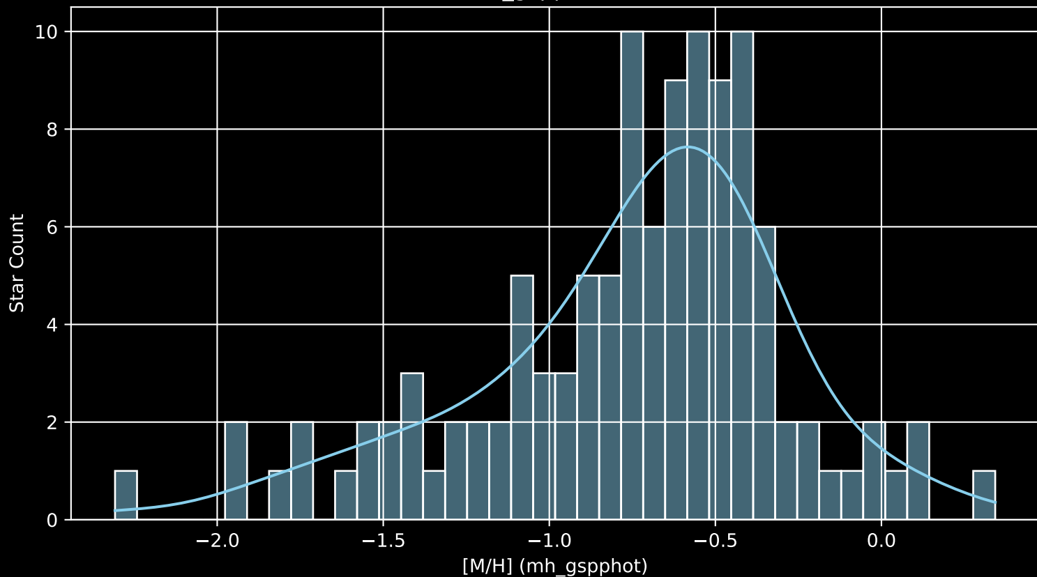
Gaia Cluster: [Collinder_185 [M/H] (mh_gspphot) (n= 114)
