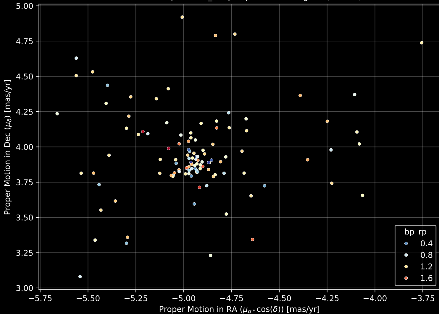
Gaia Cluster: [Collinder_185] Proper Motion Diagram (n= 114)
