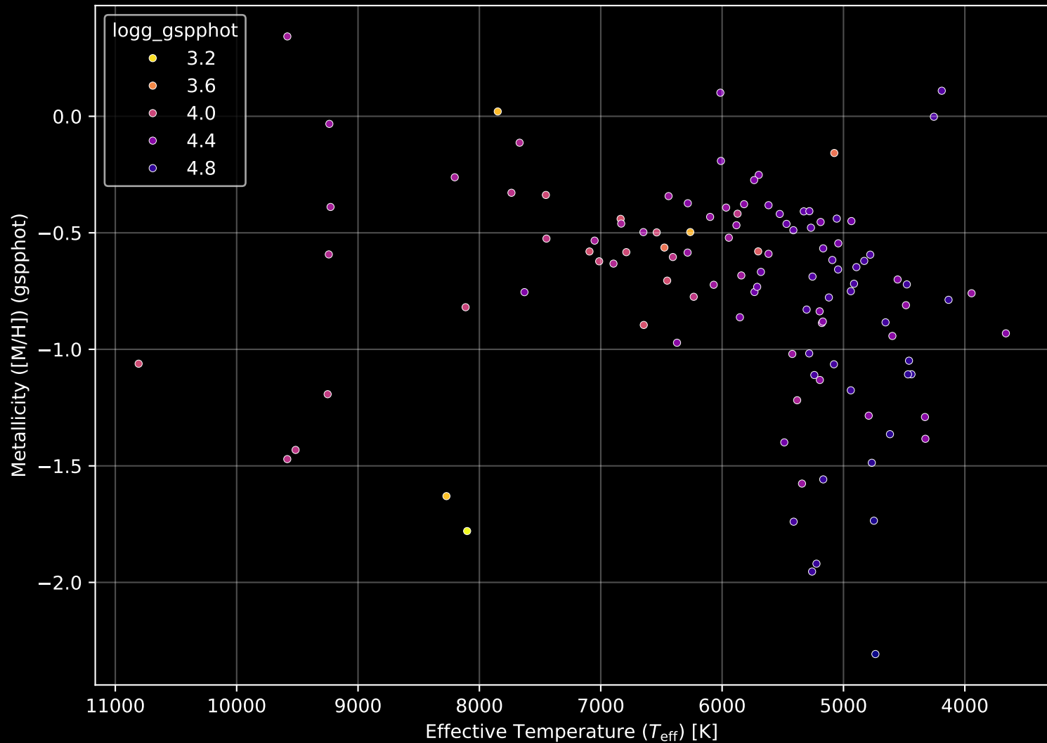
Gaia Cluster: [Collinder_185] Stellar Population Parameters (n= 114)
