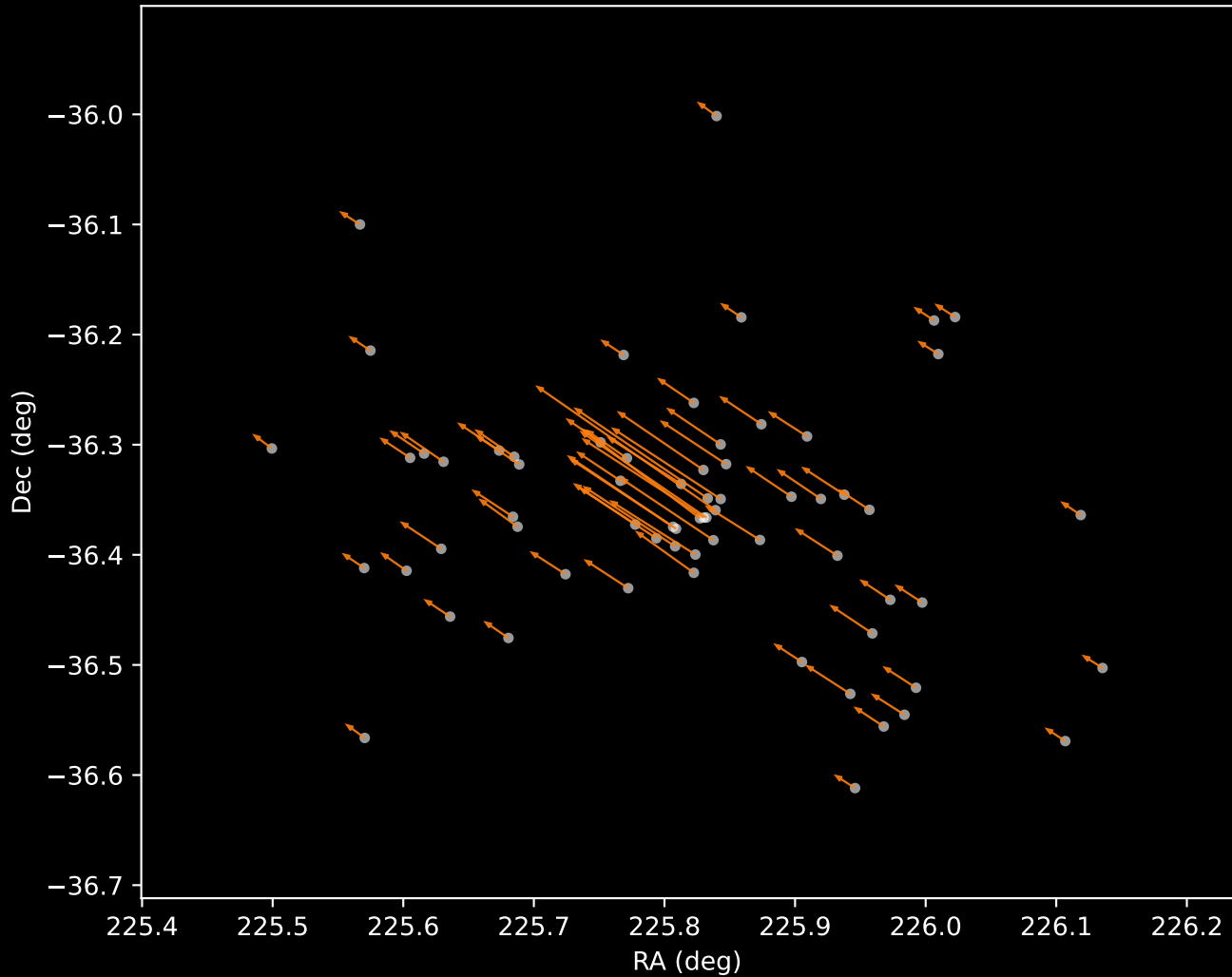
Gaia DR3 Cluster 2 Proper Motion Vectors (n=67)
