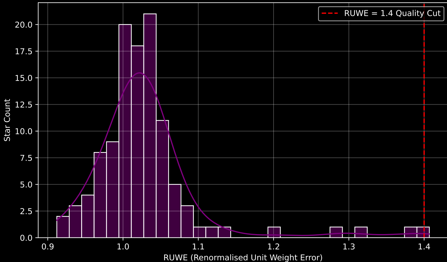
Gaia Cluster: [Collinder_185] RUWE Distribution (n= 112)
