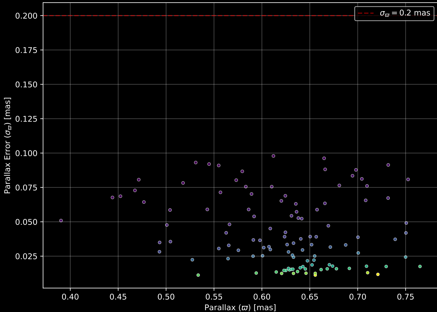
Gaia Cluster: [Collinder_185] Parallax Quality (n= 114)
