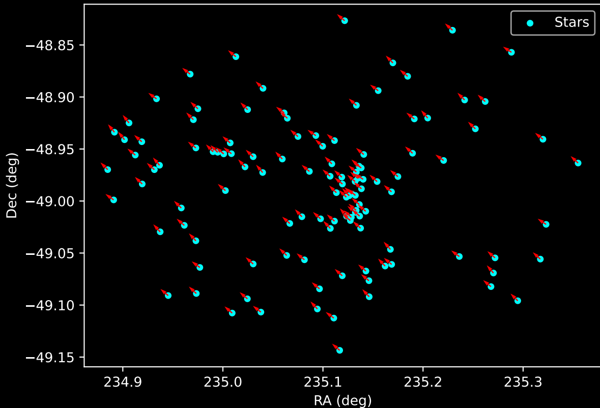
Gaia Cluster: [Collinder_205] Proper Motion Vectors for Gaia Star Field (n= 116)
