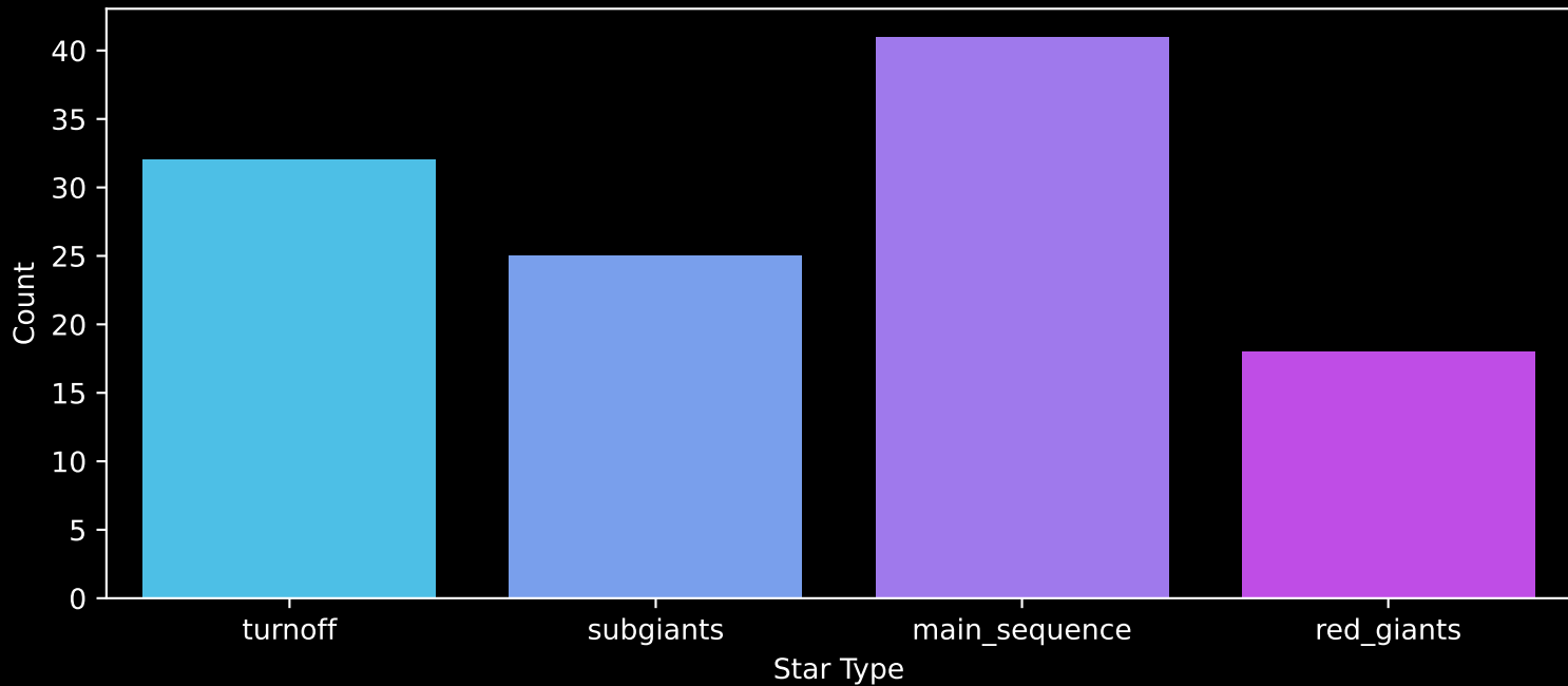
Gaia Cluster: [Collinder_205] Count plot of Star Type
