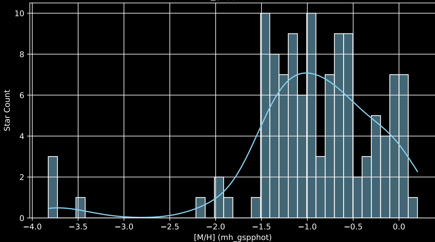
Gaia Cluster: [Collinder_205 [M/H] (mh_gspphot) (n= 116)
