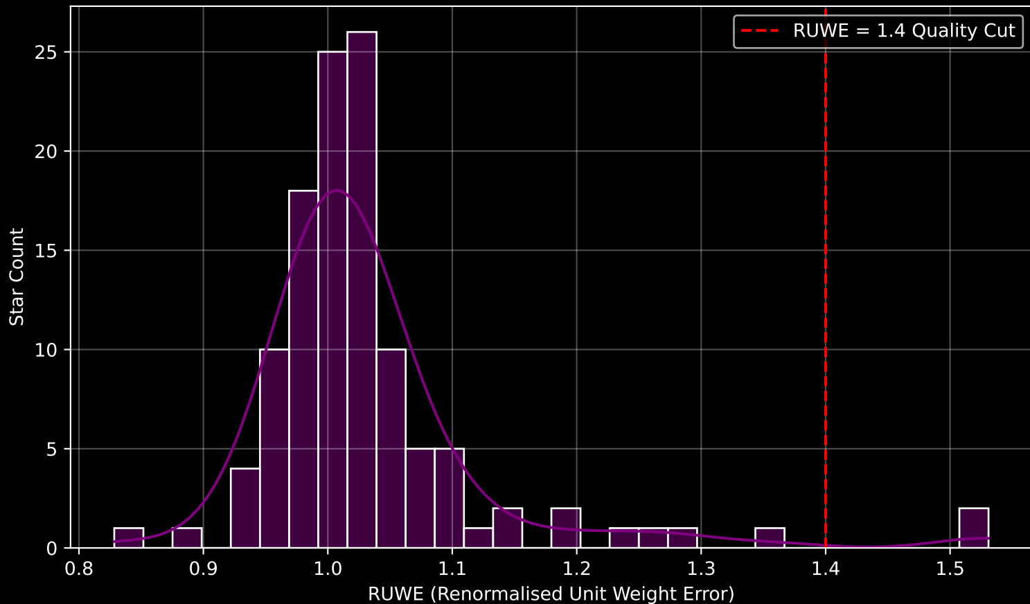
Gaia Cluster: [Collinder_205] RUWE Distribution (n= 116)
