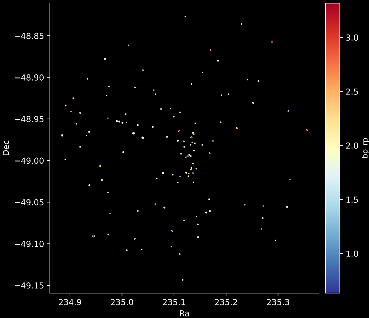
Gaia Cluster: [Collinder_205] Stars: 116
