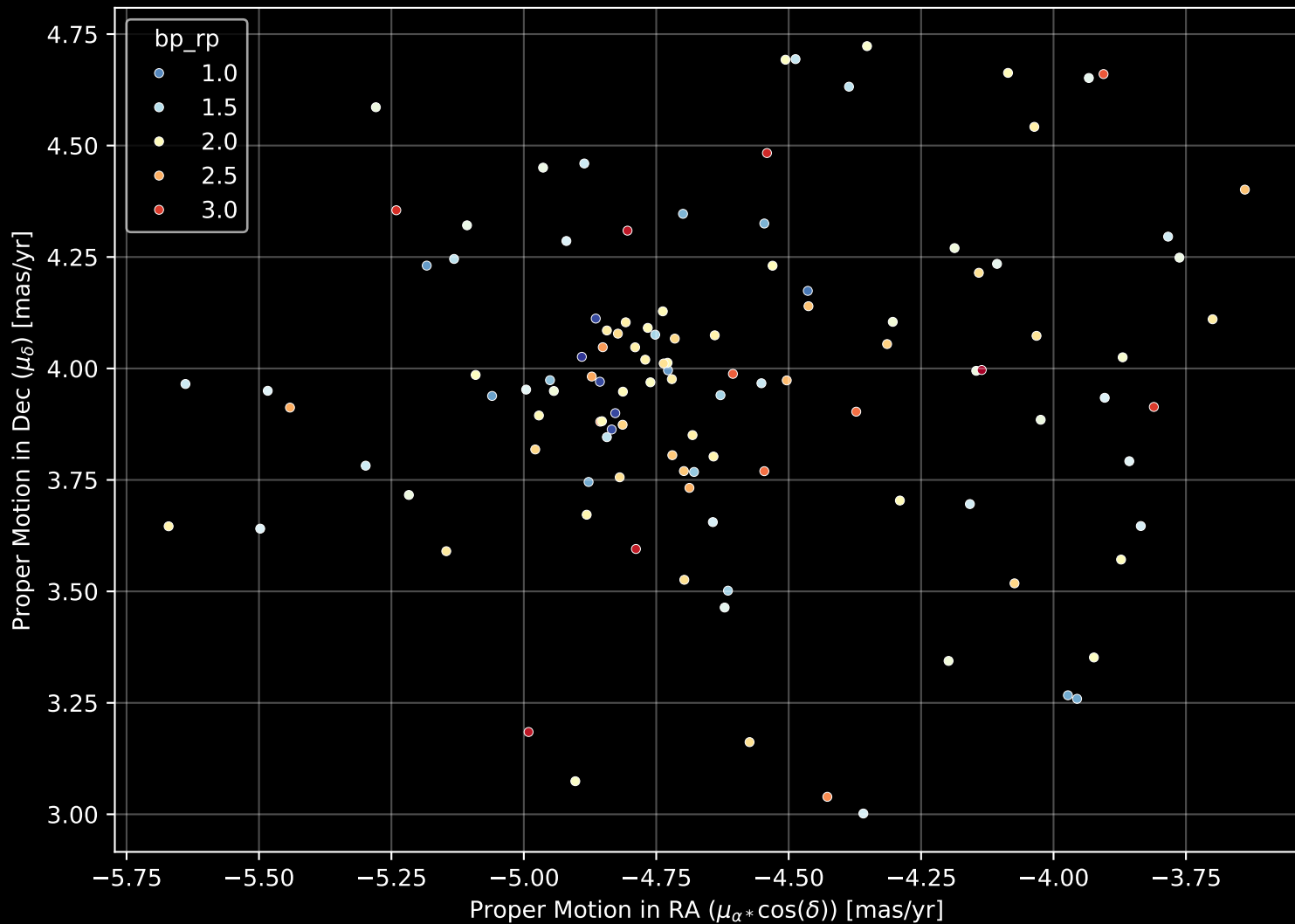
Gaia Cluster: [Collinder_205] Proper Motion Diagram (n= 116)
