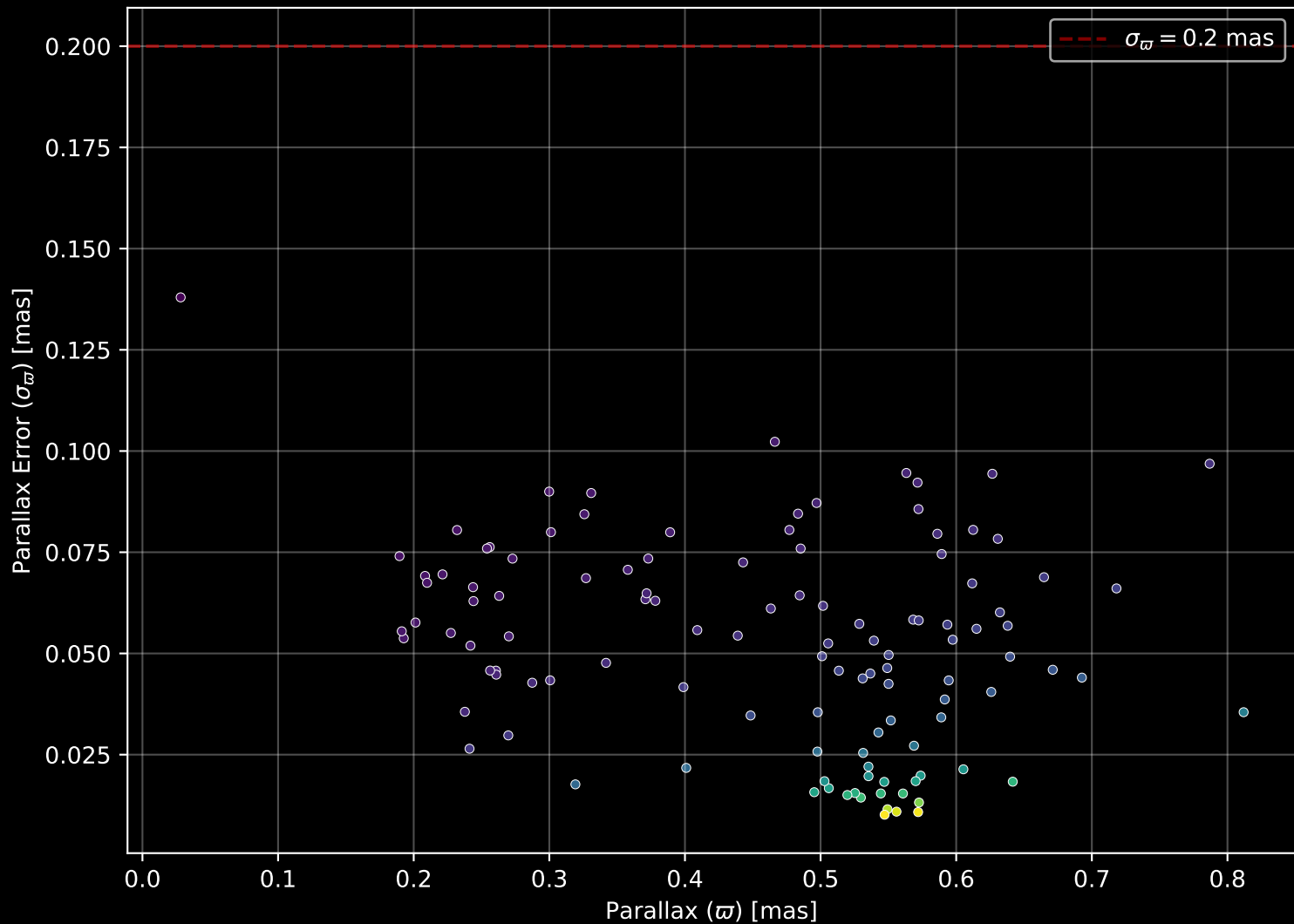
Gaia Cluster: [Collinder_205] Parallax Quality (n= 116)
