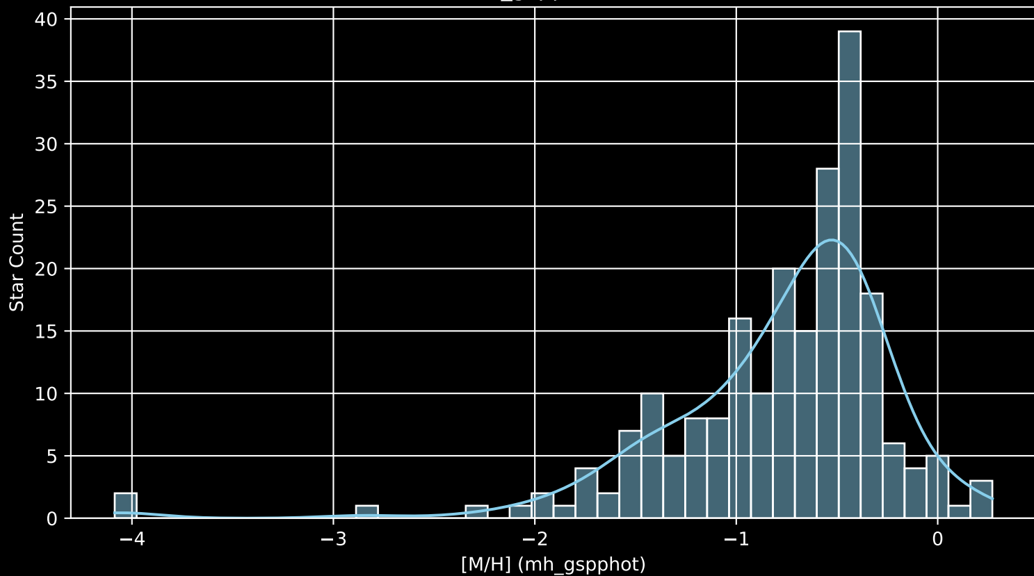
Gaia Cluster: [Collinder_258 [M/H] (mh_gspphot) (n= 217)
