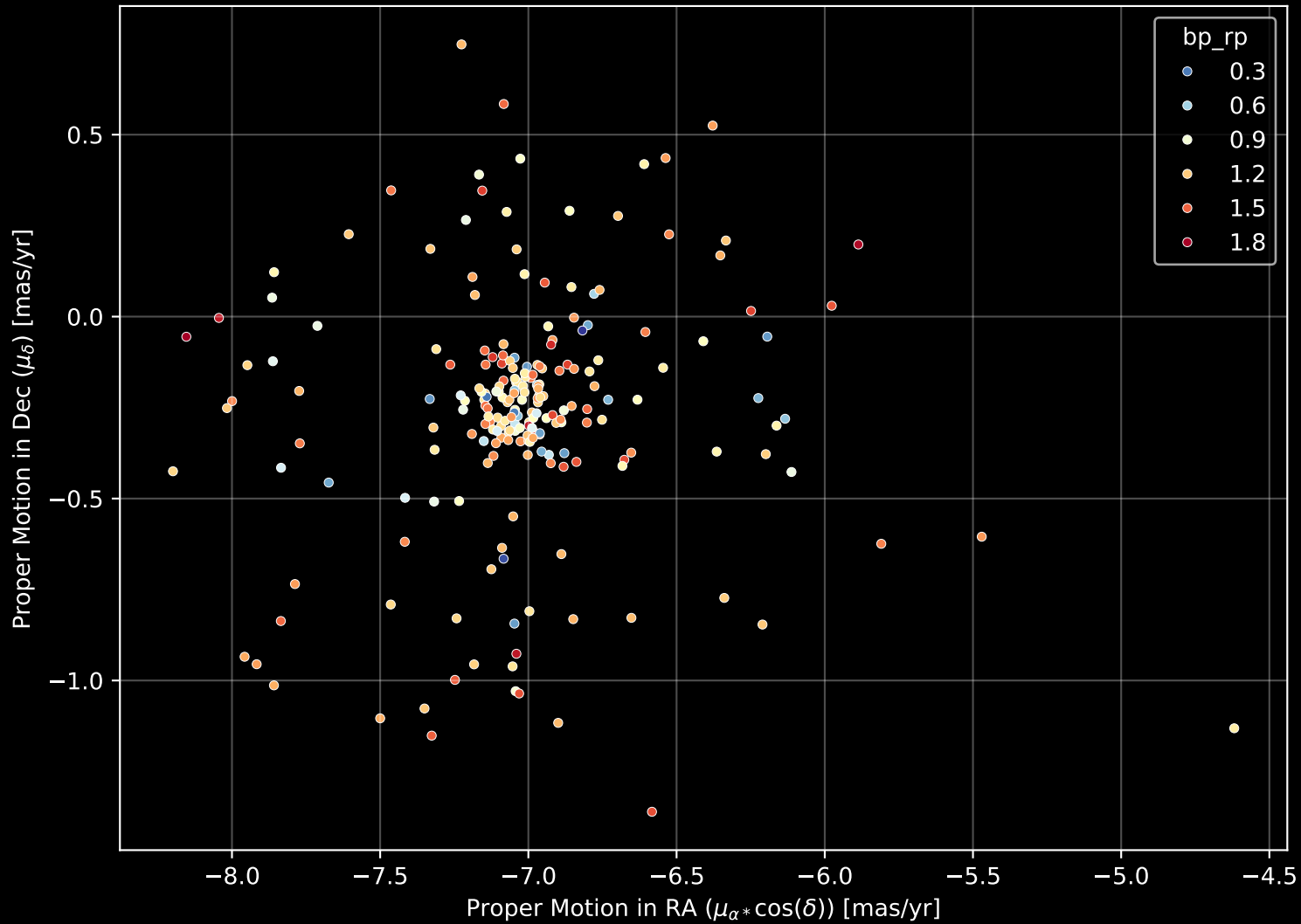
Gaia Cluster: [Collinder_258] Proper Motion Diagram (n= 217)
