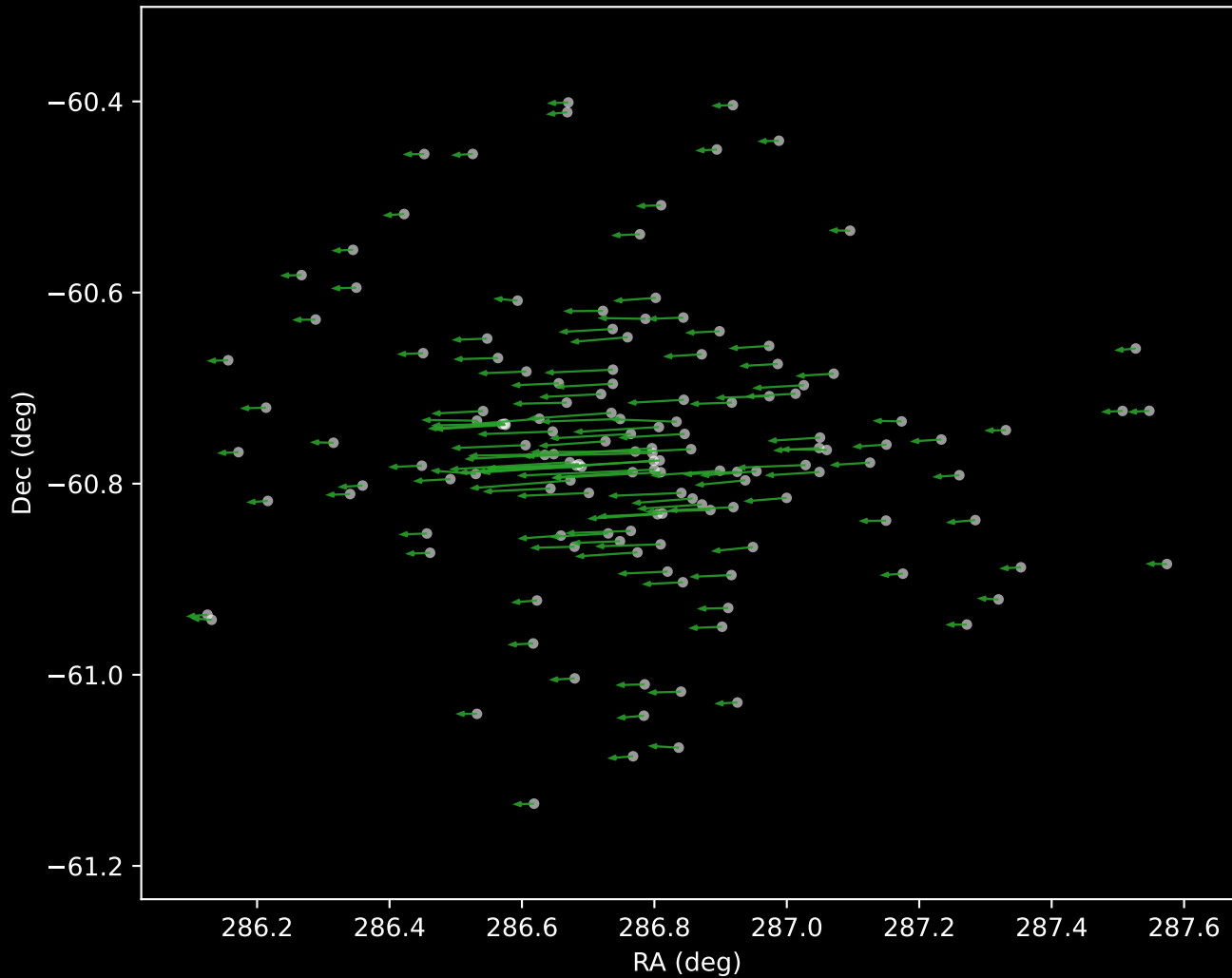
Gaia DR3 Cluster 4 Proper Motion Vectors (n=145)
