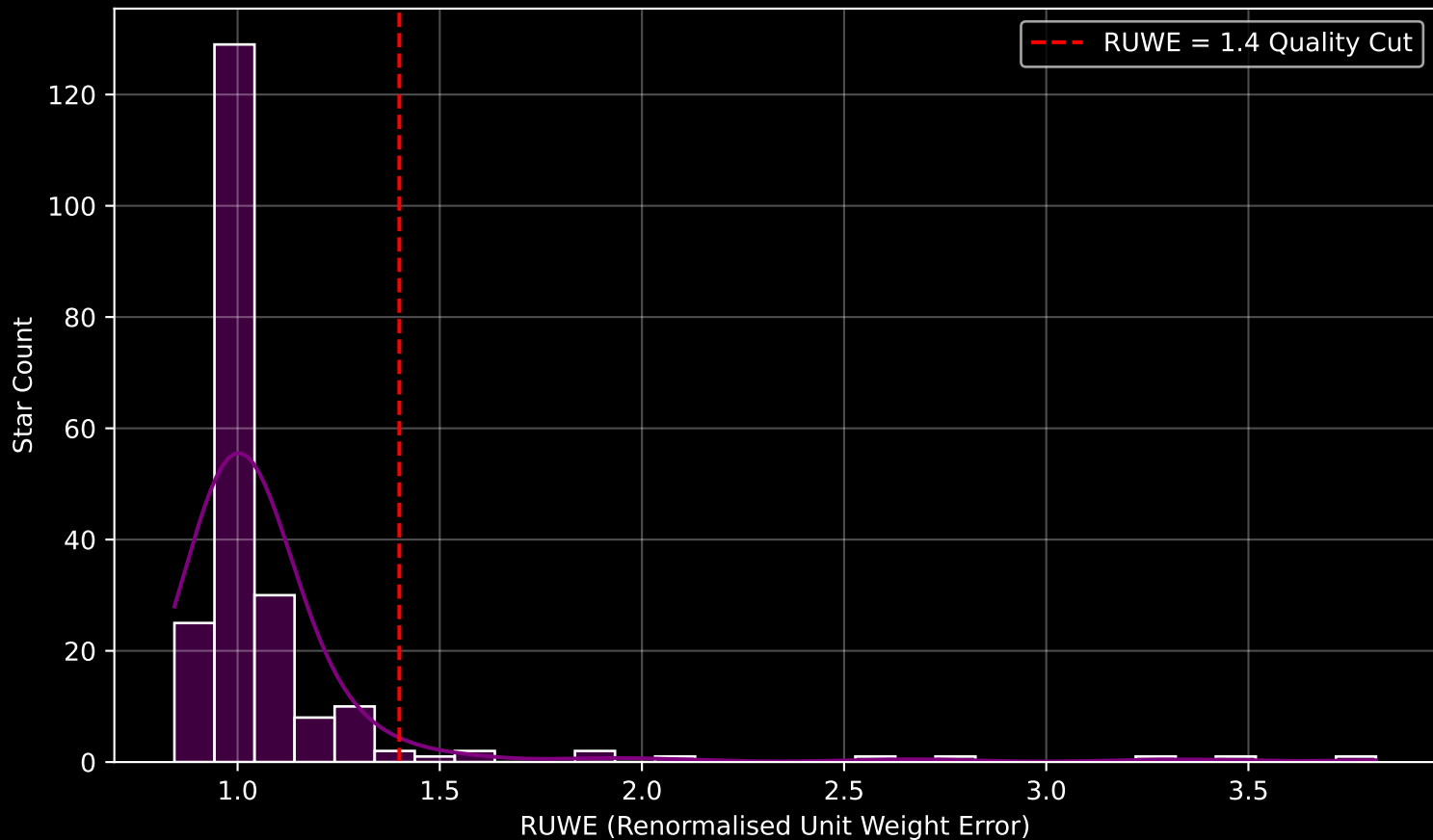
Gaia Cluster: [Collinder_258] RUWE Distribution (n= 215)
