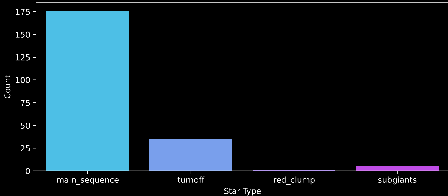
Gaia Cluster: [Collinder_258] Count plot of Star Type
