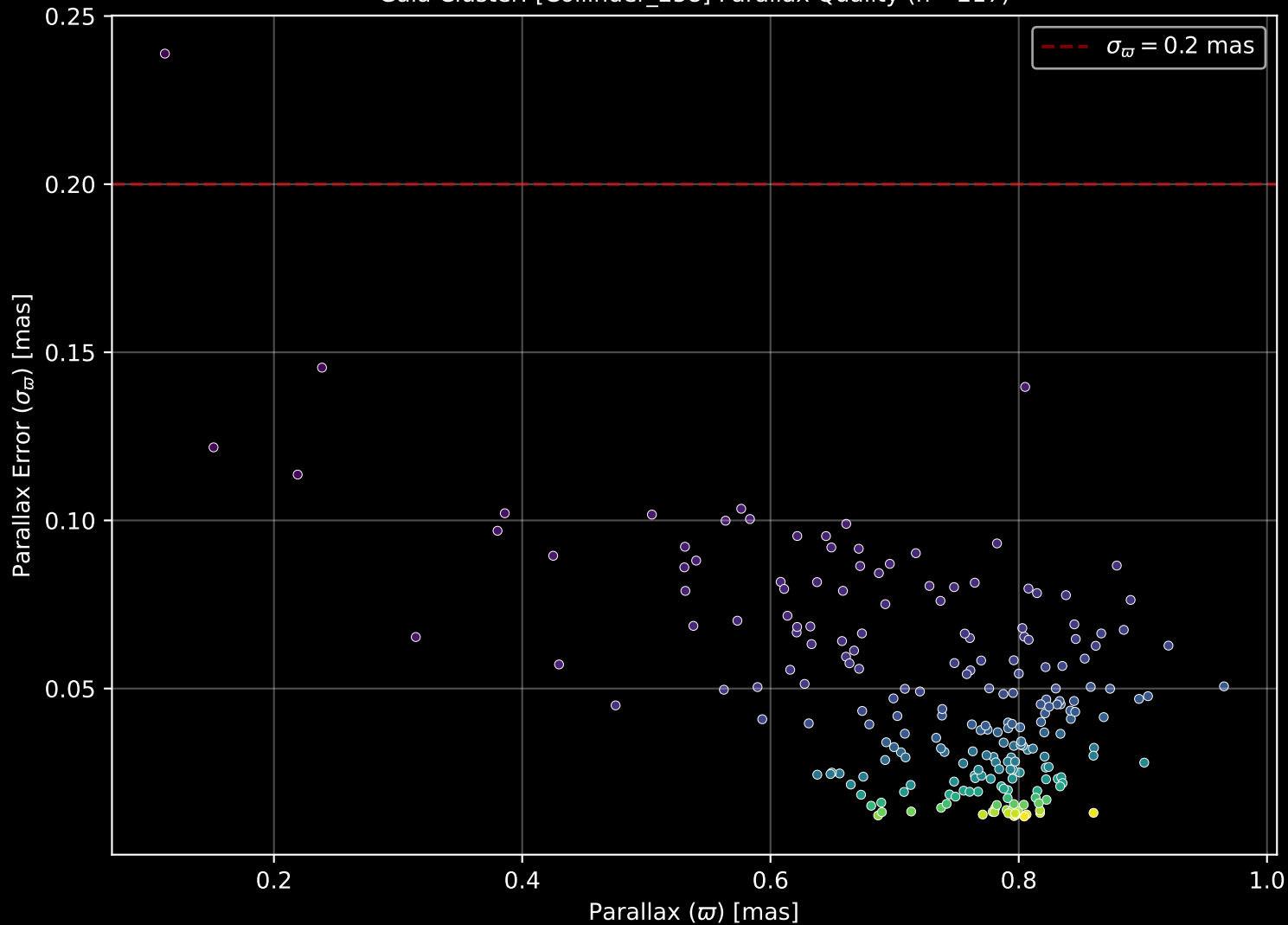
Gaia Cluster: [Collinder_258] Parallax Quality (n= 217)
