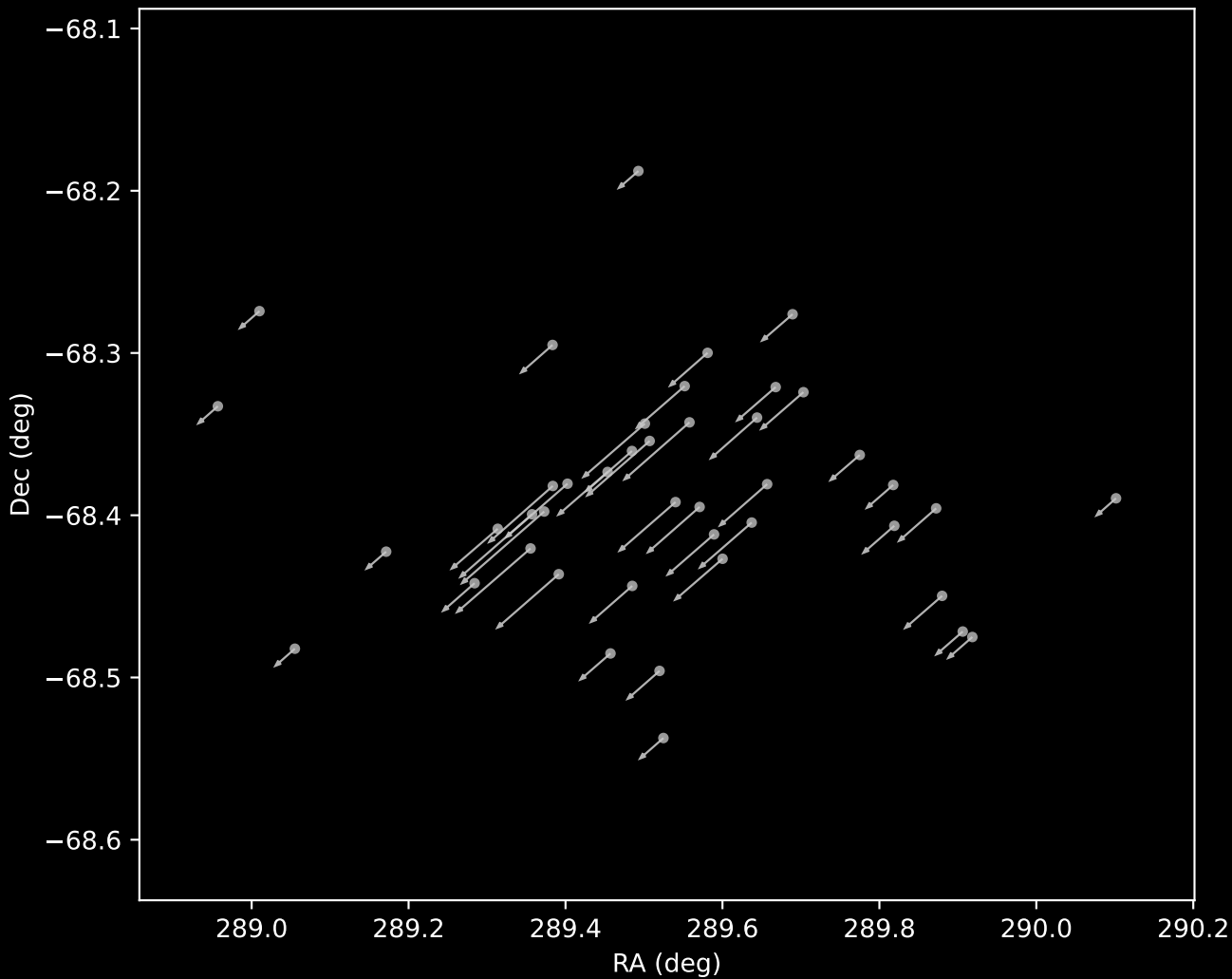
Gaia DR3 Cluster 75 Proper Motion Vectors (n=43)
