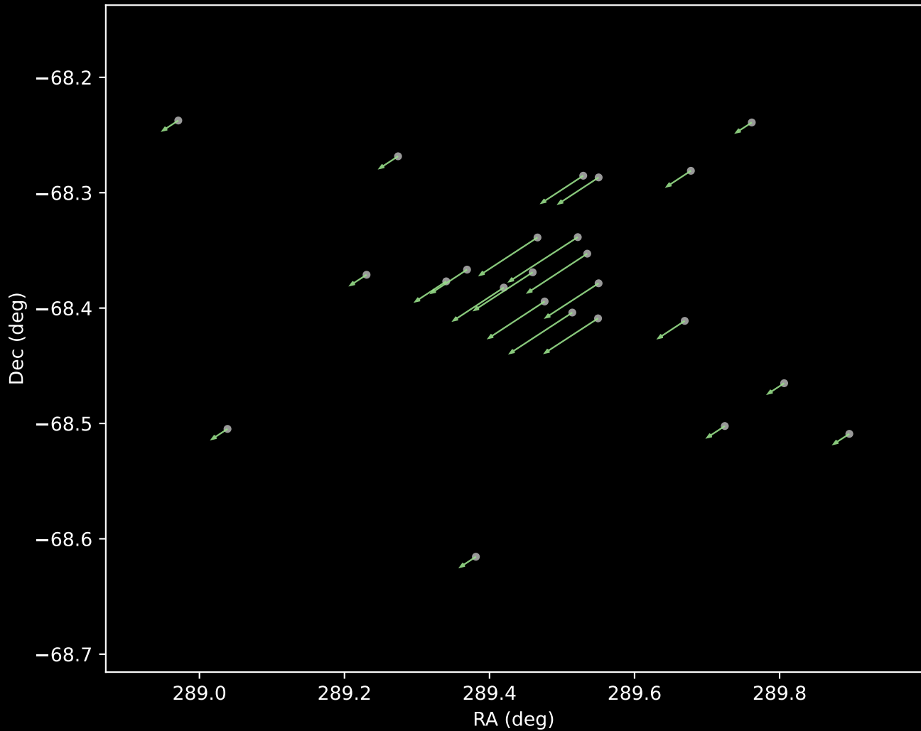
Gaia DR3 Cluster 85 Proper Motion Vectors (n=24)
