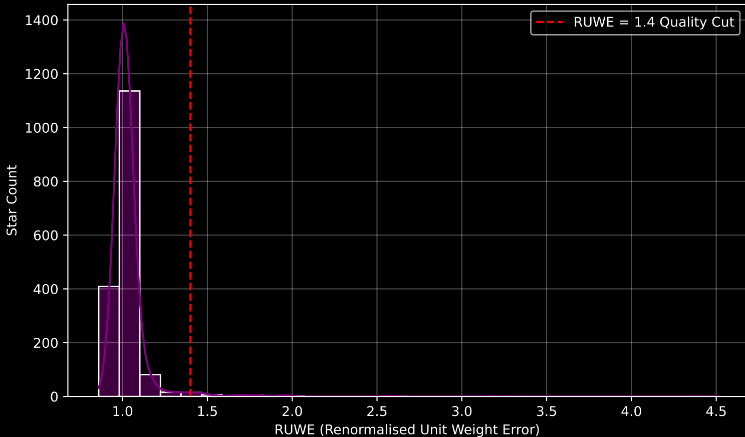
Gaia Cluster: [Collinder_261] RUWE Distribution (n= 1680)
