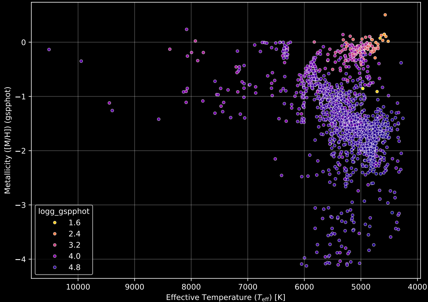
Gaia Cluster: [Collinder_261] Stellar Population Parameters (n= 1680)
