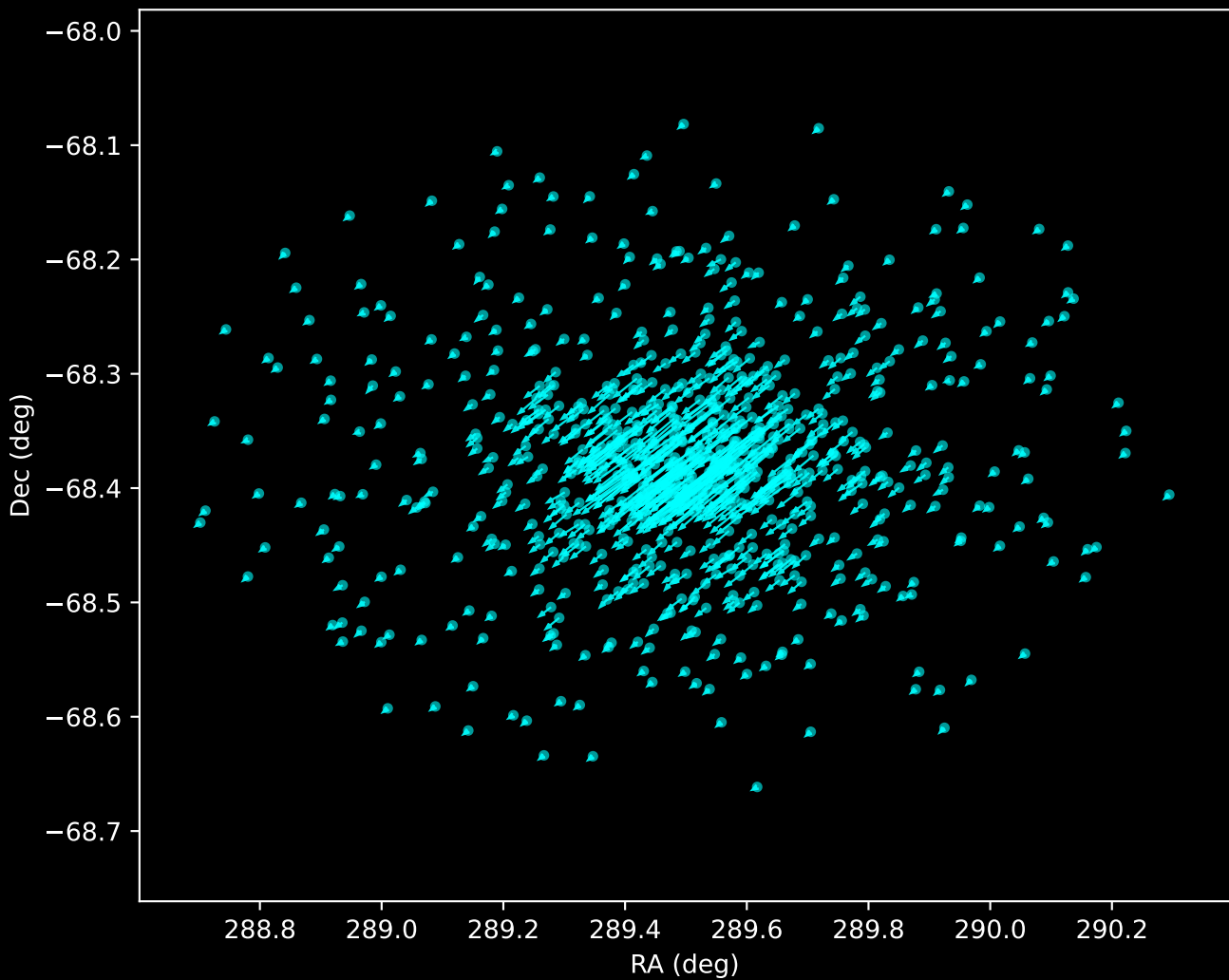
Gaia DR3 Noise Stream Proper Motion Vectors (n=746)
