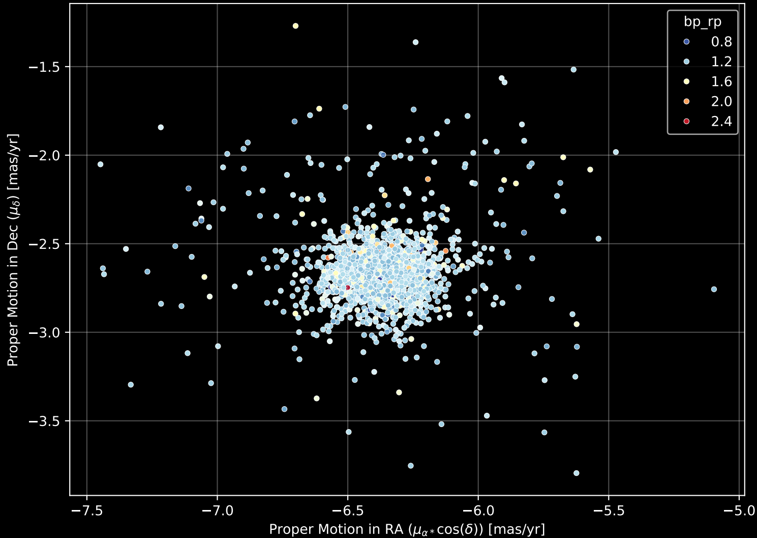
Gaia Cluster: [Collinder_261] Proper Motion Diagram (n= 1680)
