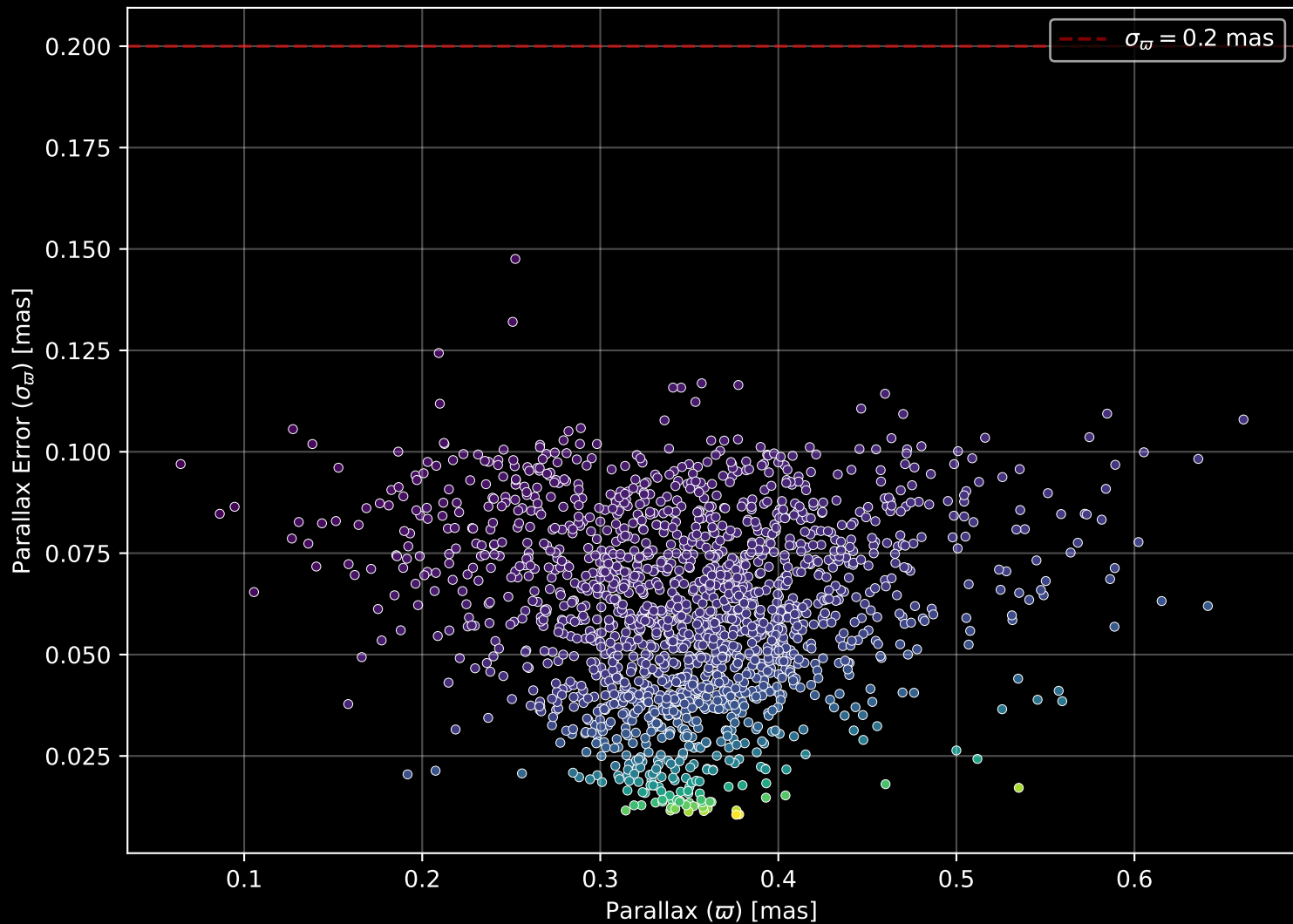
Gaia Cluster: [Collinder_261] Parallax Quality (n= 1680)
