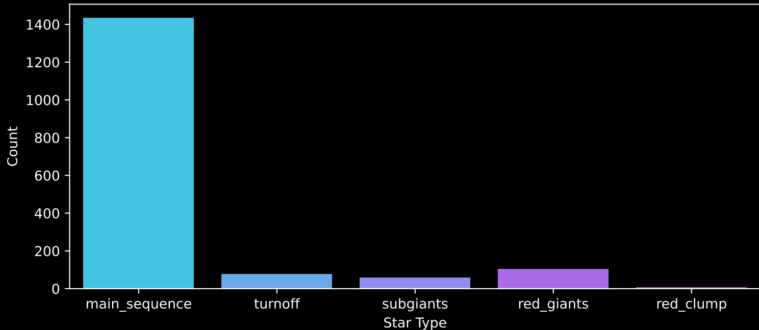
Gaia Cluster: [Collinder_261] Count plot of Star Type
