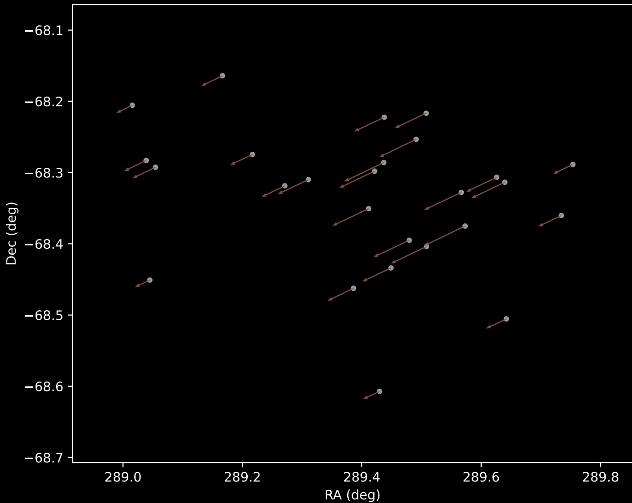
Gaia DR3 Cluster 30 Proper Motion Vectors (n=26)
