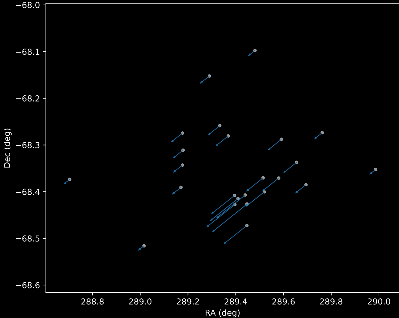
Gaia DR3 Cluster 60 Proper Motion Vectors (n=24)
