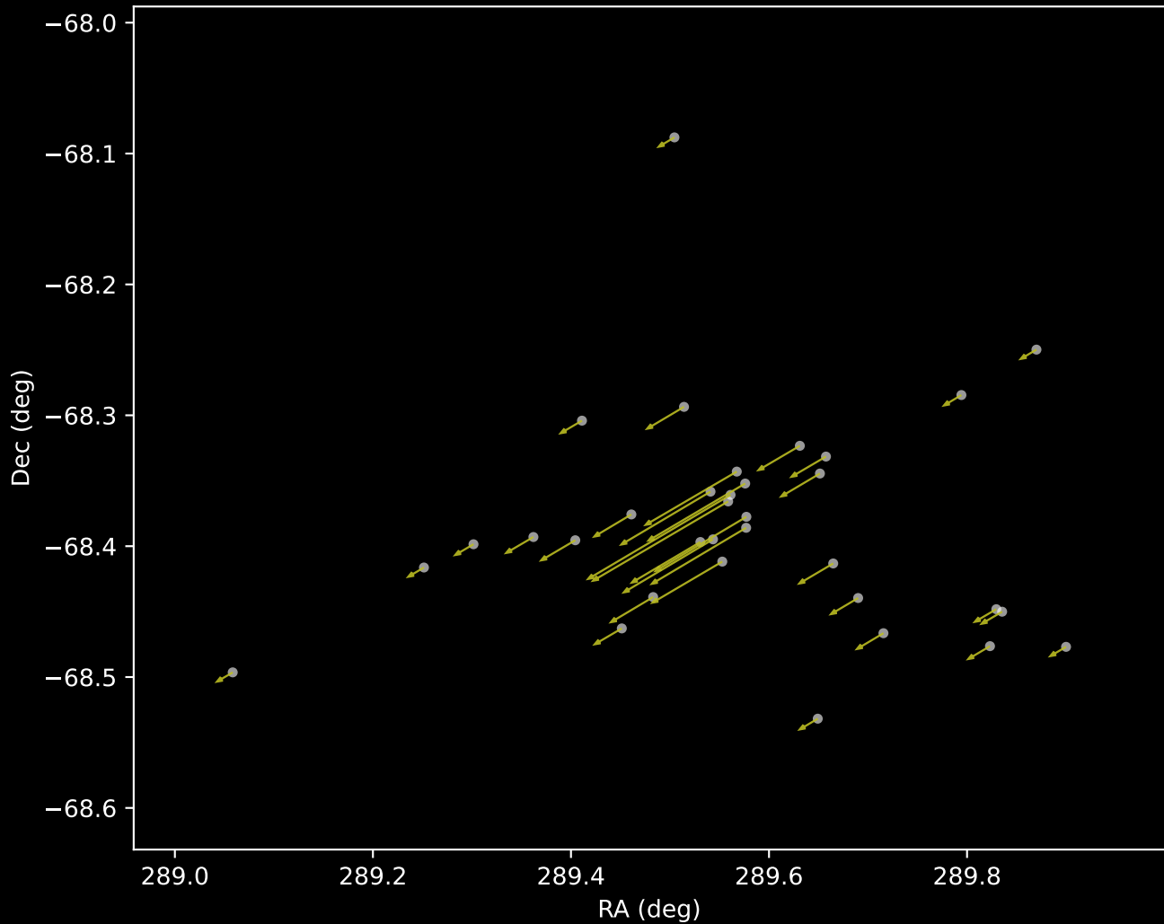
Gaia DR3 Cluster 36 Proper Motion Vectors (n=34)
