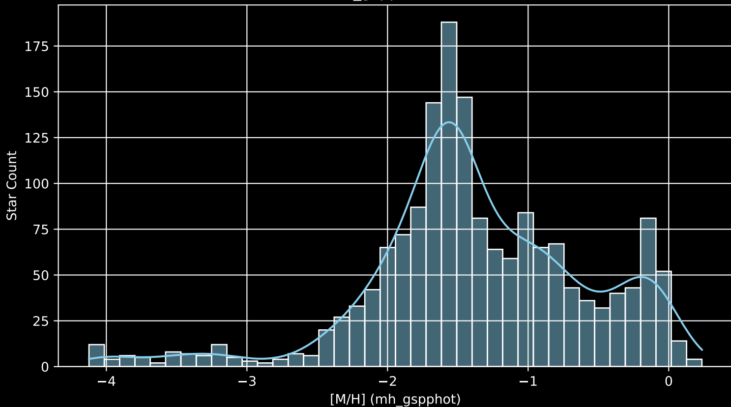
Gaia Cluster: [Collinder_261 [M/H] (mh_gspphot) (n= 1679)
