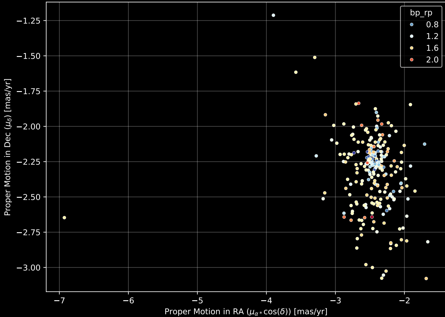
Gaia Cluster: [Collinder_292] Proper Motion Diagram (n= 247)
