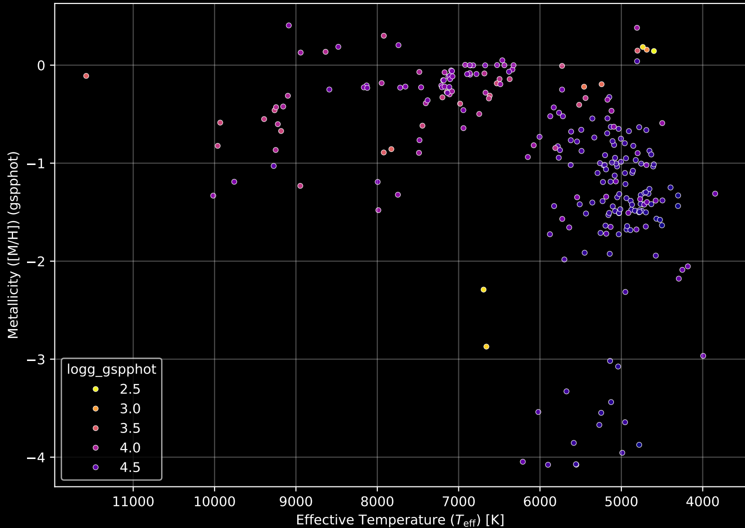
Gaia Cluster: [Collinder_292] Stellar Population Parameters (n= 247)
