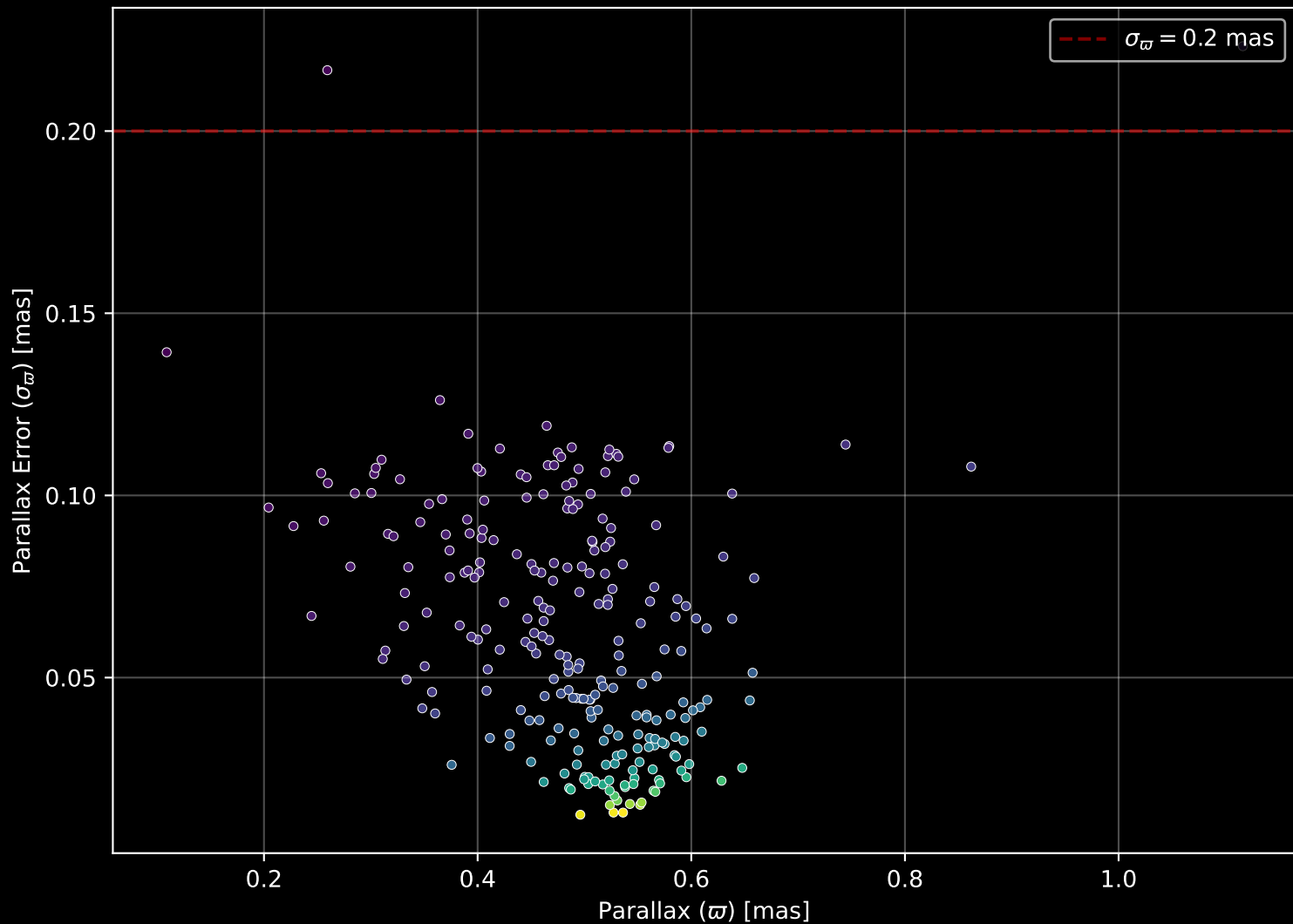
Gaia Cluster: [Collinder_292] Parallax Quality (n= 247)
