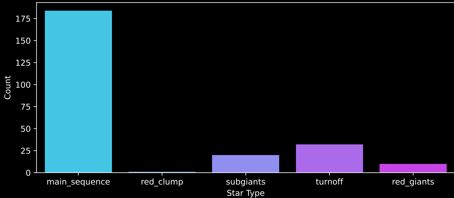
Gaia Cluster: [Collinder_292] Count plot of Star Type
