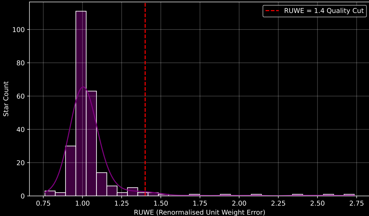
Gaia Cluster: [Collinder_292] RUWE Distribution (n= 247)
