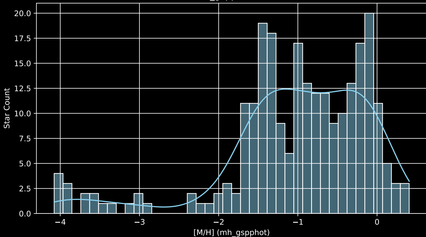
Gaia Cluster: [Collinder_292 [M/H] (mh_gspphot) (n= 247)
