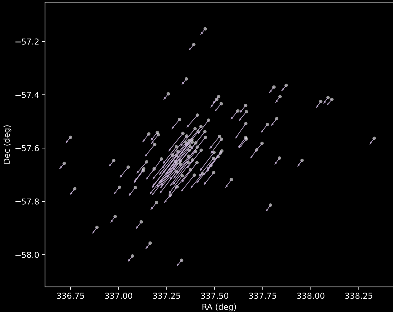
Gaia DR3 Cluster 9 Proper Motion Vectors (n=100)
