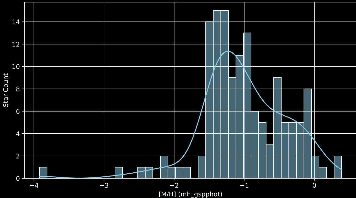
Gaia Cluster: [Collinder_307 [M/H] (mh_gspphot) (n= 139)
