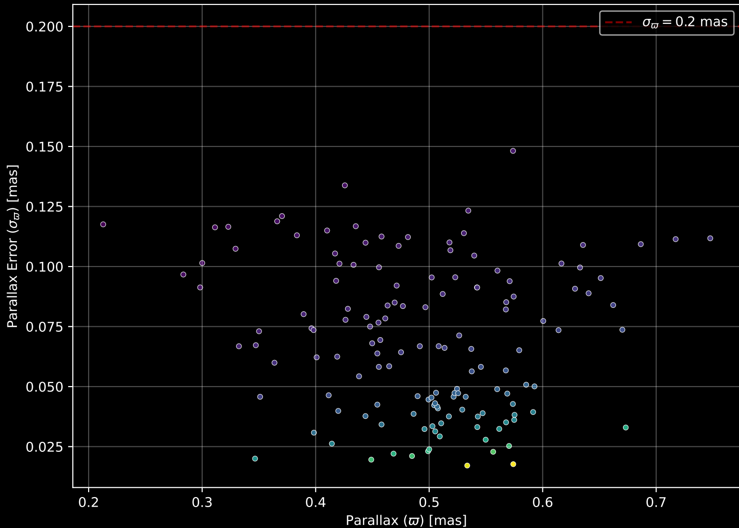
Gaia Cluster: [Collinder_307] Parallax Quality (n= 141)
