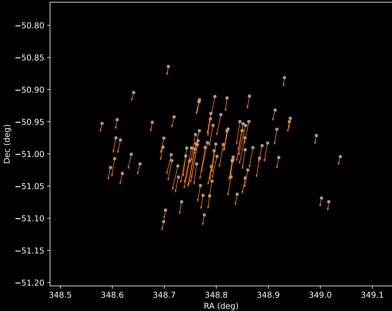
Gaia DR3 Cluster 2 Proper Motion Vectors (n=84)
