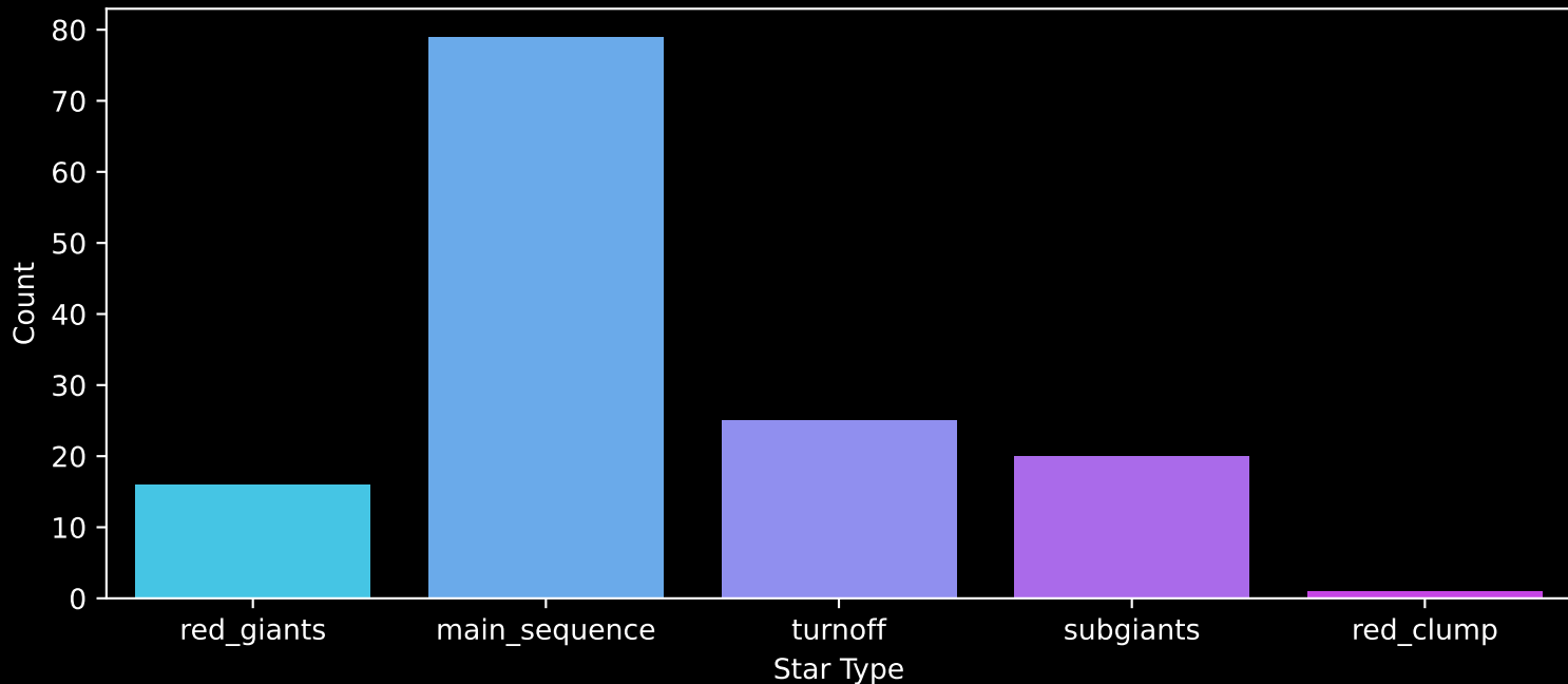
Gaia Cluster: [Collinder_307] Count plot of Star Type
