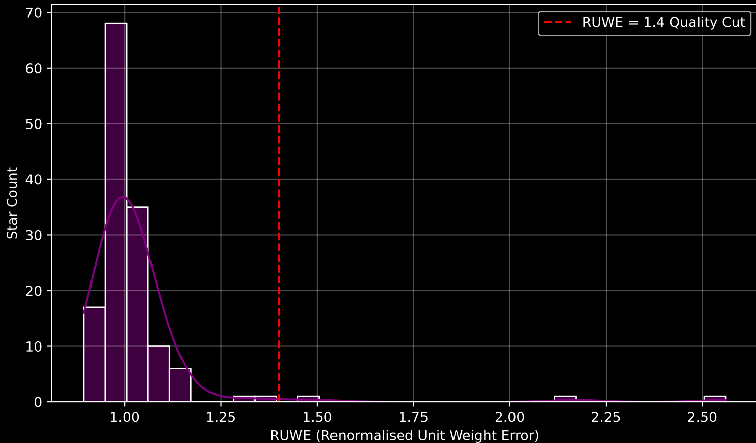
Gaia Cluster: [Collinder_307] RUWE Distribution (n= 141)
