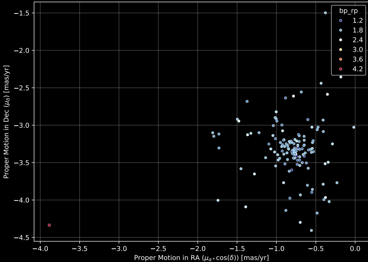
Gaia Cluster: [Collinder_307] Proper Motion Diagram (n= 141)
