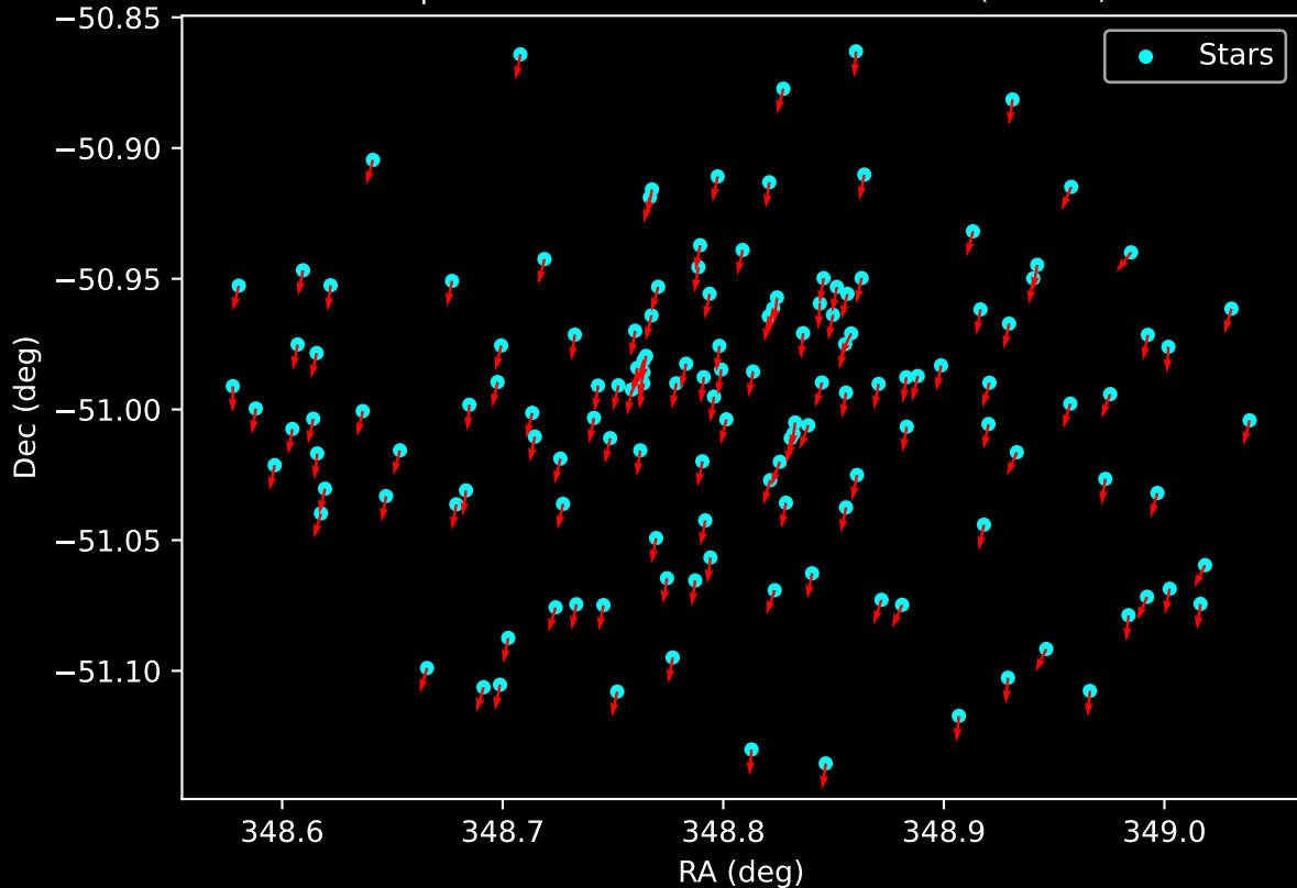
Gaia Cluster: [Collinder_307] Proper Motion Vectors for Gaia Star Field (n= 141)
