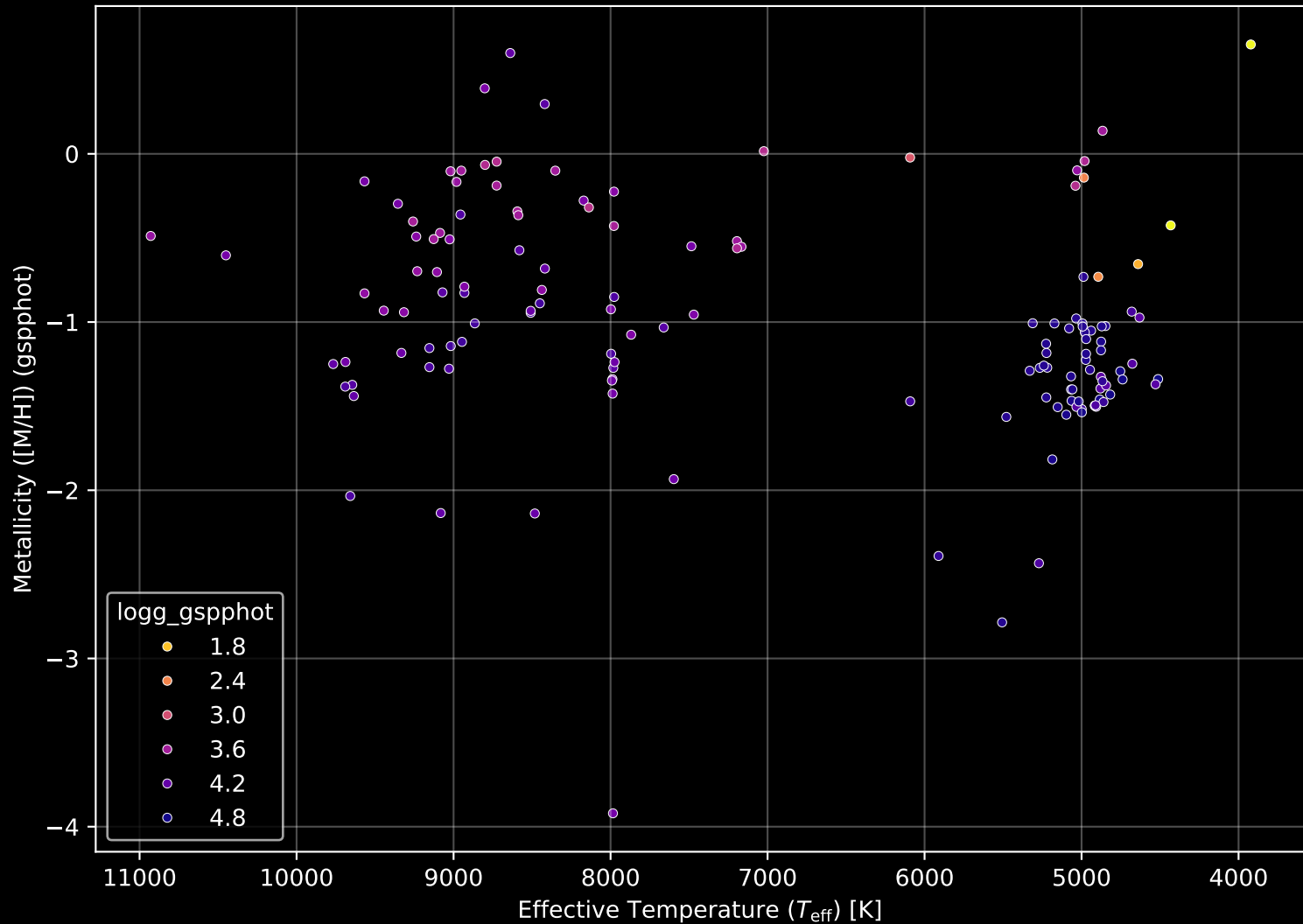
Gaia Cluster: [Collinder_307] Stellar Population Parameters (n= 141)
