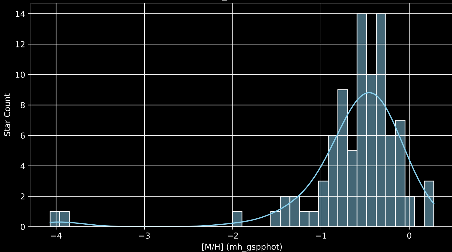
Gaia Cluster: [Collinder_338 [M/H] (mh_gspphot) (n= 89)
