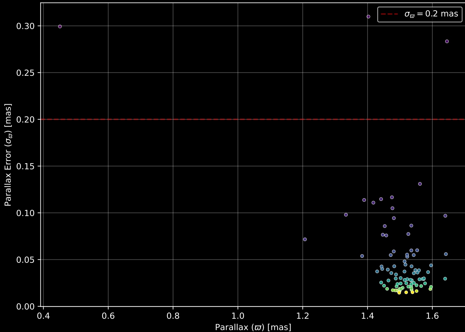
Gaia Cluster: [Collinder_338] Parallax Quality (n= 89)
