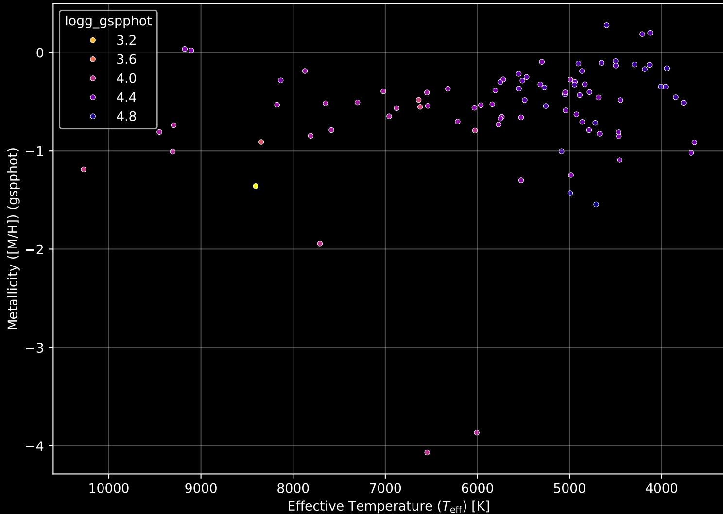
Gaia Cluster: [Collinder_338] Stellar Population Parameters (n= 89)
