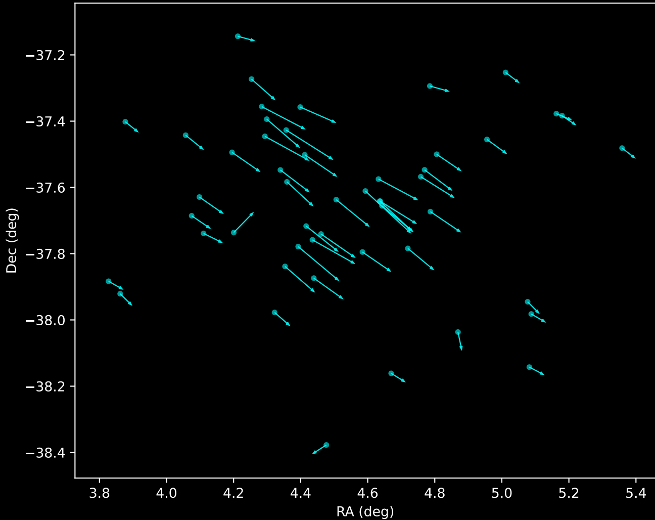
Gaia DR3 Noise Stream Proper Motion Vectors (n=50)
