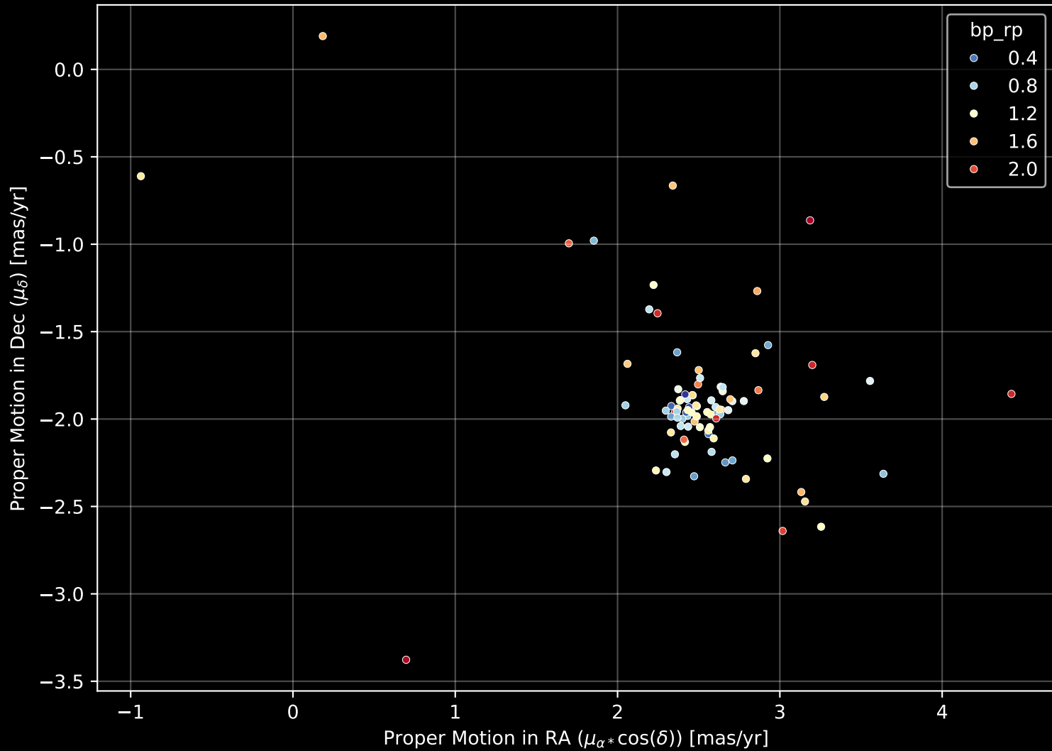
Gaia Cluster: [Collinder_338] Proper Motion Diagram (n= 89)
