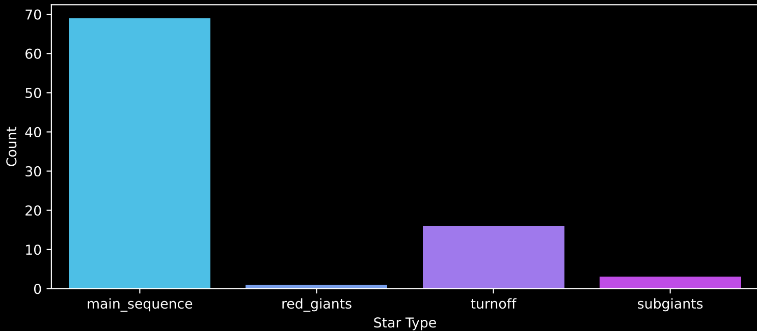
Gaia Cluster: [Collinder_338] Count plot of Star Type
