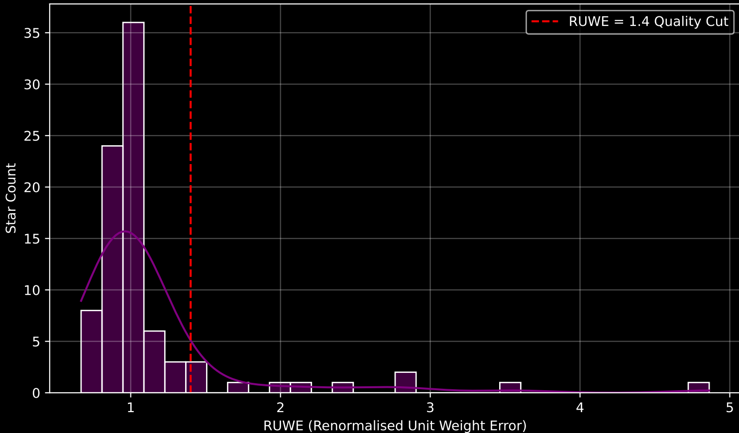
Gaia Cluster: [Collinder_338] RUWE Distribution (n= 88)
